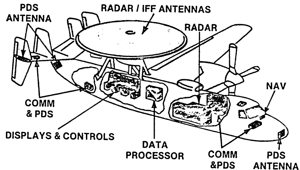
Figure 16.- Major avionics suppliers for advanced Navy aircraft E2C (courtesy Grumman Aerospace Co.).
