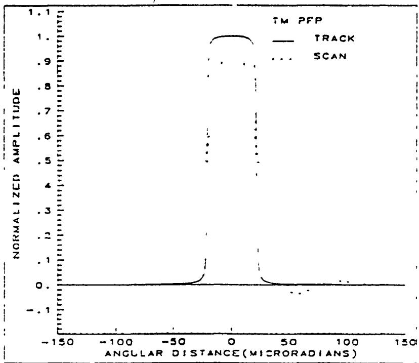
Figure 14a. TM net design LSF's: band 1.
