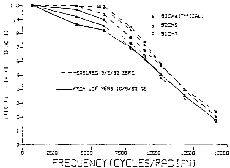
Figure 28a2. TM/F PFP SWR: Measured single channels versus derived from measured LSF.
