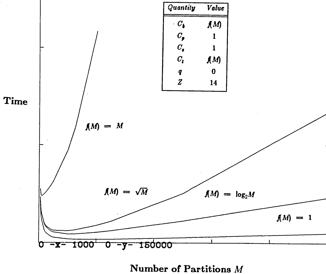
Figure V Execution time for N = 1000
