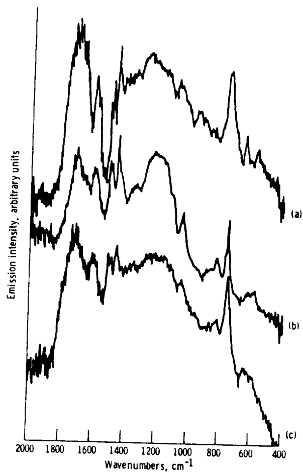
Figure 4. - Emission spectra (100 o C) of deposits produced at 125 o C by dodecane/tetralin spiked with 2 percent thiophene after (a) 6 days, (b) 13 days, and (c) 24 days.
