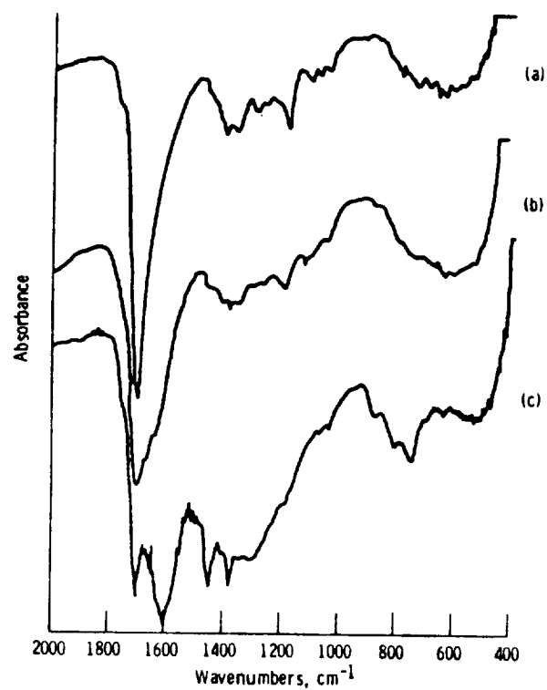
Figure 3. - Absorption spectra of accelerated storage/thermal deposits produced by ERBS spiked with 0.1% pyrrole and stressed at (a) 60°C, (b) 125°C, and (c) 250°C.
