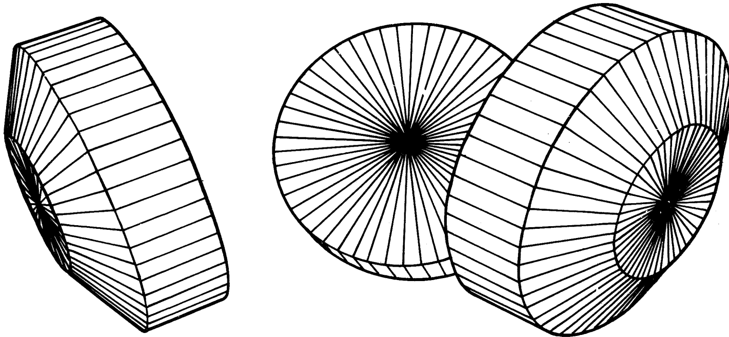
Figure 7. Four Wheel Tetrahedral Configuration for 3-axis Control and Energy Storage
