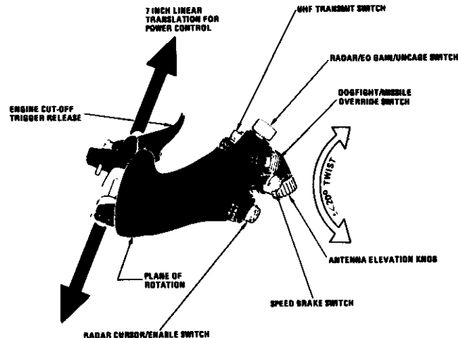
Figure 10 Throttle Twist Grip
