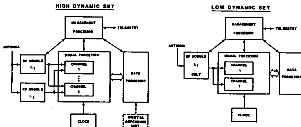
FIGURE 3 INSTRUMENTATION CONCEPTS
