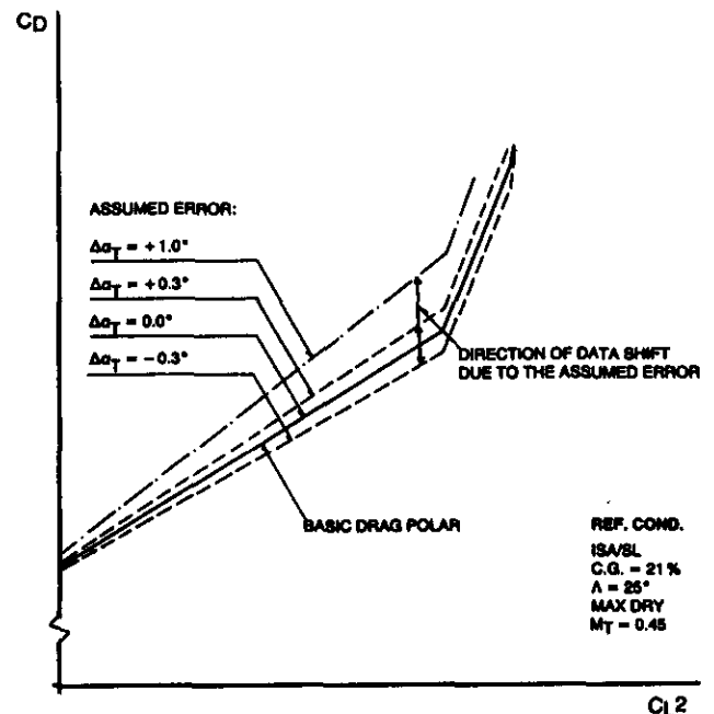
FIG. 10: Effect of Angle of Attack Accuracy on the Drag Polar
