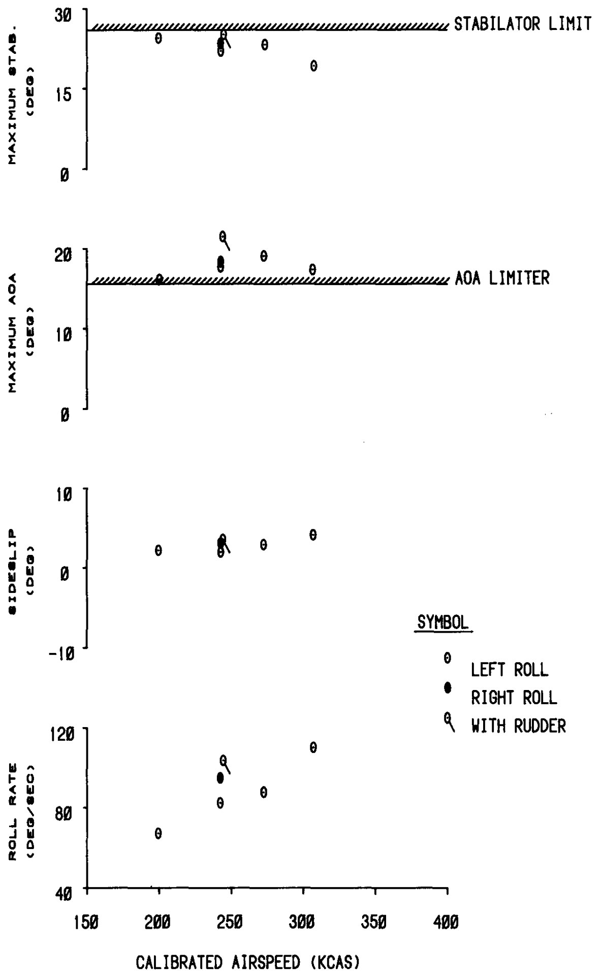
FIGURE 2. MAXIMUM-G ROLLS
