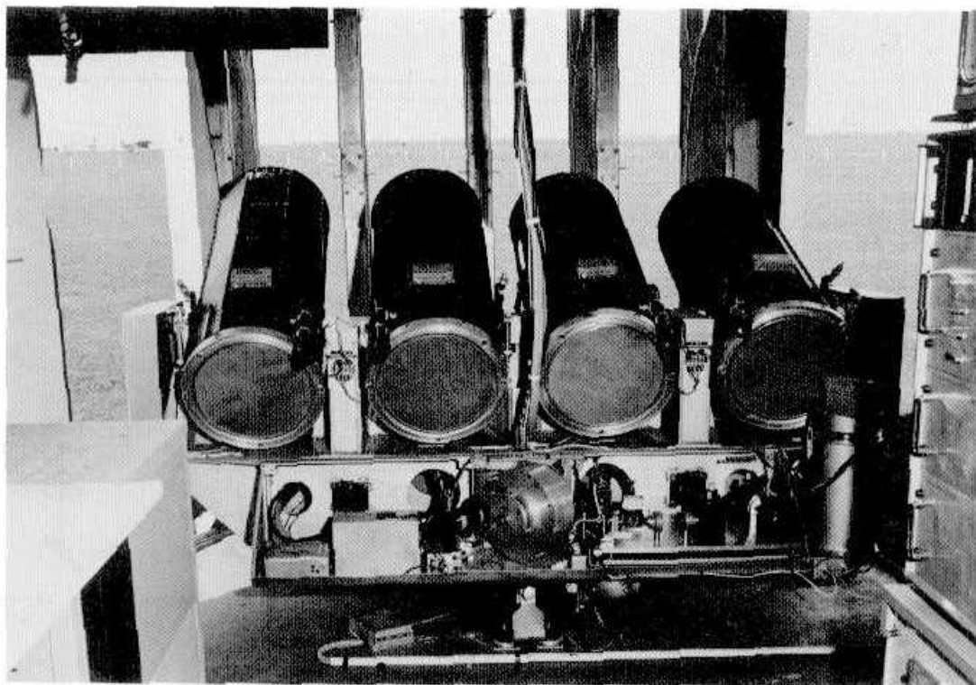
Fig. 1 The Combined Wind And Vortex Experimental Range (CWAVER) equipment. In one mode of operation the outgoing laser beam was switched between the four telescopes in which the range and elevation could be rapidly altered.
