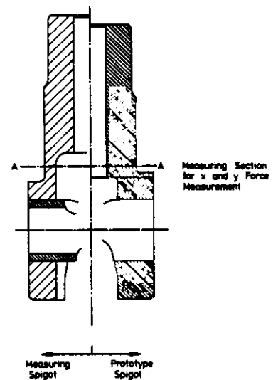
Fig. 10 COMPARISON BETWEEN MEASURING SPIGOT AND PROTOTYPE SPIGOT
