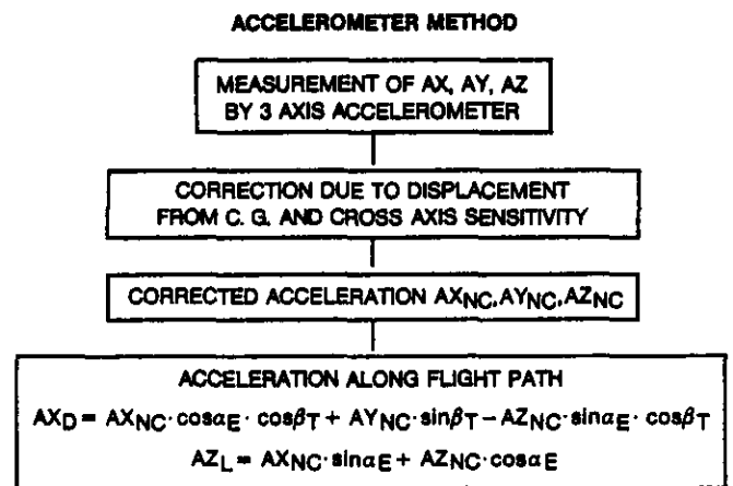
FIG. 7: Accelerometer Method
