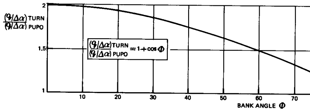
Fig. 9a Comparison between the \frac{q}{\Delta\alpha} ratios for the level turn and the pull-up/push-over (pupo) manoeuvres
