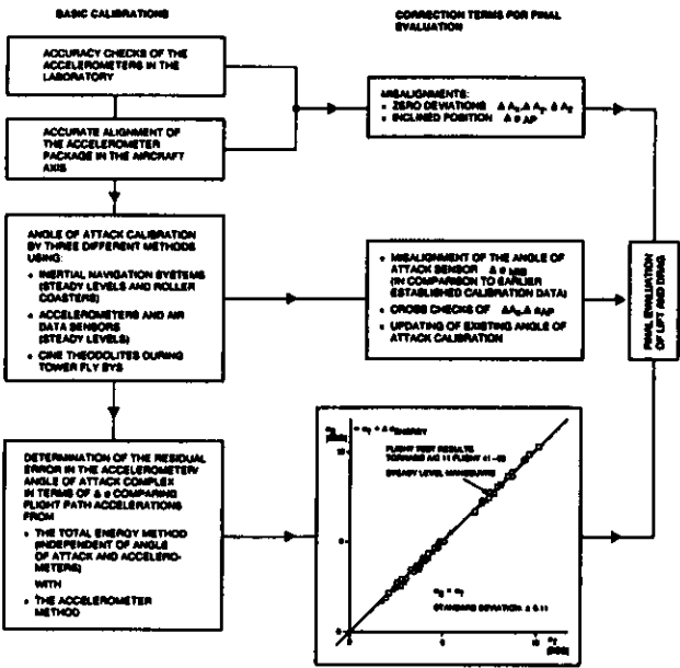
FIG. 11: Procedure of the Incidence/Accelerometer Complex Calibration
