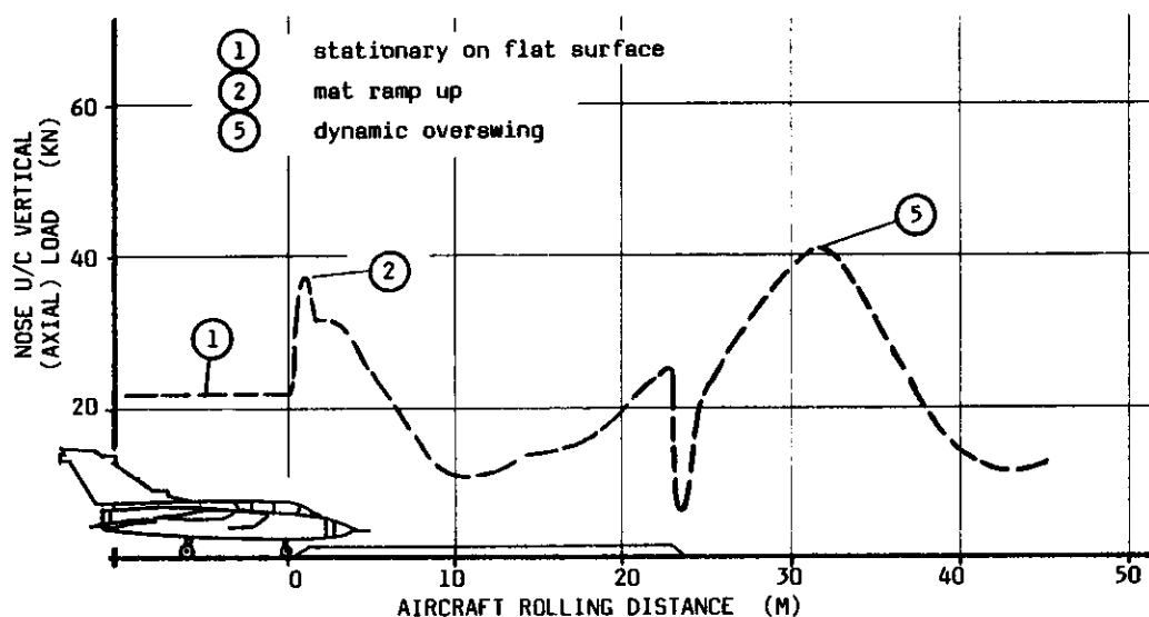
FIG. 7 TYPICAL NOSE U/C LOADS FROM A 60 KTS TRAVERSSION OF A SINGLE AM-2 MAT
