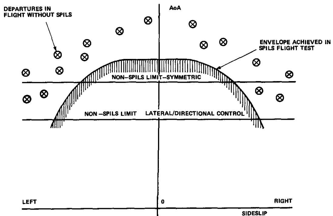
FIGURE 10 SPILS PROTECTION
