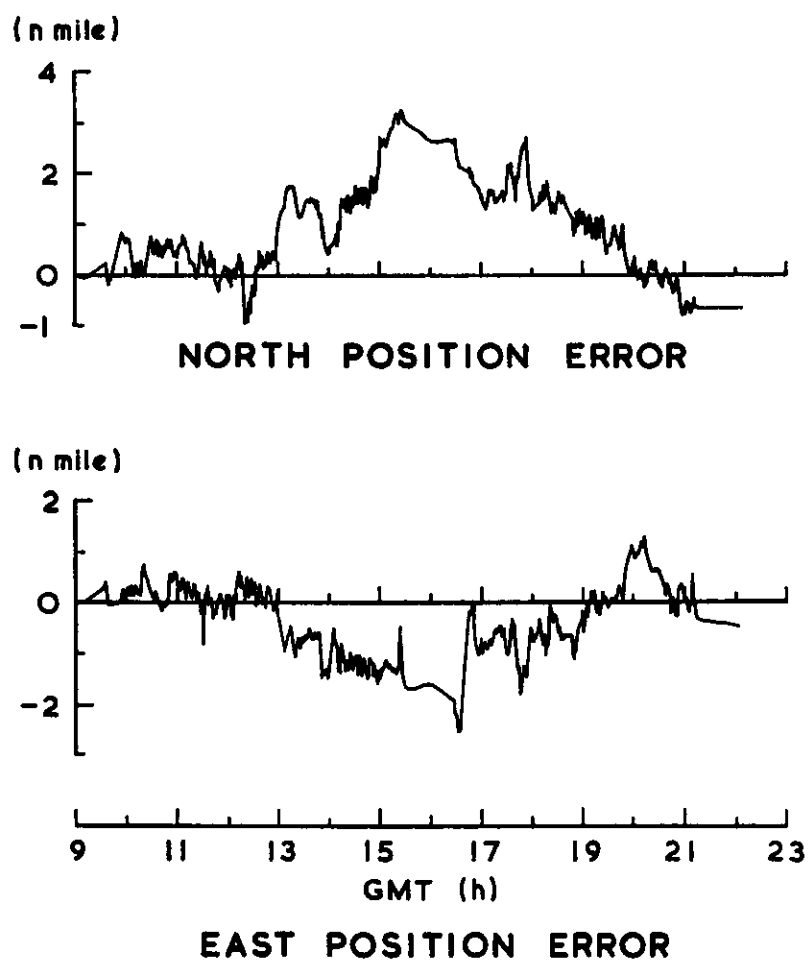
TYPICAL OMEGA POSITION ERRORS
