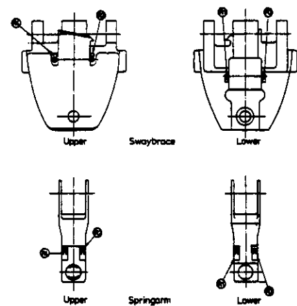
Fig. 12 STRAINING OF AUXILIARY SPIGOT FLD (SHOULDER ADAPTER)
