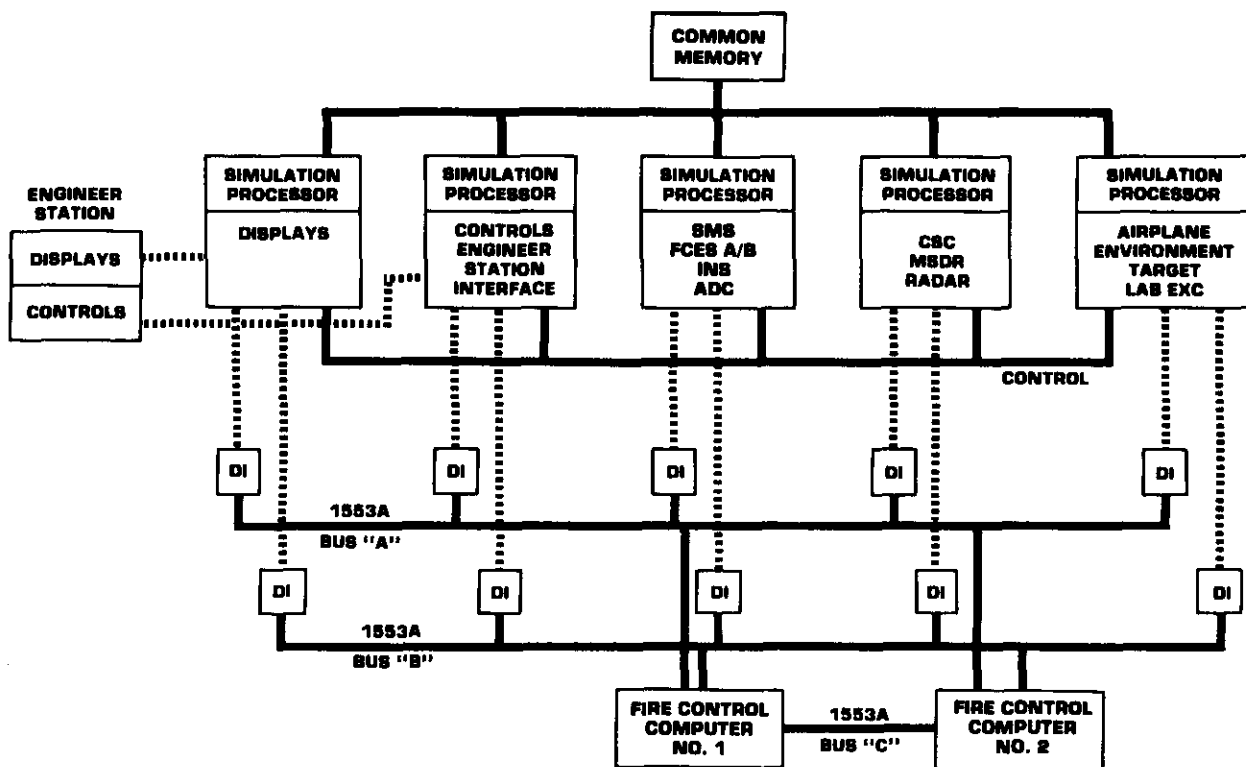
F/A-18 AVIONICS SYSTEM SIMULATION ARCHITECTURE
