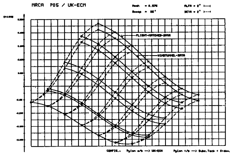
Fig. 9.3 YAW-MOMENT COEF. AT O/B PYLON SPIGOT
