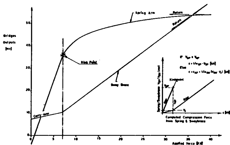
Fig. 15 ERU SPRINGARM/CRUTCHARM BRIDGE RESPONSE AND LOAD COMPUTATION
