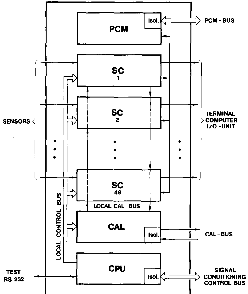
FIG. 4 SIGNAL CONDITIONING UNIT BLOCK DIAGRAM
