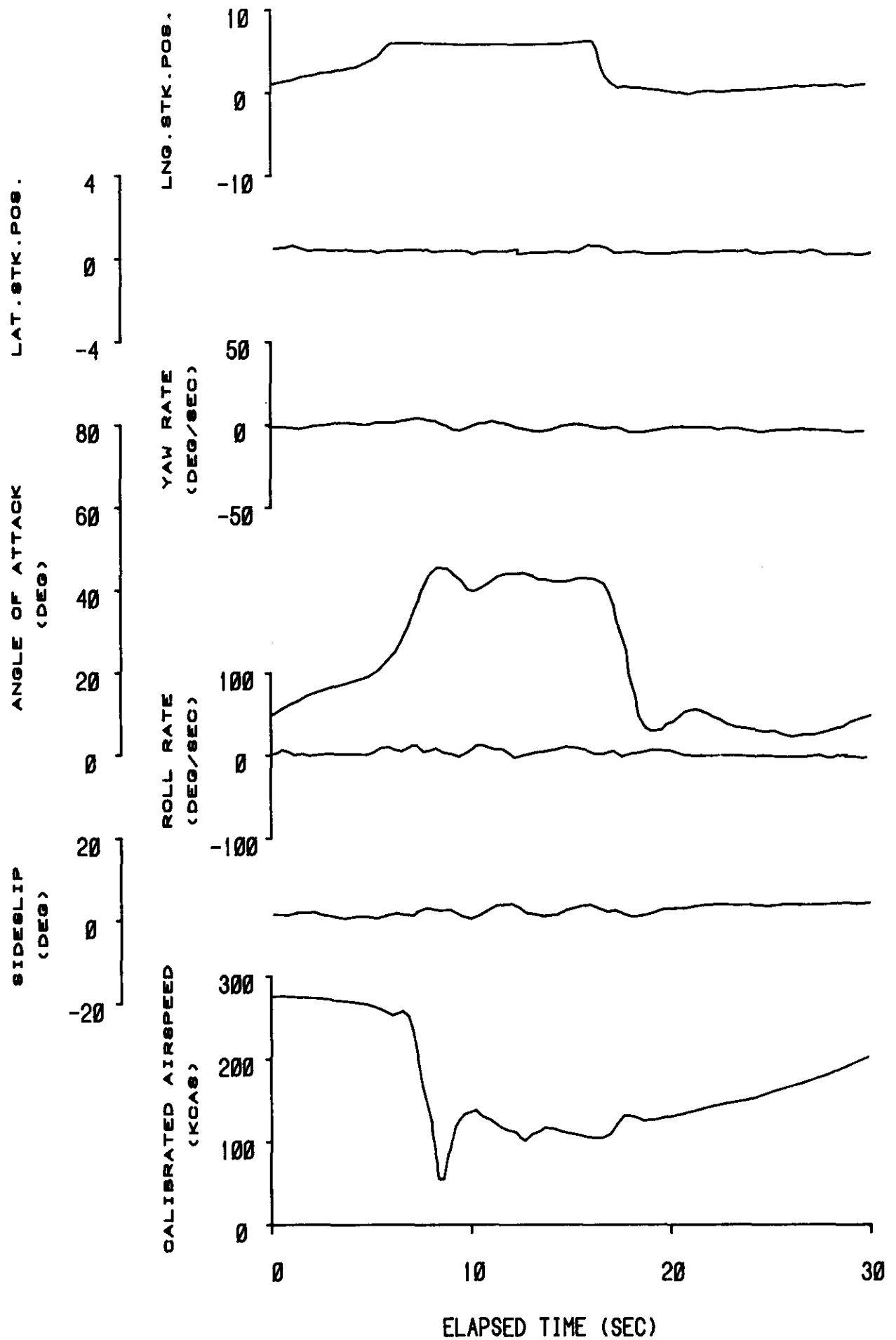
FIGURE 4. WINDUPTURN - NOSEBOOM OFF
