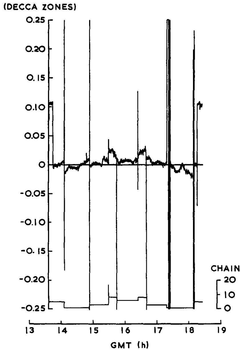
TYPICAL DECCA NAVIGATOR PHASE ERRORS
