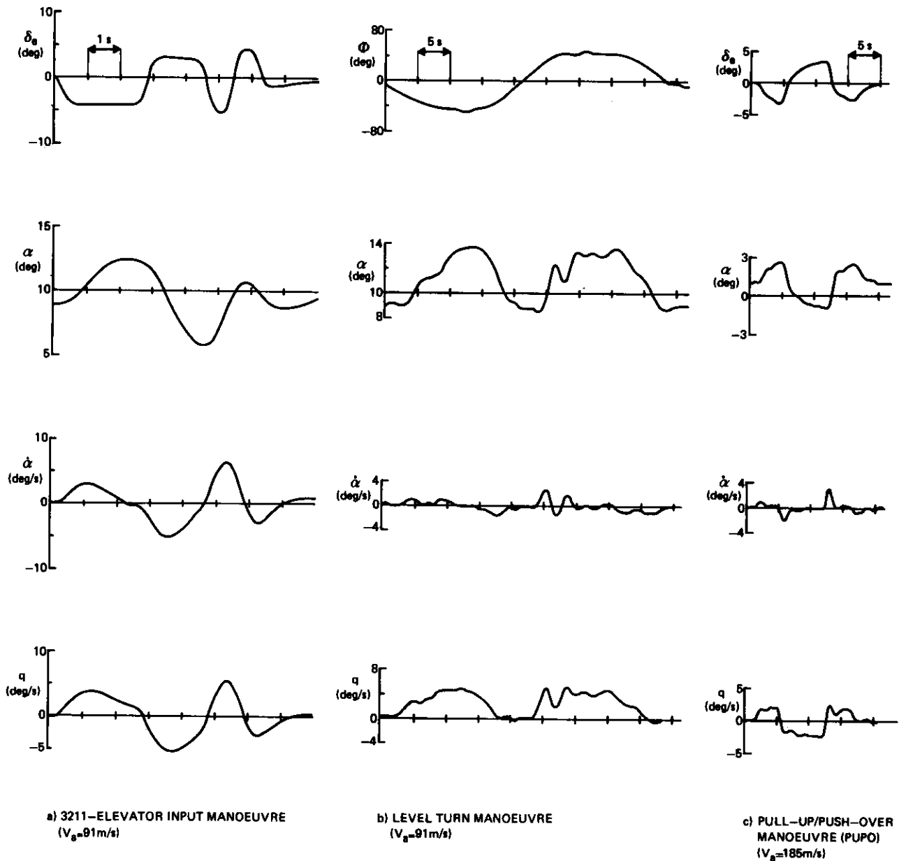
Fig. 8 Time histories of aircraft response during the manoeuvres considered for the determination of the longitudinal stability and control derivatives
