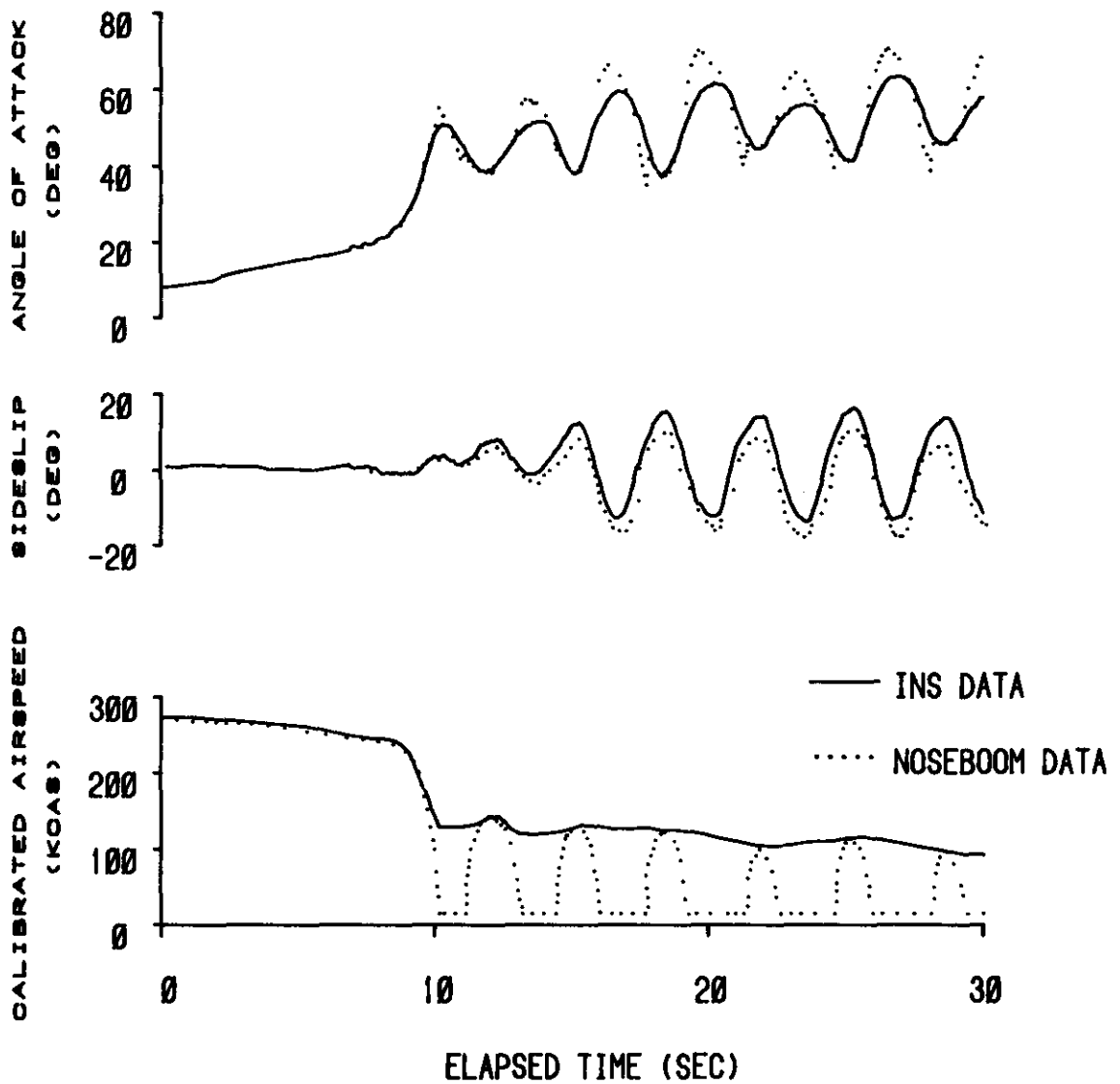
FIGURE 6. NOSEBOOM VS INS DATA COMPARISON
