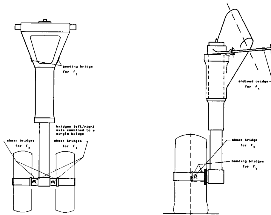
FIG. 3 UNDERCARRIAGE STRAINGAUGE INSTALLATION
