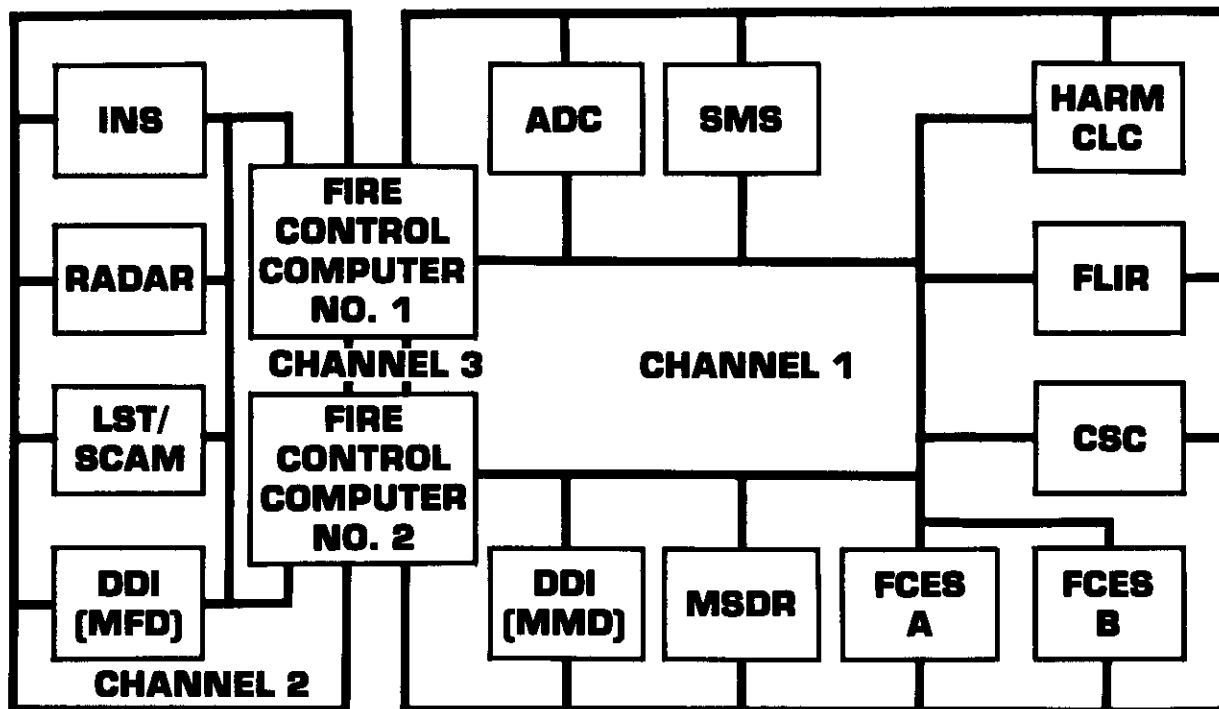
F/A-18 AVIONICS MULTIPLEX BUS SYSTEM
