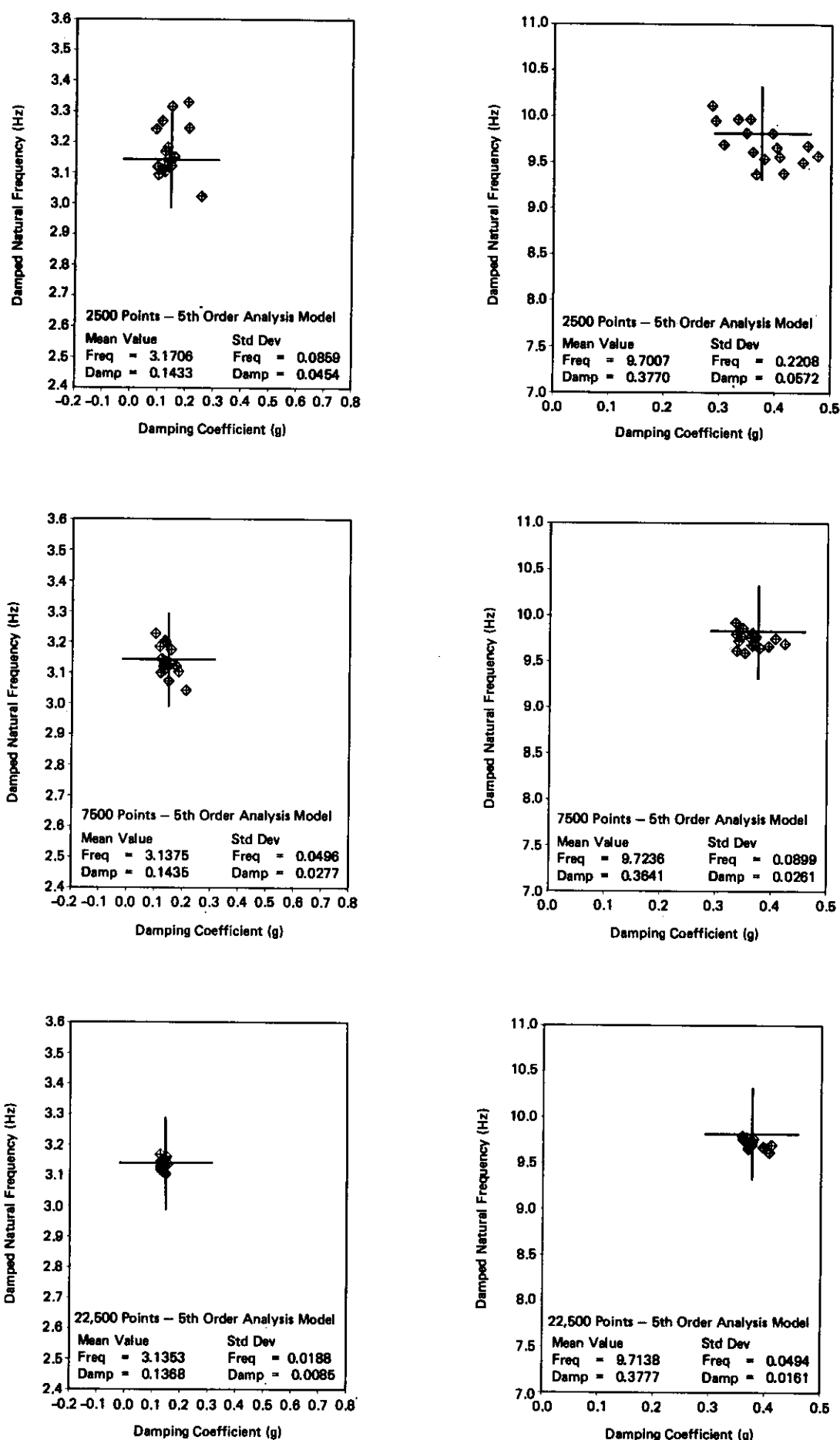
Fig. 8 Scatter Plots of Maximum Likelihood Results on Randomly Excited Data Using a 5th Order Analysis Model
