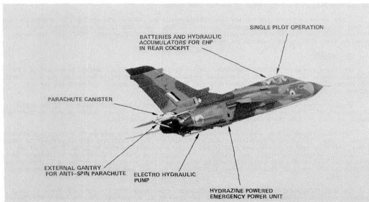
FIGURE 2 SAFETY DEVICES
