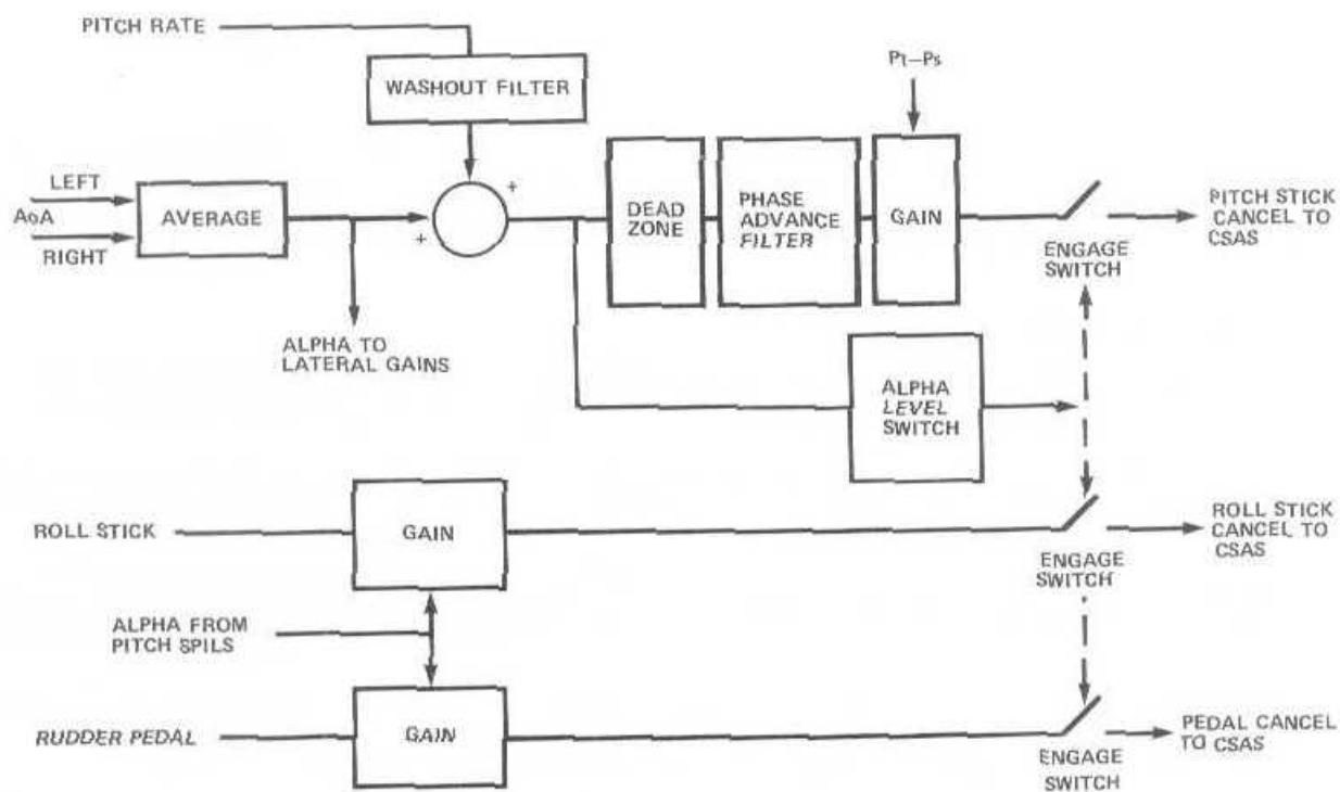
FIGURE 1 SPILS FUNCTIONS
