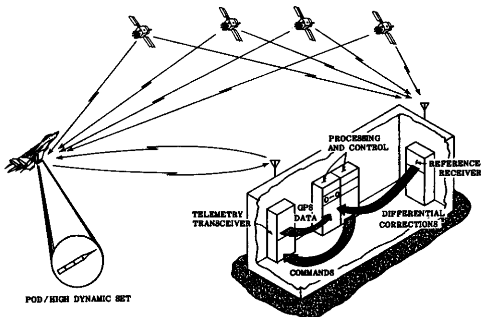
FIGURE 4 POD SYSTEM CONCEPT
