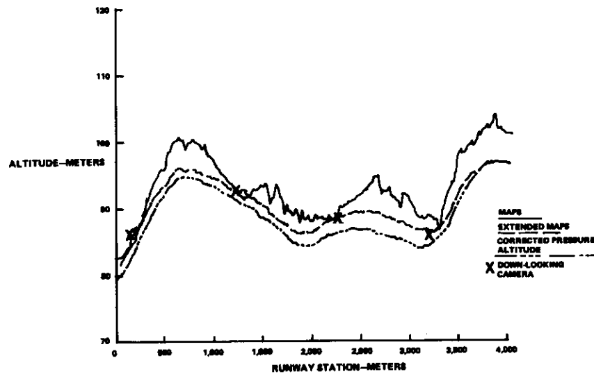
Figure 9. MAPS Acceptance Test
