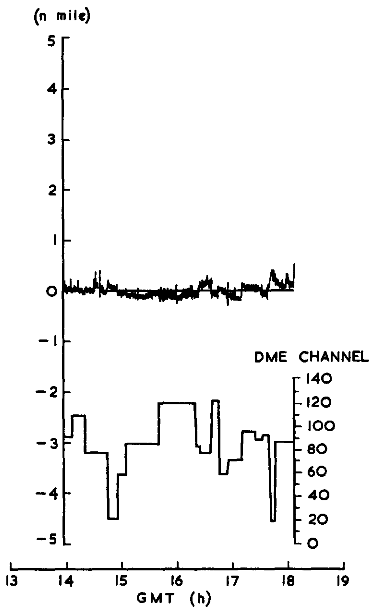
TYPICAL DME RANGE ERRORS
