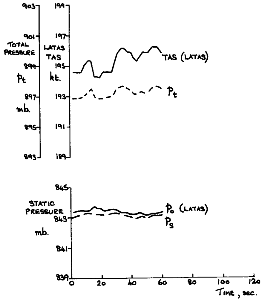
Fig. 11 Time history of recorded data and derived static pressure. 5000 ft altitude and negligible turbulence.
