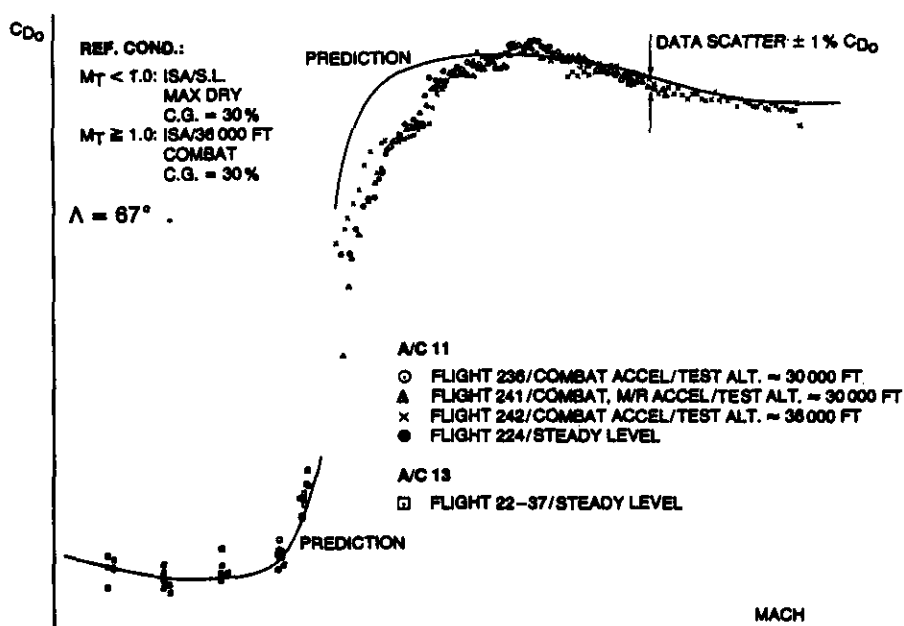
FIG. 18: Zero Lift Drag Variation with Mach
