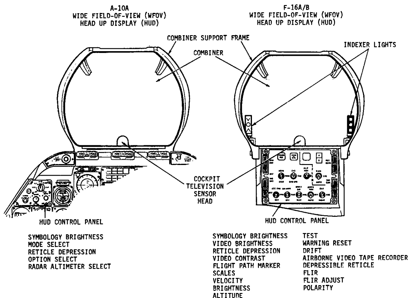
FIGURE 5 A-10 (LEFT) AND F-16 (RIGHT) WIDE FIELD-OF-VIEW HEAD UP DISPLAY
