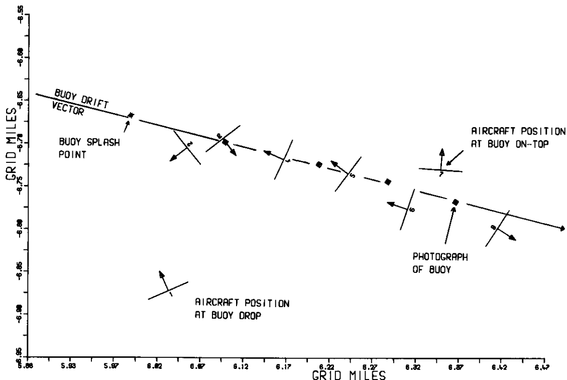
FIGURE 8 - CALCULATION OF SONOBUOY DRIFT VECTOR BY PHOTOGRAPHIC ON-TOP METHOD
