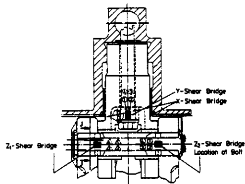
Section J-J
