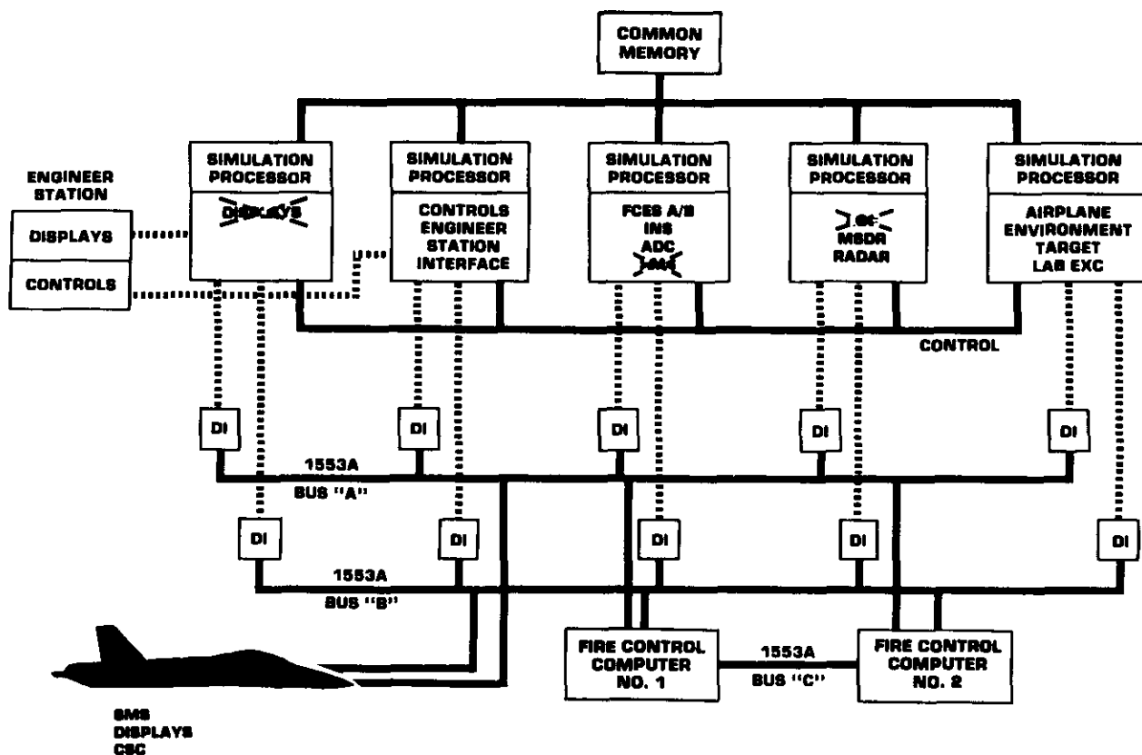
AIRCRAFT IN THE LOOP SIMULATION ARCHITECTURE
