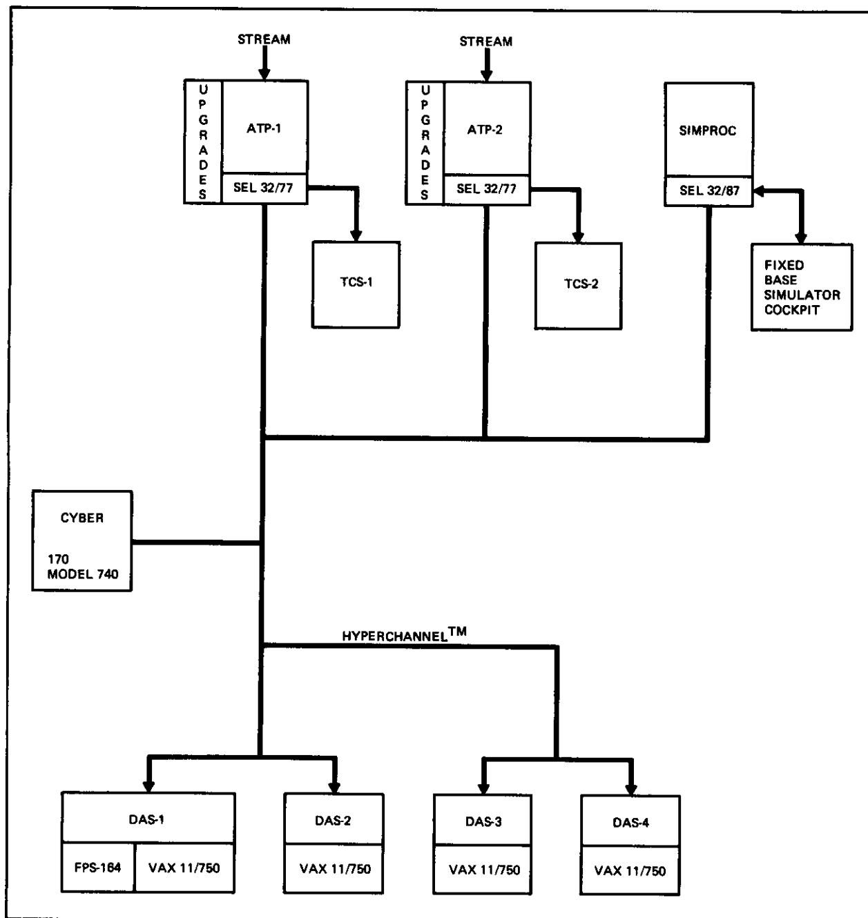
Fig. 3 NDCS Baseline Configuration
