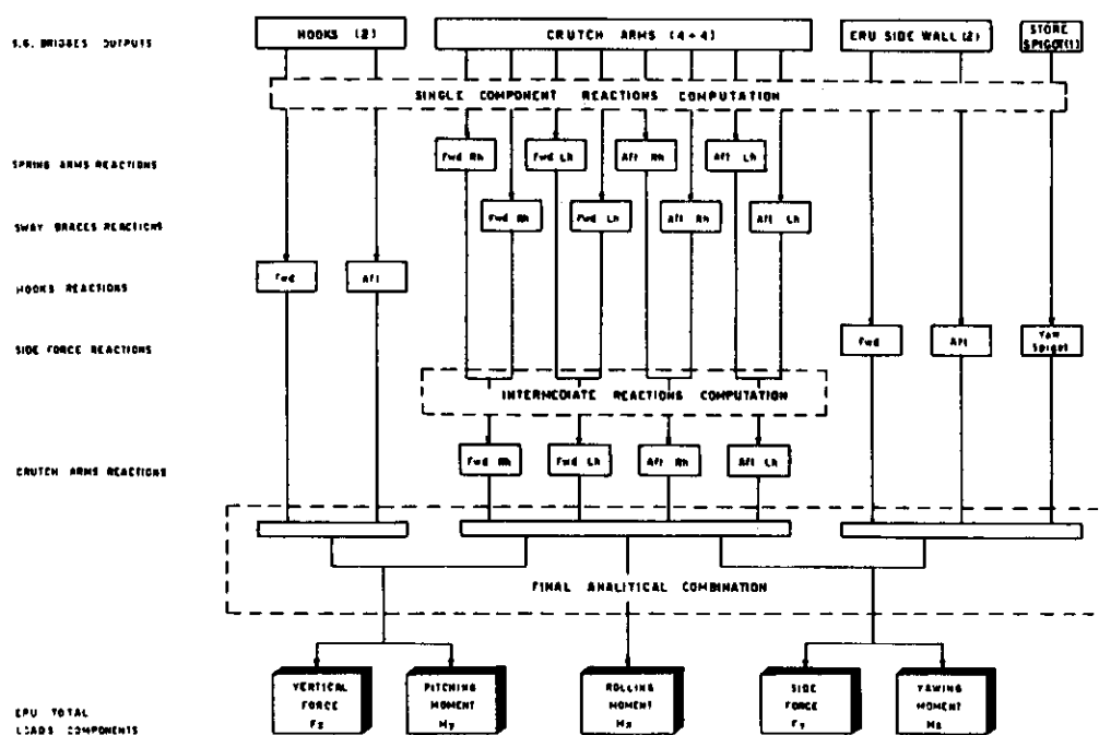
Fig. 20 30° HM-ERU TOTAL LOADS COMPONENTS CALCULATION
