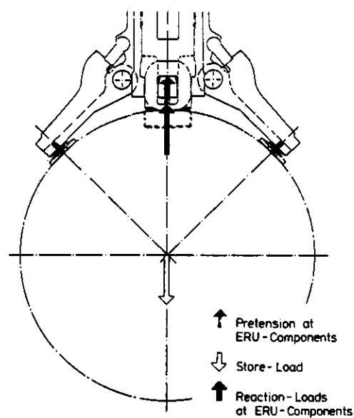
Fig.19 PRINCIPLE OF REACTION-LOAD OF ERU-COMPONENTS
