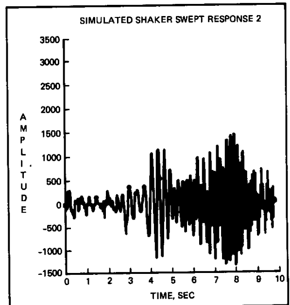
Fig. 10 Typical Time History for 2nd Simulated Swept Frequency Measurement
