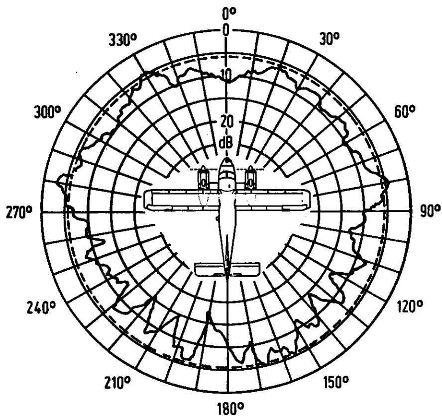
Fig. 7: Antenna Radiation Pattern
