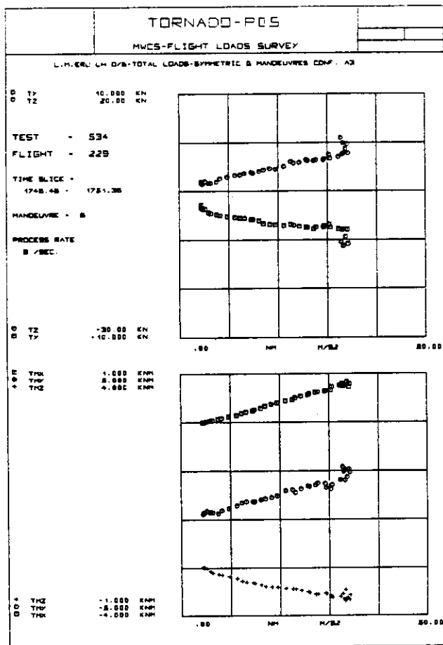
Fig.22 EXAMPLE OF FLIGHT TEST DATA PRESENTATION
