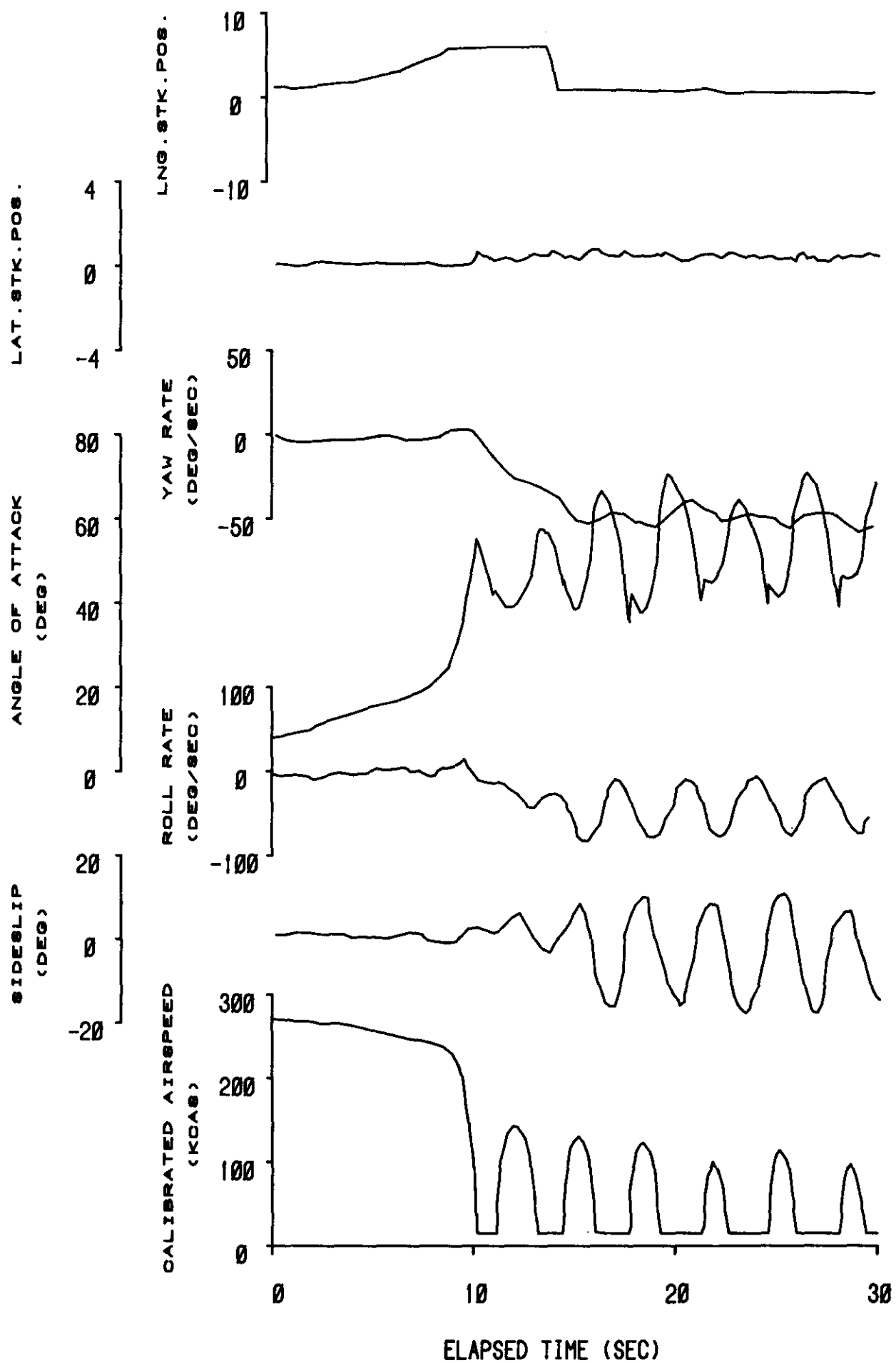
FIGURE 3. WINDUPTURN - NOSEBOOM ON
