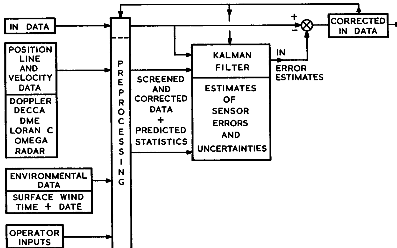
FORM OF THE INTEGRATED NAVIGATION SYSTEM FIG 2
