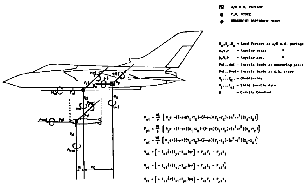
Fig. 21 INERTIA LOADS COMPUTATION AT MEASURING POINT
