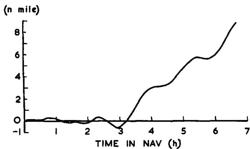
EAST POSITION ERROR
