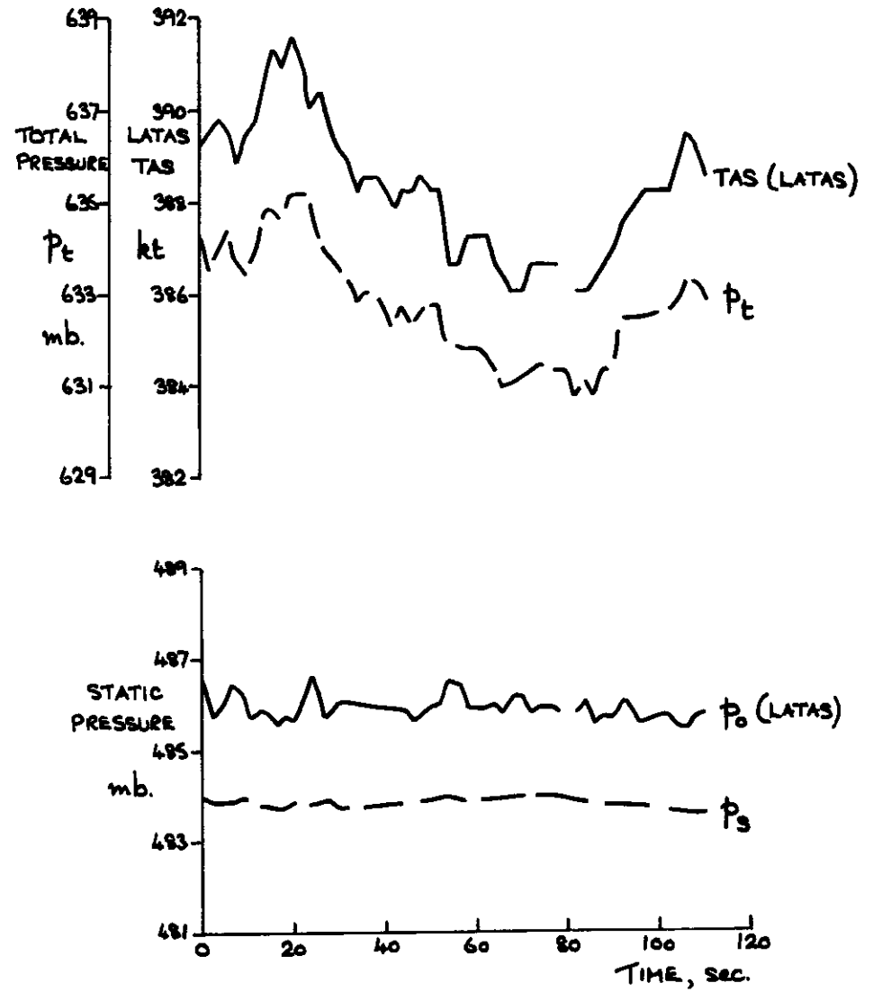
Fig. 12 Time history of recorded data and derived static pressure. 19000 ft altitude and detectable clear air turbulence.
