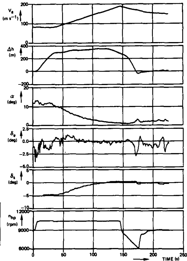
Fig. 3 Time histories of the motion and control variables during an accelerated run
