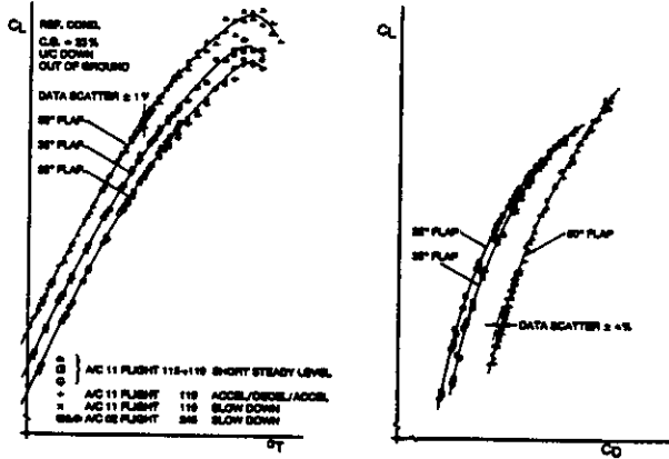
FIG. 15: Low Speed/High Lift Configuration
