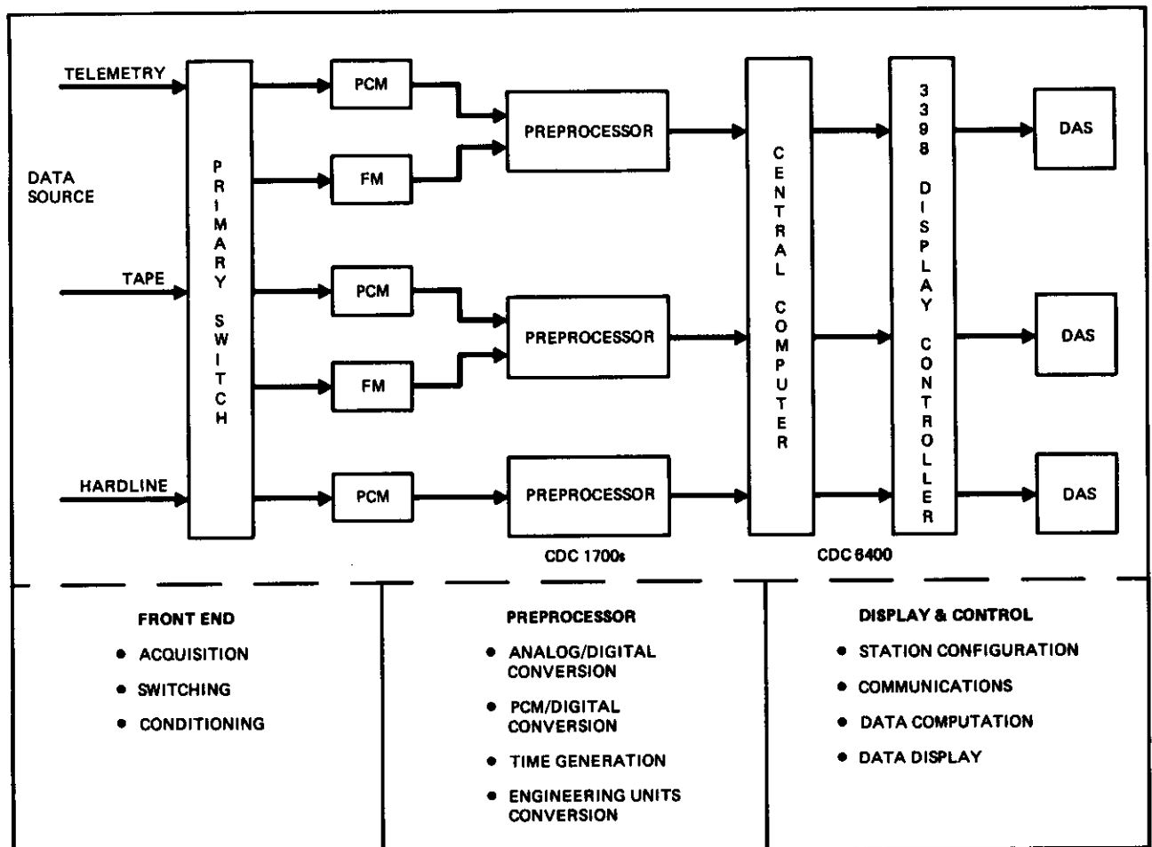
Fig. 1 ATS -Original Flight Test System
