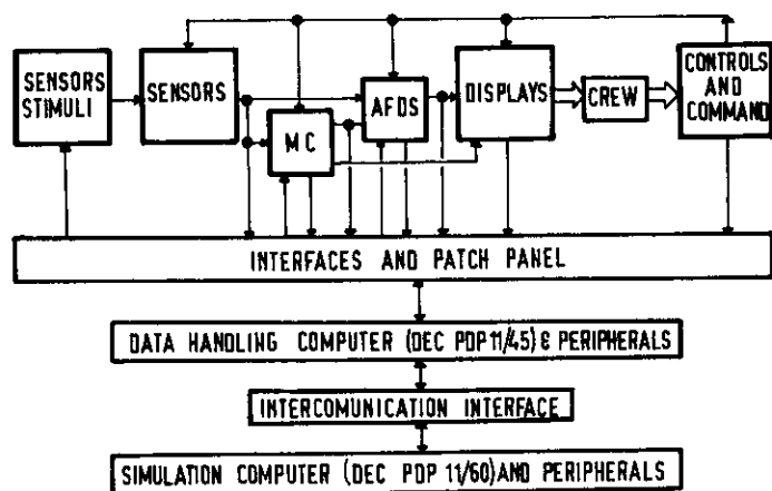
FIGURE 9 - CLOSED LOOP SYSTEM SET UP
