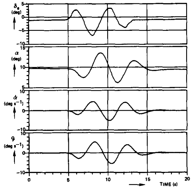
Fig. 6 Time histories of the sinusoidal elevator input signals and the resulting aircraft response
