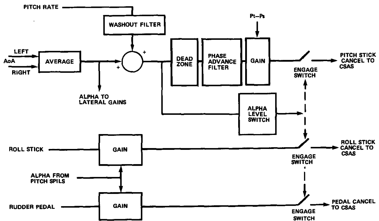
FIGURE 1 SPILS FUNCTIONS
