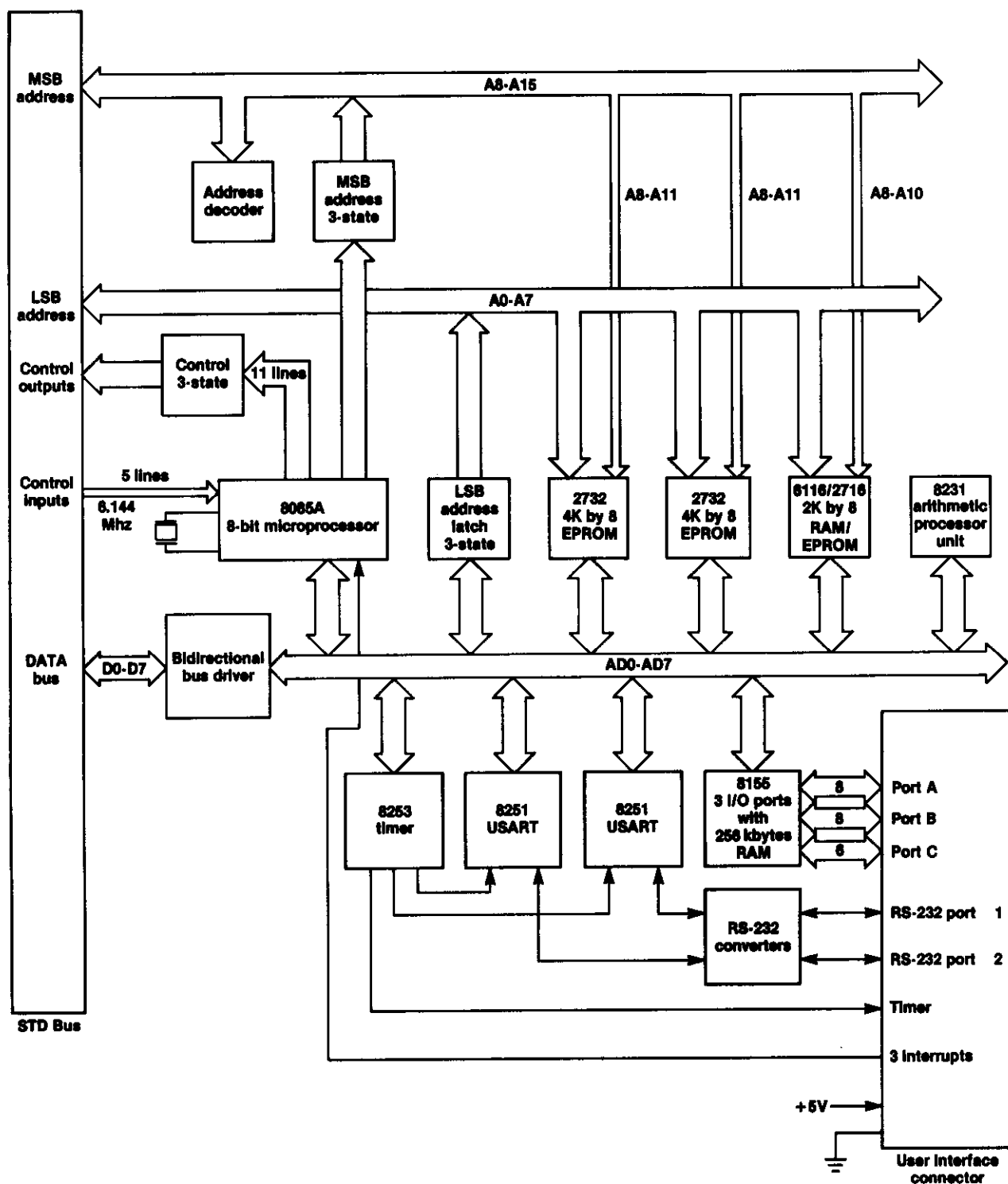
Figure 3. Simplified block diagram of a single-board microcomputer.
