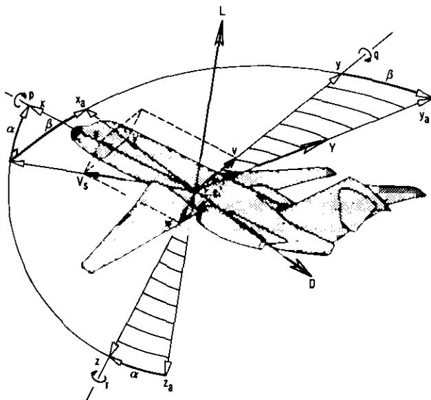
Fig. 1 Body fixed and air-trajectory reference frames
