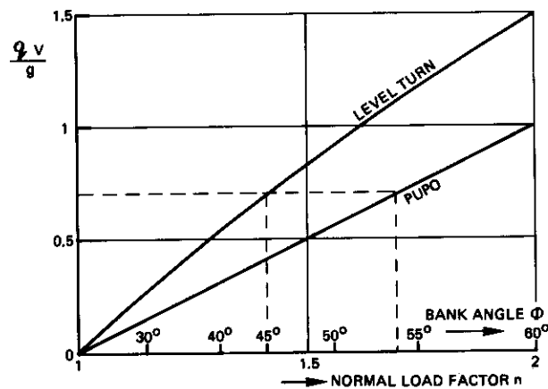
Fig. 9b Amount of pitch rate produced by the level turn and the pull-up/push-over manoeuvres as a function of the normal load factor
