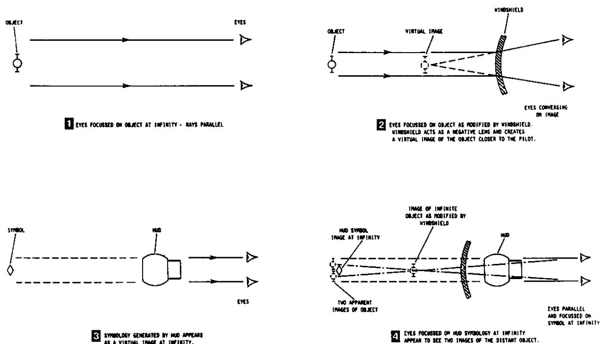
FIGURE 10 F-16 WIDE FIELD-OF-VIEW HEAD UP DISPLAY DECOLLIMATION EFFECT.
