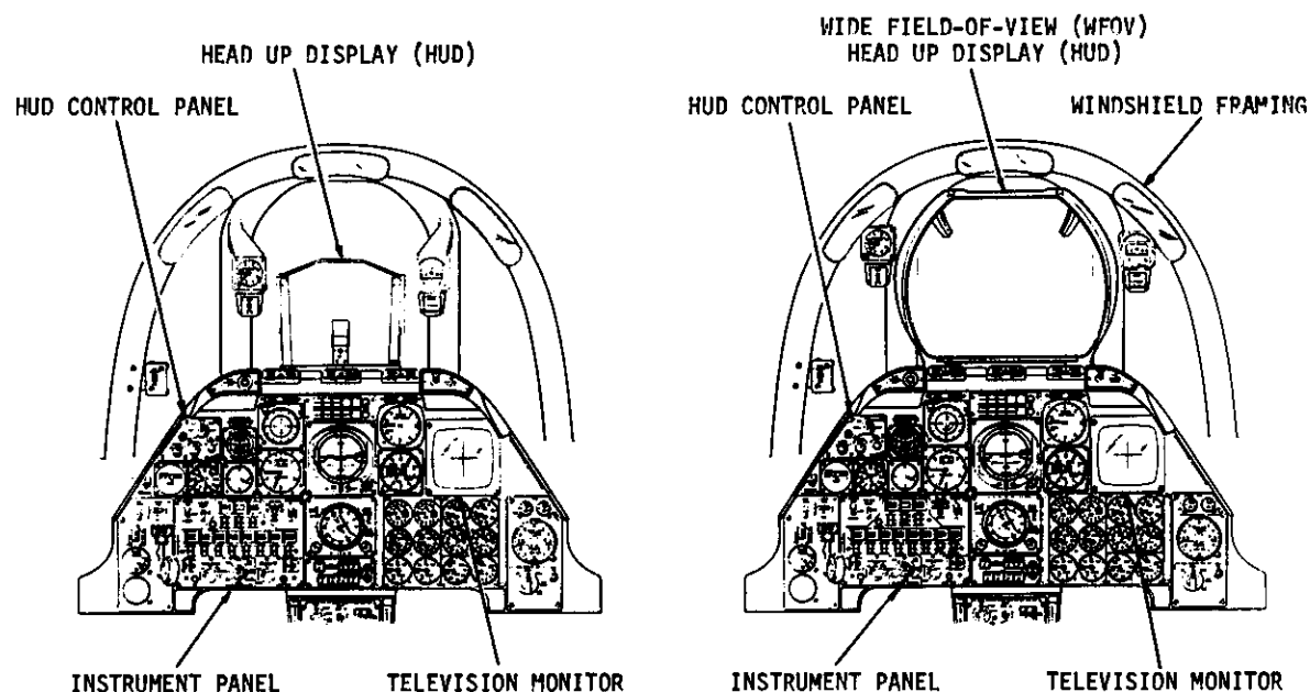
FIGURE 3 A-10 INSTRUMENT PANEL CONFIGURATION PRE- AND POST- LANTIRN SYSTEM INCORPORATION INCLUDING THE WIDE FIELD-OF-VIEW HEAD UP DISPLAY.
