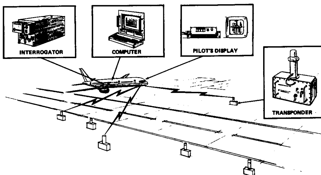
Figure 1. Microwave Airplane Positioning System Components
