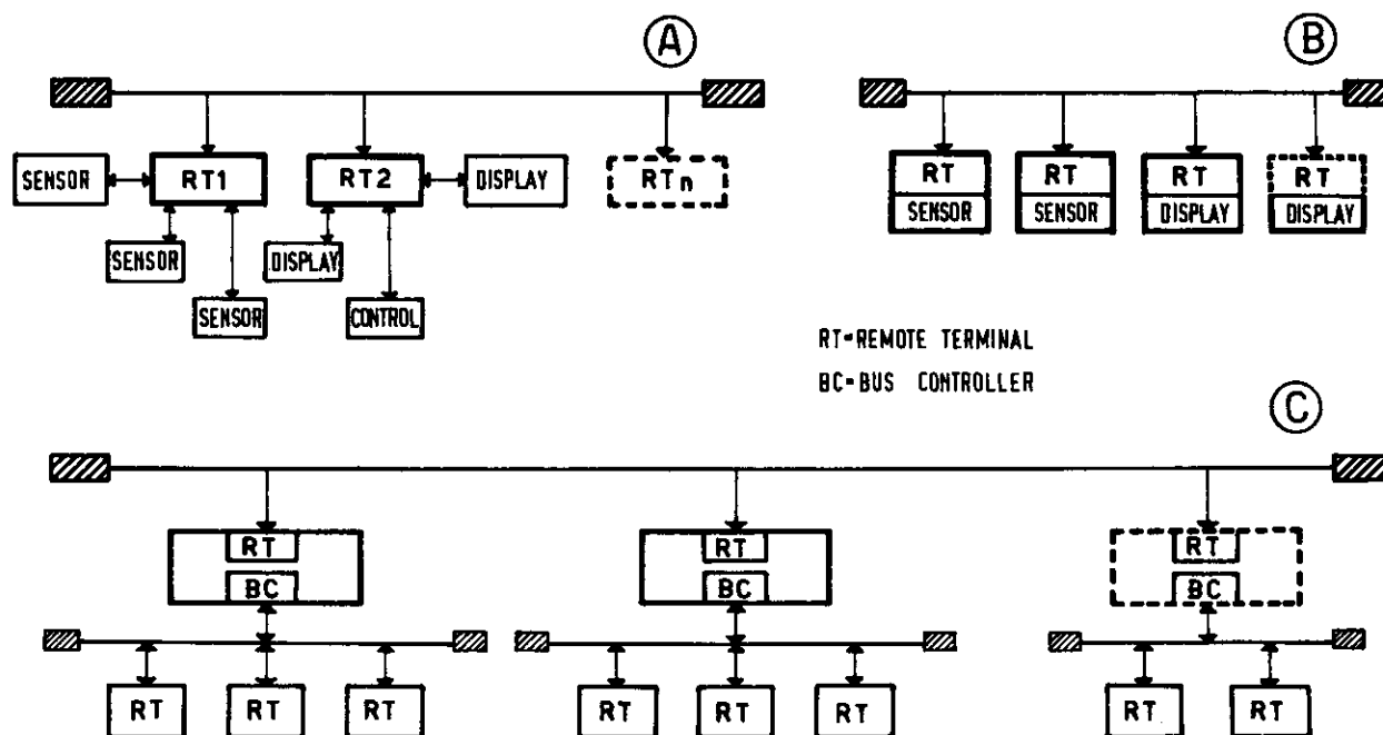
FIGURE 3 - DATA BUS SYSTEM STRUCTURE
