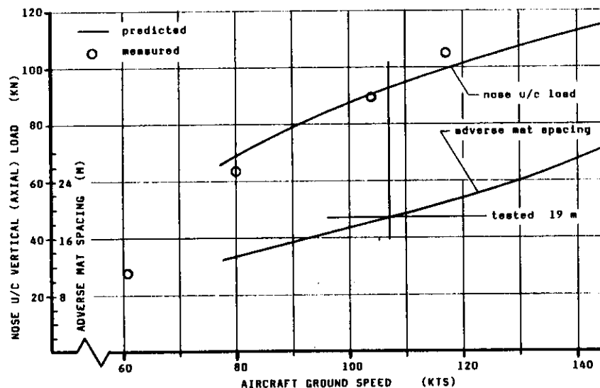
FIG. 18 NOSE U/C VERTICAL (AXIAL) LOAD ON THE 2ND MAT RAMP IN MAX DRY T/R DECELERATION AFTER LANDING
