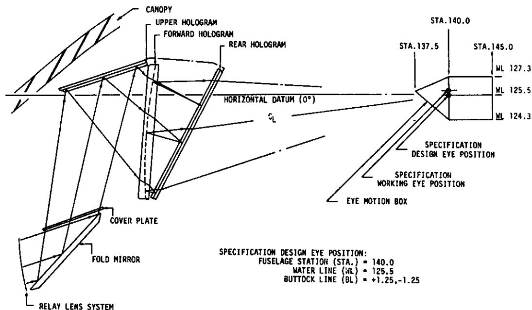
FIGURE 11 F-16 SPECIFICATION DESIGN EYE POSITION AND HEAD MOTION BOX.
