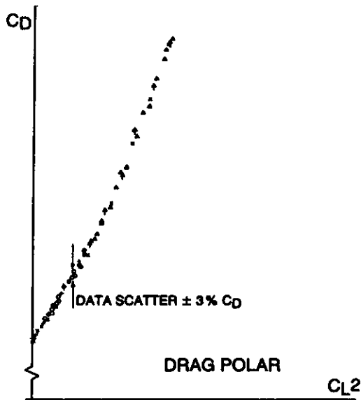
FIG. 14: Repeatability of Flight Test Data
