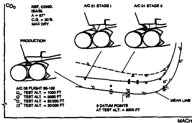
FIG. 16: Airframe Optimization
