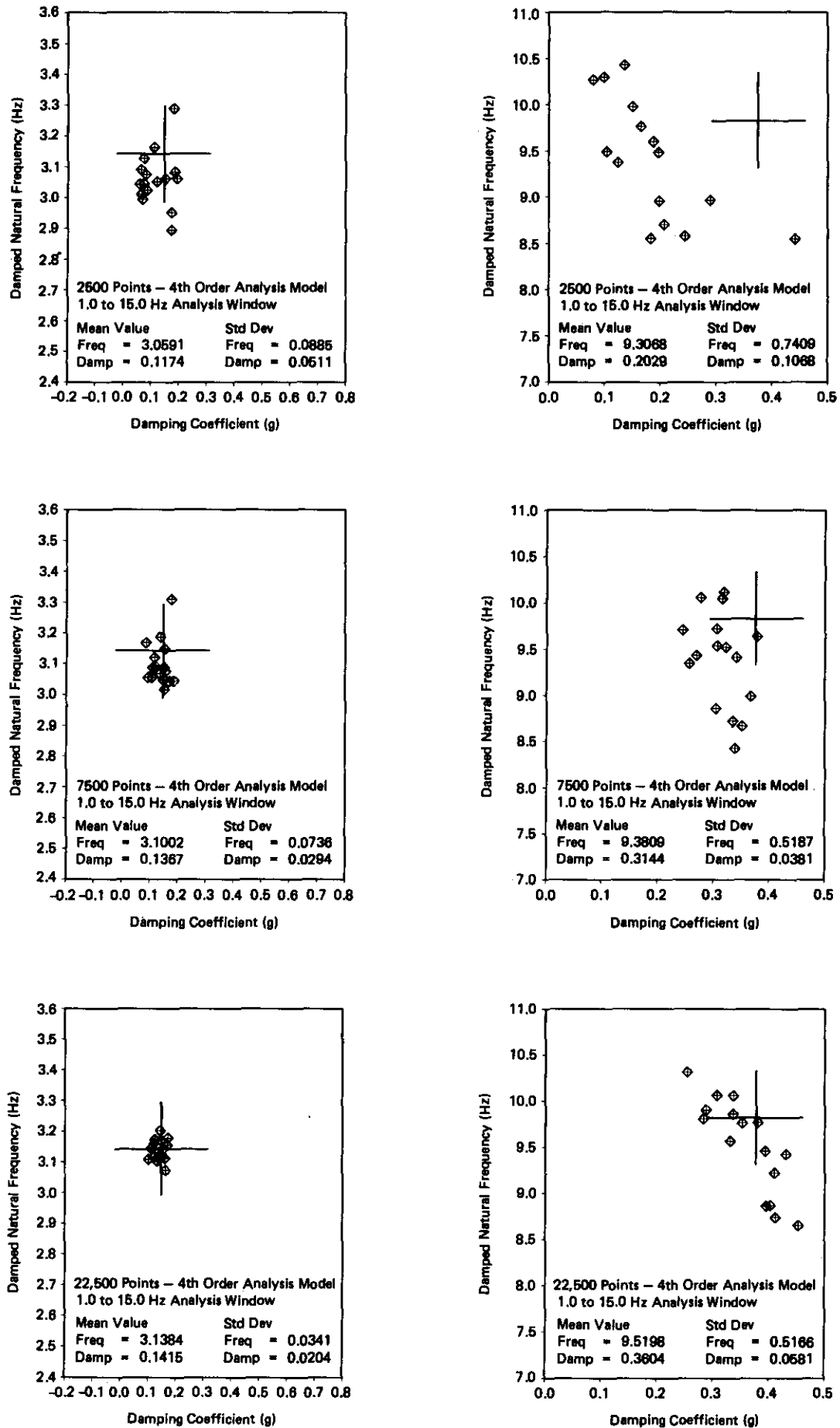
Fig. 16 Scatter Plots of Least-Squares Results on Randomly Excited Data
