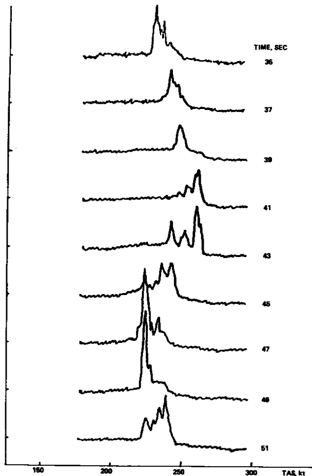
Fig. 17 Successive LATAS Doppler spectra on passage through a thunderstorm microburst. The reference times are the same as for figures 14 and 16 (Flt 792, pm 14 July 1982, run 3).
