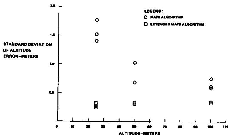
Figure 5. Simulator Data
