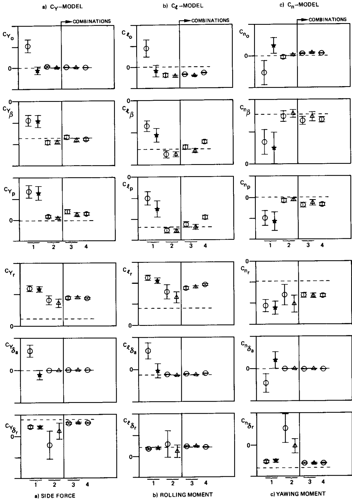
Fig. 13 Coefficients of the lateral-directional model as derived from flight test measurements
