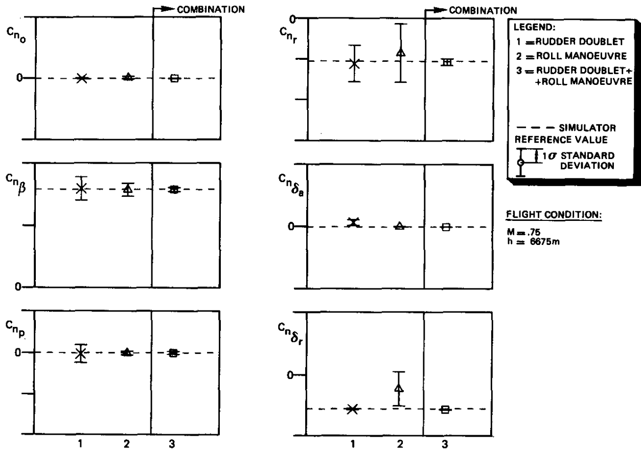
Fig. 12 Coefficients of the yawing moment model as derived from the simulated data
