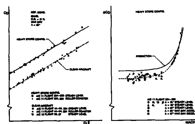
FIG. 19: External Store Drag
