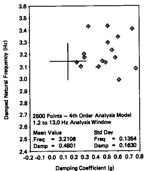
Fig. 17 Scatter Plots for Least-Squares Results on Data Excited Via a 10 sec Shaker Sweep
