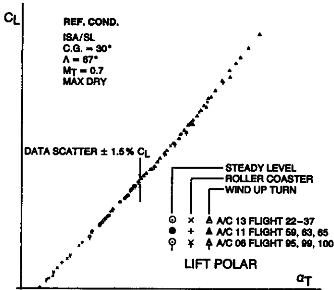
FIG. 14: Repeatability of Flight Test Data
