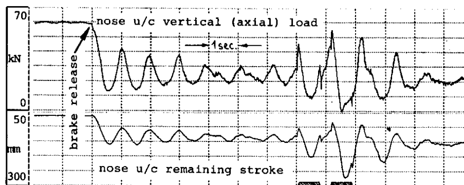
FIG. 13 NOSE U/C LOADS OSCILLATIONS FROM BRAKE RELEASE AT HIGH POWER SETTING
