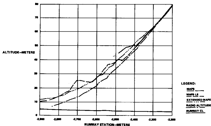
Figure 12. 767 Takeoff With Reversed Input
