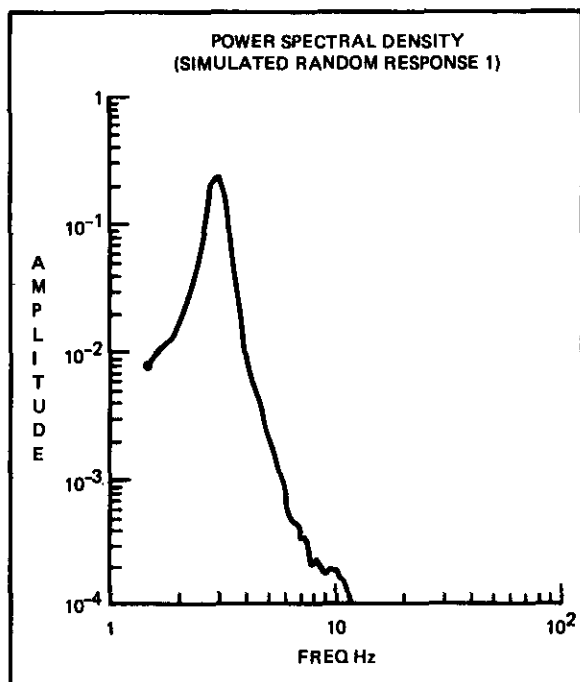
Fig. 5 Typical Power Spectral Density for 1st Simulated Randomly Excited Measurement
