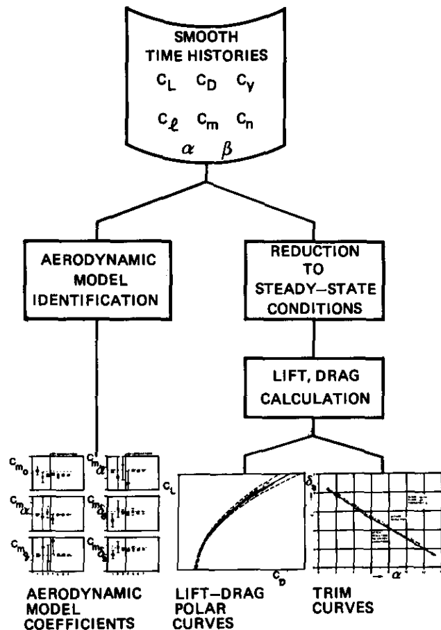
Fig. 2b Analysis of dynamic manoeuvres
