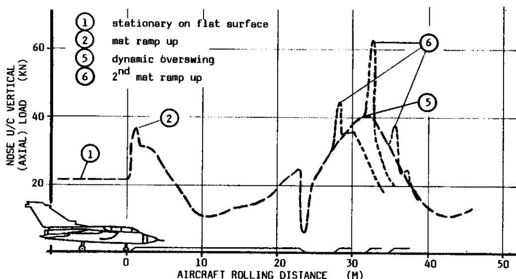
FIG. 9 TYPICAL NOSE U/C LOADS RESPONSES ON THE RAMP OF A SECOND MAT
