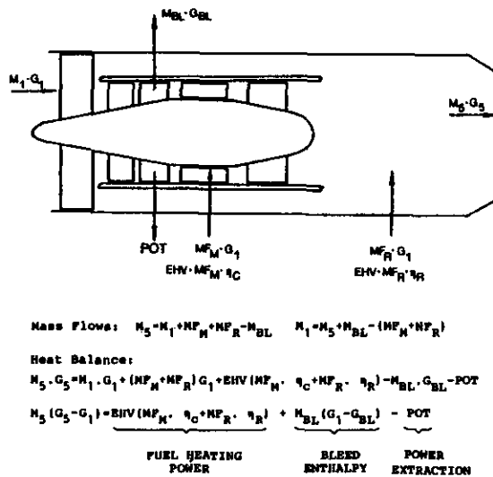
FIG. 5: Heat Balance Method
