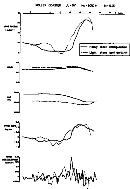
Fig. 16 SYNTHETIC MANOEUVRE-FLIGHT TESTING TECHNIQUE
