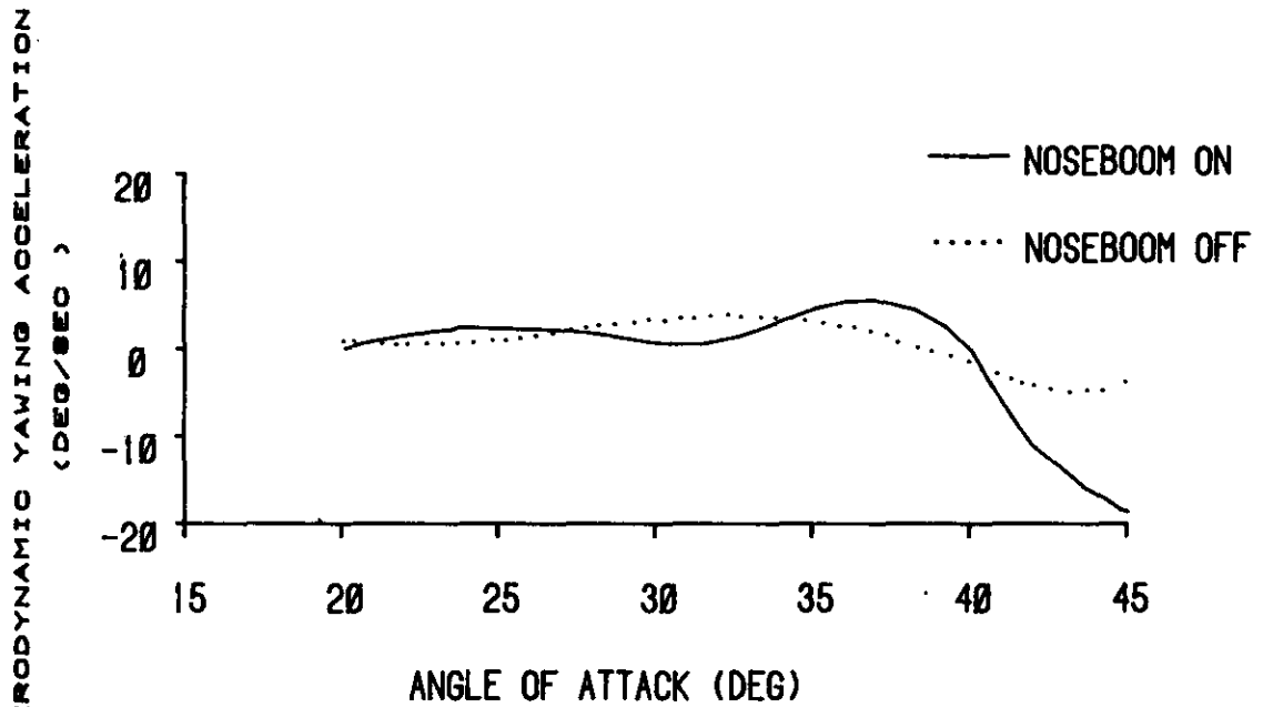
FIGURE 5. NOSEBOOM YAW ASYMMETRY
