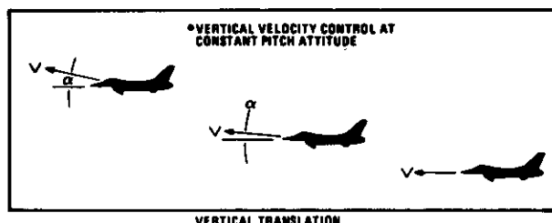
VERTICAL TRANSLATION
