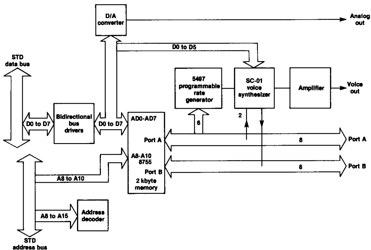
Figure 6. Simplified block diagram of a voice synthesizer.
