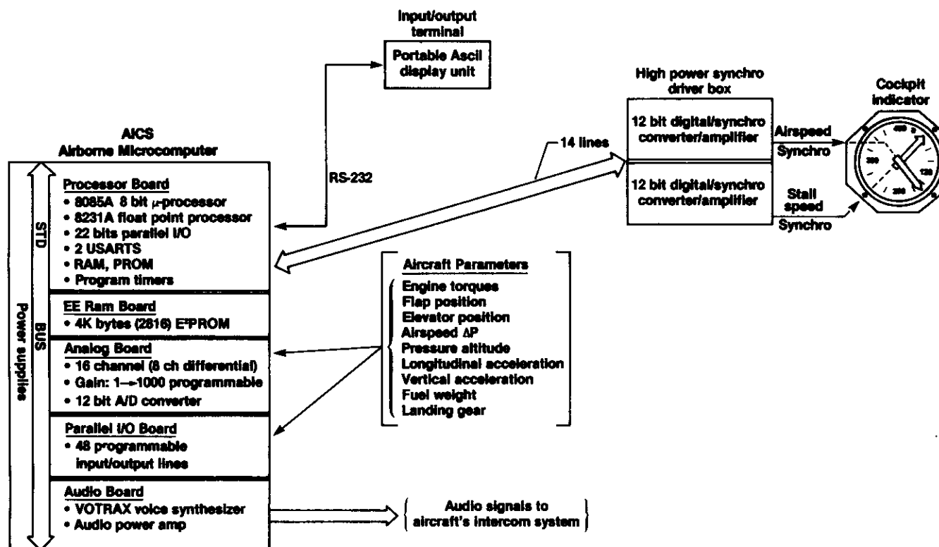
Figure 8. Overall block diagram of the OV-1C stall-warning system.
