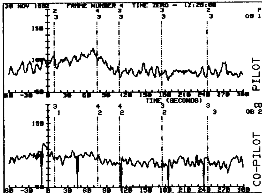
Fig 10 Example of beat-to-beat heart rate plots and workload ratings from the BAe 146 certification programme. (Recorded during a take-off from Amsterdam.)
