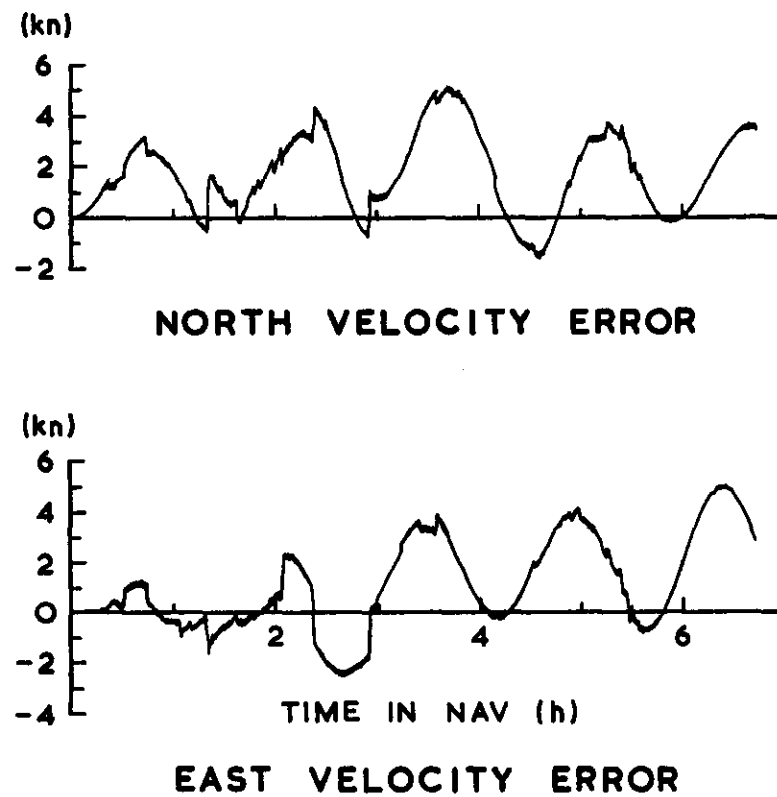
TYPICAL INERTIAL NAVIGATOR VELOCITY ERRORS
