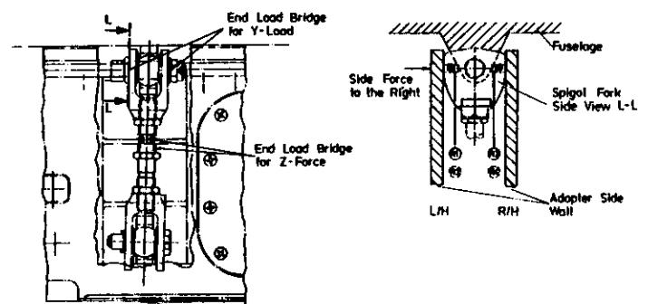
Fig. 10 COMPARISON BETWEEN MEASURING SPIGOT AND PROTOTYPE SPIGOT
