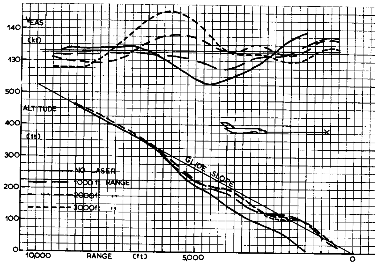
Fig. 18 Flight simulations of a coupled approach through thunderstorm windshear, for a BAC 1-11 medium jet transport, with and without LATAS type advance warning from different ranges. The thunderstorm cell was set at 4,500 ft range, and offset 1500 ft.
