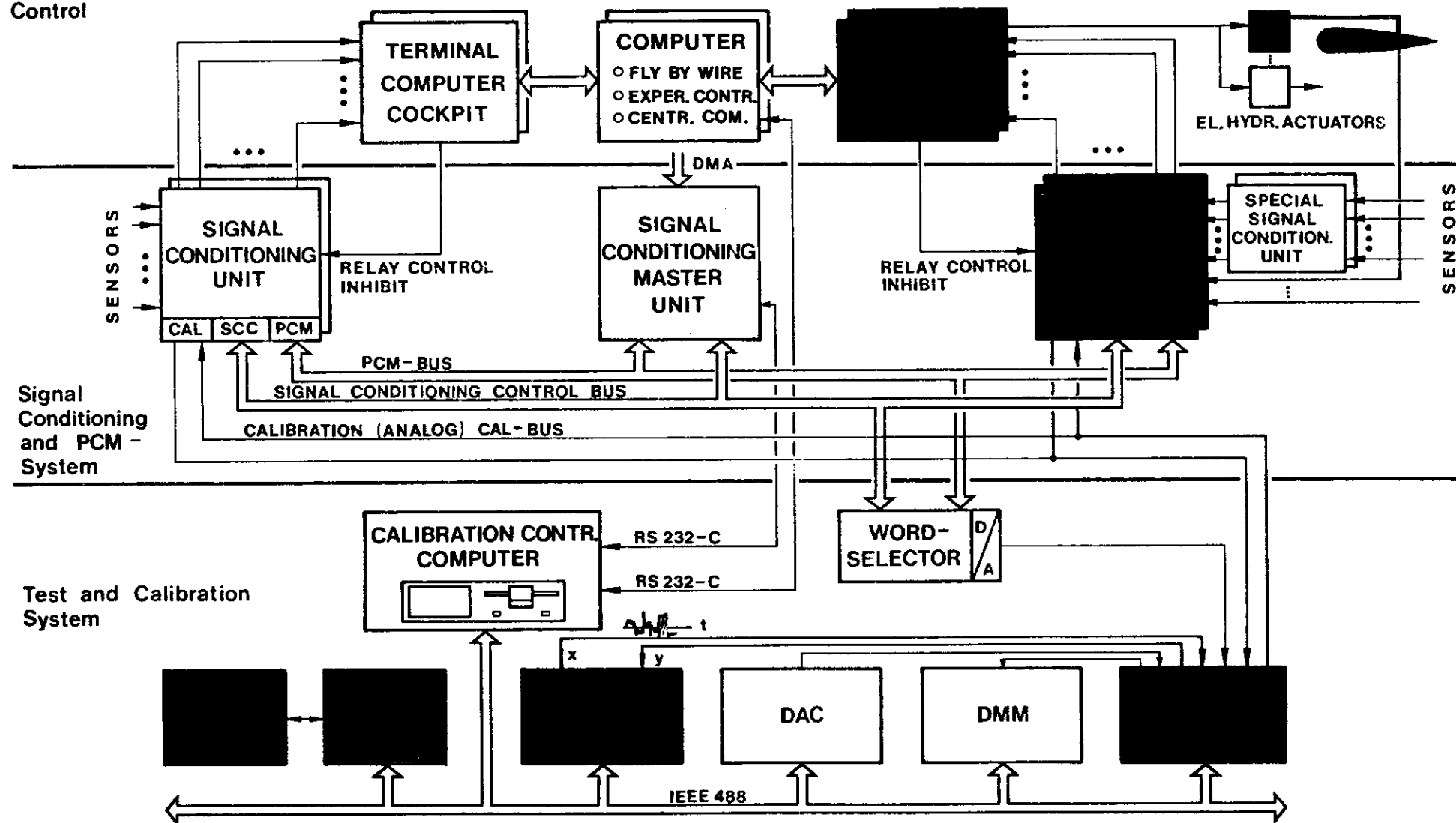
FIG. 10 DYNAMIC IN-FLIGHT CALIBRATION
