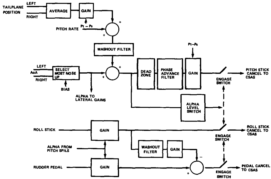
FIGURE 7 MARK 5 SPILS
