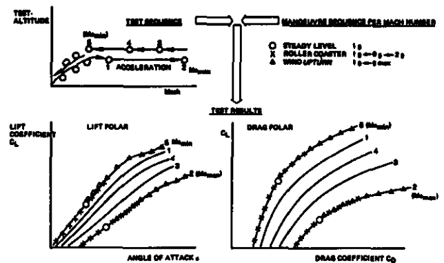
FIG. 9: Test Technique
