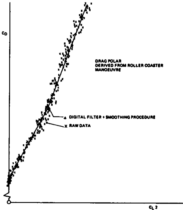
FIG. 12: Application of Digital Filter and Data Smoothing Procedure
