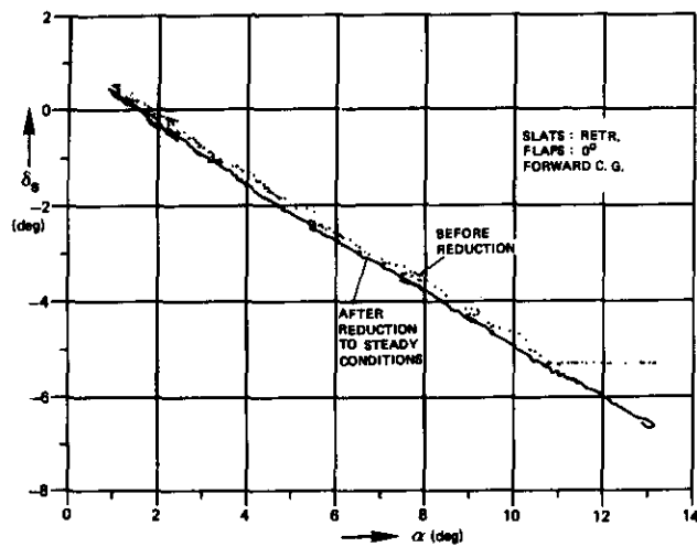
Fig. 5 Stabilizer trim curve
