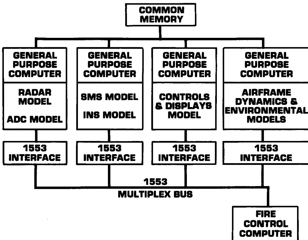
SIMULATION ARCHITECTURE FOR A SIMPLIFIED WEAPONS SYSTEM
