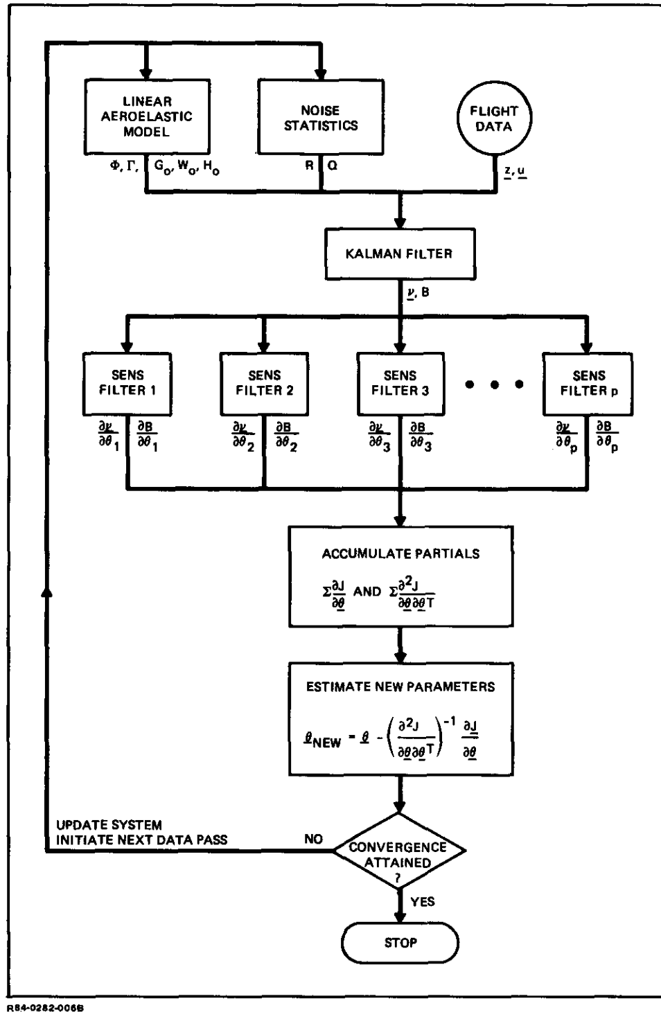
Fig. 2 Computational Sequence for Maximum Likelihood Parameter Identification Algorithm
