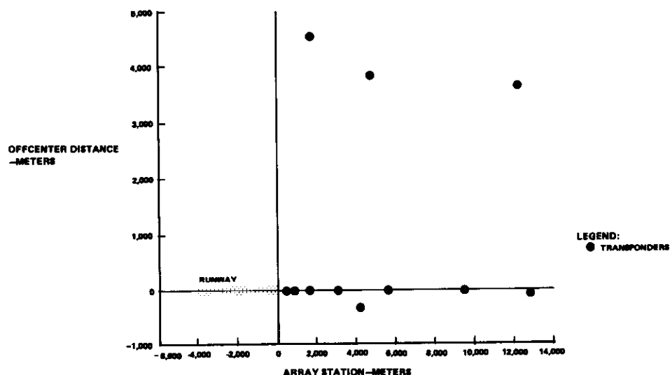
Figure 6. 737 Approach Test Transponder Array
