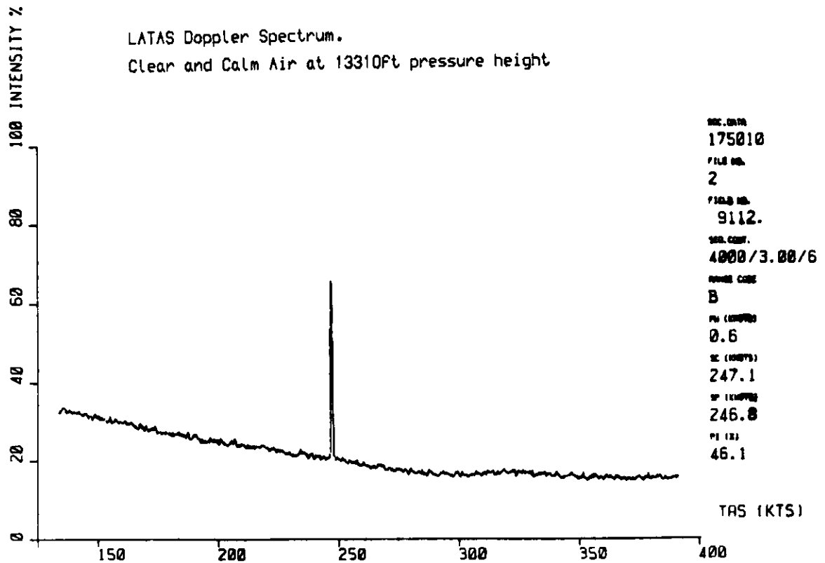
Fig. 7 LATAS Doppler spectrum in clear and calm air at 13310 ft pressure height. Note the narrow Doppler signal with peak corresponding to a true airspeed of 246.8 knots.
