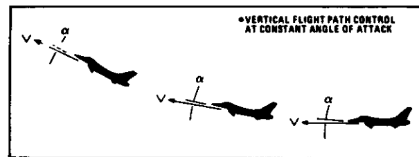
DIRECT LIFT
