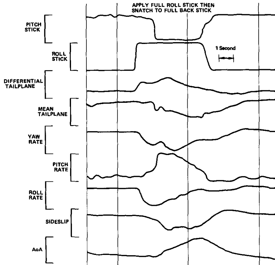
FIGURE 9 INERTIALLY COUPLED MANOEUVRE
