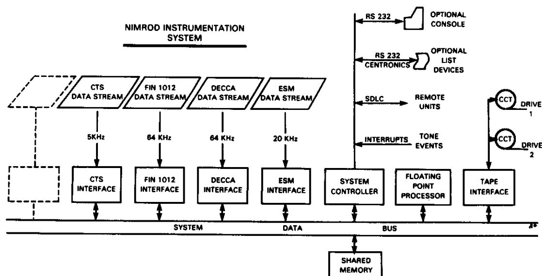
FIGURE 12 - THE MARDAS INSTRUMENTATION SYSTEM
