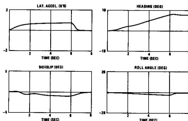
Figure 11 Flat Turn Time History
