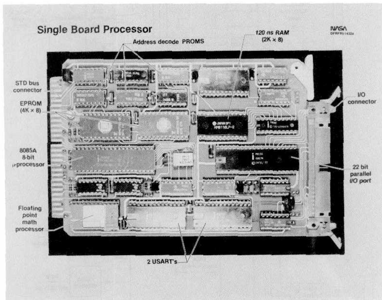
Figure 4. Single-board microcomputer.
