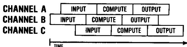
Figure 5 Time Skew
