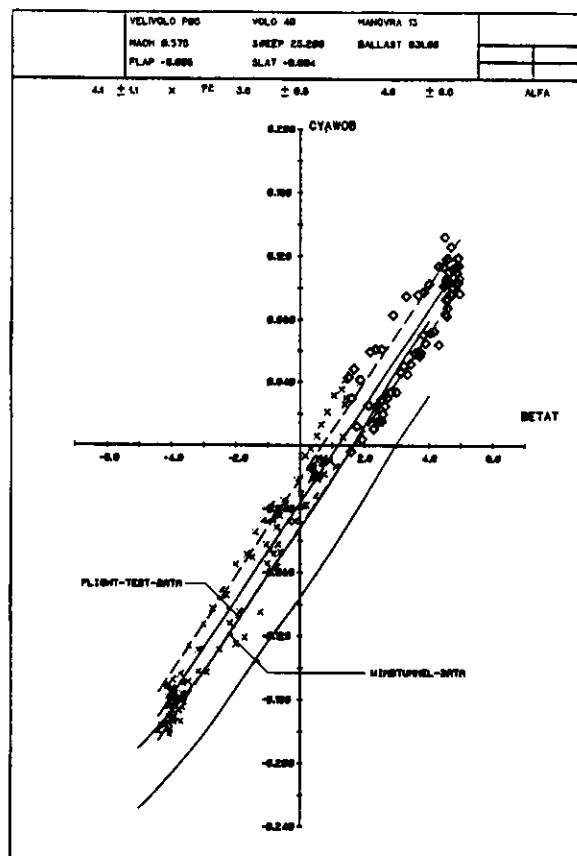
Fig. 9.2 MACE-COMPARISON OF FT-WT MEAS. YAW-MON. AT O/B PYLON SPIGOT
