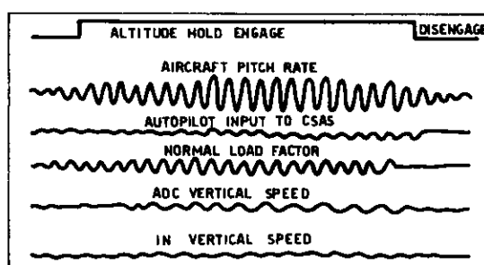
FIGURE 14 - LIMIT CYCLE WITH BARO-ALTITUDE MODE ENGAGED
