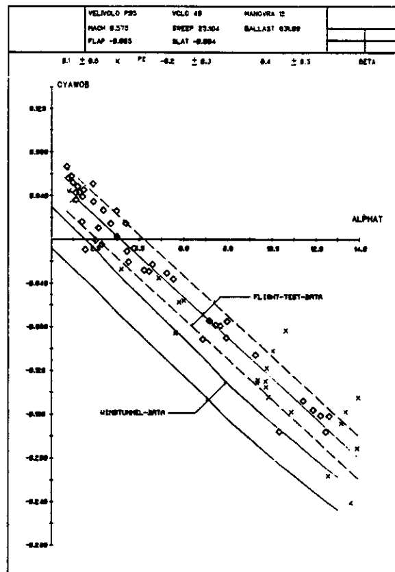
Fig. 9.1 MACE-COMPARISON OF FT-/WT MEAS. YAW MON. AT O/B PYLON SPIGOT
