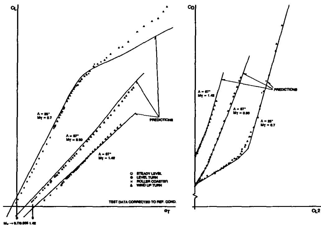
FIG. 17: LIFT/DRAG Polars (Comparison Flight Test/Prediction)
