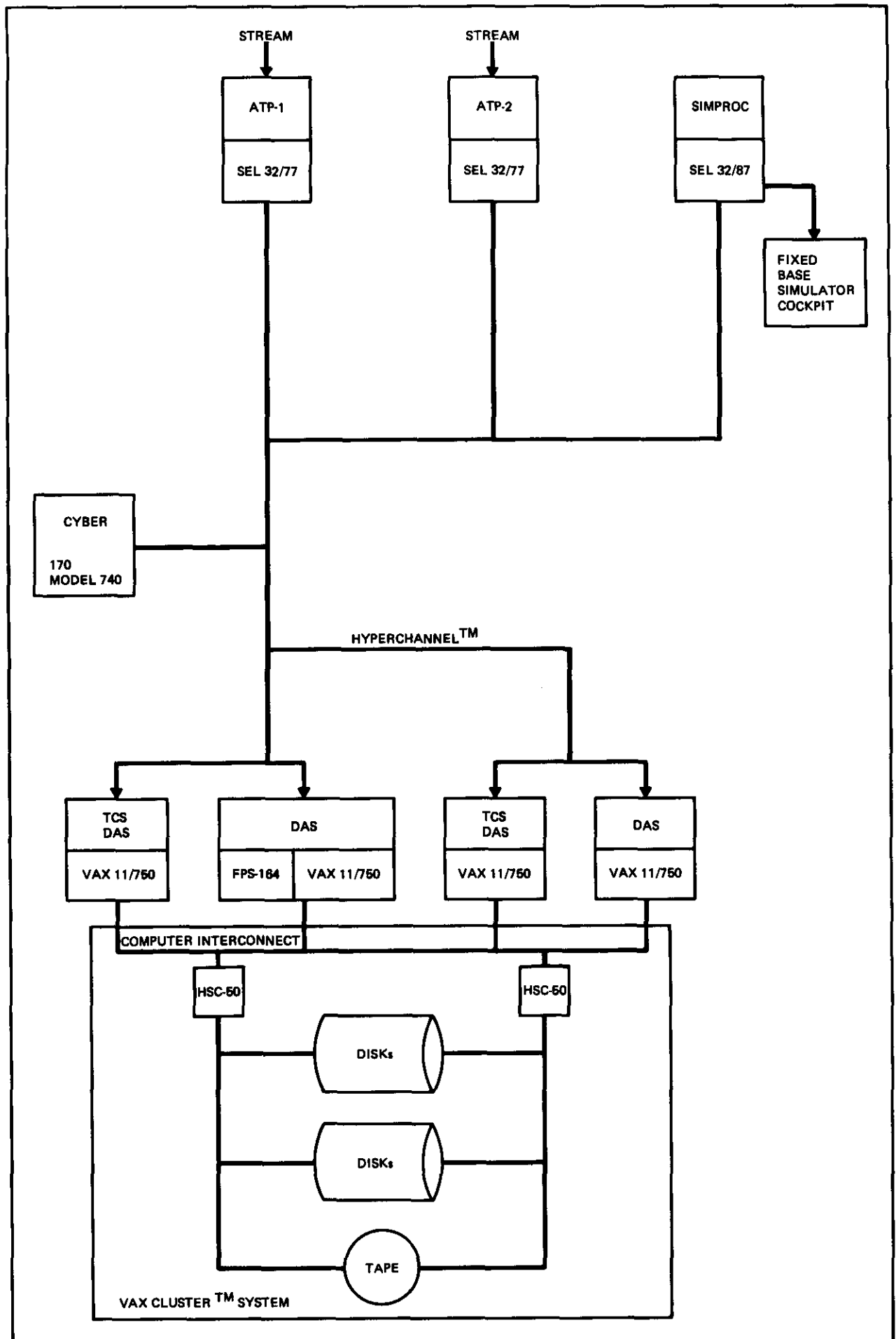
Fig. 6 Current NDCS Configuration
