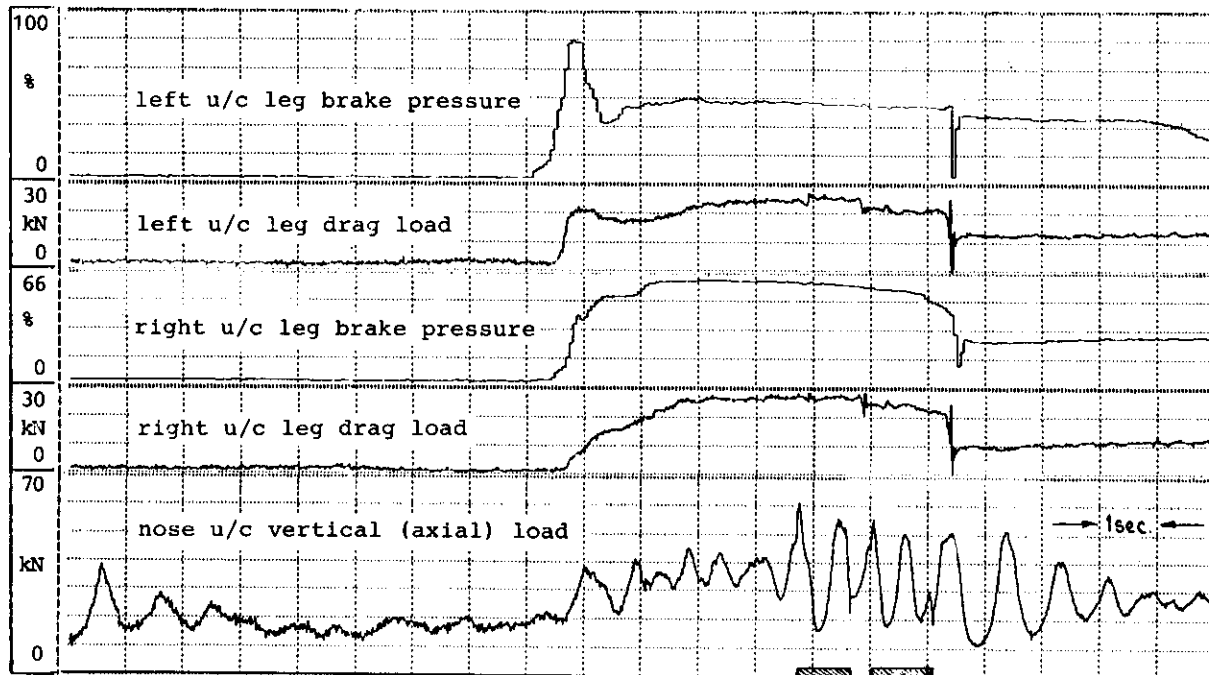
FIG. 16 UNSATISFACTORY BRAKE APPLICATION IN A BRAKED TEST RUN
