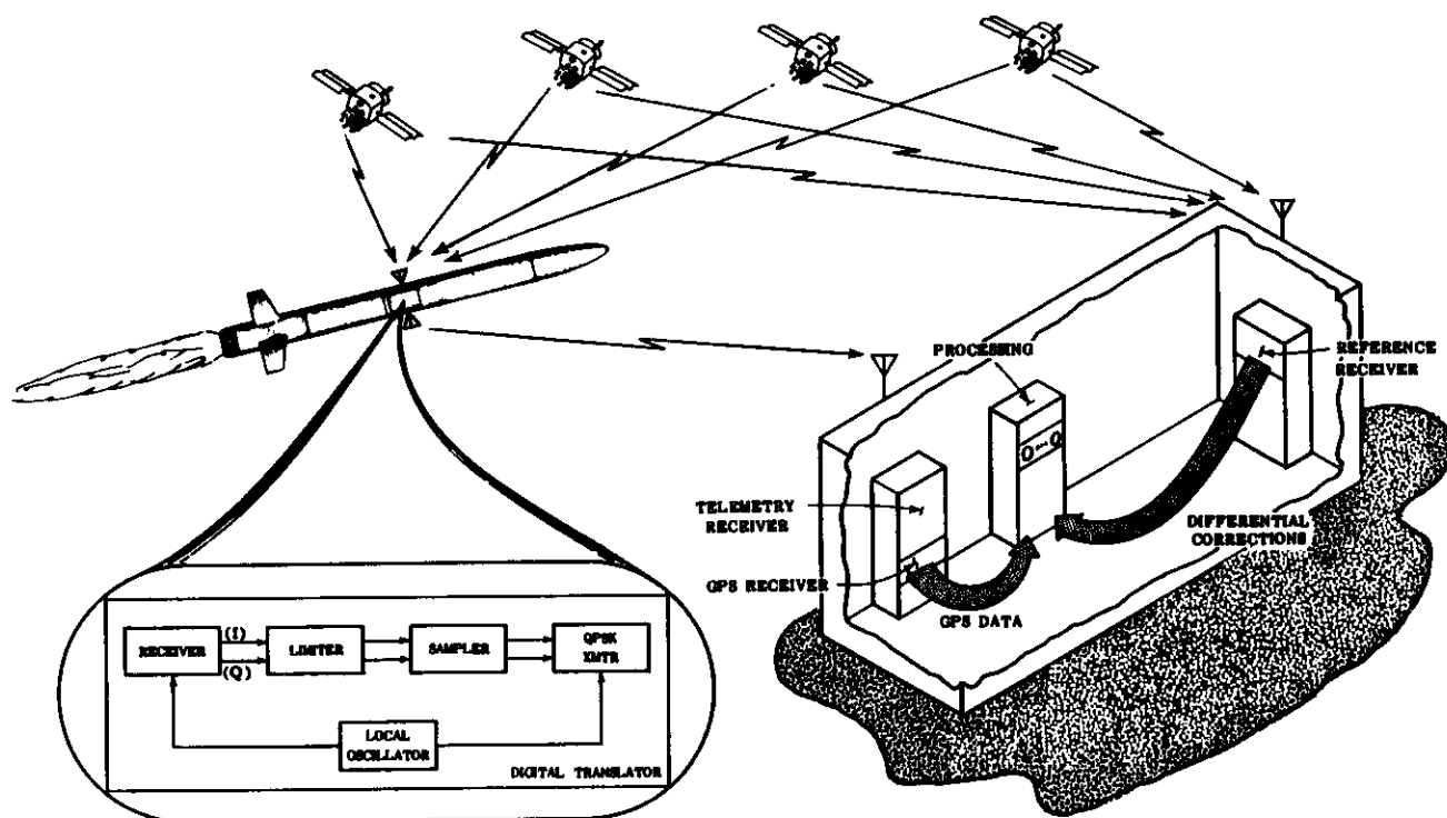
FIGURE 2 TRANSLATOR SYSTEM CONCEPT
