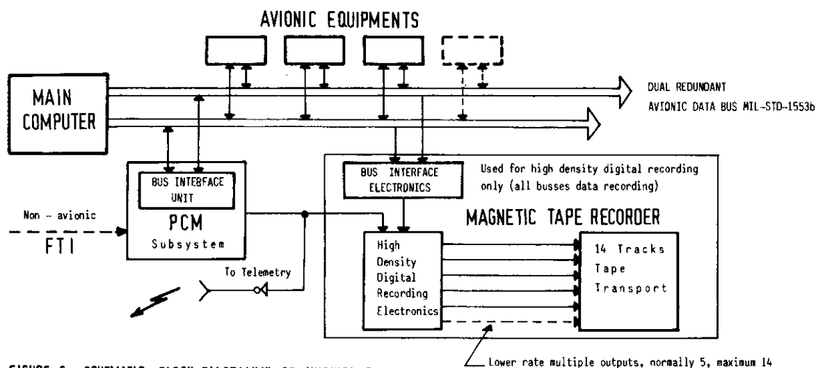
FIGURE 6 - SCHEMATIC BLOCK DIAGRAMME OF AVIONICS RELATED FLIGHT TEST DATA RECORDING SYSTEM
