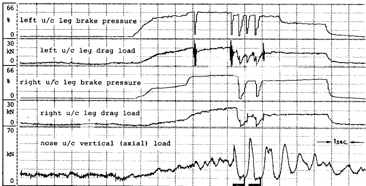
FIG. 17 RESULTS OF IMPROVED BRAKING TECHNIQUE
