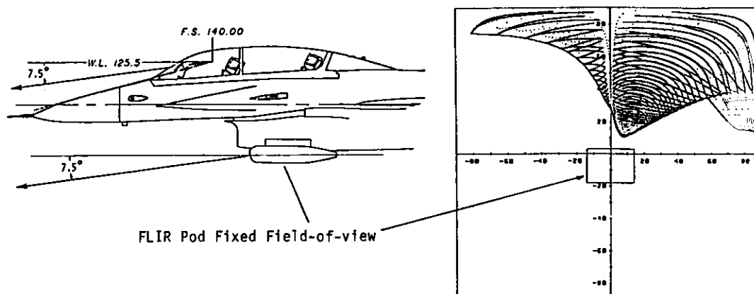
FIGURE 8 F-16 FORWARD LOOKING INFRARED (FLIR) POD FIELD-OF-VIEW.
