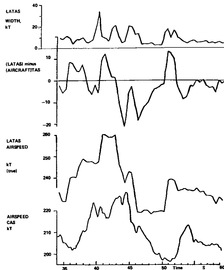
Fig. 16 Passage through a thunderstorm microburst showing the response of the RAE/RSRE LATAS system. (Flt 792, pm 14 July 1982, run 3, JAWS project). Note the 2 sec lead (corresponding to ~ 250m) of the LATAS airspeed.
