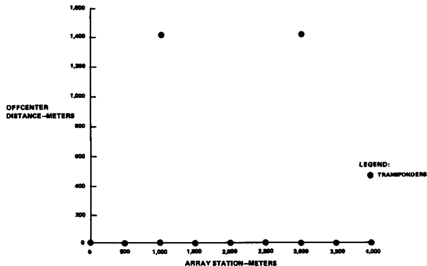
Figure 3. Simulator Transponder Array
