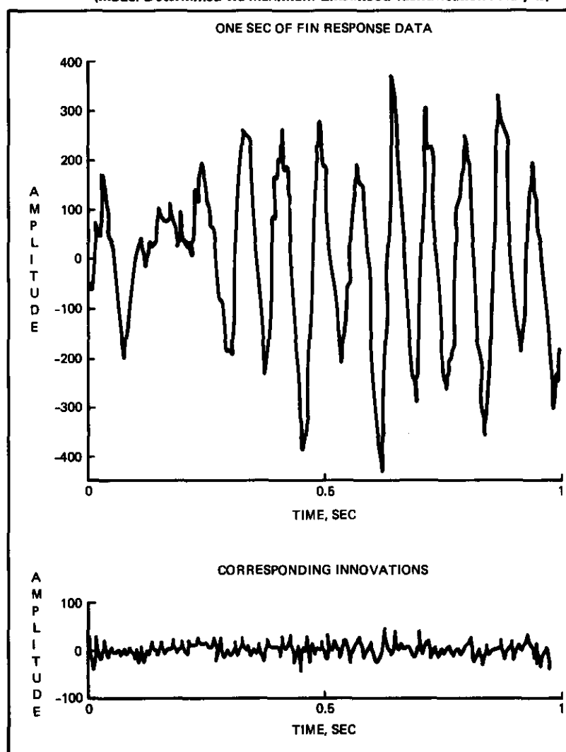
Fig. 15 Typical High Resolution Comparison of Actual F-14A Fin Response Data Segment & Maximum Likelihood Innovation Signal Level
