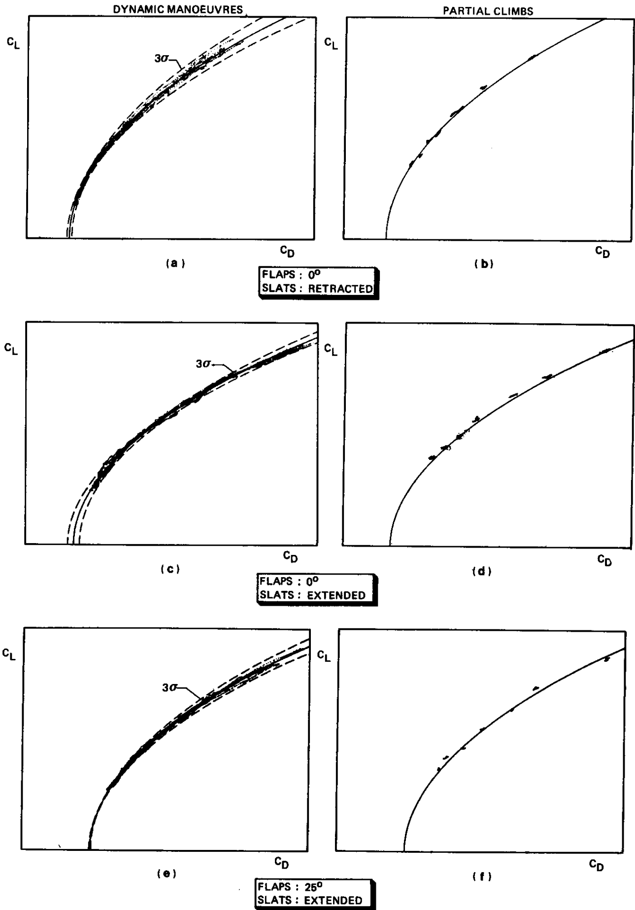
Fig. 4 Survey of the lift-drag polar measurement results
