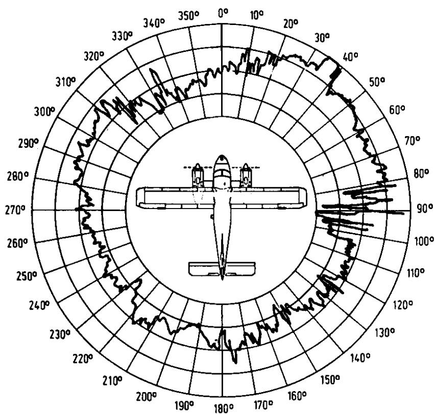
Fig. 8: Simulated typical ESM-DOA-Error
