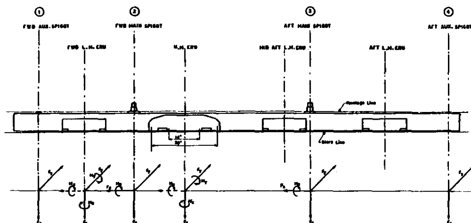
Fig. 7 RIGHT SHOULDER PYLON-SPIGOTS AND ERU'S LOCATION IN RESPECT TO MEASURED LOADS COMPONENTS
