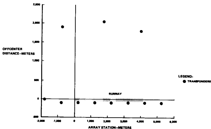
Figure 8. MAPS Acceptance Test Transponder Array
