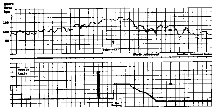
Fig 6 Typical beat-to-beat heart rate and nozzle angle traces recorded during a ski-jump take-off in an HS Harrier. (Note the rapid downwards rotation of engine thrust (upwards in the trace) as the aircraft left the ramp (arrow) followed by the gradual rearwards rotation (downwards in the trace) as speed was increased.)
