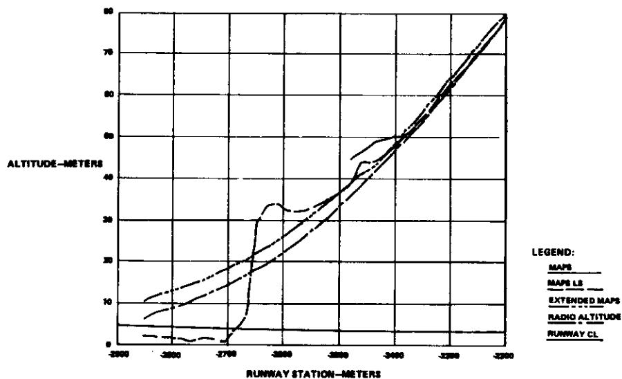
Figure 11. 767 Takeoff
