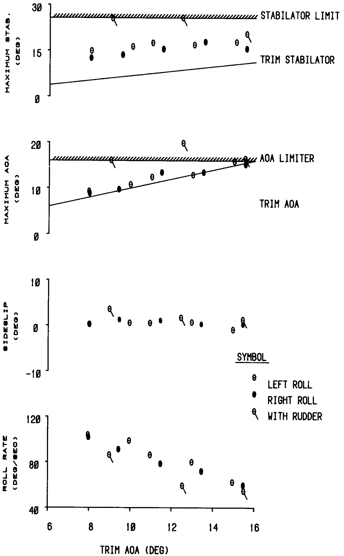
FIGURE 1. ONE-G ROLLS
