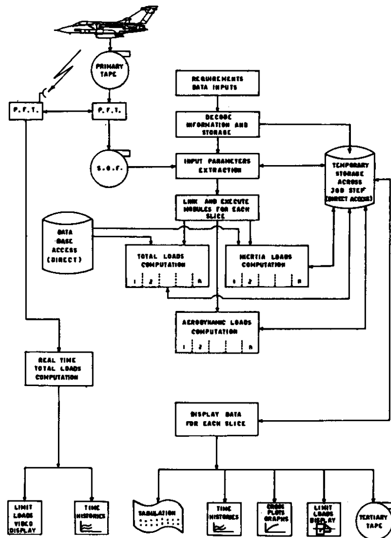
Fig.18 FLIGHT TEST DATA PROCESSING
