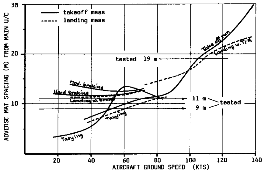
FIG. 11 CALCULATED ADVERSE MAT SPACING FROM MAIN U/C LOADS
