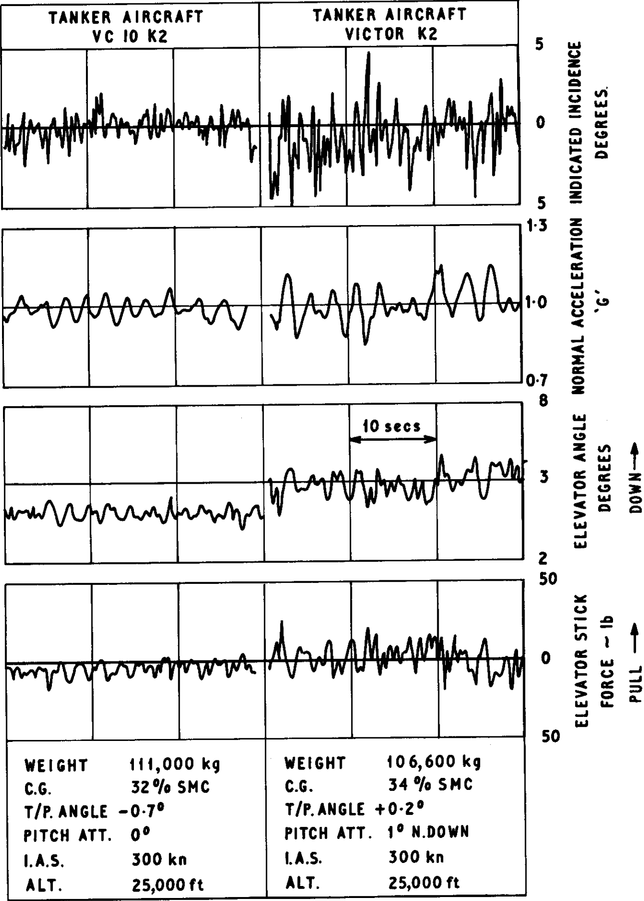
FIG. 4 COMPARATIVE TIME HISTORIES OF VC 10 K2 REFUELLING BEHIND TWO TYPES OF TANKER UNDER SIMILAR FLIGHT CONDITIONS.
