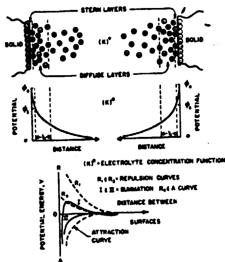
THE DIFFUSE DOUBLE-LAYER AND ATTRACTION-REPLICATION
