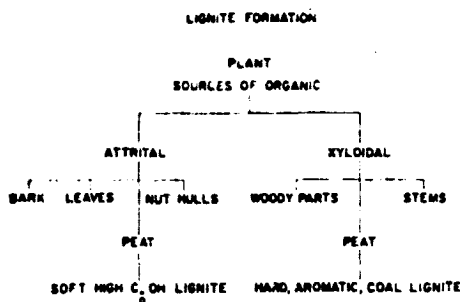
Figure 11. Diagram showing the dependence of the type of lignite on the sources of organic substances from which it is formed. Types of soft lignite and with a high carboxylic content are more susceptible to the activity of alkaline hydroxides and hydrolyzable alkaline salts in the formation of humus.
