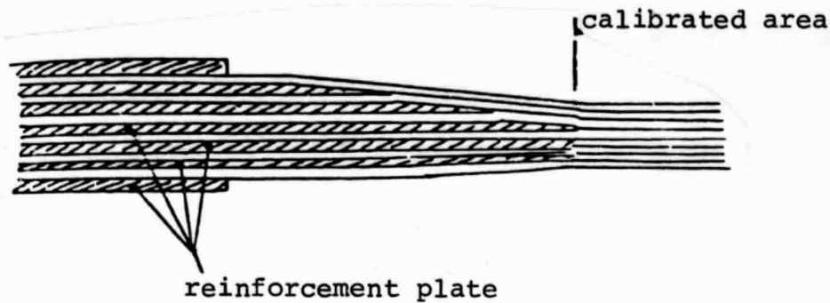
Figure 33 - Type of sample used for tensile tests on composites
