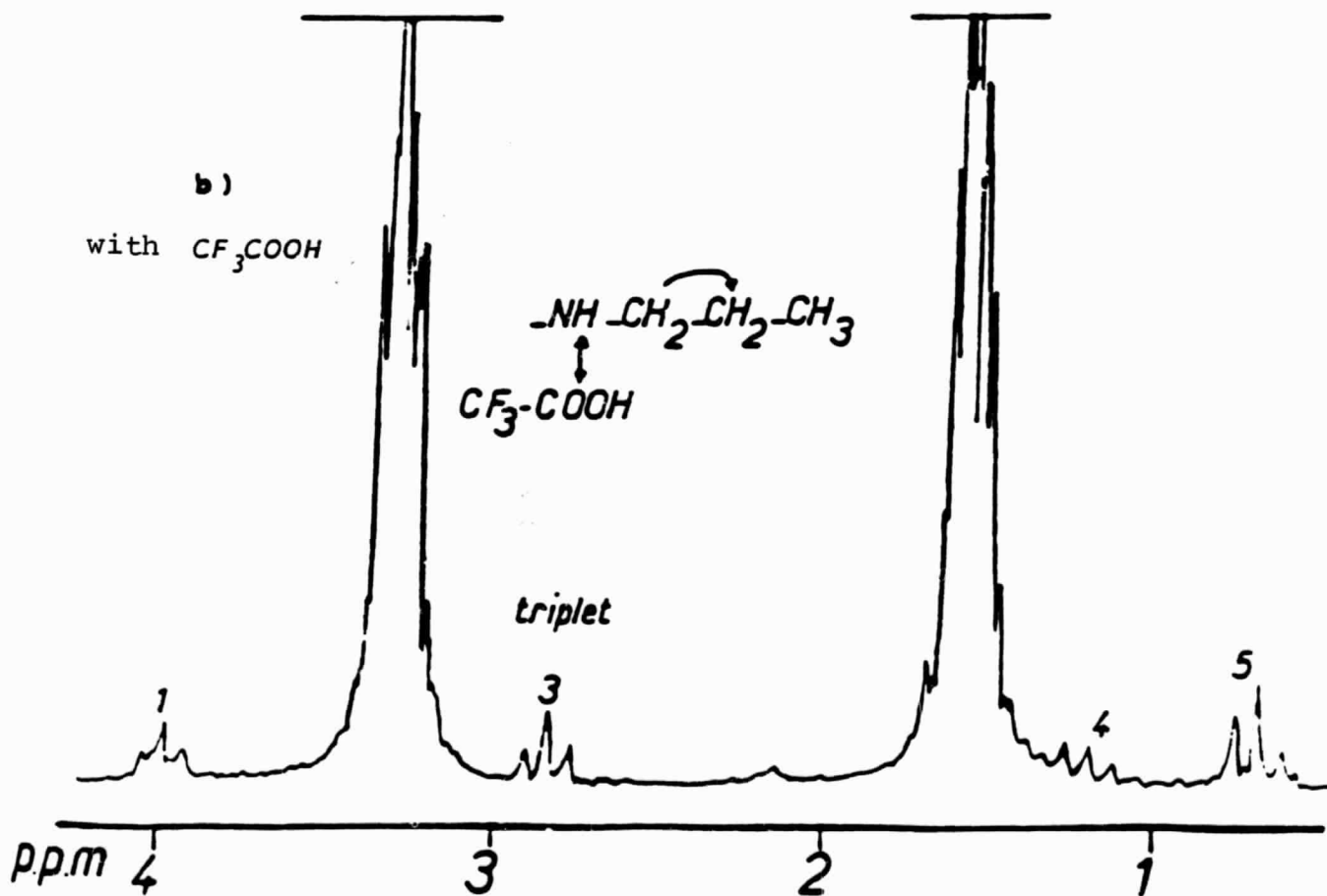
Figure 86 - RMN ^1\text{H} spectrum of a glycol polyoxetetramethylene after reaction with n-propylisocyanate.
