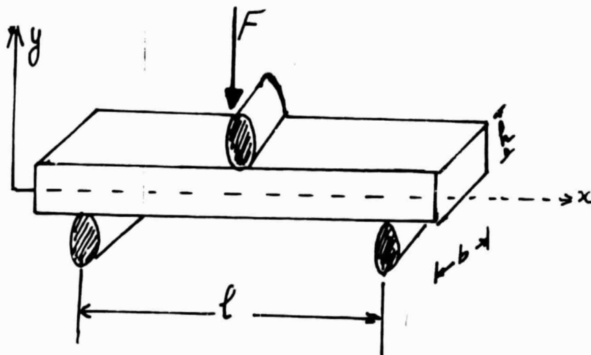
Figure 88 - Bending Test on 3 Points
