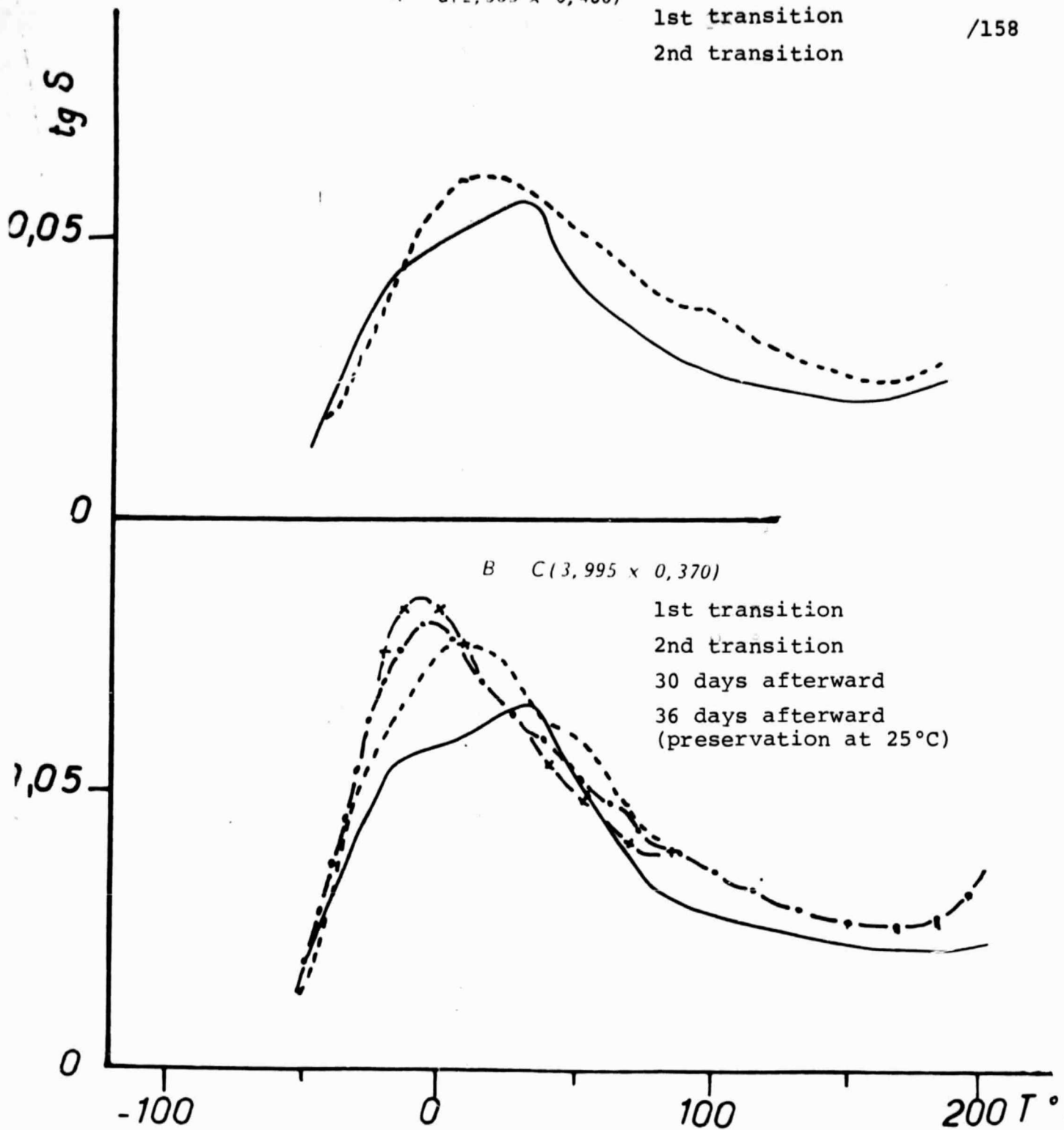
Figure 73: Annealing impact on samples cut out at 60^\circ
