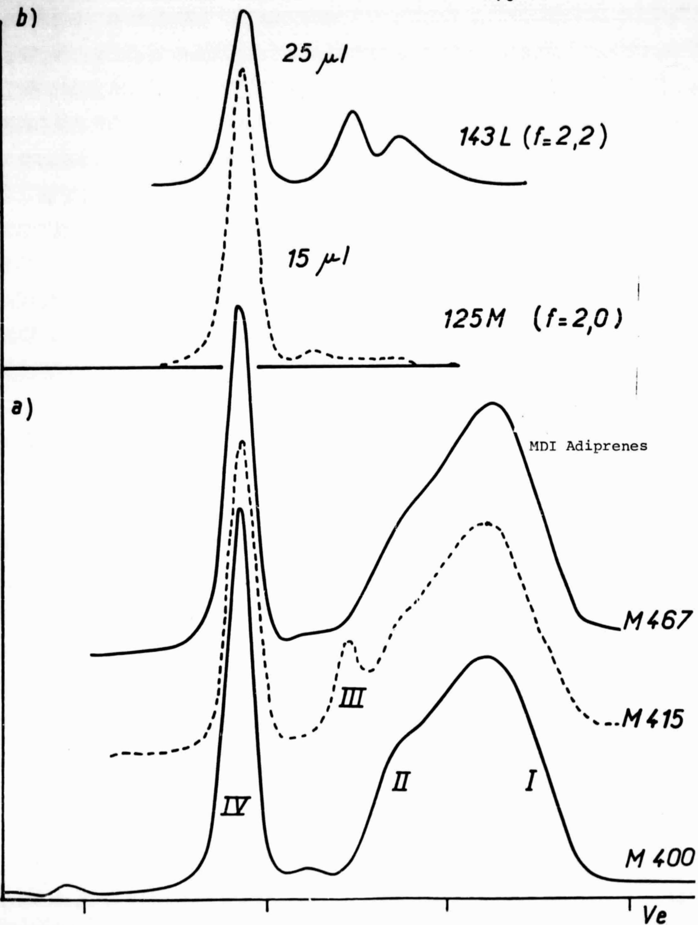
Figure 15 - GPC Analysis of the M Adiprenes
