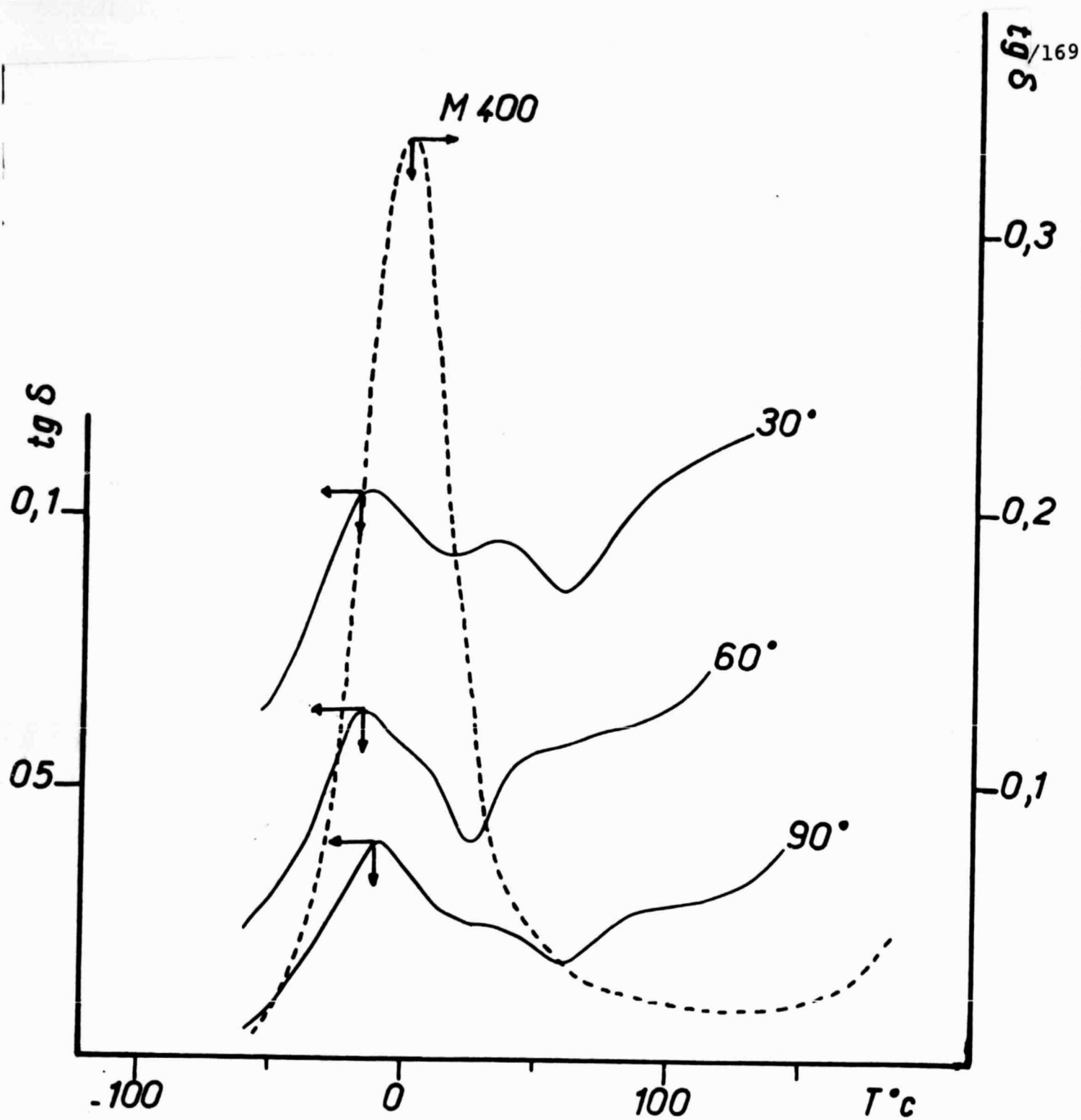
Figure 81 - Curves giving tg \delta as a function of the temperature for PUR-M400 (-----) and C-M400 composite according to the various angles \theta .
