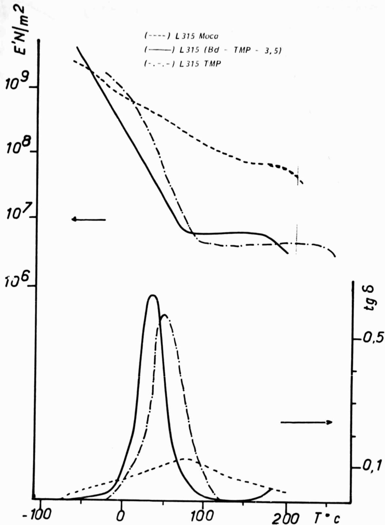
Figure 24 - Comparison of the dynamic mechanical behavior of the two types of chain extenders, (\text{---}) diamine; (-\cdot-\cdot-) triol and (\text{---}) (diol + triol).
