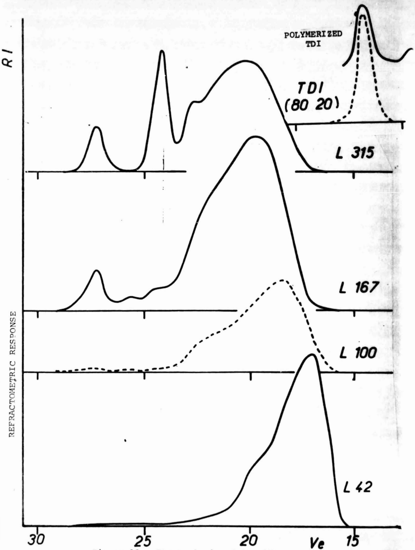
Figure 12 - GPC Analysis of the Adiprenes
