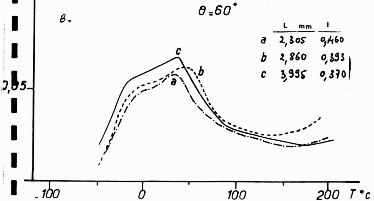
Figure 72 - Impact of form factor on tg.
