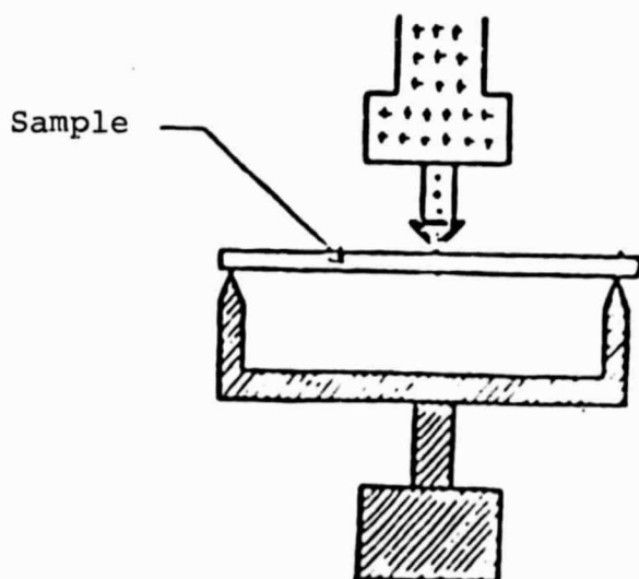
Figure 64 - Dynamic mechanical properties under beam bending forces.
