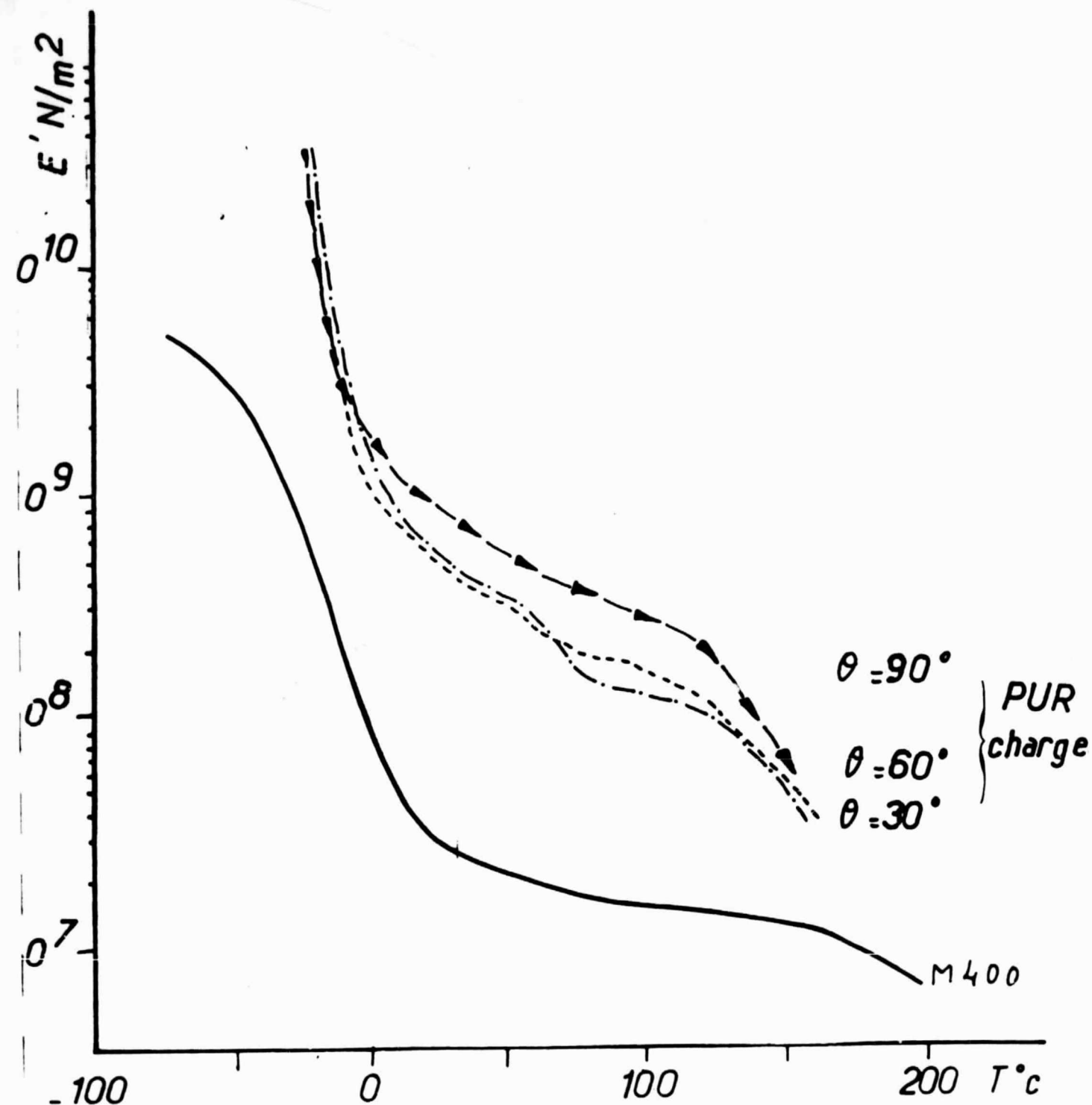
Figure 70 - Curves giving the modulus E' as a function of the temperature for PU-M400 and the V-M400 composite according to various angles \theta .
