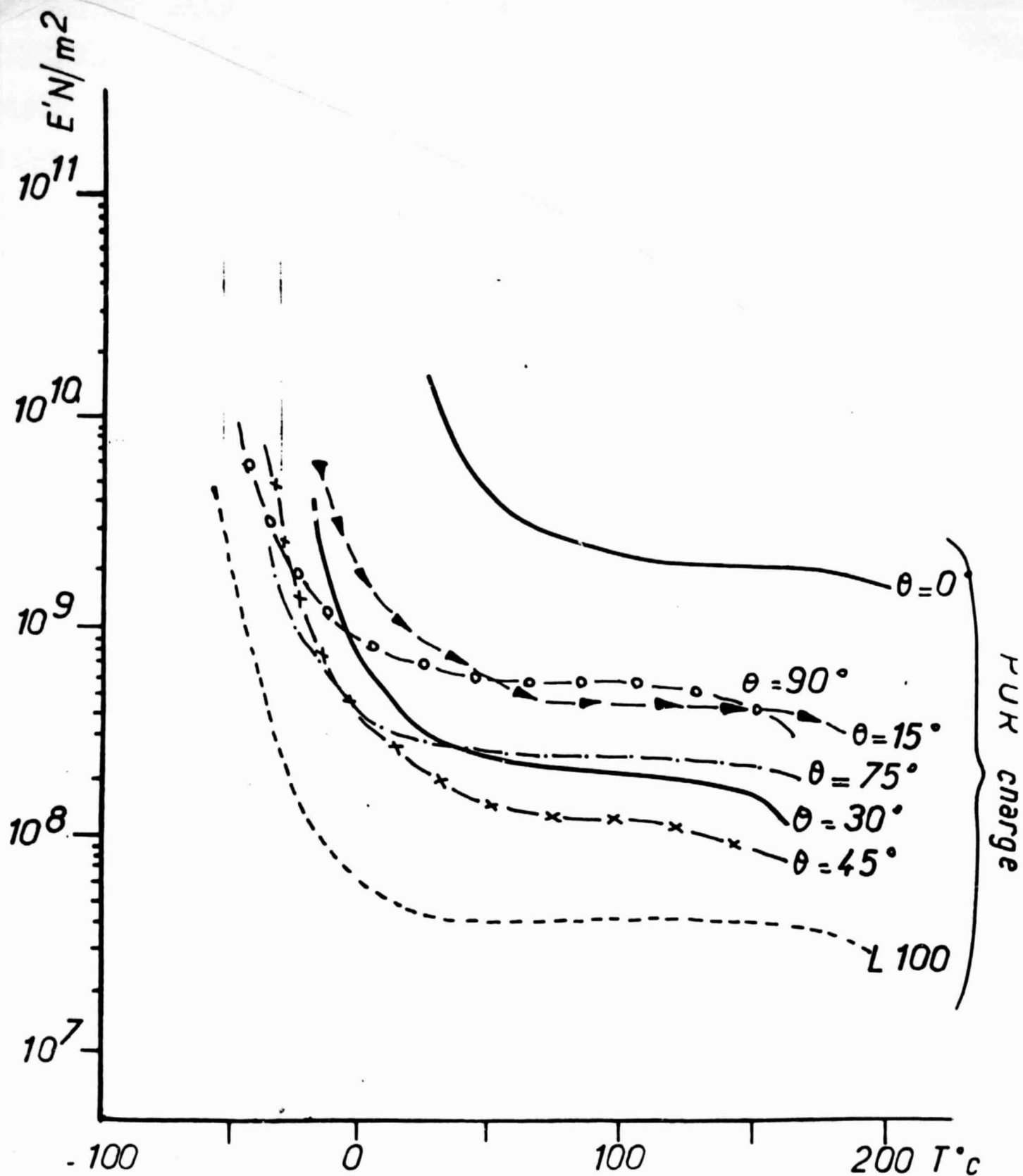
Figure 68 - Curves giving the modulus E' as a function of the temperature for PU-L100 (-----) and for the composite VL100 along different angles \theta .
