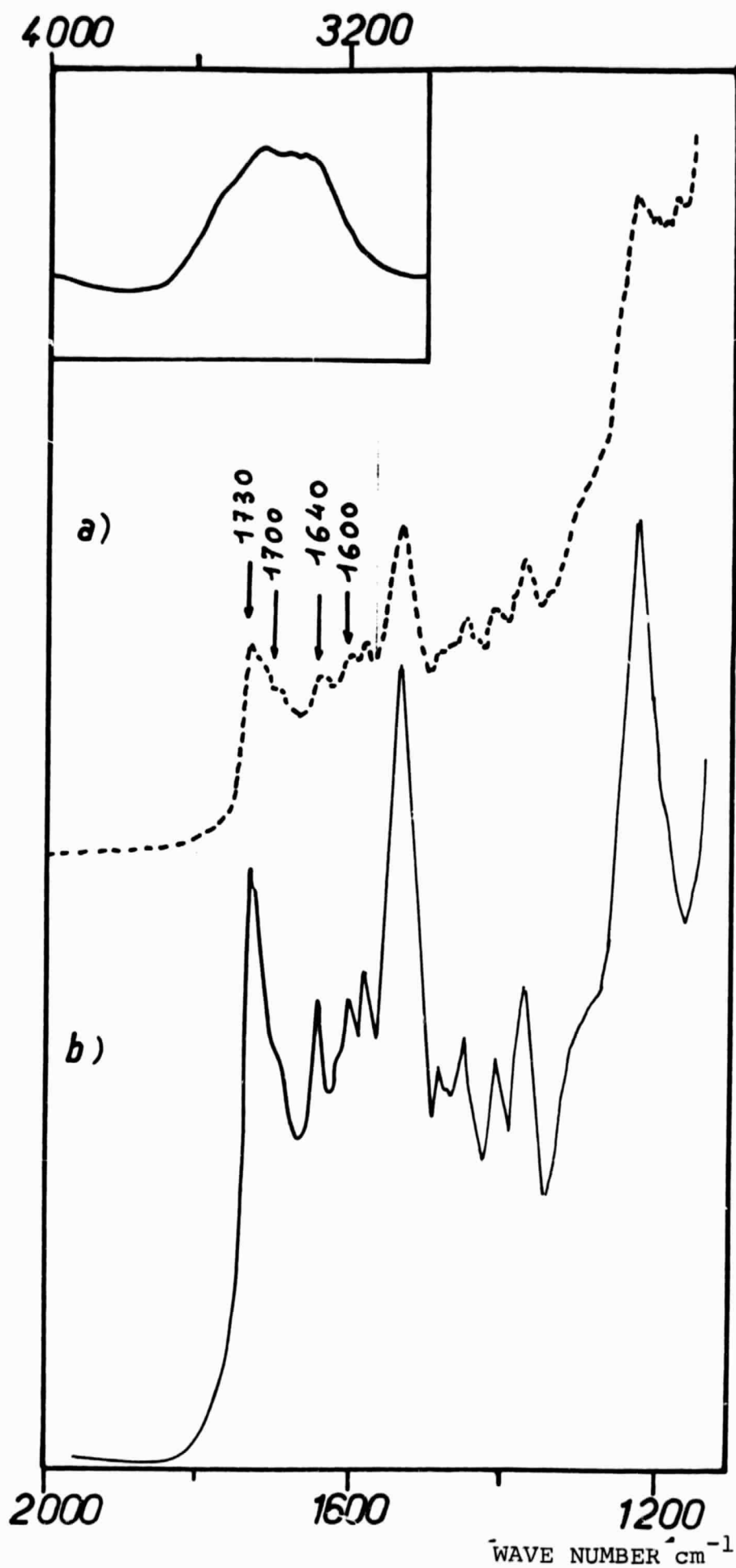
Figure 48 -IR Spectra of C-L100 Composites a) At Core; b) On Fiber Surface
