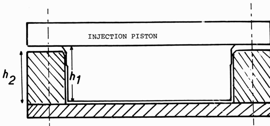
Figure 35 - Composite Plate Modulus - Elastomer - Reinforcement. Schematic Diagram. e = h_2 - h_1 = thickness of cast plate
