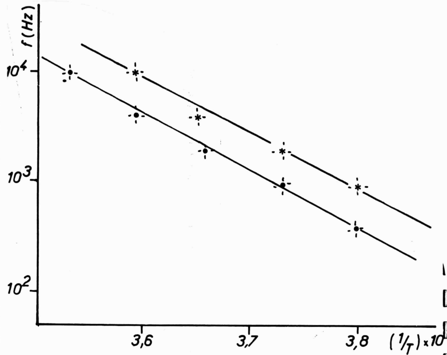
Figure 78 - Calculation of the activation energy for PUR-L100 and for V-L100 straight lines giving frequency as a function of \frac{1}{T} .
