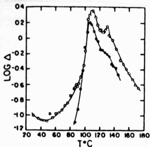
Figure 83 g - Logarithm of decrement for polystyrene ( M_w = 20,400 ) in the case of two different braids (○) → braid length # 6 cm; (●) → # 2) as a function of the temperature. The braid torsion is kept constant in both cases.
