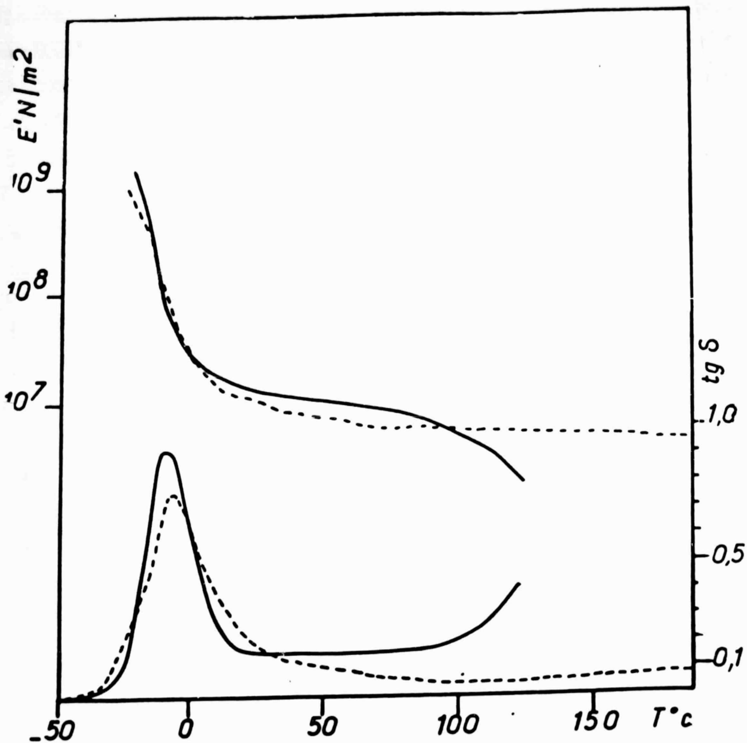
Figure 6 - E' and \text{tg } \delta curves as a function of the temperature for the PURs prepared from Bd (—) and butanediamine (-----)
