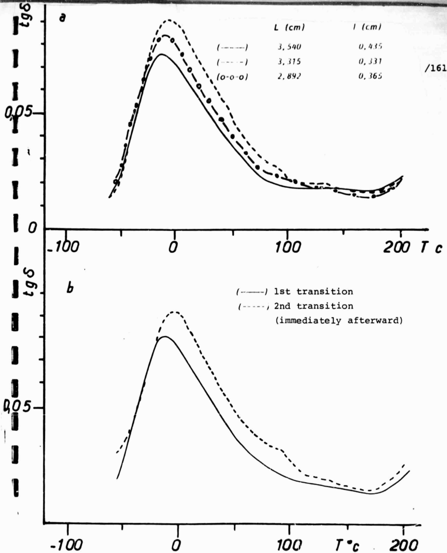
Figure 75 - Behavior of V-L100 composite with layers of fabrics crossed at 90° (α = ± 45°)
