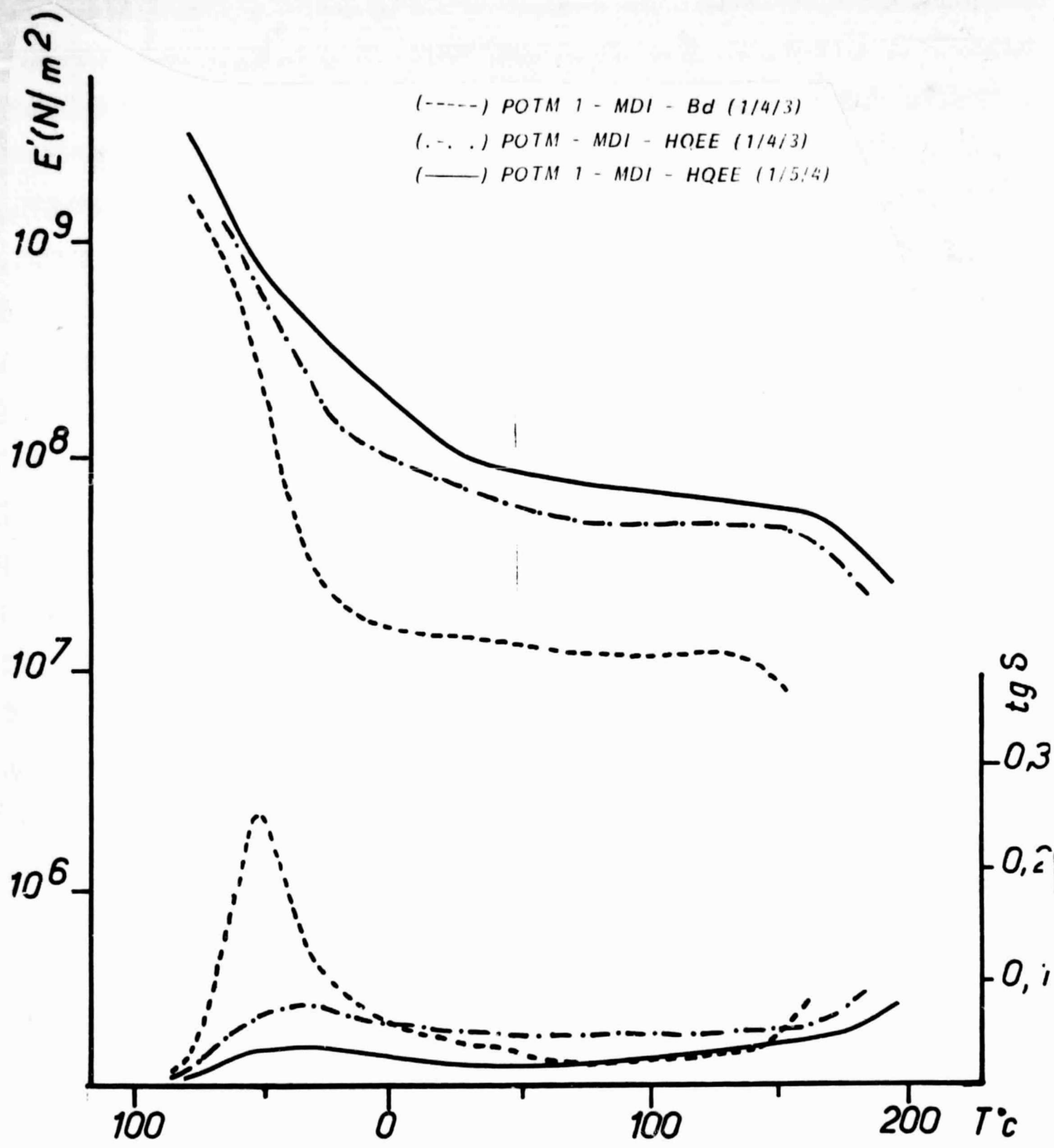
Figure 9 - Curve of modulus E' and of tg \delta as a function of the temperature at 11 Hz for POTM1-based polyurethanes. Comparison between two hardeners: Bd and HQEE.
