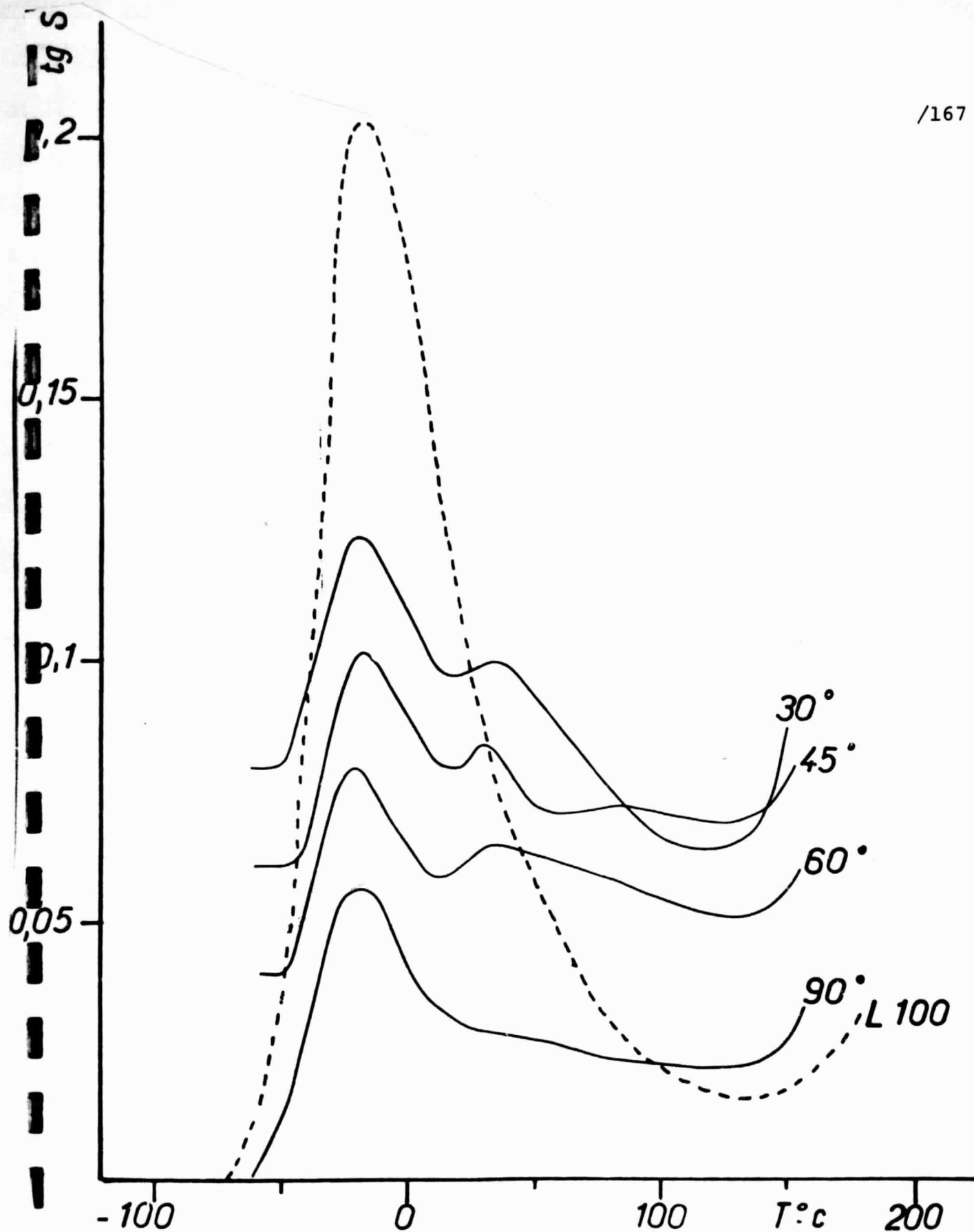
Figure 79 - Curves giving \text{tg } \delta as a function of the temperature for L100 polyurethanes (-----) and for C-L100 composite according to the various values of angle \theta .
