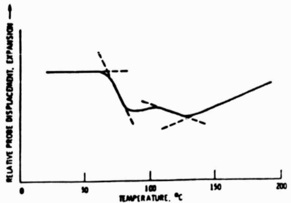
c) thermomechanical analysis curve of a unidirectional epoxy/glass E composite.
