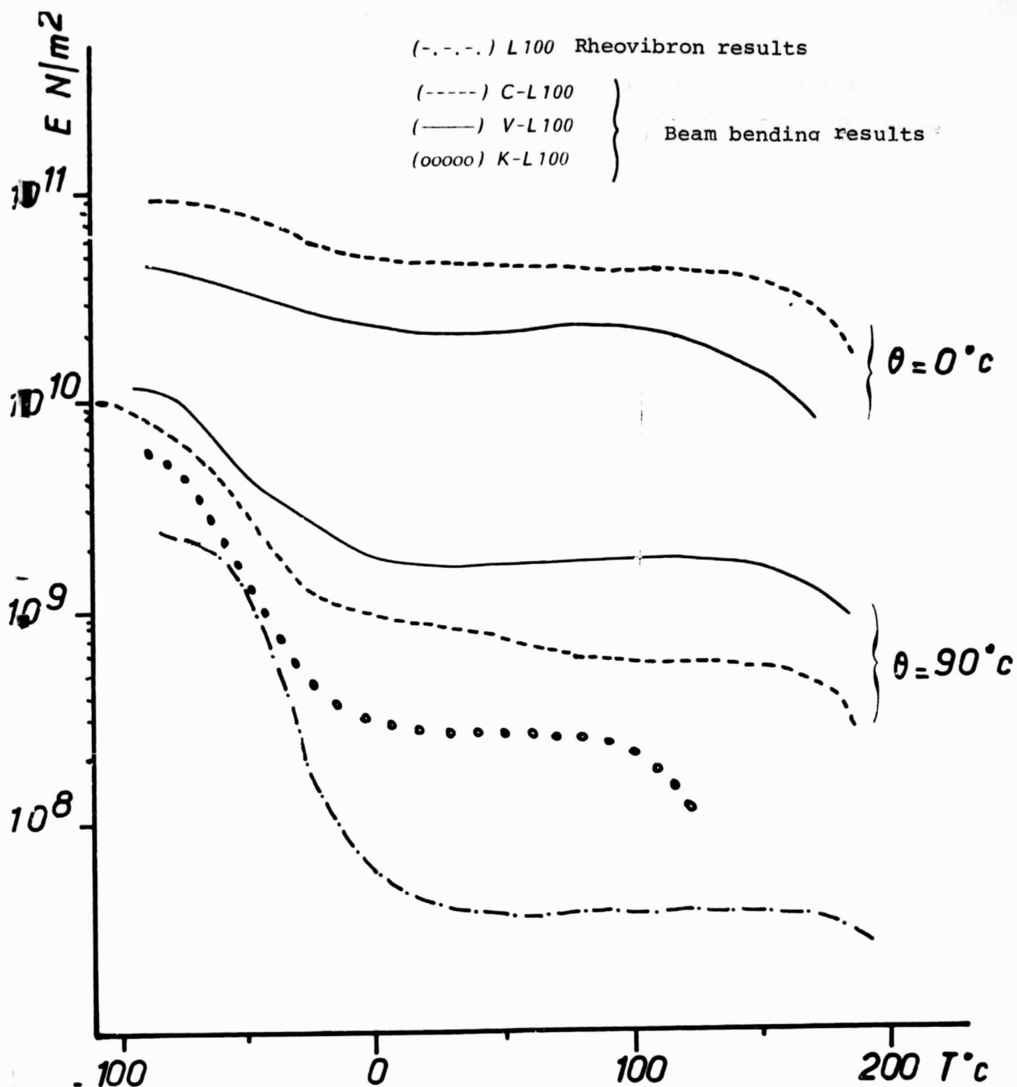
Figure 53 - Variation of the E_1 and E_2 moduli as a function of the temperature determined by beam bending on 3 points for the composites V-L100, C-L100 and K-L100 as well as the E modulus of the matrix determined with Rheovibron.
