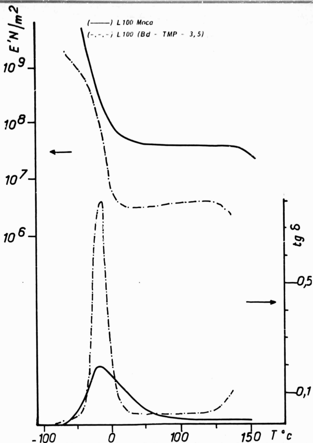
Figure 25 - Comparison of the dynamic mechanical behavior of two types of chain extenders (—) diamine and (-.-.-) polyol.
