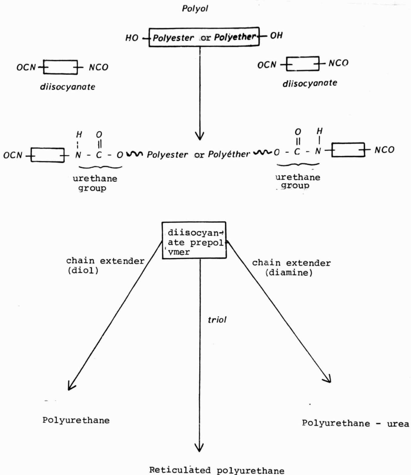
Figure 87 - Obtaining a PUR - General Diagram
