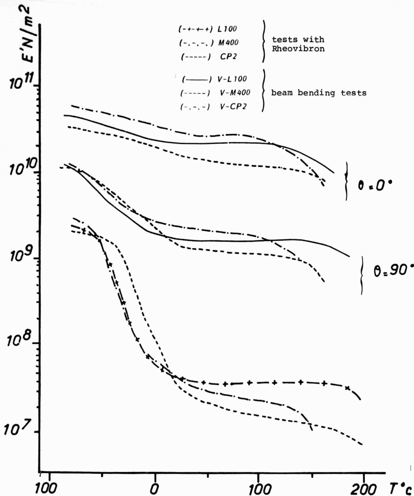
Figure 54 - Variation of the E_1 and E_2 moduli as a function of the temperature of composites V-L100 and V-M400 and V-CP2 (P109 oiling) under beam bending on 3 points, as well as the corresponding matrix, measured with Rheovibron.
