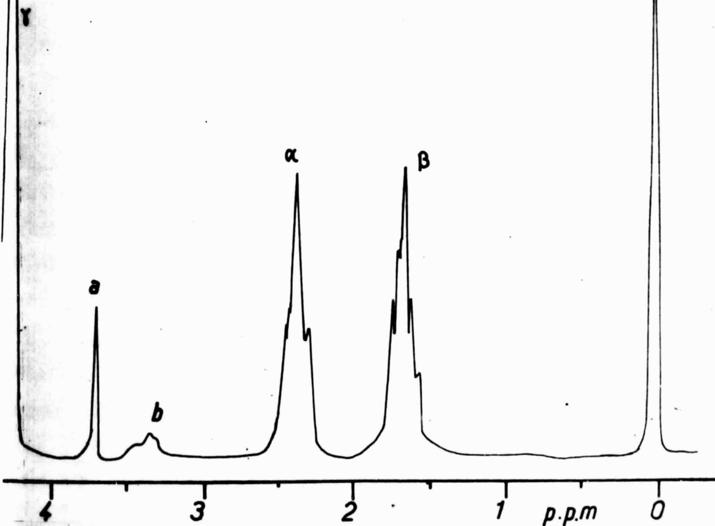
Figure 11 - RMN Spectrum of Cyanaprene A9
