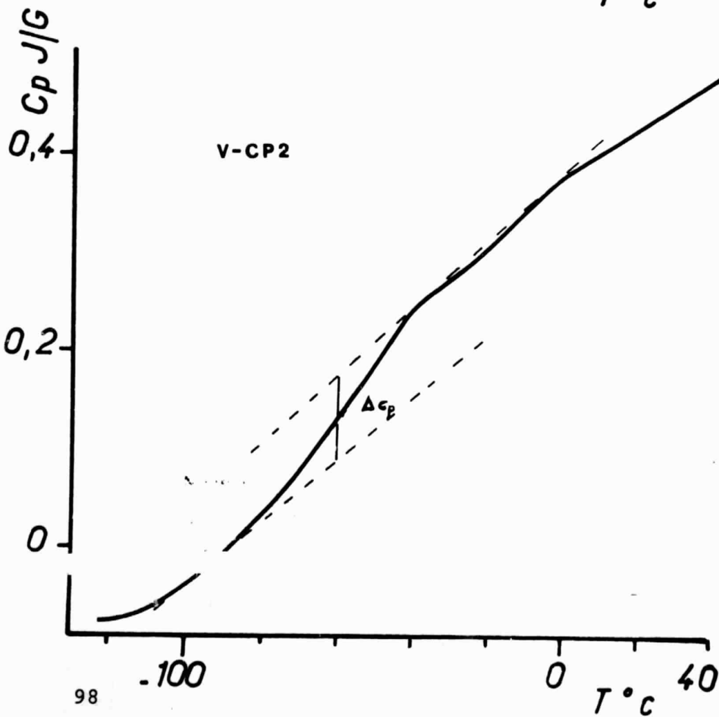
Figure 42 Measurements of \Delta C_p for the Polyurethane Matrix, CP2, and the Corresponding Glass Composite, V-CP2
