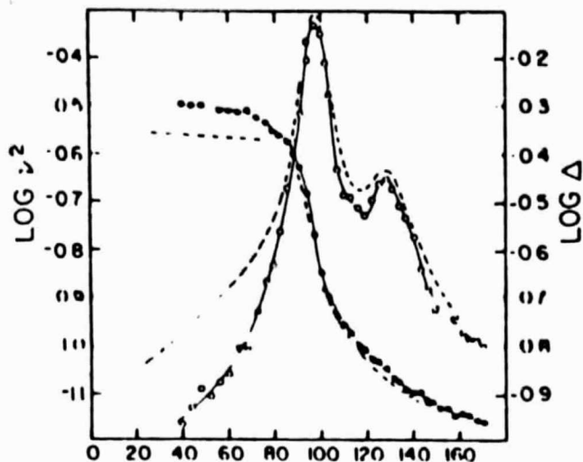
Figure 83 b (right) - Variation of \text{Log } \nu^2 and \text{Log } \Delta as a function of the temperature for polystyrene ( M_s = 20,400 ) using a braid # 5 cm long ( \nu = frequency; \Delta = decrement) (-----) curves obtained during temperature rise (——) curves obtained during temperature decline.
