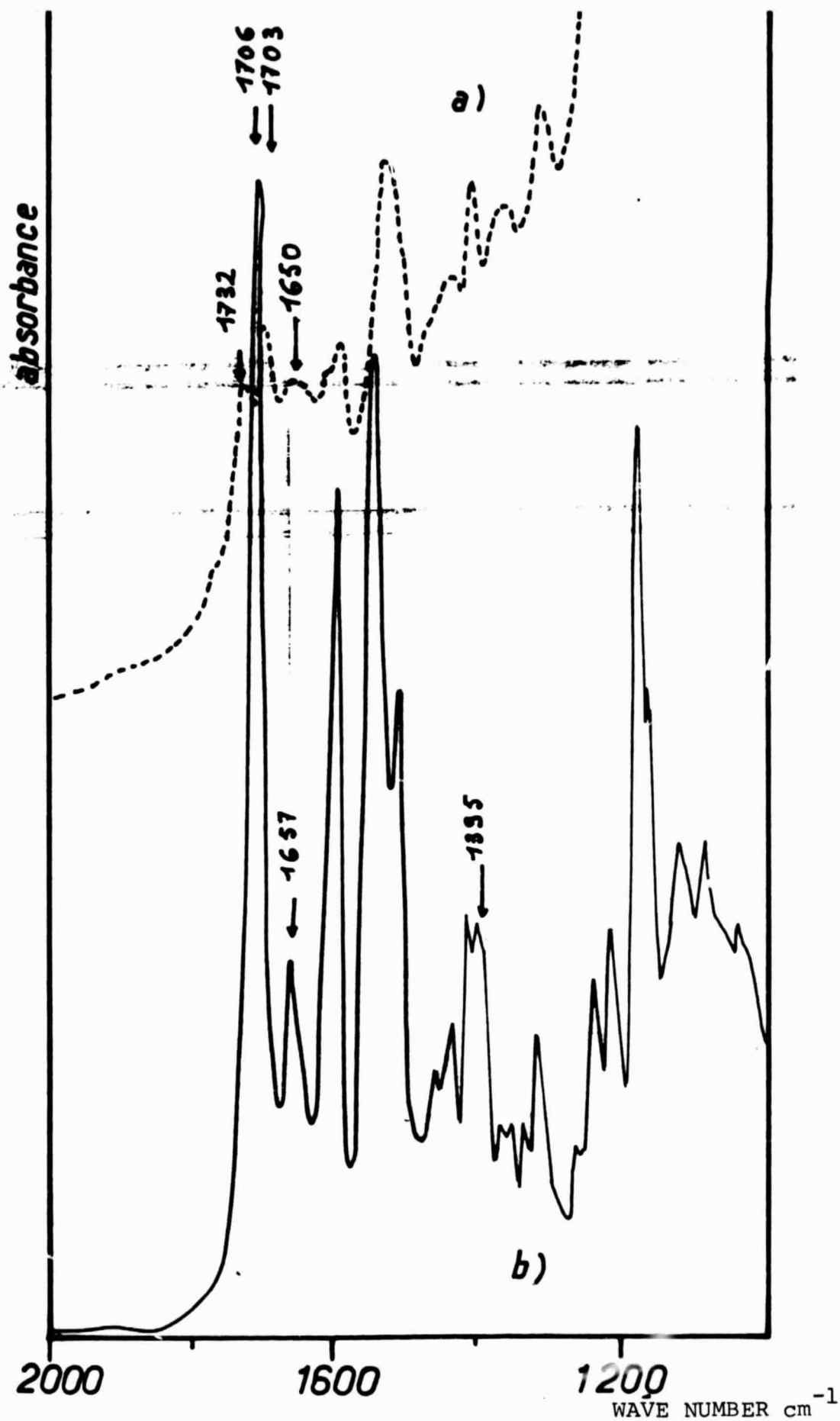
Figure 46 - IR Spectra of V(P109)-M400 Composite a) At Core; b) On Fiber Surface
