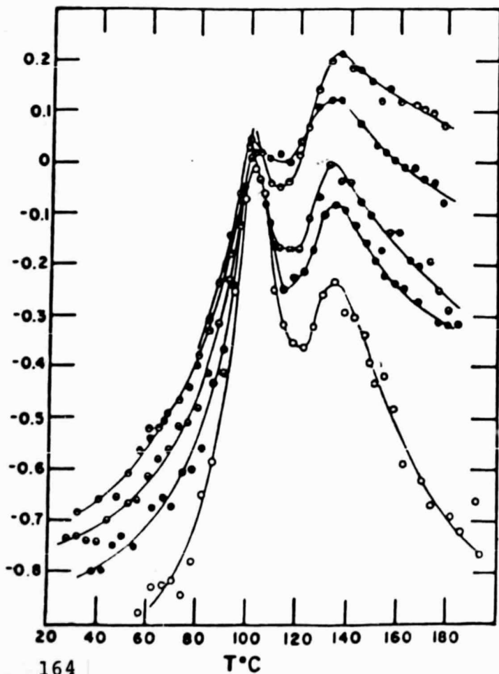
Figure 83 b (right) - Variation of \text{Log } \nu^2 and \text{Log } \Delta as a function of the temperature for polystyrene ( M_s = 20,400 ) using a braid # 5 cm long ( \nu = frequency; \Delta = decrement) (-----) curves obtained during temperature rise (——) curves obtained during temperature decline.
