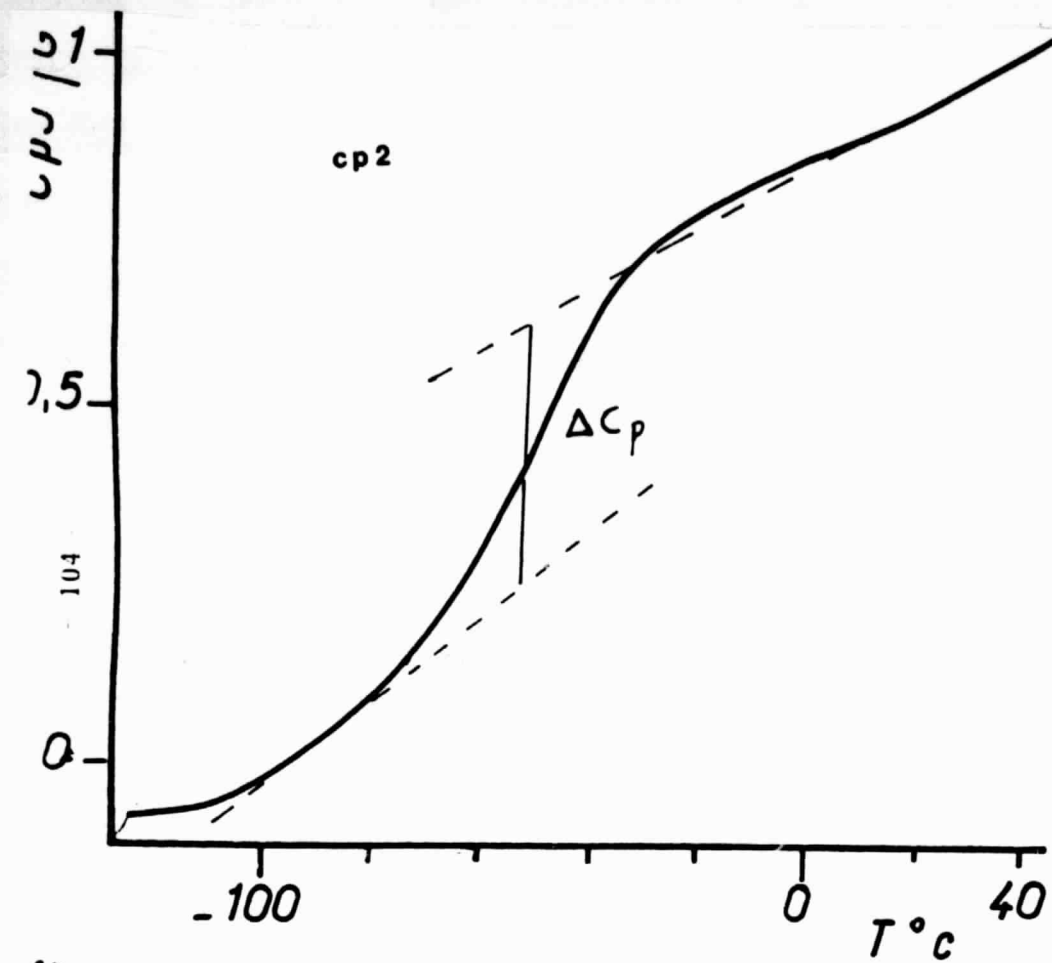
Figure 42 Measurements of \Delta C_p for the Polyurethane Matrix, CP2, and the Corresponding Glass Composite, V-CP2
