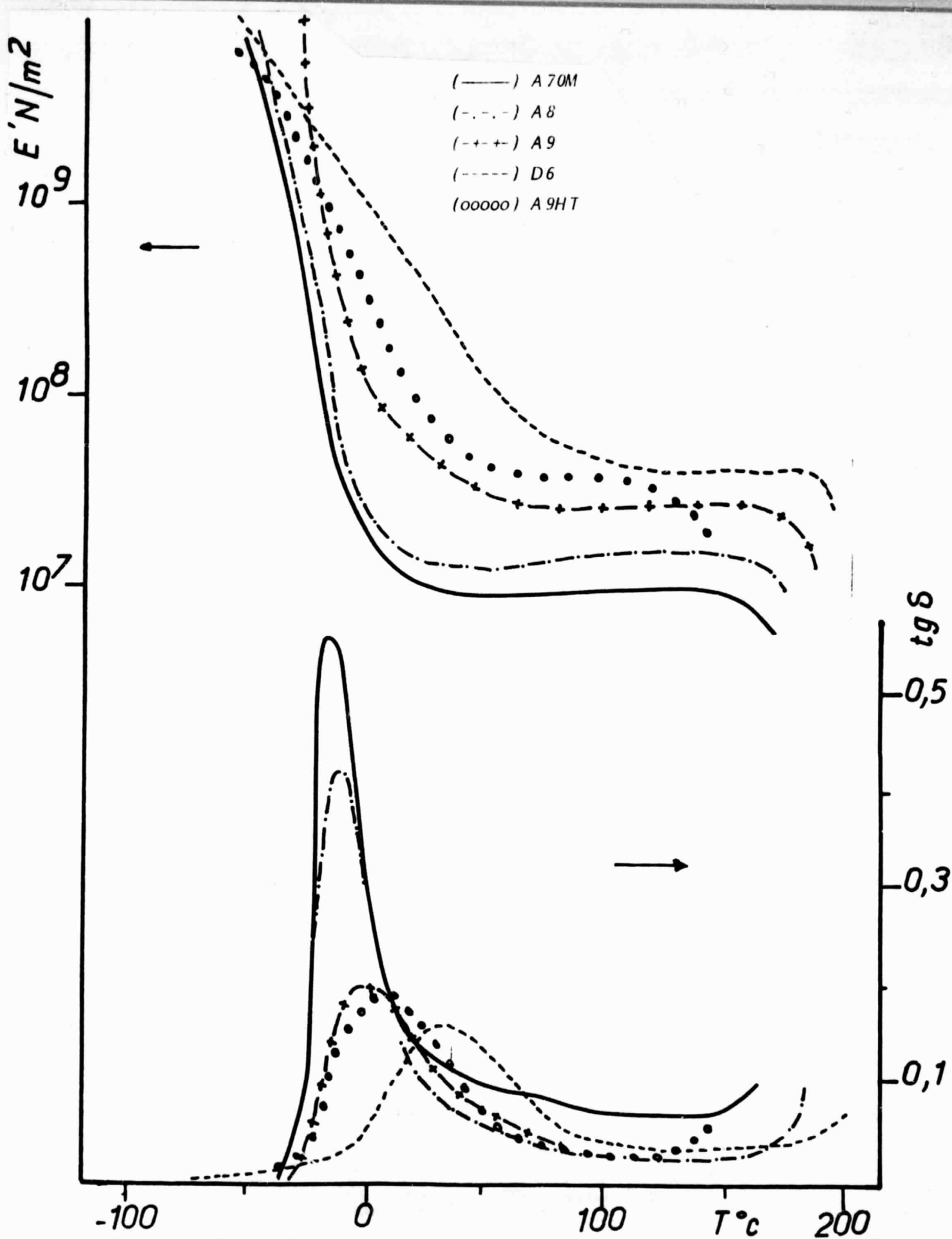
Figure 20 - Dynamic mechanical properties of commercial formulations for Cyanaprenes - Moca
