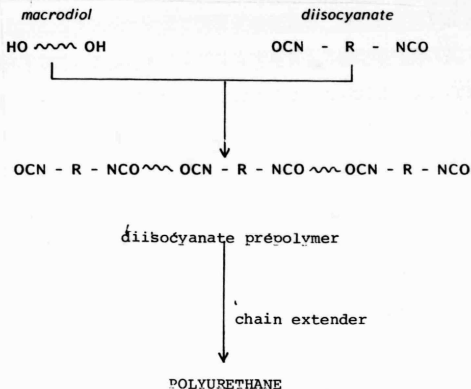
Fig 1 - Diagram of Polyurethane Synthesis
