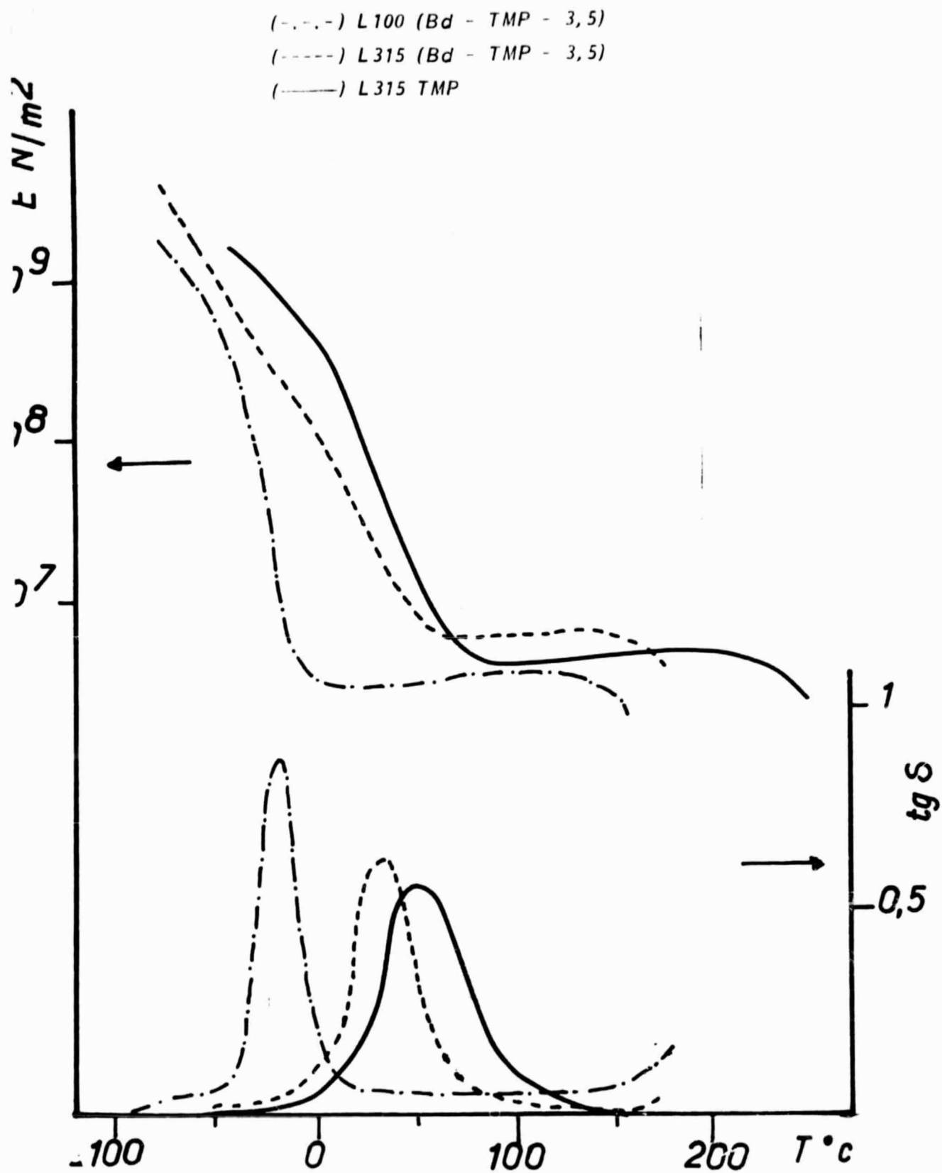
Figure 23 - Dynamic mechanical properties of PUR - alcohols
