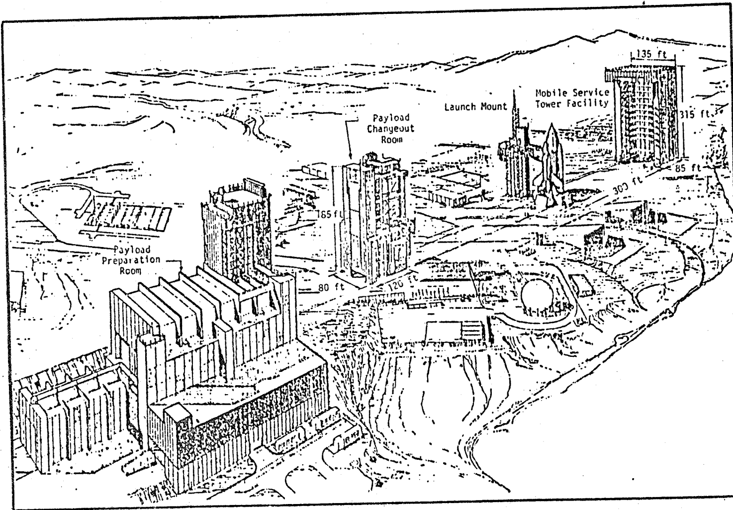
Figure 4.5. Launch site facility.
