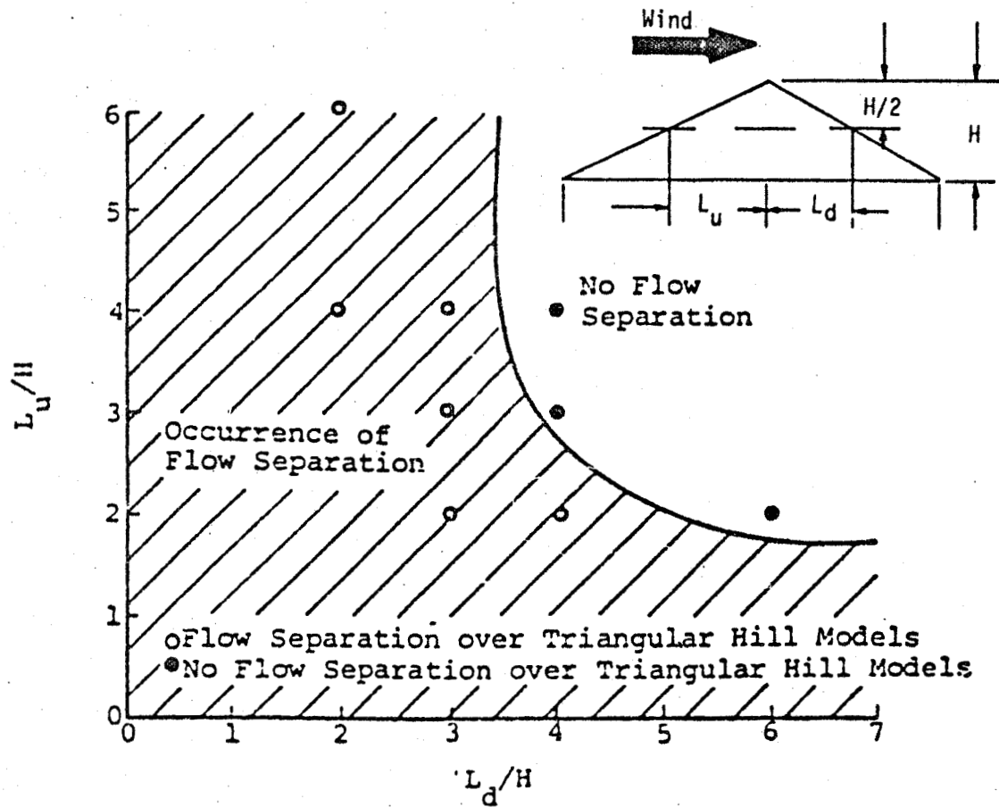
Figure 4.3. Criterion for flow separation over two-dimensional triangular hills.
