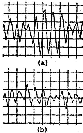
Oscillograms of Pressure Pulsations behind a Prismatic Model with a Sloping Roof. Each Horizontal Division--20 Milliseconds. Each Vertical Division--0.20 mm Hg. \rho u_{\infty}^2/2 = 0.60 mm Hg. (a) Region A (b) Region B
