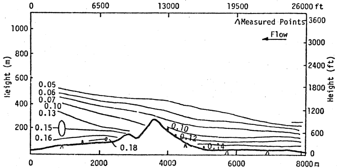
(b) Isoturbs for Model B with roughness.
