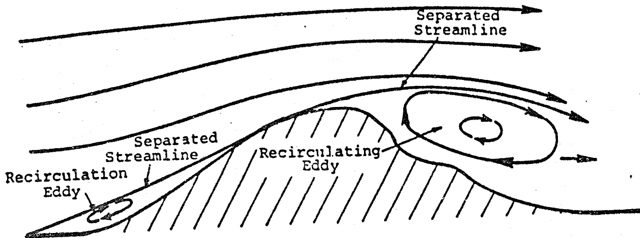
Figure 4.1. Flow separation.
