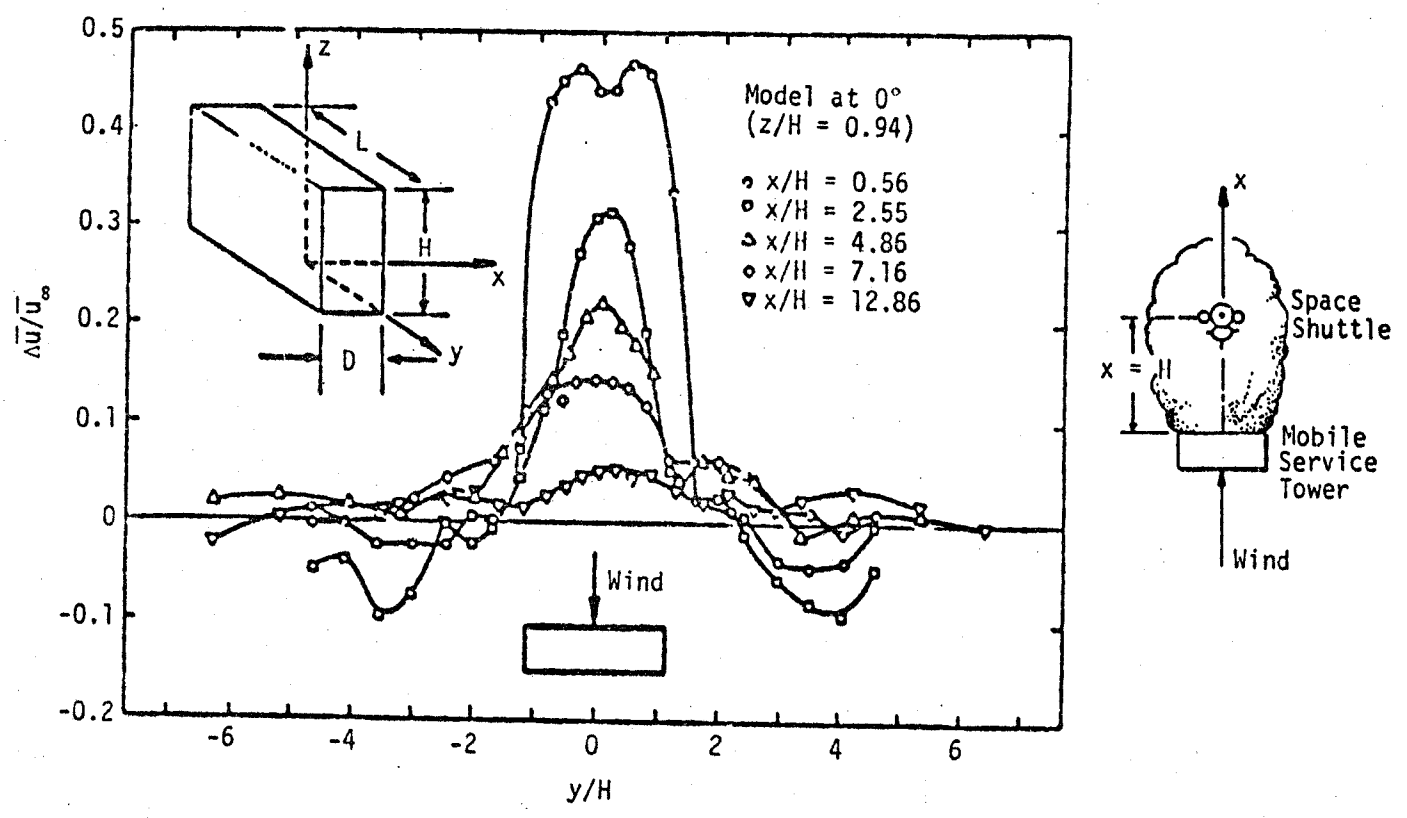
Figure 4.10. Lateral profiles of mean velocity deficit in the wake of a block at 0° (Woo et al. 1977).
