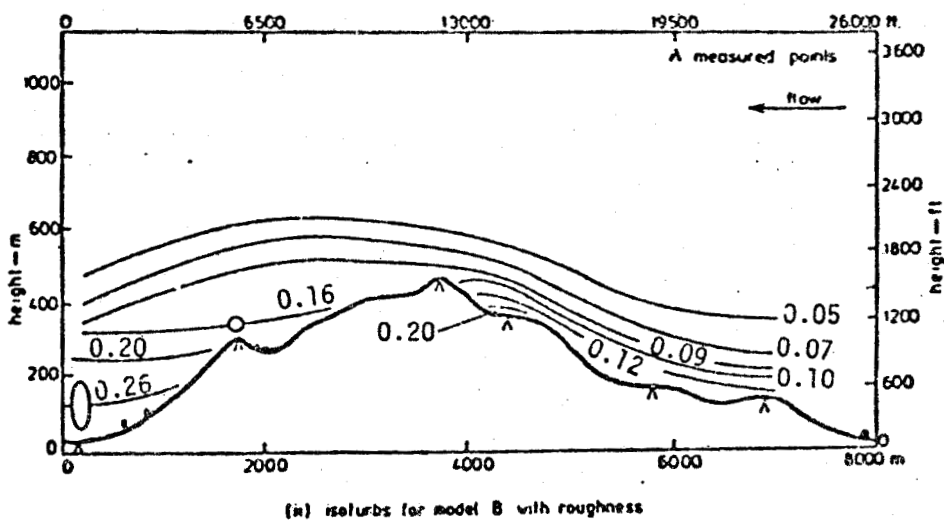
Figure 7.1. Isocontour graphs for longitudinal cross section YY.
