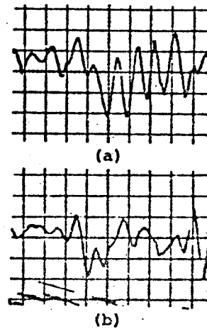
Oscillograms of Pressure Pulsations in Region C. Each Horizontal Division--20 Milliseconds. Each Vertical Division--0.20 mm Hg. \rho u_{\infty}^2/2 = 0.60 mm Hg. (a) Sloping Roof (b) Flat Roof
