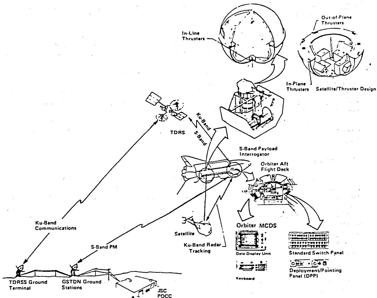
Figure 1. Design Overview - TSS/Orbiter/Ground Interfaces
