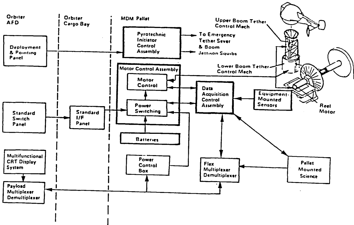
Figure 6. Design Overview - TSS Electrical Interfaces
