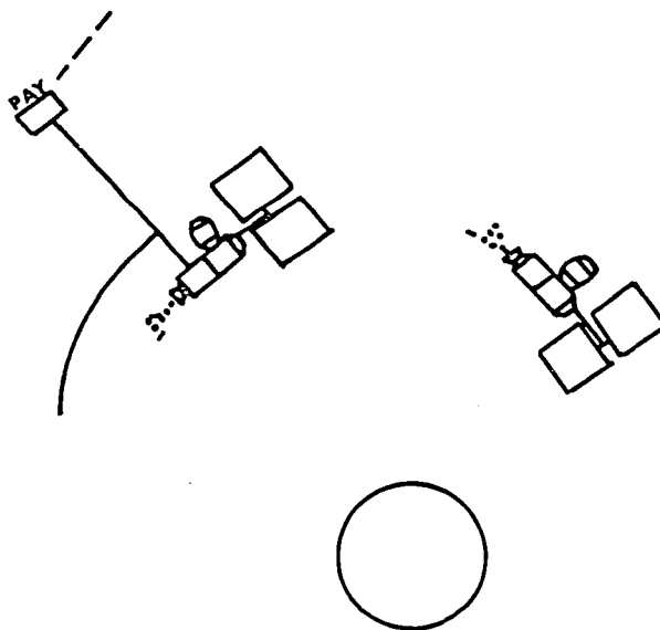
Figure 12. Using Station-Based Tether to Assist GEO or Deep Space Launch, Plus Electric Propulsion to Restore Orbit
