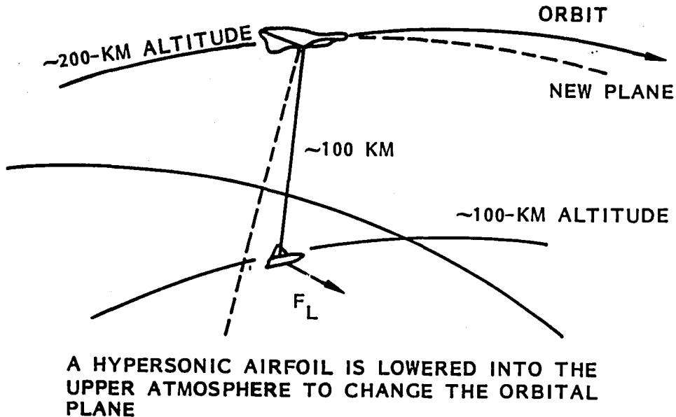
Figure 16. Satellite Sail
