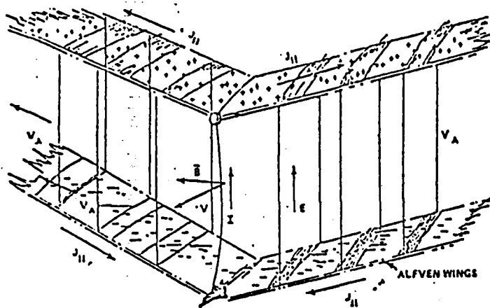
Figure 5. Schematic View of the Upper and Lower Current Sheets Which Spread Out from the Electrodynamics Tether System. The periodic darkened regions represent the outward propagation of Alfvén waves along the magnetic field. There is a net positive charge excess on the top wing and a net negative charge density on the lower wing.
