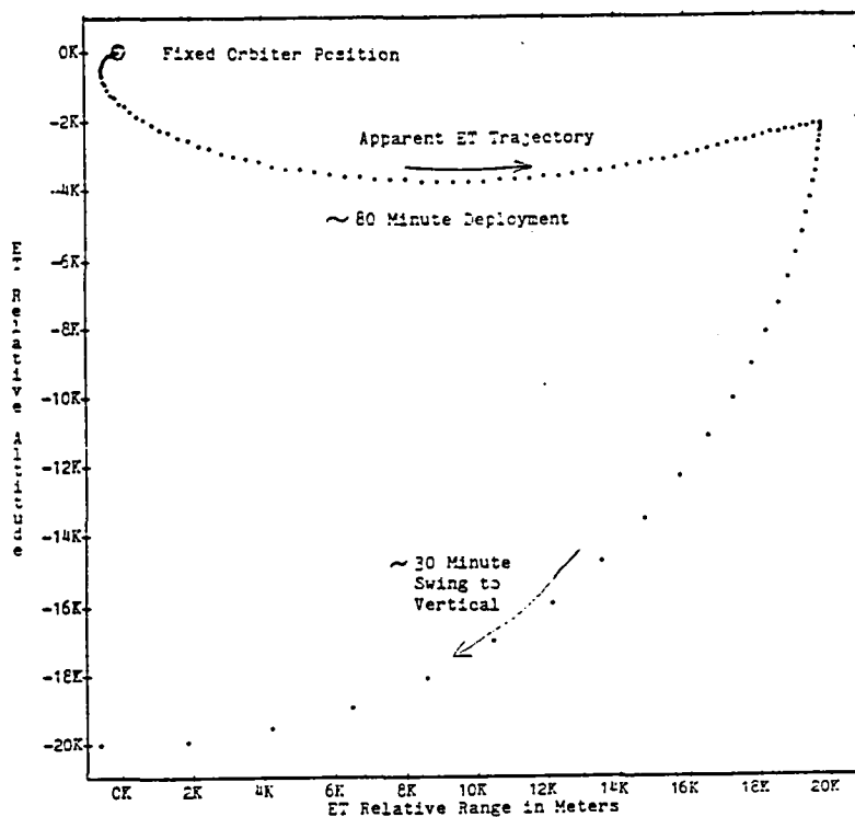
Figure 1. ET Position Relative To Orbiter at One-Minute Intervals
