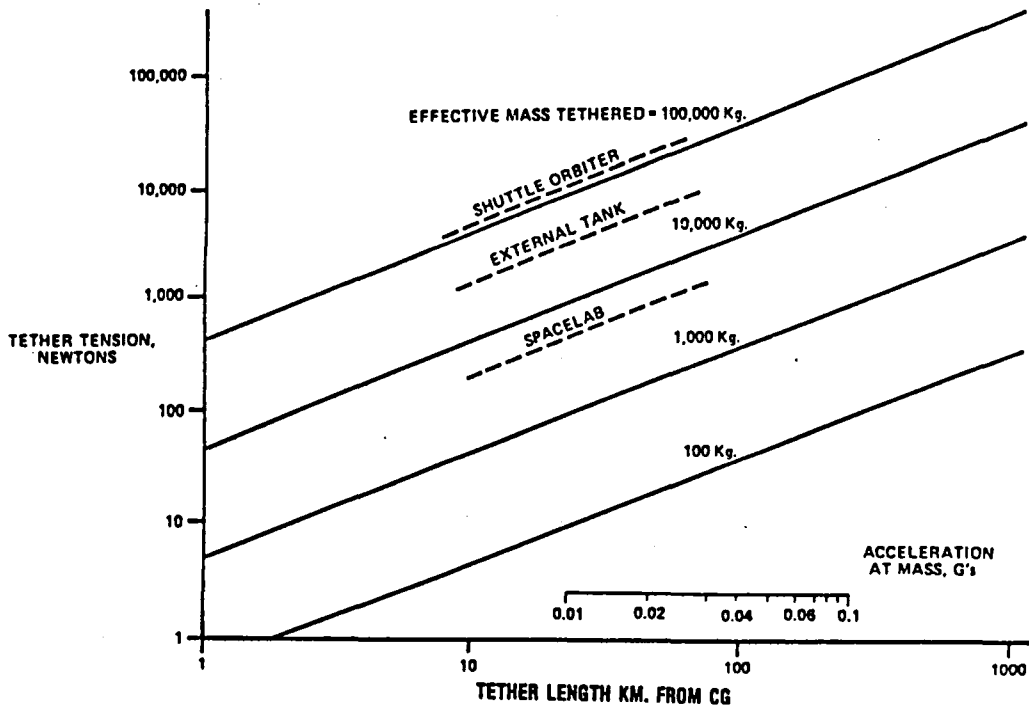
Figure 2. "Artificial Gravity" at Tethered Masses
