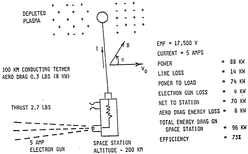
TETHER POWER GENERATOR
