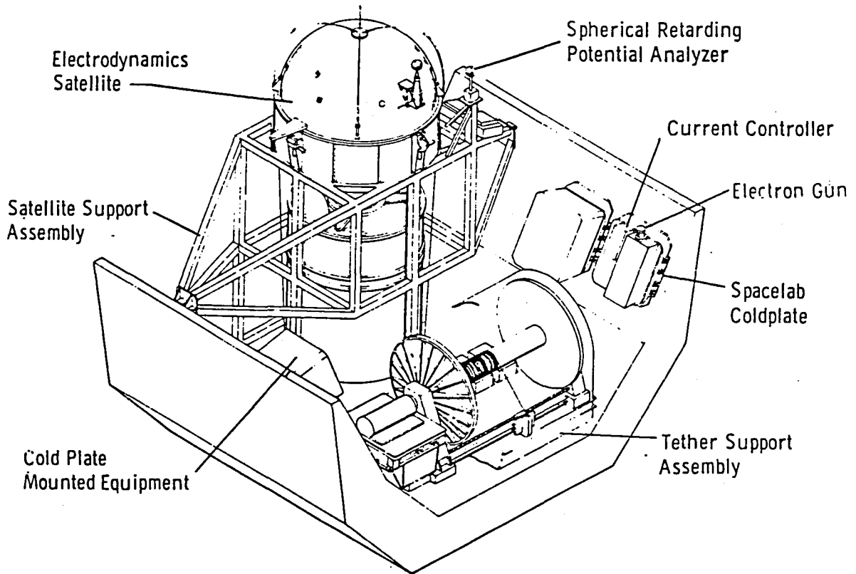
Figure 7. Design Overview - Electrodynamic Satellite
