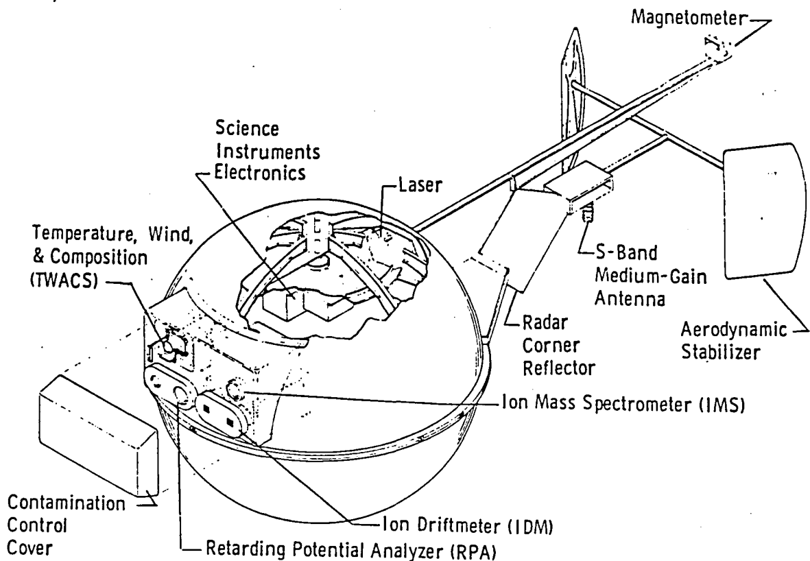
Figure 8. Design Overview - Atmospheric Probe Satellite
