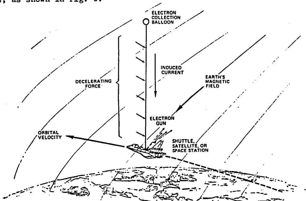
Figure 5. Tether As a Generator of High Power
