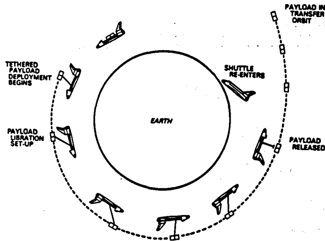
Figure 11. Payload Orbit is Raised and the Shuttle Deorbited
