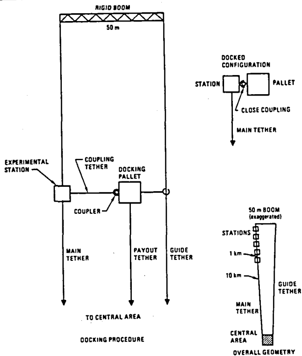
Transferring Pallet to Experimental Station
