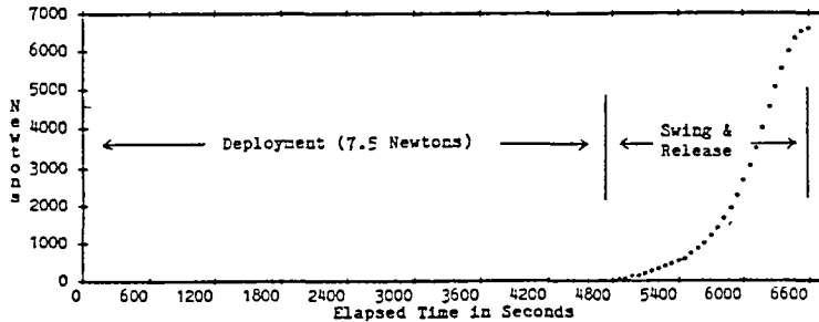
Figure 4. Tether Tension vs Time
