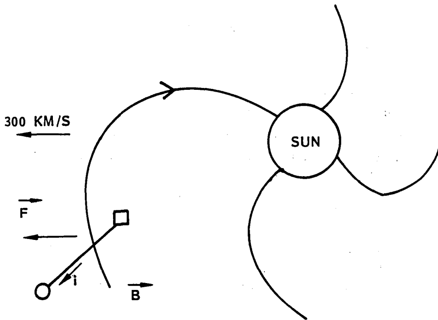
Figure 3. A Tether Thrust Generator for Interplanetary Missions
