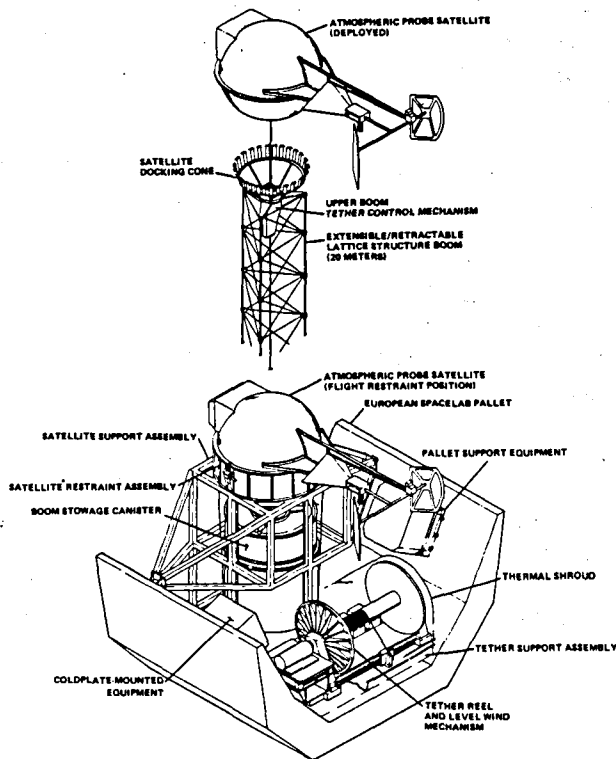
Figure 4. Typical Deployment and Control Mechanism
