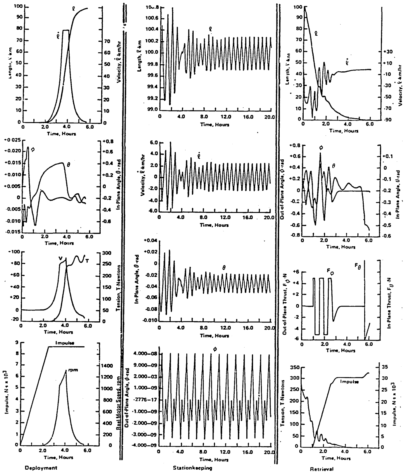
Figure 3. Typical Satellite Deployment, Stationkeeping, and Retrieval Profiles (130 km Deployment Altitude)
