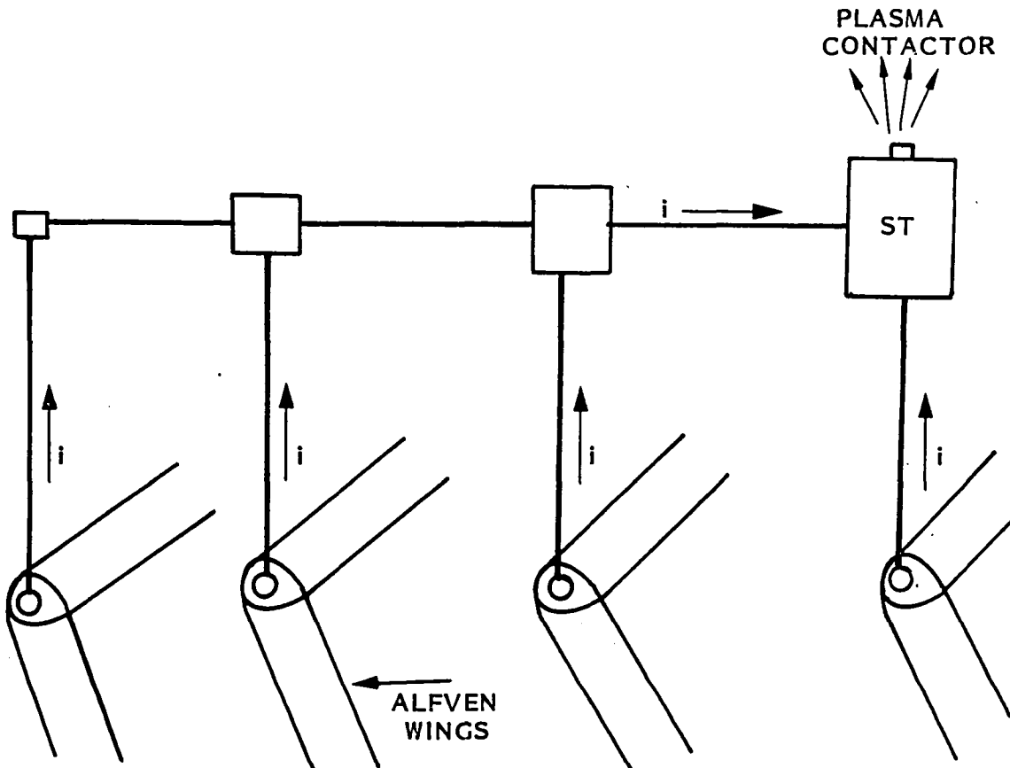
Figure 1. A Parallel Tether Current Generator
