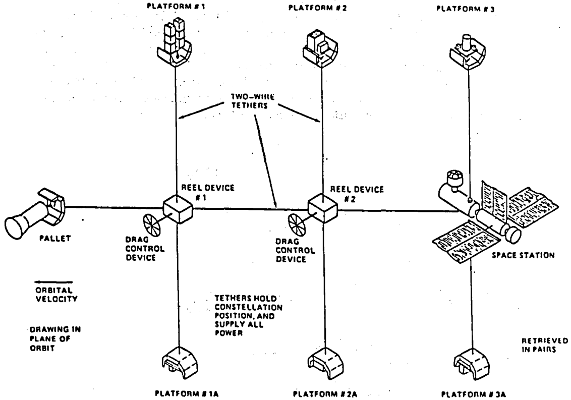
Figure 10. Two-Dimensional Tethered Constellation
