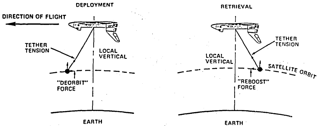
Figure 3. Deployment and Retrieval of a Tethered Satellite
