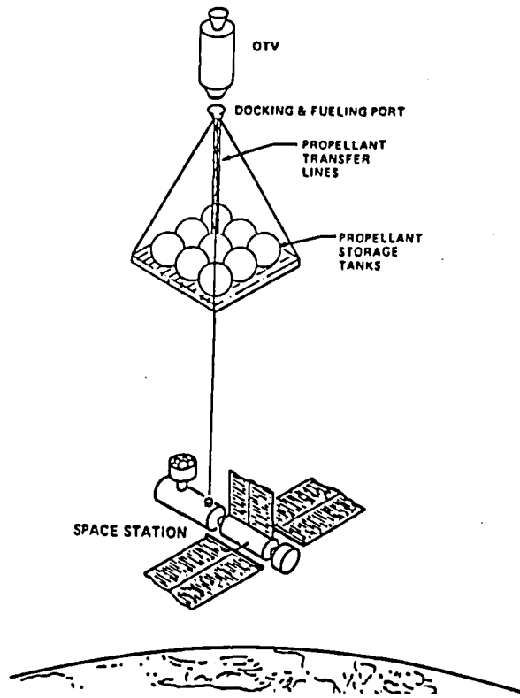
Figure 8. Cryogenic Propellant Storage and Transfer Platform
