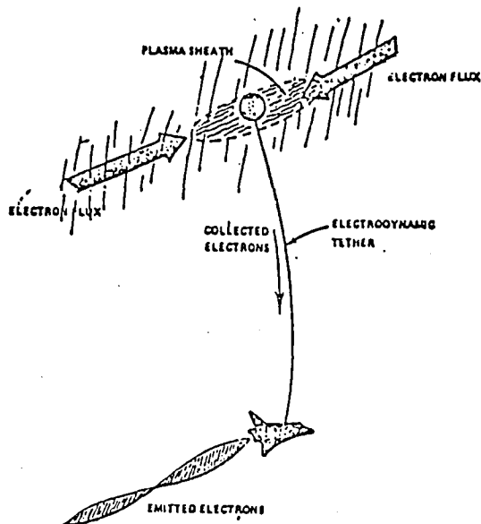
Figure 4. Basic Components of Electrodynamic Experiments with the Tethered Satellite System. The conducting tether is insulated along its length from the ionospheric plasma so electrons can enter or leave the system only at the satellite and the Orbiter. Active electron emission occurs at the Orbiter, while electron collection takes place at the electrodynamic satellite.
