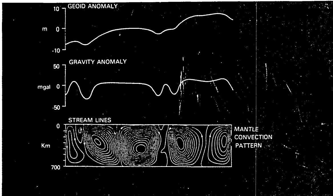
EXAMPLE OF GRAVITY AND GEOID ANOMALIES PRODUCED BY CONVECTION IN THE MANTLE (AFTER WATTS AND DALY, 1981)
