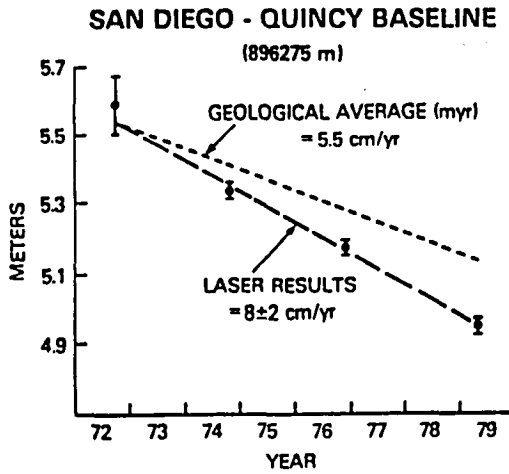
MOTION ALONG THE SAN ANDREAS FAULT
