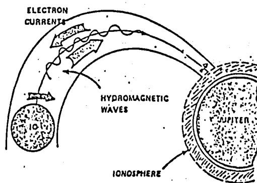
Figure 7. Schematic View of the Interaction of Io with the Rapidly Rotating Jovian Ionosphere. Large magnetic field-aligned currents connect to the Jovian ionosphere, propagating at the Alfvén speed in the moving medium.
