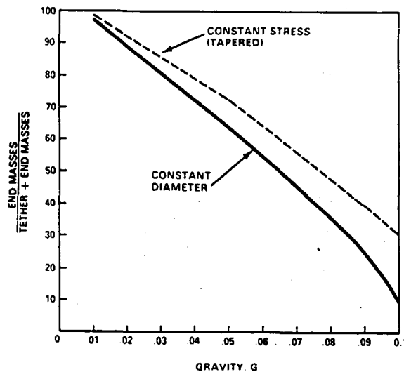
Figure 7. Mass of Tether Grows with Desired Gravity Level
