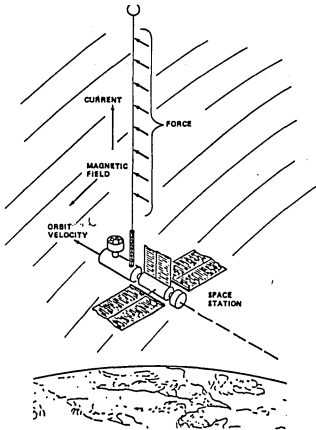
"ELECTRIC MOTOR EFFECT REBOOST"
