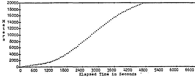
Figure 3. Deployed Tether Length vs Time
