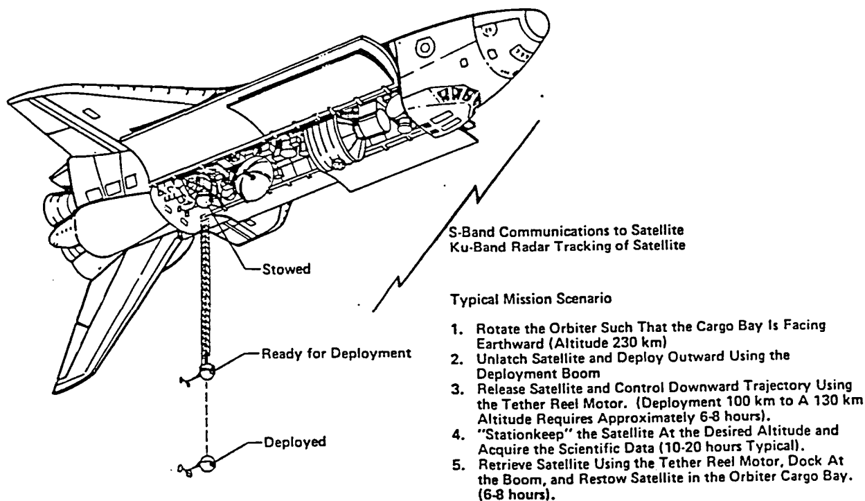
Figure 2. Design Overview - TSS Deployment Concept
