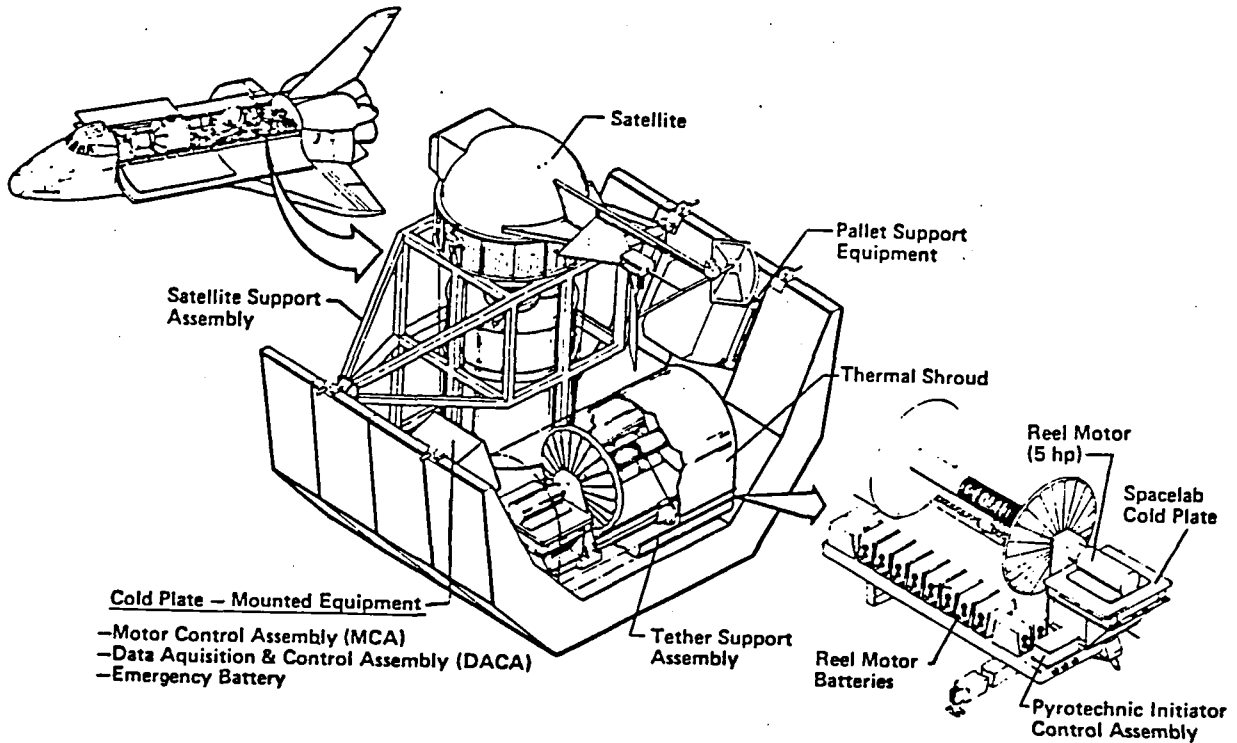
Figure 4. Design Overview - TSS/Pallet/Orbiter Interface
