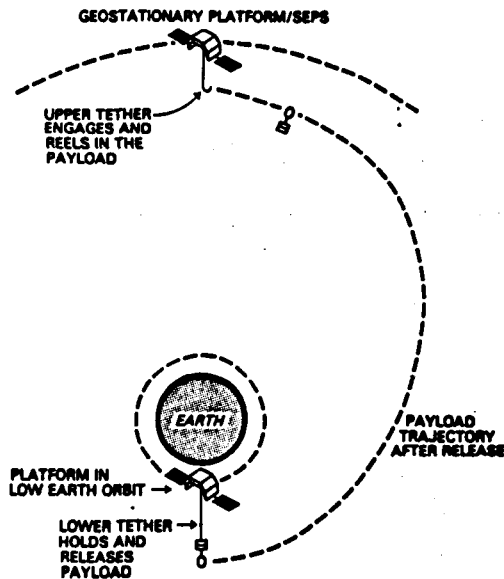
Figure 12. Two-Piece Tether "Elevator"
