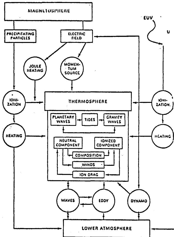
Figure 1. Schematic Diagram Illustrating the Important Processes Linking the Lower Atmosphere, Thermosphere, and Magnetosphere. Within the thermosphere a variety of waveforms are generated ranging from planetary scale to gravity waves.
