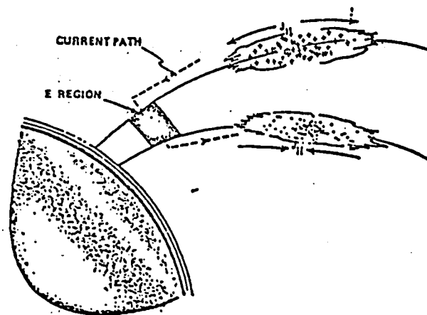
Figure 6. Illustrating the Magnetic Field-Aligned Currents Which Are Caused in the Ionosphere by the Transfer of Electrons from the TSS Satellite to the Shuttle. The net charge imbalance spreads along the magnetic field until the perpendicular resistivity is sufficiently high to permit transverse currents to connect the two magnetic flux shells.
