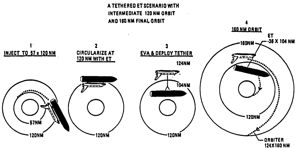
Figure 3. Downward Release of ET from Shuttle Orbit
