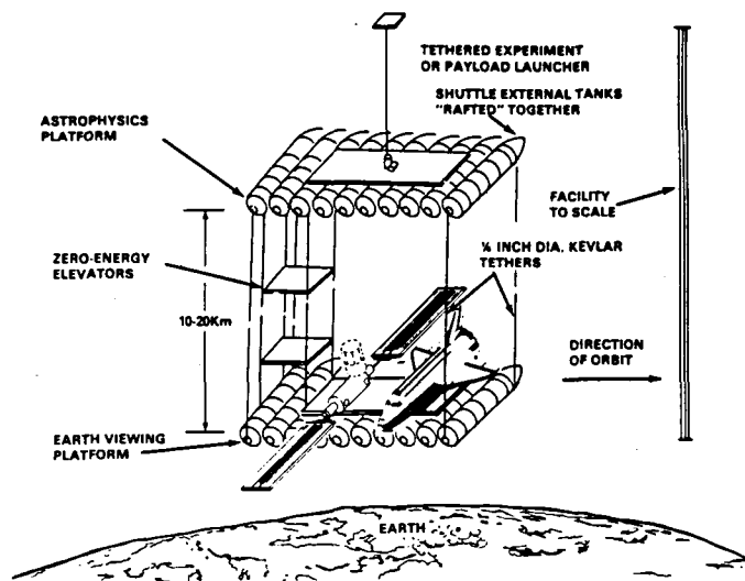
Figure 9. Passive Space Facility
