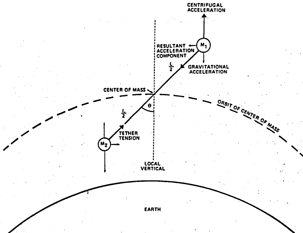
Figure 1. Stabilizing Forces Acting on Tethered Masses
