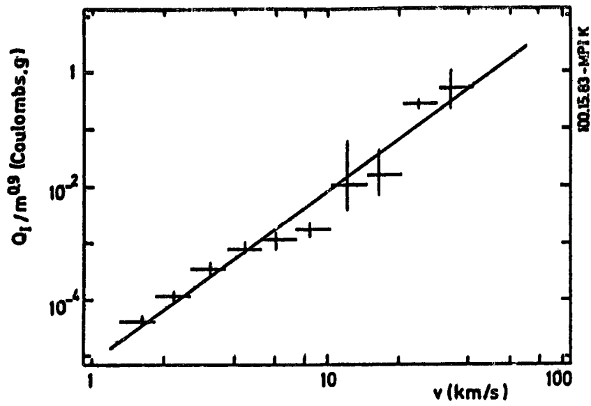
Fig. 2: Positive impact charge Q_I normalized to m^{0.9} versus impact speed v for iron projectiles.
