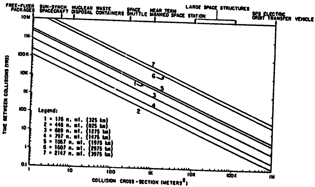
FIGURE 10. EXPECTED TIMES BETWEEN COLLISIONS AFTER 20 YEARS, AS A FUNCTION OF COLLISION CROSS-SECTION
