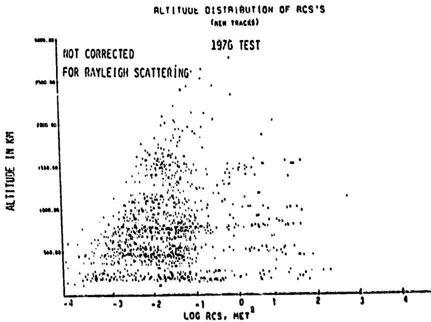
FIGURE 3 - Altitude Distribution of RCS's (New Tracks Only).
