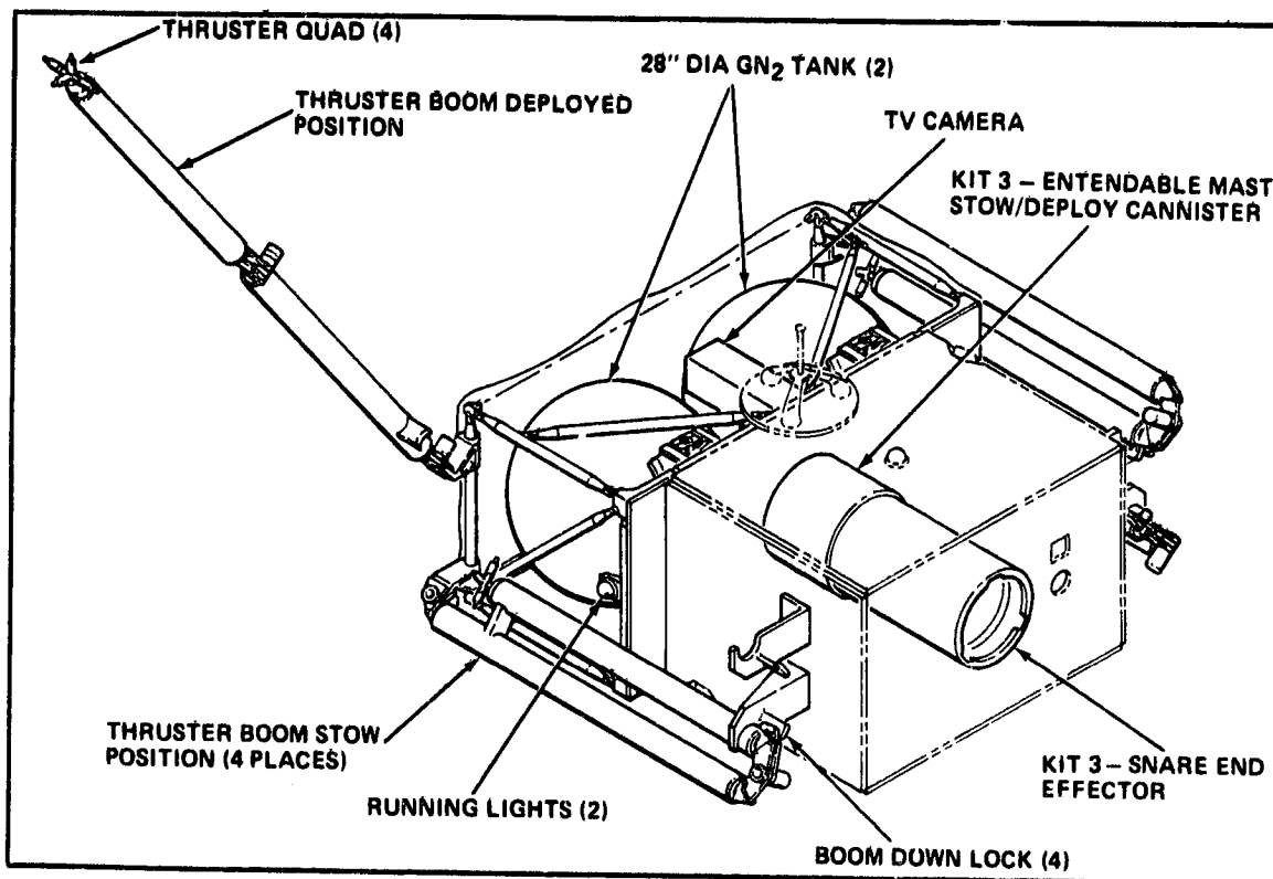
Fig. 12 MTV-POM Kit 2 - Satellite (5000 kg) Retrieval
