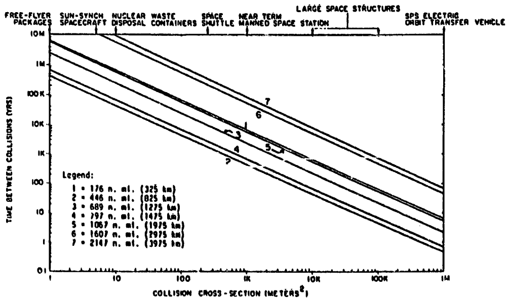
FIGURE 5. EXPECTED TIMES BETWEEN COLLISIONS AFTER 20 YEARS, AS A FUNCTION OF COLLISION CROSS-SECTION
