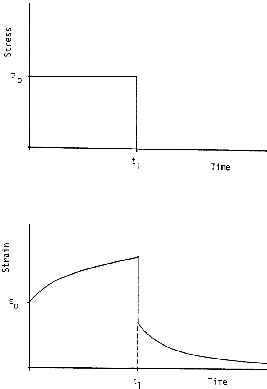
Figure 2.1: Stress and Strain Histories for a Creep/Creep Recovery Test
