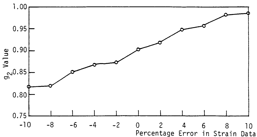
Figure 4.13: Sensitivity of g_2 to Percentage Errors in Strain Data; Stress = 1750 psi, A_0 = 0.674 , C = 0.0145 , n = 0.33
