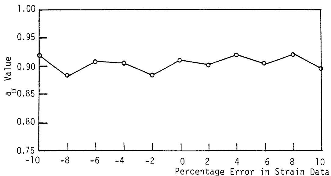
Figure 4.14: Sensitivity of a_0 to Percentage Errors in Strain Data; Stress = 1750 psi, A_0 = 0.674 , C = 0.0145 , n = 0.33
