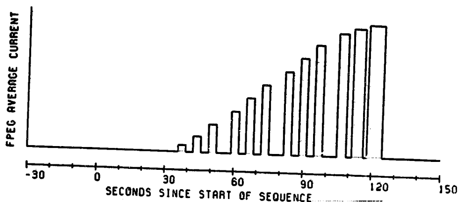
Figure 4. - Sequence of electron current pulses emitted by the Fast Pulse Electron Generator.
