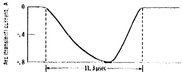
(a) Fully exposed solar module. Applied voltage, -600 V; capacitance, 0.01 μF.
