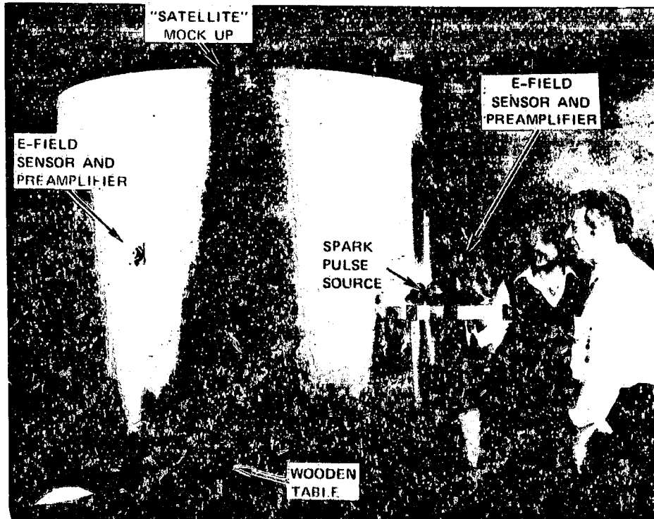
Figure 6. - Satellite mock-up.
