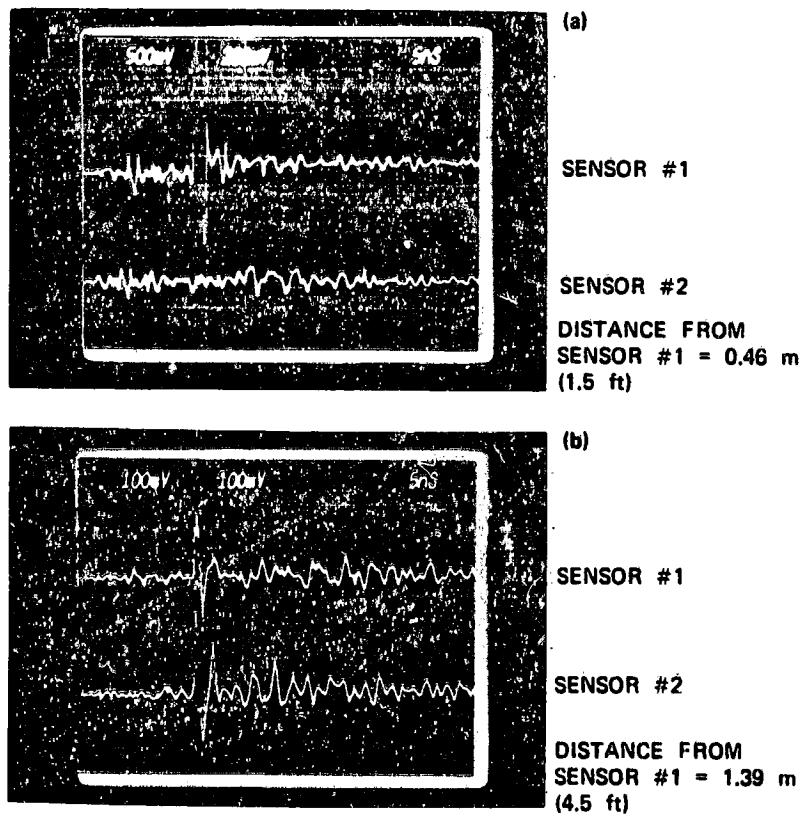
Figure 8. - Sensor responses.
