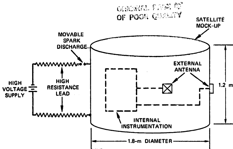
Figure 7. - SRI laboratory test of discharge localization technique.
