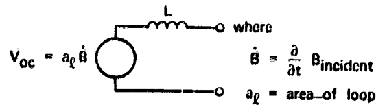
(a) THEVENIN EQUIVALENT CIRCUIT OF MAGNETIC DIPOLE
