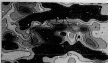
MAGSAT 1 DEGREE FILTERED
