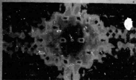
2D FFT of Australian Region 2 degree average data
