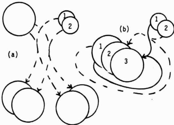
Figure 8. Concurrency control would prevent these lost updates and inconsistency. This represents the situation in Case 4 where a data entity is (a) in either the readset or the writeset or (b) in both the readset and the writeset.
