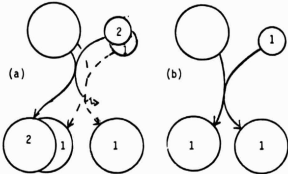
Figure 7. Failure control eliminates all the effects of aborting a transaction (a) back to the previous state (b). While a transaction is in progress access to writesets could be blocked by concurrency control.
