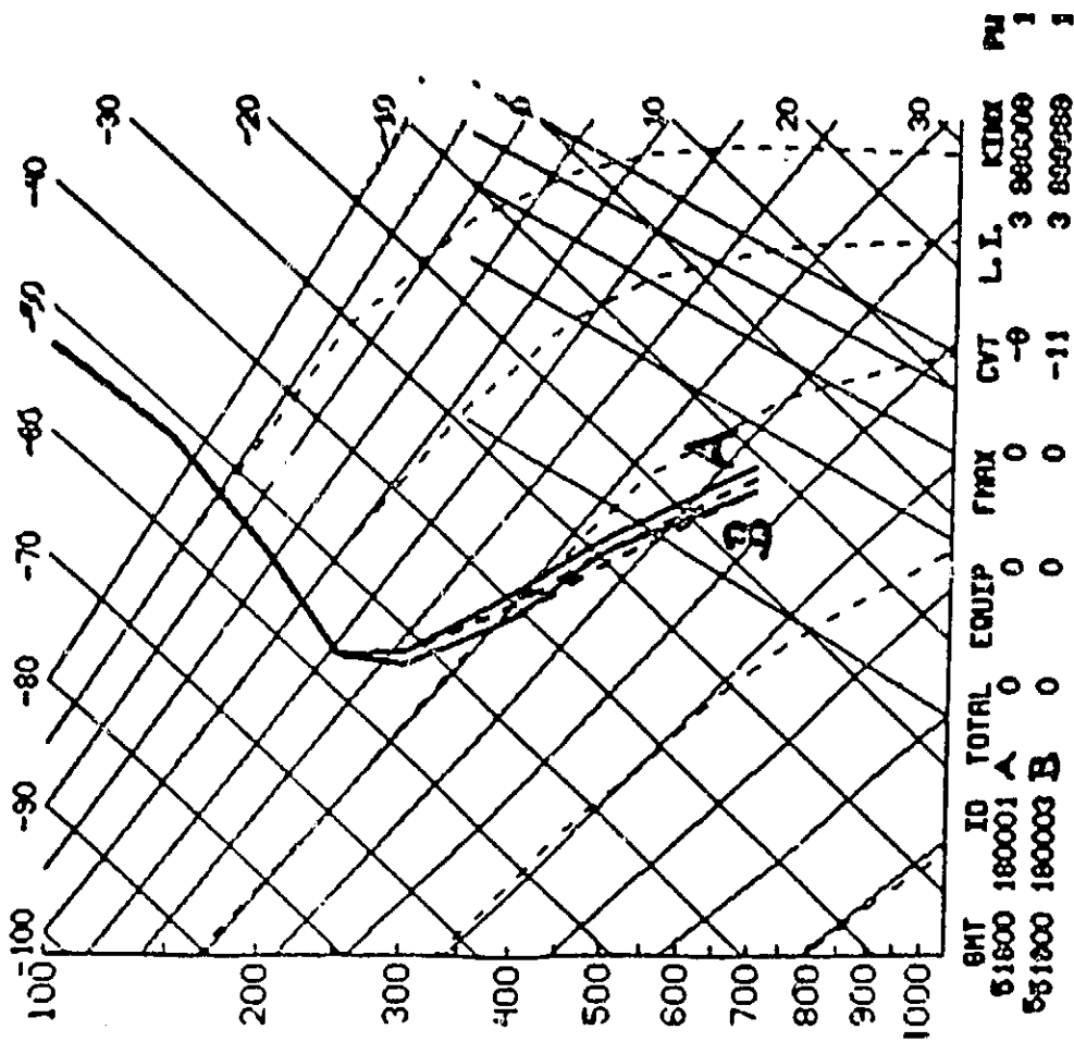
Figure 7. Single FOV retrievals at Pontresina (A) and Umbrail Pass (B), solid lines are temperatures.
