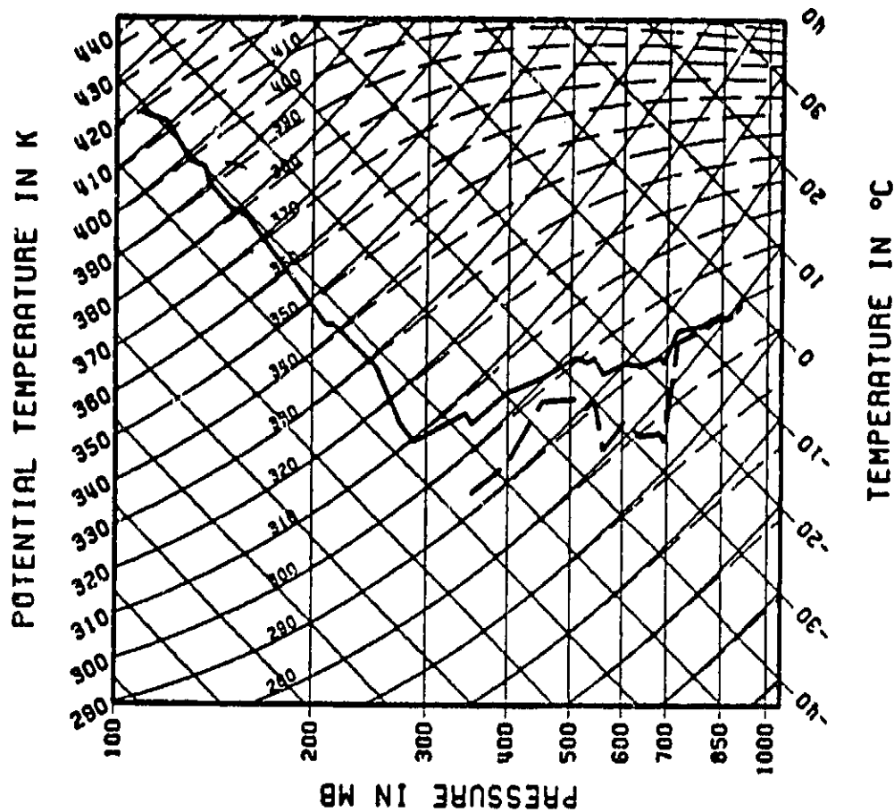
Figure 12. Radiosonde observation of Hohenpeißenberg, 5 March 1982, 1050 GMT.
