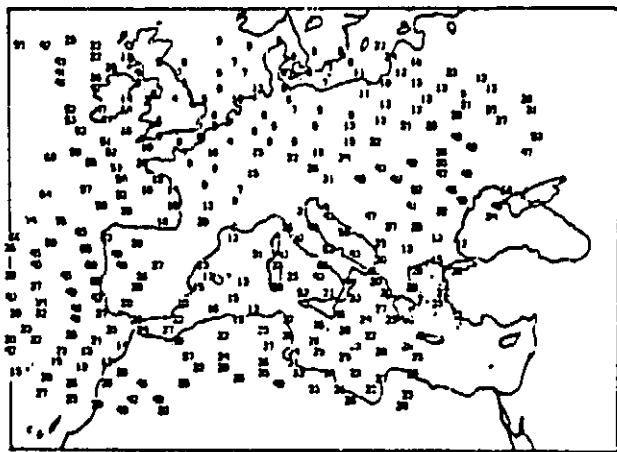
PREC. WATER ABOVE 700MB(ICM=100) 5 MAR 1982 03Z
