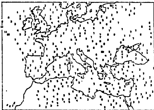
PREC. WATER ABOVE 500MB(ICM=100) 4 MAR 1982 13Z
