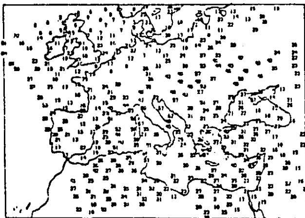
PREC. WATER ABOVE 700MB(ICM=100) 4 MAR 1982 13Z
