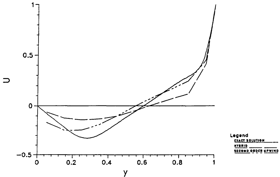
Fig. 13. Comparison of Vertical Center-line u-velocity Profile for Re = 400, 10x10 Grid
