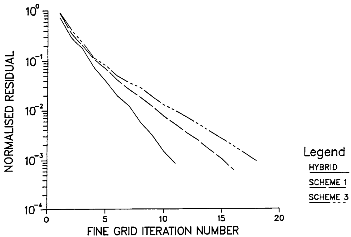
Fig. 4. Rates of Convergence, Re = 100 , 20 \times 20 Grid
