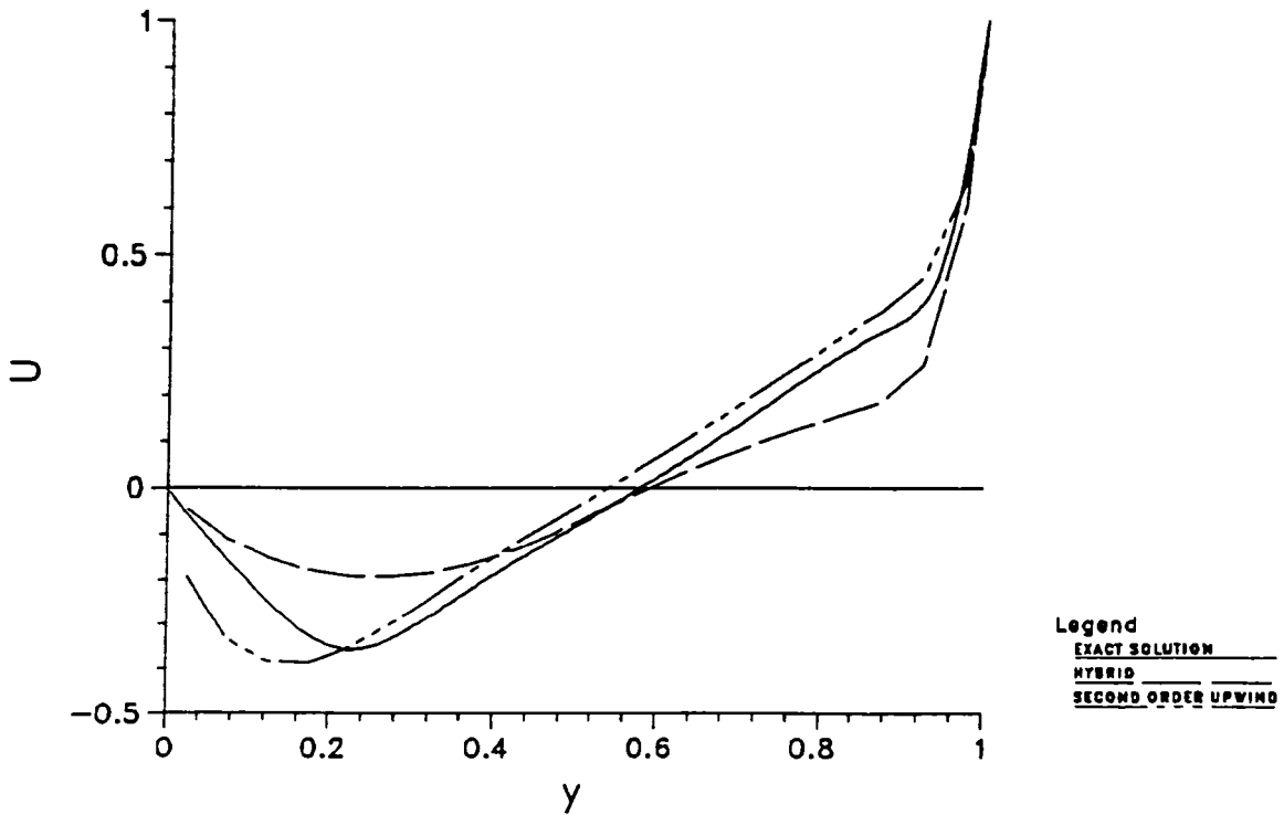
Fig. 22. Comparison of Vertical Center-line u-velocity Profile for Re = 600, 20x20 Grid
