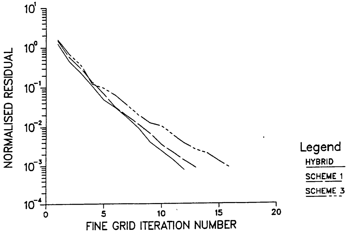
Fig. 5. Rates of Convergence, Re = 100, 40x40 Grid
