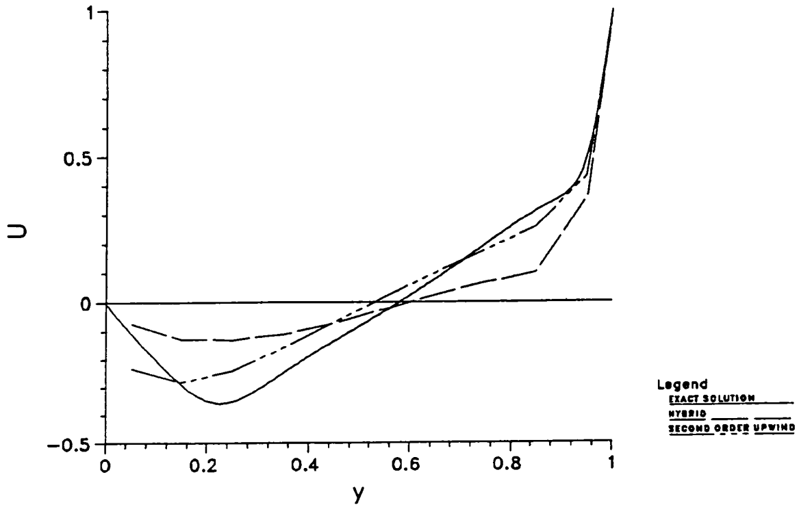
Fig. 21. Comparison of Vertical Center-line u-velocity Profile for Re = 600, 10x10 Grid
