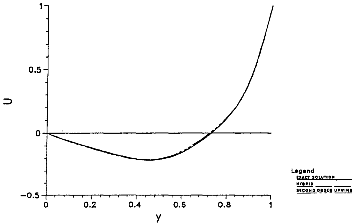
Fig. 8. Comparison of Vertical Center-line u-velocity Profile for Re = 100, 40x40 Grid
