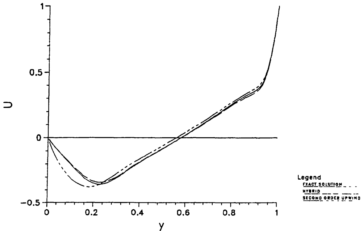
Fig. 24. Comparison of Vertical Center-line u-velocity Profile for Re = 600, 80x80 Grid
