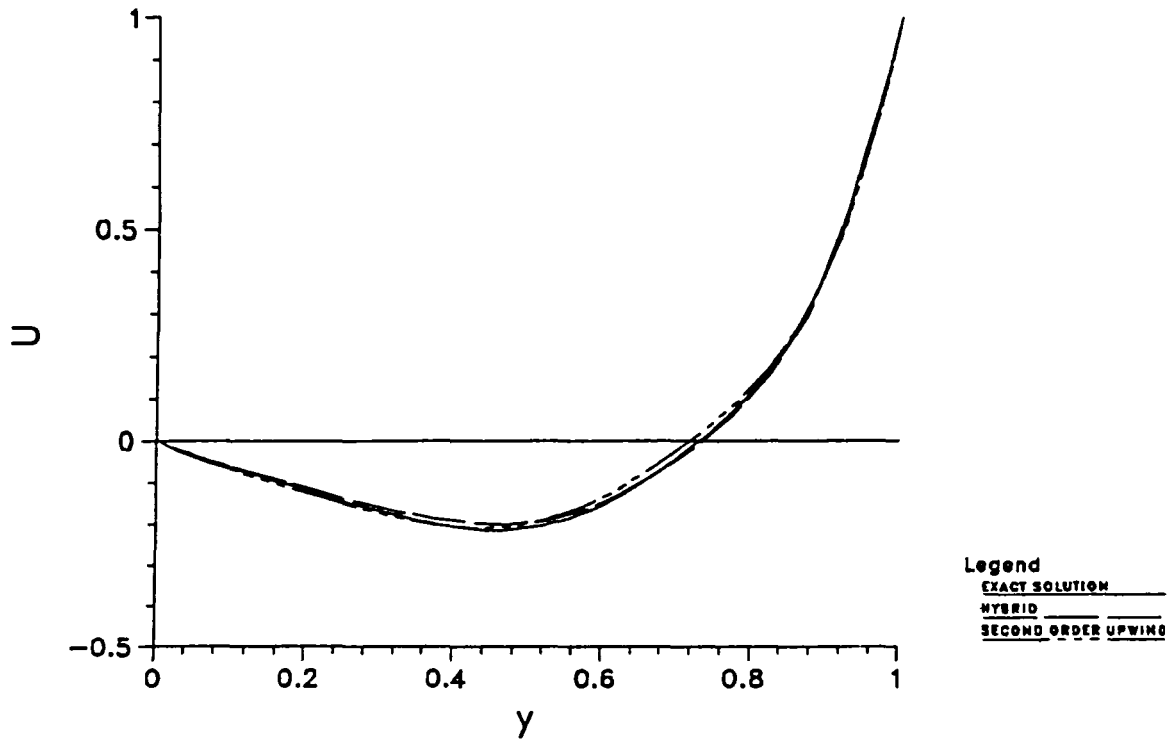
Fig. 7. Comparison of Vertical Center-line u-velocity Profile for Re = 100, 20x20 Grid
