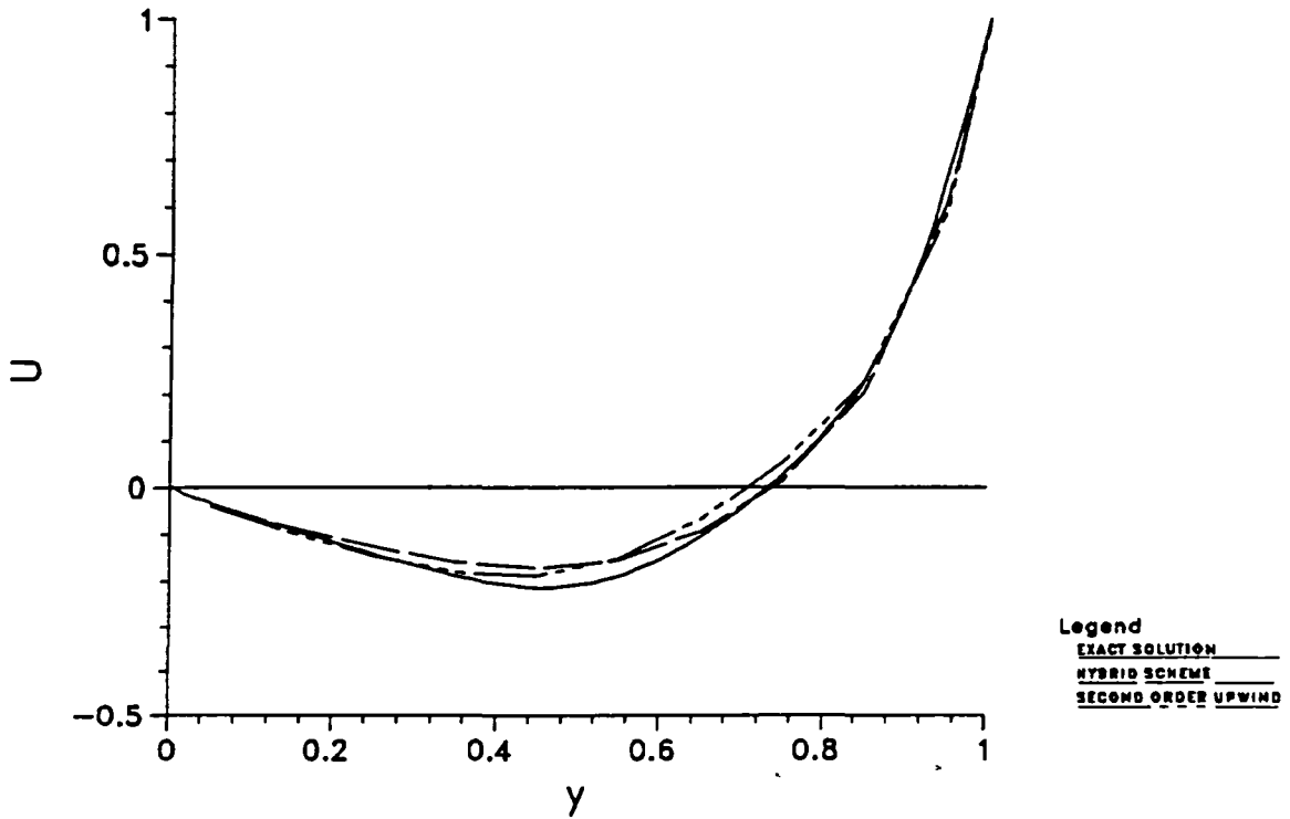
Fig. 6. Comparison of Vertical Center-line u-velocity Profile for Re = 100, 10x10 Grid
