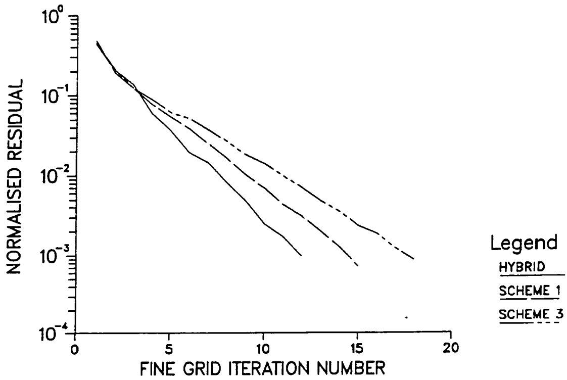
Fig. 3. Rates of Convergence, Re = 100 , 10 \times 10 Grid
