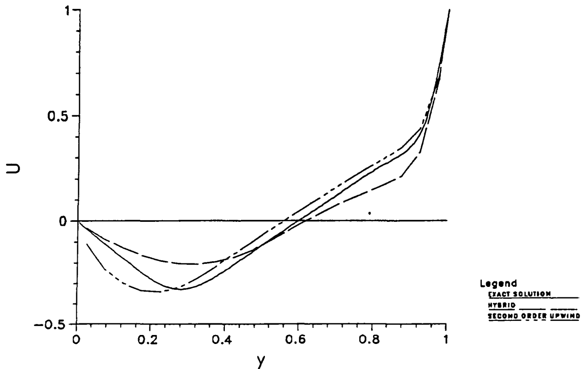
Fig. 14. Comparison of Vertical Center-line u-velocity Profile for Re = 400, 20x20 Grid
