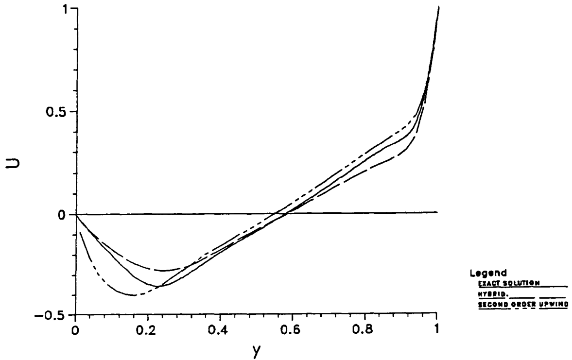
Fig. 23. Comparison of Vertical Center-line u-velocity Profile for Re = 600, 40x40 Grid
