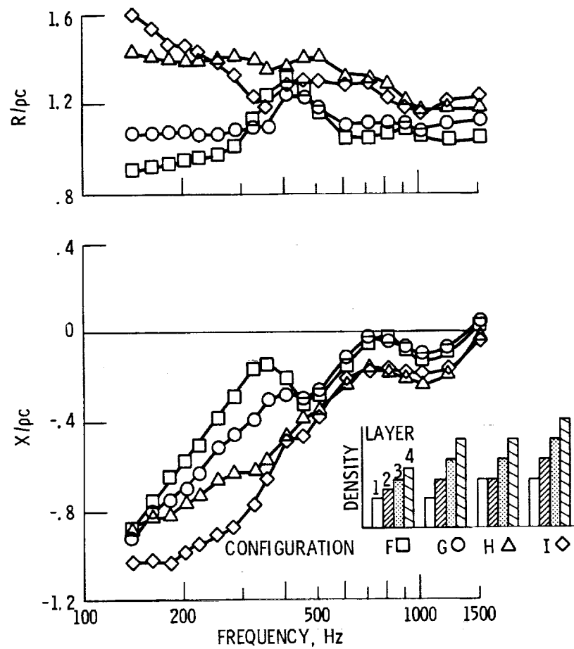
Figure 10. - Measured specific acoustics impedance of 4 layer configurations.
