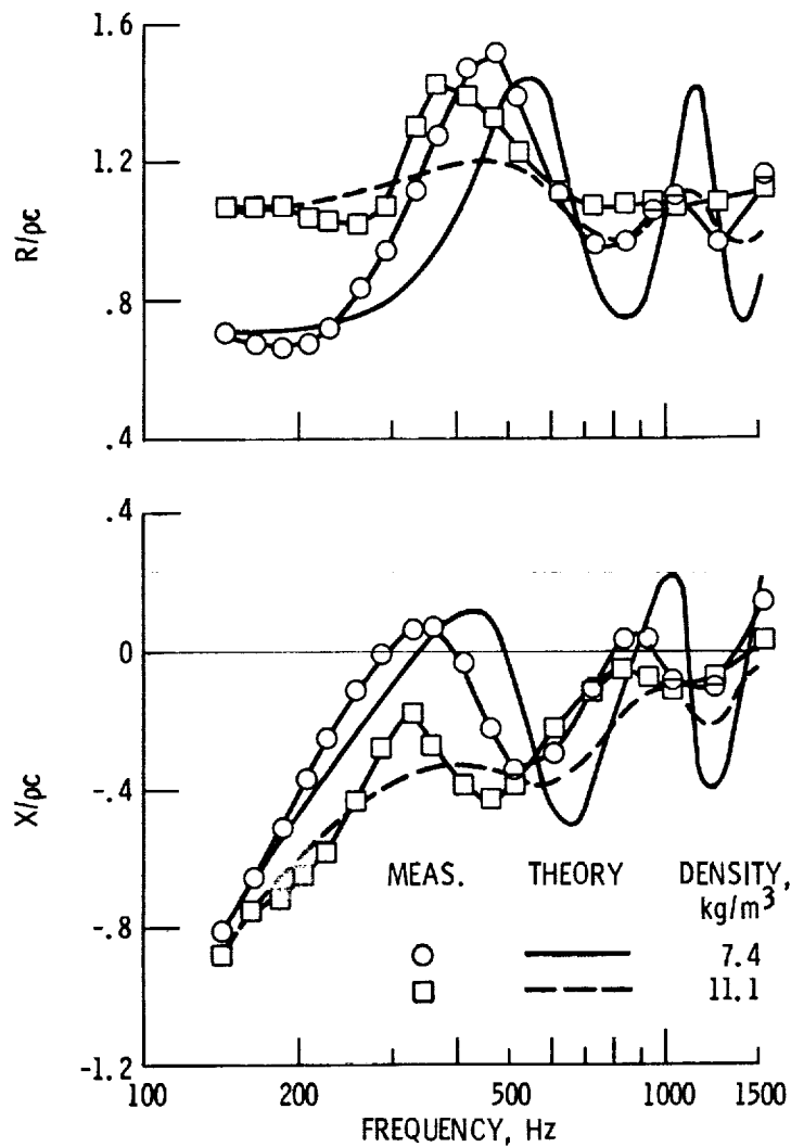
Figure 4. - Specific acoustic impedance of uniform density bulk absorbers with depth of 30.5 cm (12 in).
