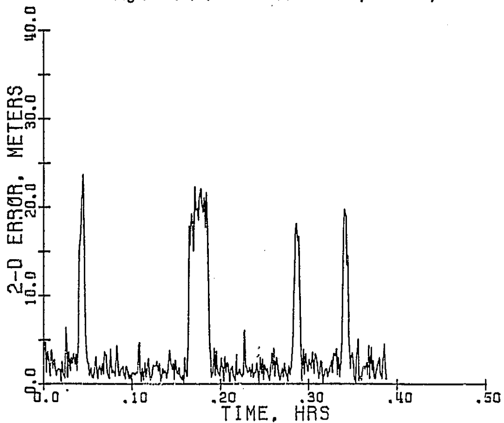
Figure 4.0.6.3 2D Position Error, Run D-8, with SA
