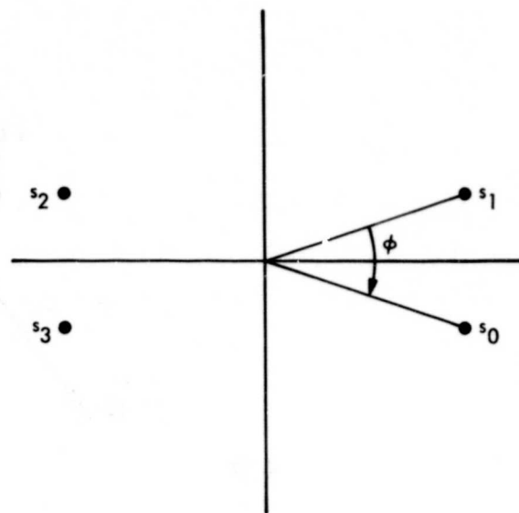
ASYMMETRIC 4-PSK
