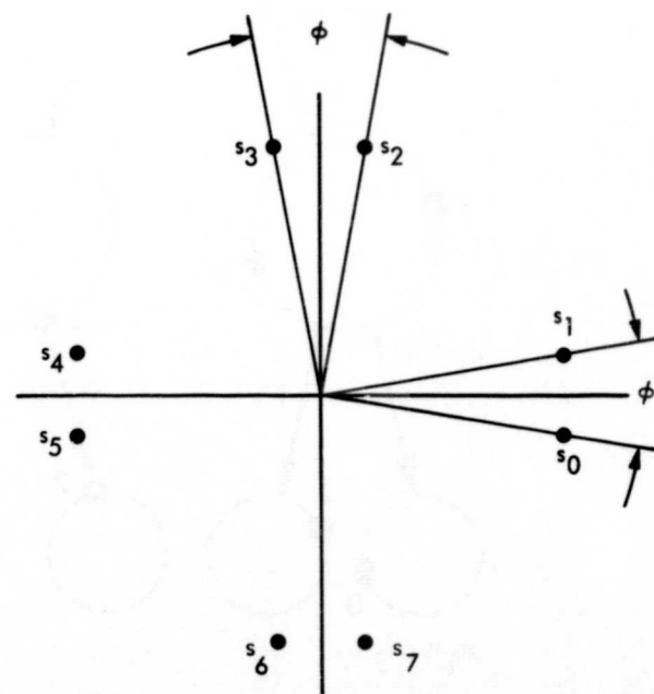
ASYMMETRIC 8-PSK
