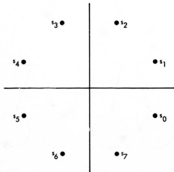
SYMMETRIC 8-PSK
