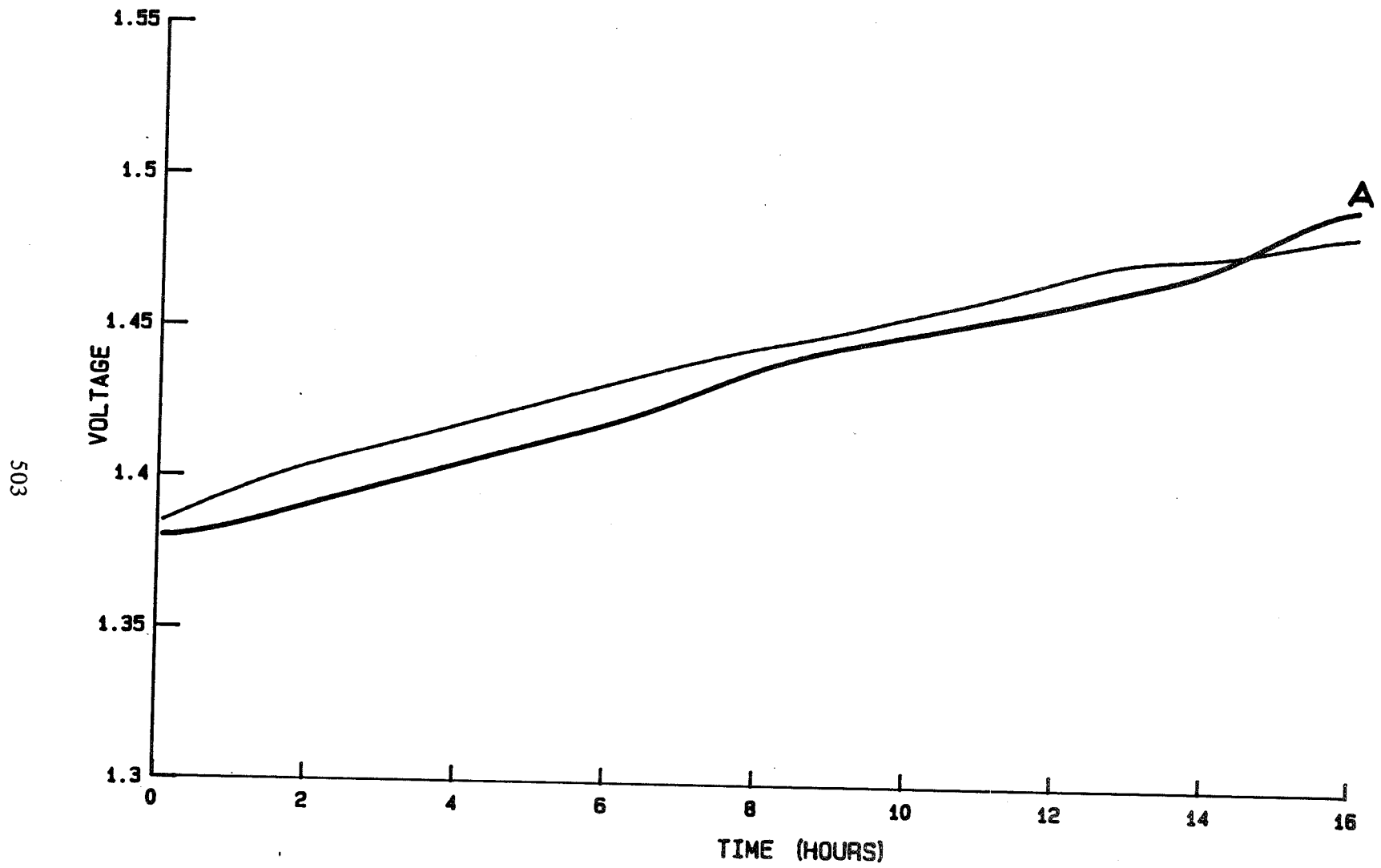
Figure 11. 20 Degree Charge
