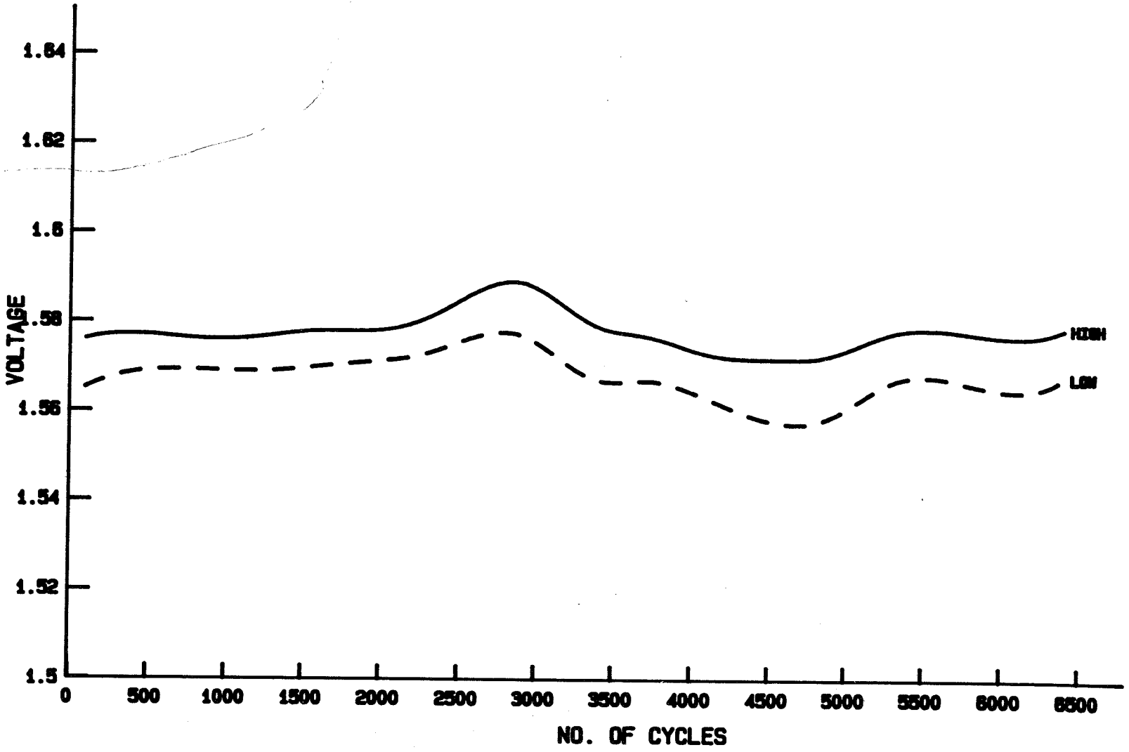
Figure 4. End-of-Charge Voltages
