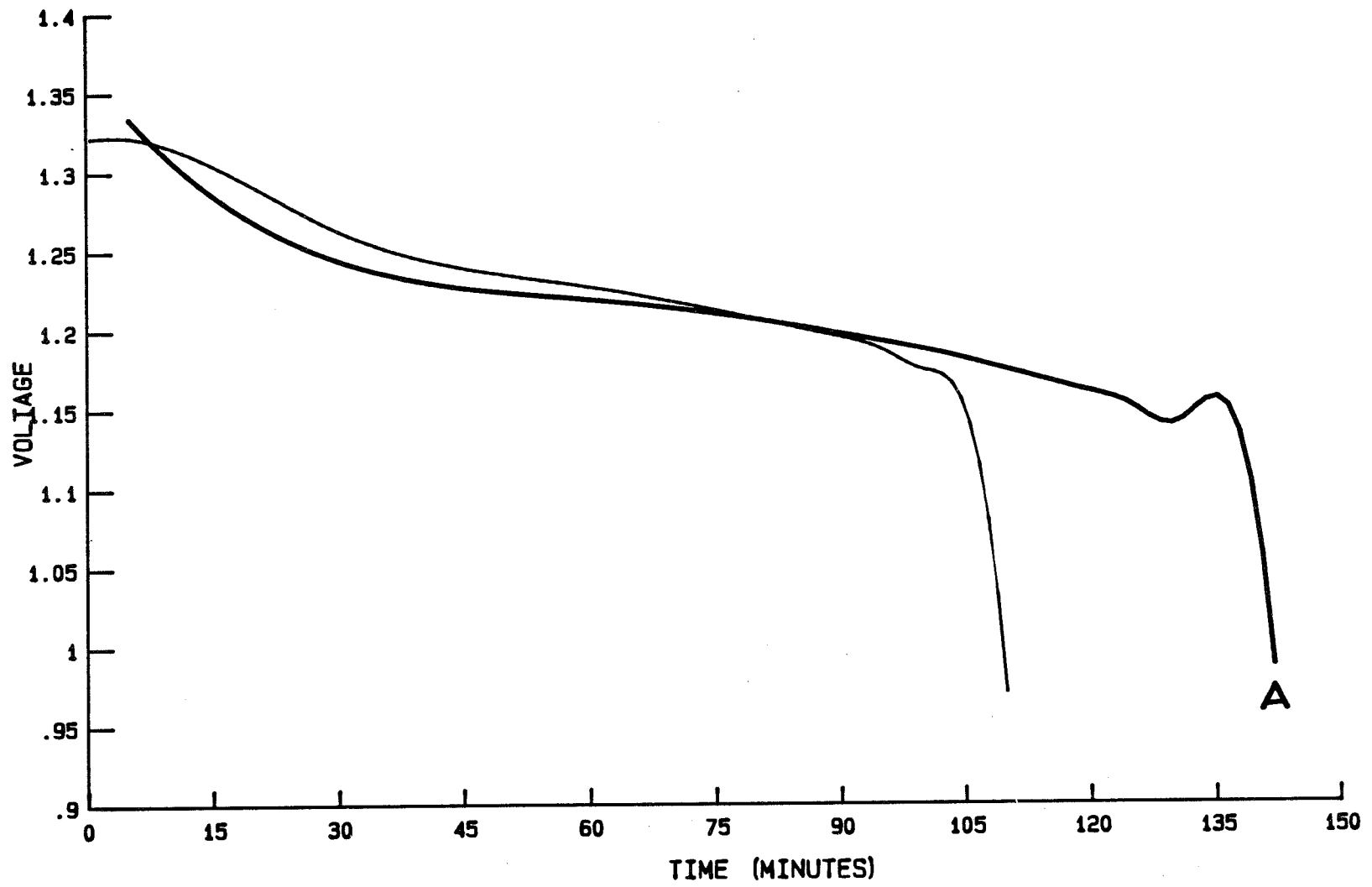
Figure 10. 30 Degree Discharge
