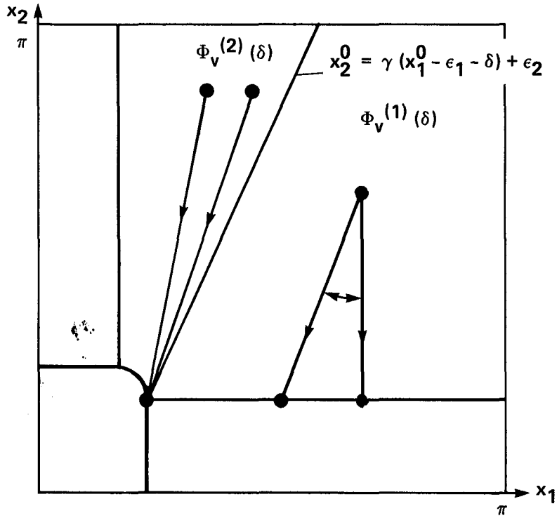
(c) \gamma > 1 .
