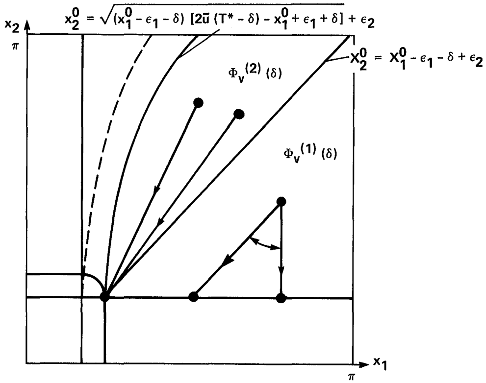
(b) \gamma = 1 .
