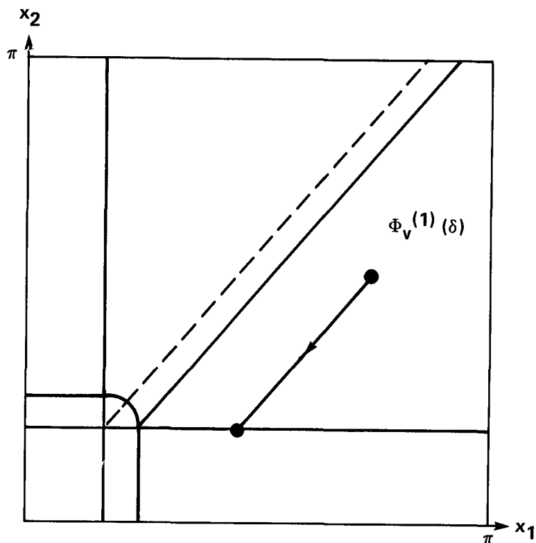
(b) \gamma_1 = 1 .
