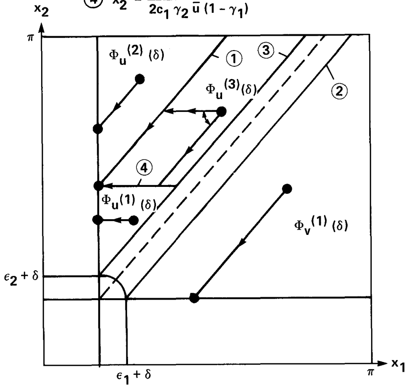
(a) \gamma_1 < 1 .
