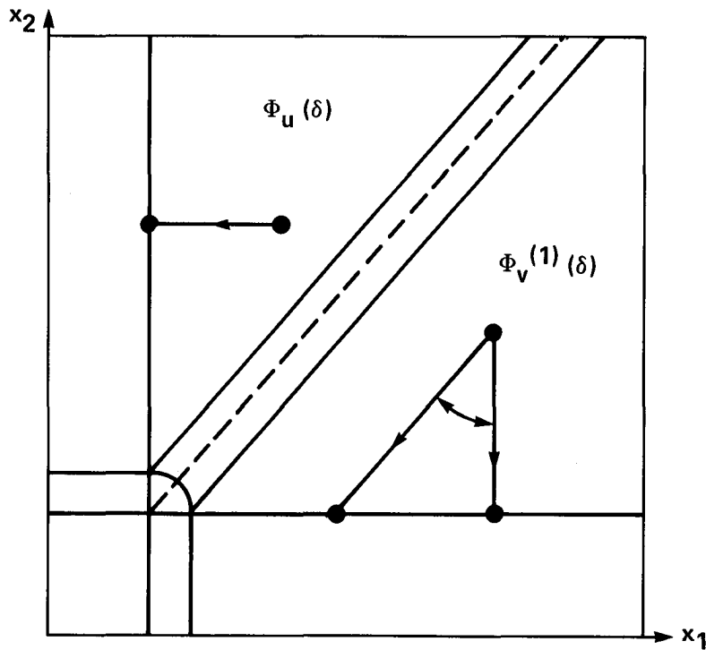
(a) \gamma_1 < 1 .
