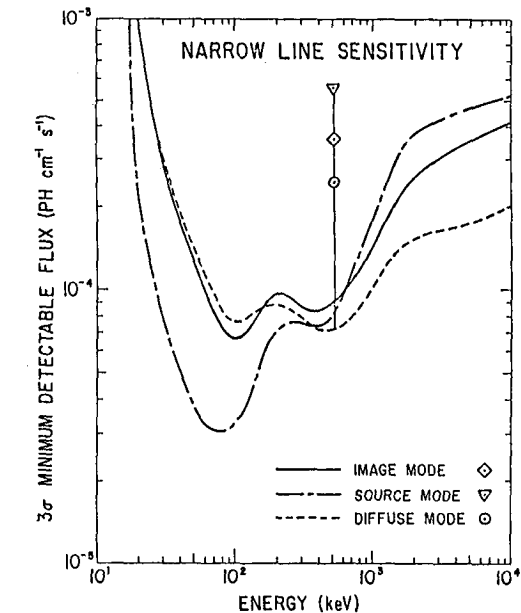
Figure 3. The sensitivity to narrow lines is shown for a 6 hour balloon observation. The increase below \sim 50 keV is primarily due to decreasing atmospheric transmission. Differences among the observing modes are due to different backgrounds and source modulation efficiencies. Carried in space with a 10 cm BGO shield, this instrument could achieve an Image Mode sensitivity of 10^{-5} ph/cm 2 -sec over most of its energy range in a 7-day observation.
