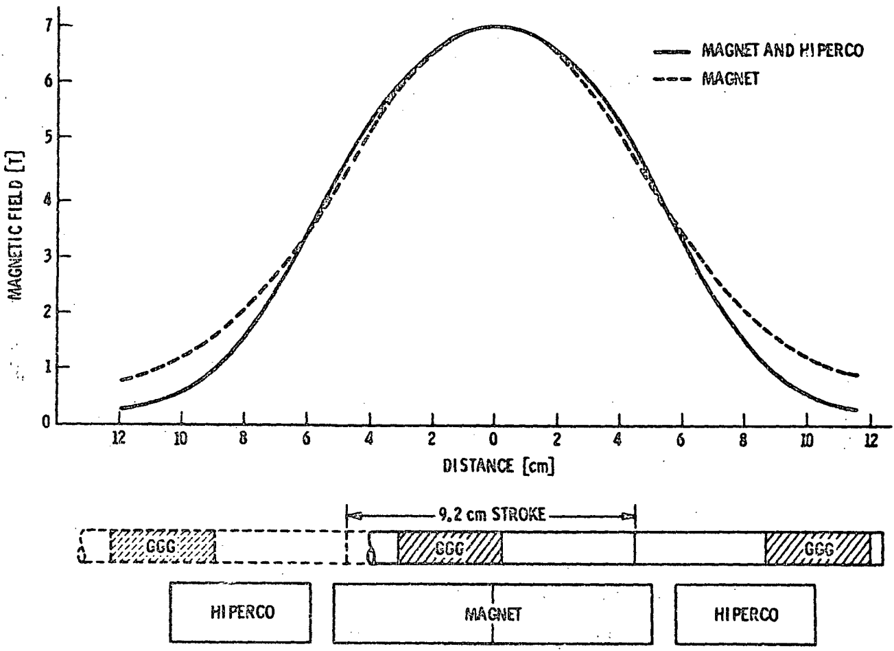
Fig. 4 Comparison of the measured axial magnetic field profiles with and without the Hiperc material. The extreme positions of the piston are shown with respect to the field profiles.
