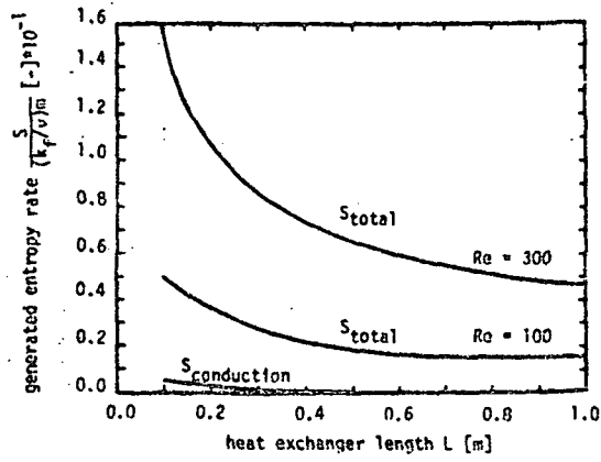
Figure 2: Entropy generation rate vs. length of heat-exchanger for two Reynolds numbers ( T_1 = 300 K, T_2 = 60 K, p_L = 2 bar, p_H = 20 bar) ( m^1 = 0.1 g/s, t = 0.2 mm)
