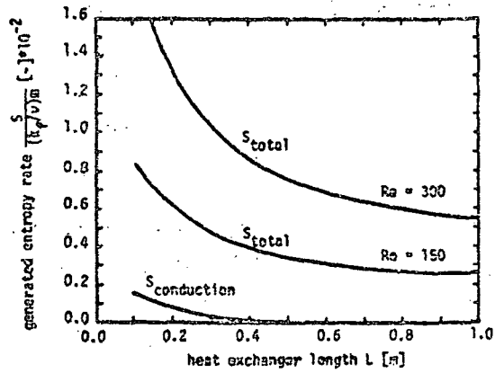
Figure 3: Entropy generation rate vs. length of heat exchanger parameter: Reynolds number Re ( T_1 = 30 K, T_2 = 14 K, p_L = 2 bar, p_H = 20 bar) ( m^1 = 0.085 g/s, t = 0.2 mm)
