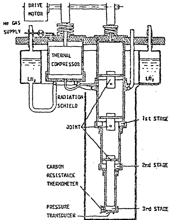
Fig.1. Schematic diagram of three-stage VM cooler
