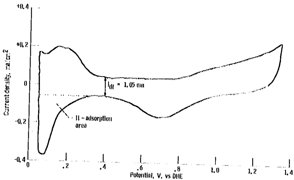
Figure 1. - Cyclic voltammogram of electrode 5, 0.5 \text{ mg}/\text{cm}^2 Pt on carbon paper in \text{H}_2\text{SO}_4 , 25^\circ\text{C} , 5 \text{ mV}/\text{s} scan.
