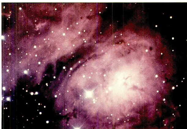
Figure 33. Interstellar Medium
