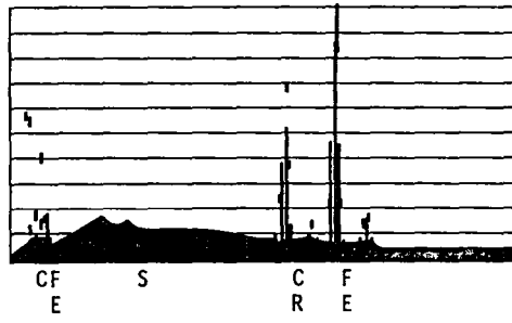
Figure 6. - EDX analysis of outer race.
