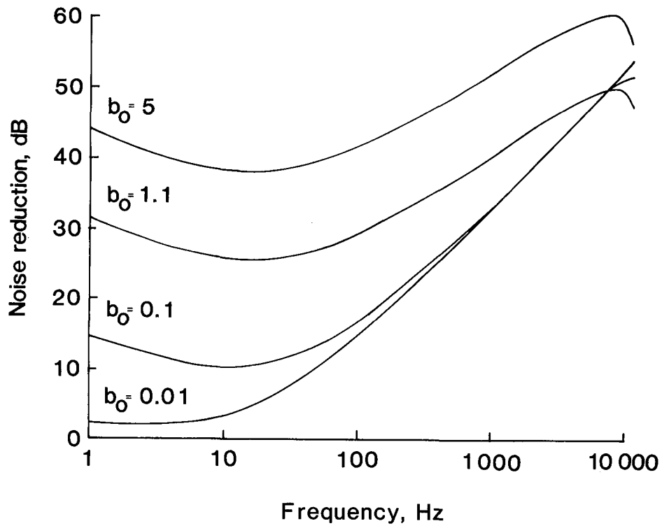
Figure 11.- Variation of calculated noise reduction with nondimensional source-plate parameter. b_o = b/k_0 ; k_0 = 2\pi/\lambda_p = \sqrt{m\omega^2/D} .
