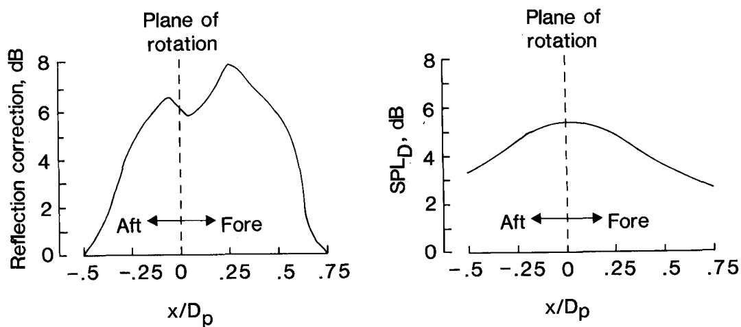
(b) Predicted curve using equation (20).
