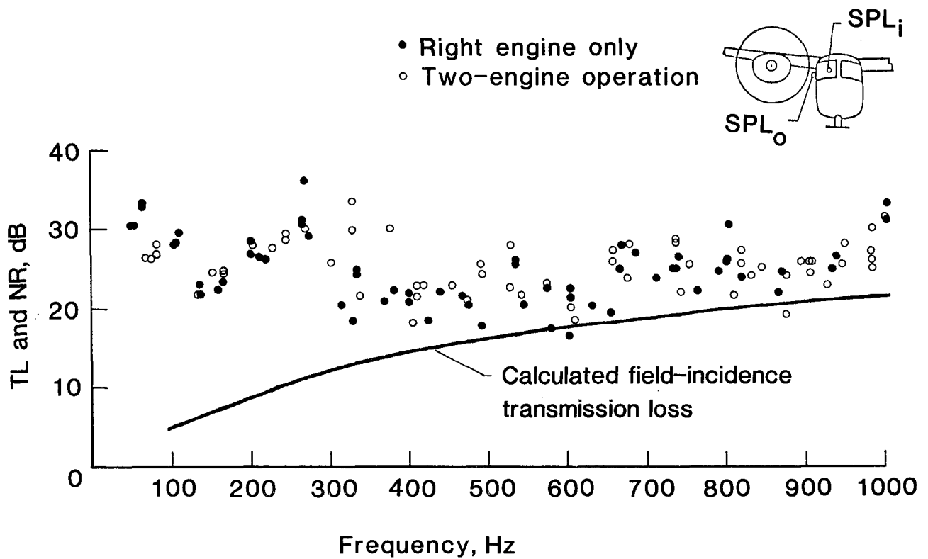
Figure 1.- Noise transmission from propeller tests and infinite panel theory.
