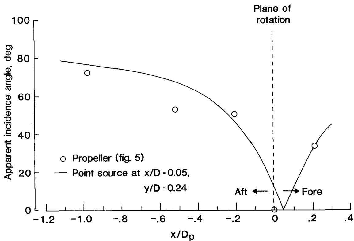
Figure 6.- Apparent incidence directions. \theta = \tan^{-1}(x/D) .
