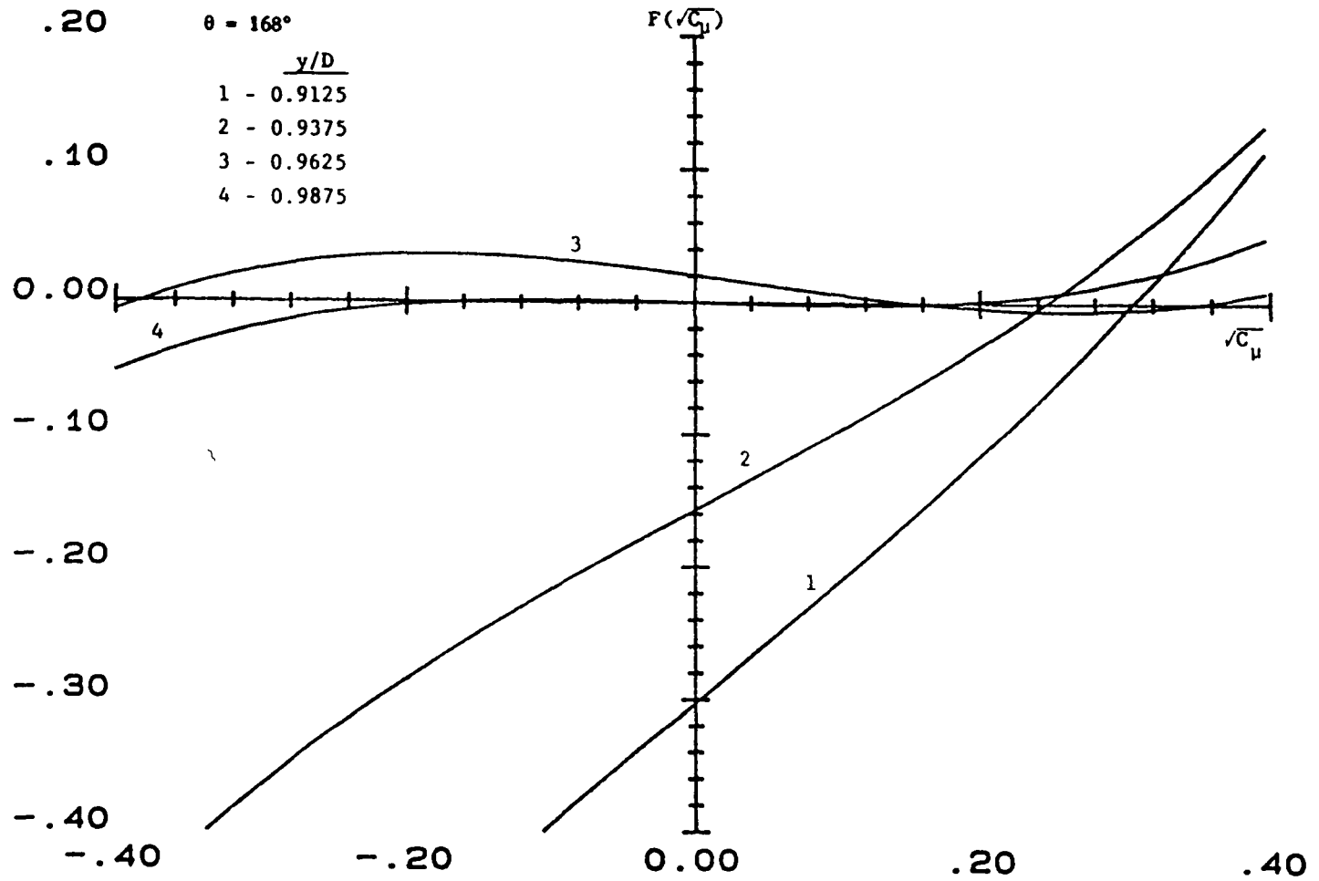
Figure 13. Behavior of F(\sqrt{C_\mu}) polynomial at various cross stream locations for \theta=168^\circ : Analysis 3.
