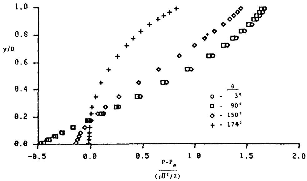
Figure 8. Pressure profiles for simple TAD geometry with FDP flow inlet: Analysis 2.
