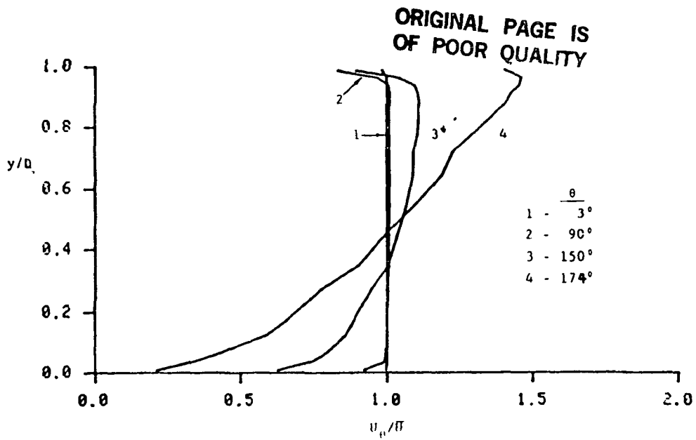
Figure 4 Streamwise velocity profiles for simple TAD geometry with plug flow inlet: Analysis 1
