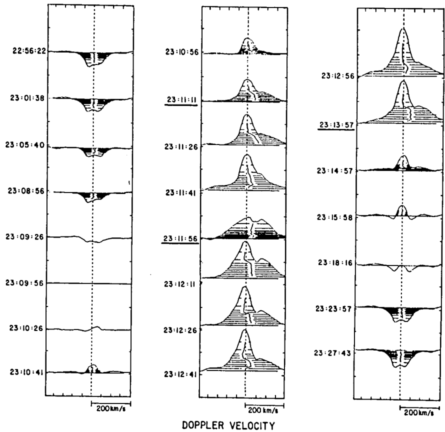
Figure 5. The relationship between (top) the hard X-ray count rate measured by the SMM Hard X-Ray Burst Spectrometer and (bottom) the H\alpha spectral excess (relative to its pre-impulsive H\alpha spectrum) and Doppler shift of one of the H\alpha kernel pixels of the flare of 2312, UT 23 June 1980. In difference spectra of sufficient amplitude a bisector is drawn at various intensity levels indicated by horizontal striations, centered within the most intense spectral feature. Both the hard X-ray count rate and the H\alpha Doppler shift show several episodes, whose occurrence is indicated by vertical bars (top panel) and underlined times of observation (bottom panel). From Canfield, Gunkler, and Kiplinger (1985).
