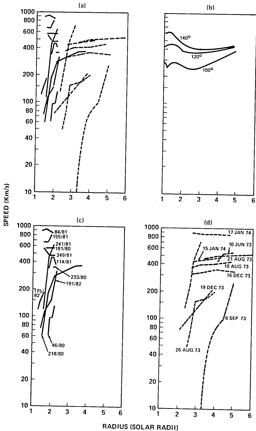
Figure 1. (a) Radial speed of transients, including measurements from the Mauna Loa K-coronameter, Skylab coronagraph, and the SMM coronagraph/polarimeter. (From MacQueen and Fisher, 1983.) (b) Sum of flow speed and fast-mode speed for three positions in and near an MHD model coronal streamer. (From Steinolfson, Suess, and Wu, 1982.) (c) Data from panel (a) that were taken only with the Mauna Loa K-coronameter, with the date the observations were made. (d) Data from panel (a) that were taken only from the Skylab coronagraph and SMM coronagraph/polarimeter, with the date the observations were made.
