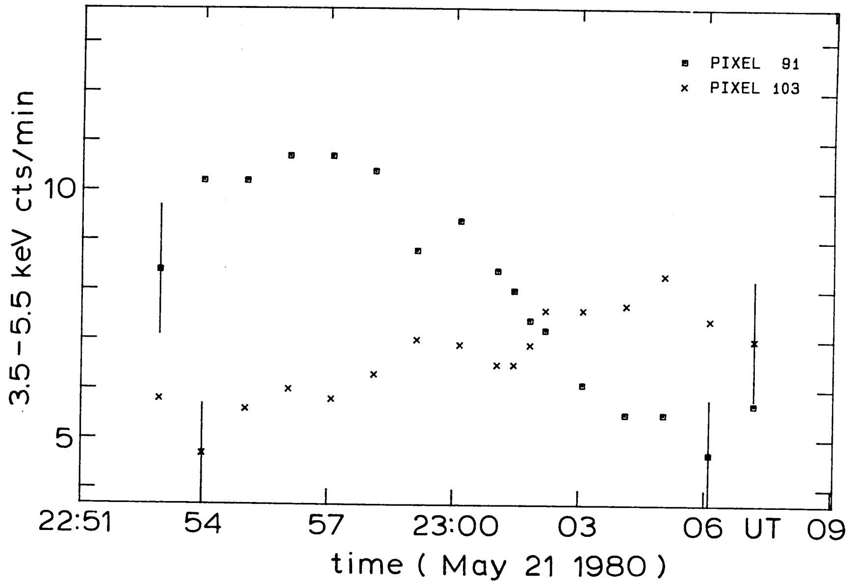
Figure 6. Count rates versus time for the two pixels 91 and 103 (maxima in Figure 5) around the time of their maximum brightness.
