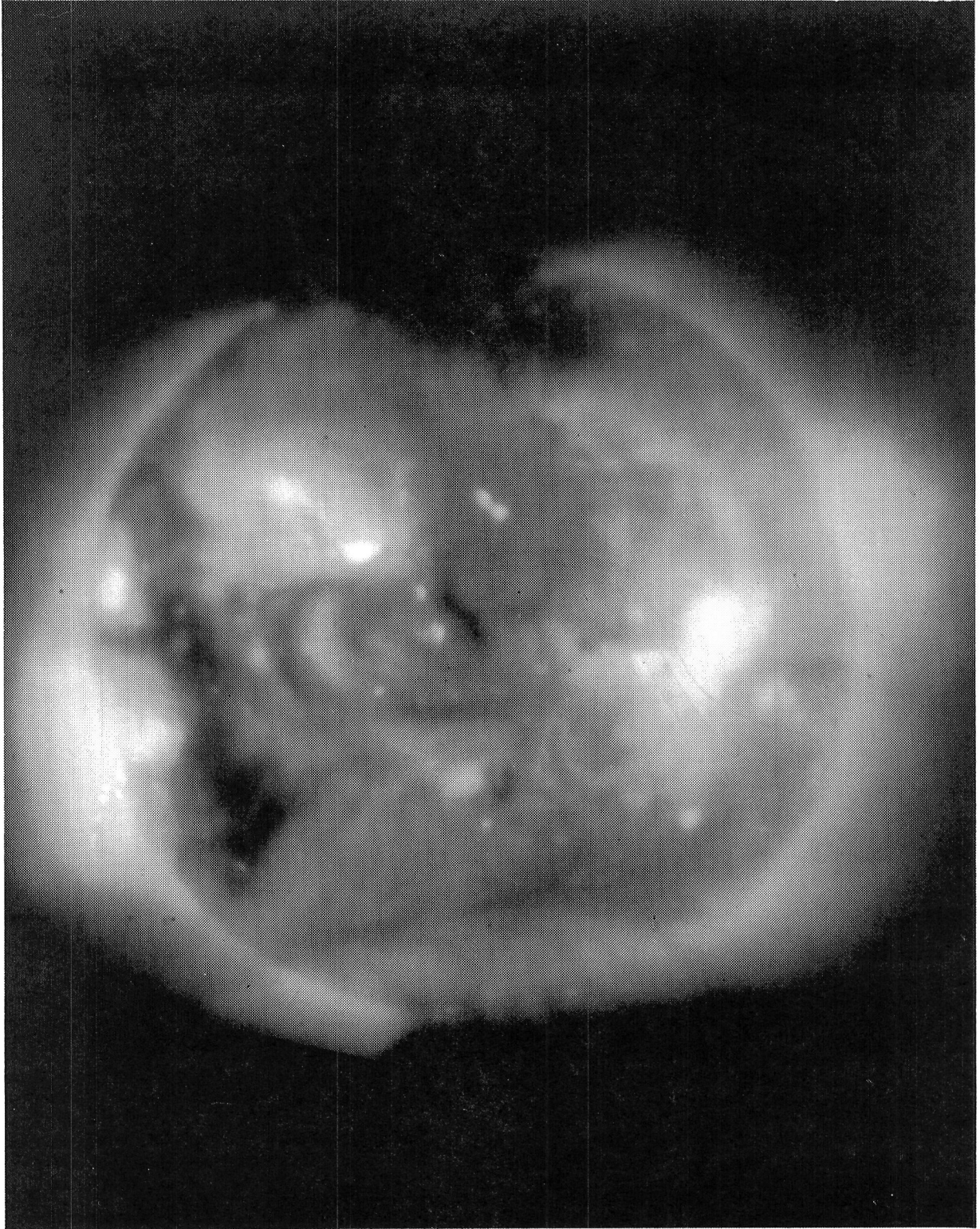
Figure 5. X-ray photograph of the solar corona acquired during Skylab (courtesy American Science and Engineering and Harvard College Observatory). Coronal holes are visible as dark areas at the north (upper) pole and near the east (left) limb.
