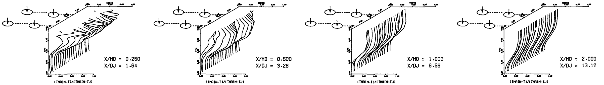
MEASURED THETA PROFILES FOR TEST NO. 10, TEST SECTION I, PLATE M5 , J = 6.72 , S/D = 2.83 , H/D = 5.66
