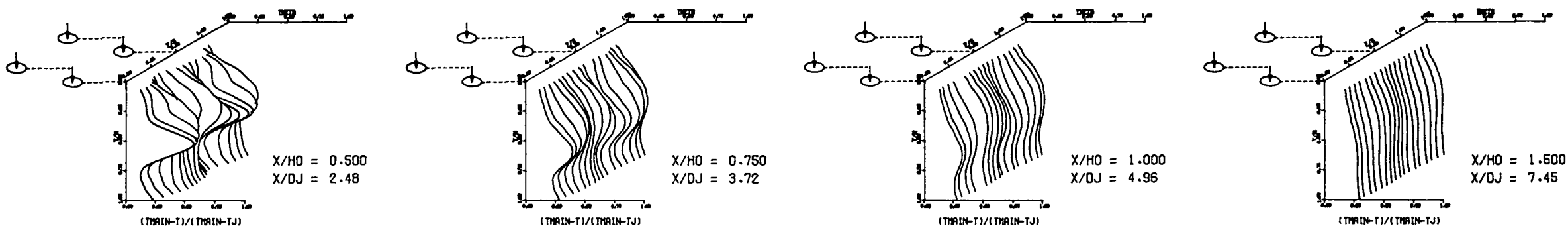
MEASURED THETA PROFILES FOR TEST NO. 9, TEST SECTION I, PLATE M4(STG) , J = 26.77 , S/D = 4.00 , H/D = 4.00
