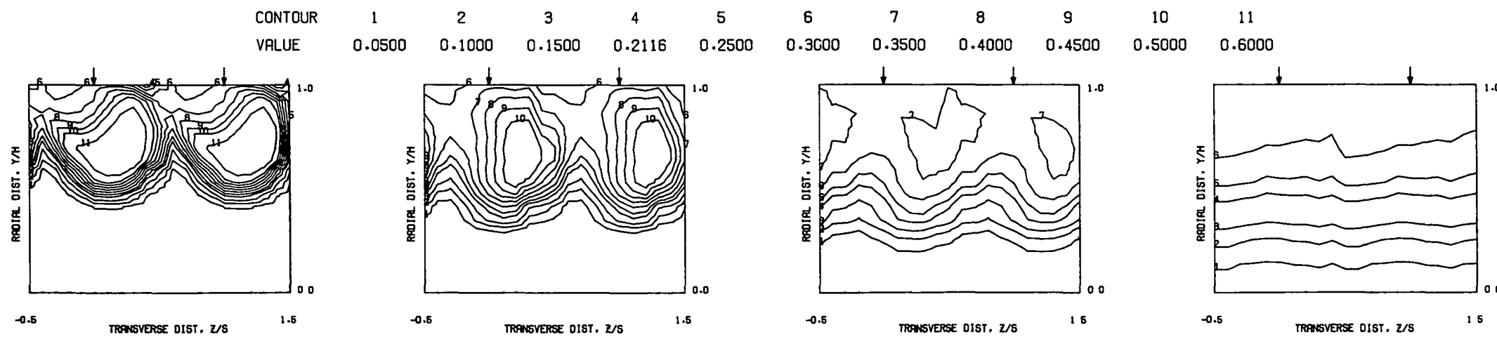
MEASURED THETA CONTOURS FOR TEST NO 18, 45-DEG SLOT, J=6.64, S/D=2.00, H/D=4.00
