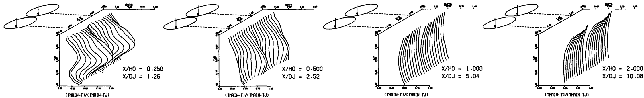
MEASURED THETA PROFILES FOR TEST NO 20, TEST SECTION I, 45-DEG SLOT , J = 106.18 , S/D = 2.00 , H/D = 4.00
