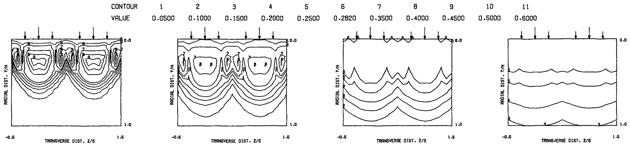
PREDICTED THETA CONTOURS FOR TEST NO 13, PLATE M5, J1=26.4, J2=6.4, S/D=2.0, H/D=4.0
