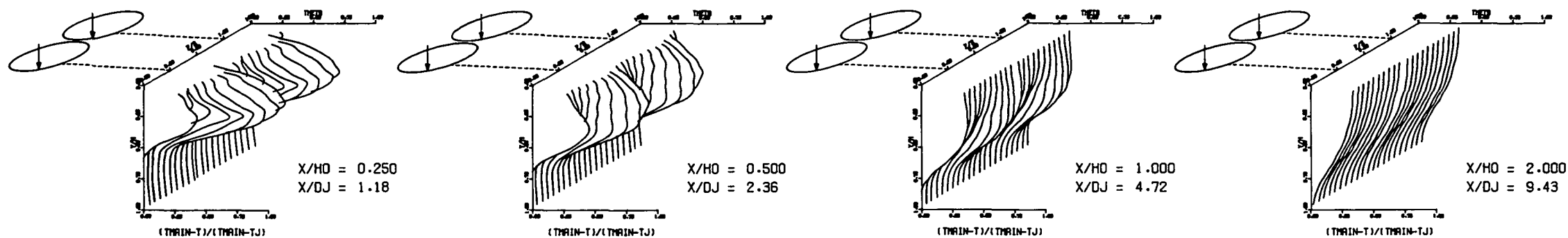
MEASURED THETA PROFILES FOR TEST NO 18, TEST SECTION I, 45-DEG SLOT , J = 6.64 , S/D = 2.00 , H/D = 4.00
