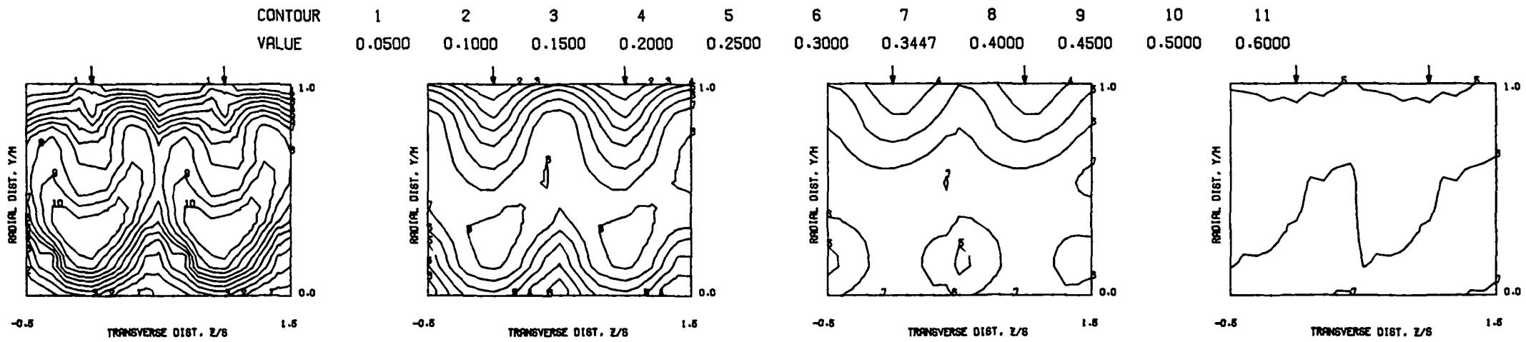
MEASURED THETA CONTOURS FOR TEST NO 2, S.L. SLOTS, J=26.47, S/D=2.00, H/D=4.00
