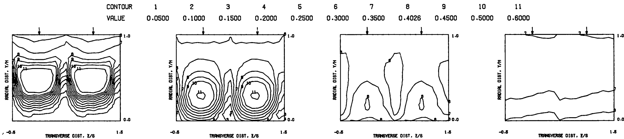
MEASURED THETA CONTOURS FOR TEST NO 3, BLUFF SLOTS, J=26.59, S/D=2.00, H/D=4.00
