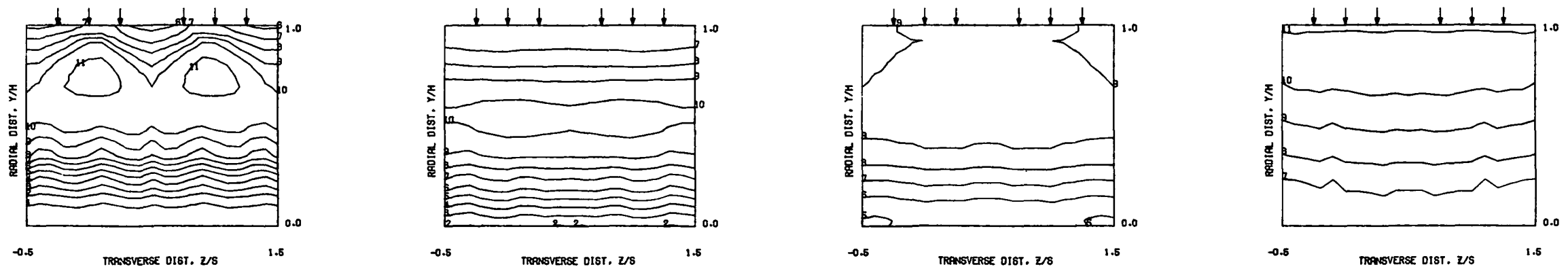
MEASURED THETA CONTOURS FOR TEST NO 16, PLATE M6, J1=106, J2=6, S/D=2.83, H/D=5.66
