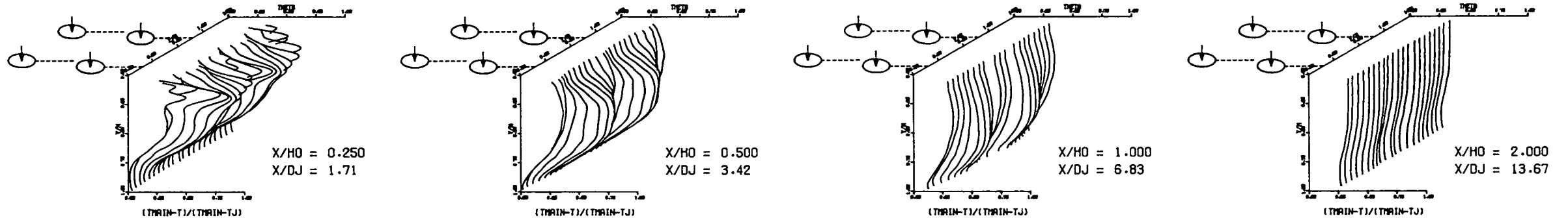
MEASURED THETA PROFILES FOR TEST NO. 11, TEST SECTION 1, PLATE M5 , J = 26.79 , S/D = 2.83 , H/D = 5.66
