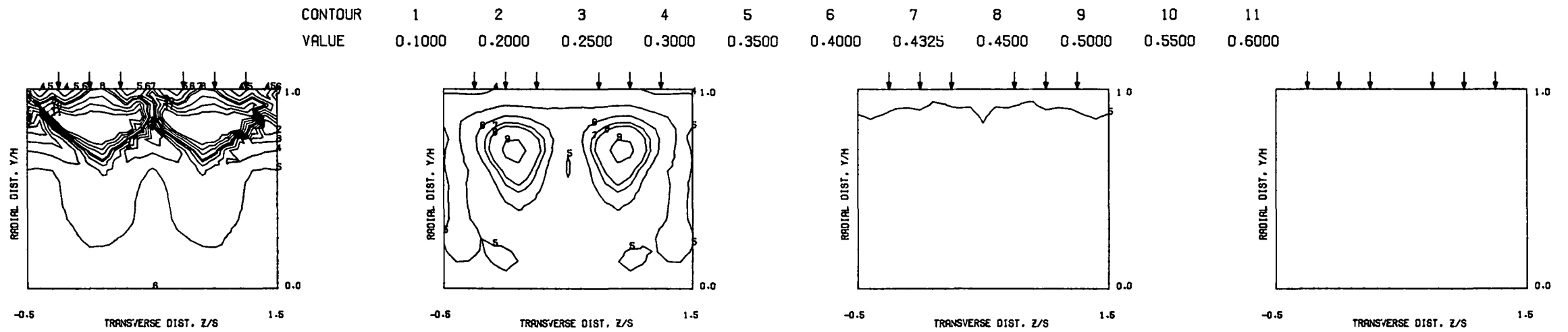
MEASURED THETA CONTOURS FOR TEST NO 15, PLATE M5, J1=106, J2=26, S/D=2.83, H/D=5.66
