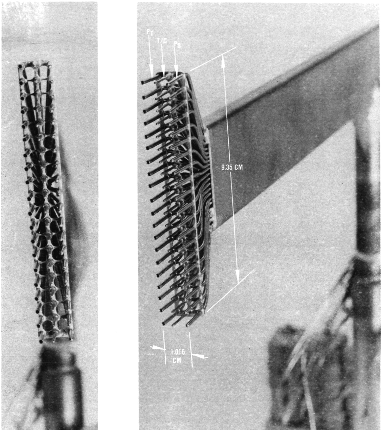
Figure 5. Total Pressure, Thermocouple, and Static Pressure Rake.
