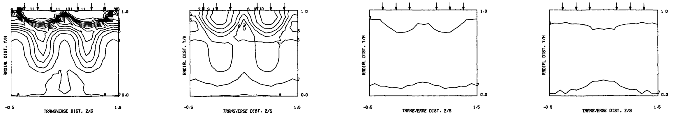
MEASURED THETA CONTOURS FOR TEST NO 14, PLATE M5, J1=106 , J2=6.5, S/D=2.83, H/D=5.66
