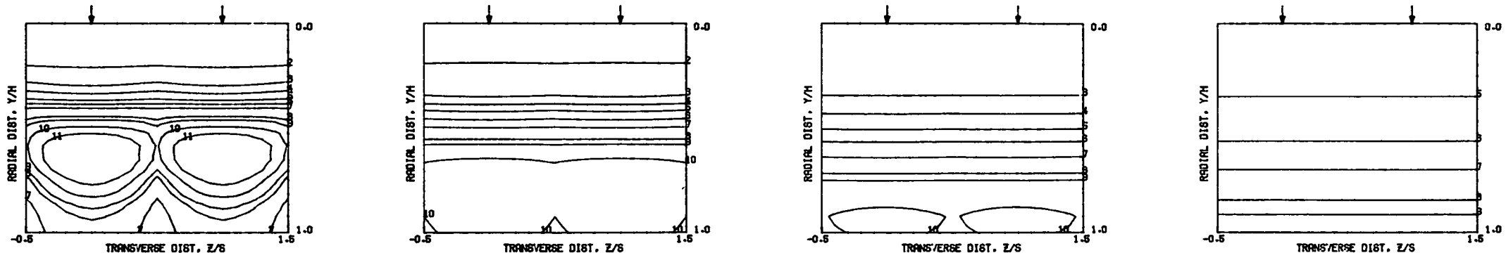
PREDICTED THETA CONTOURS FOR TEST NO. 4, BLUFF SLOT, J=106.5 , S/D=2.00 , H/D=4.00
