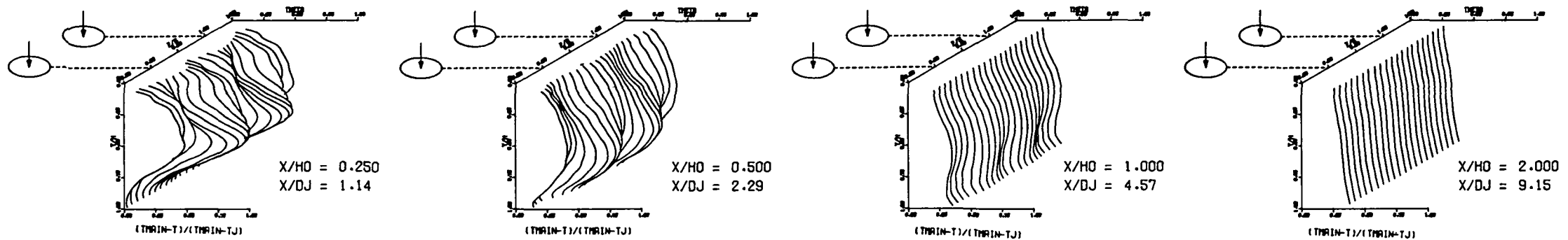
MEASURED THETA PROFILES FOR TEST NO 22, TEST SECTION I, TM=CONST, J = 26.24, S/D = 2.00, H/D = 4.00
