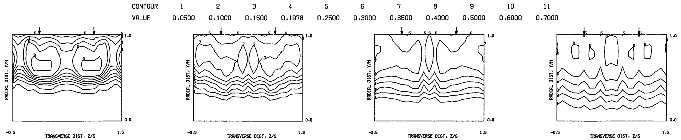
MEASURED THETA CONTOURS FOR TEST NO 5, PLATE M3, J=6.65, S/D=2.83, H/D=5.66
