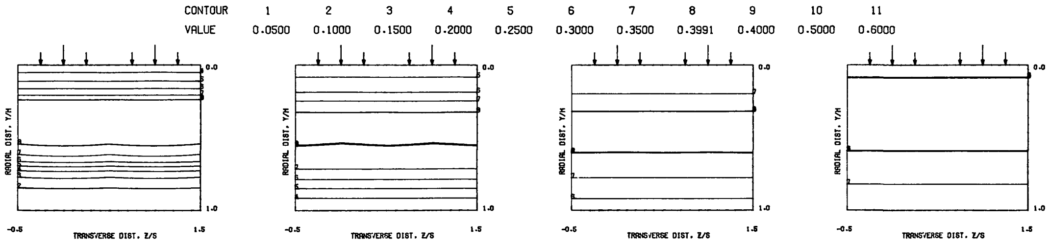
PREDICTED THETA CONTOURS FOR TEST NO 16, PLATE M6, J1=106, J2=6, S/D=2.0, H/D=8.0
