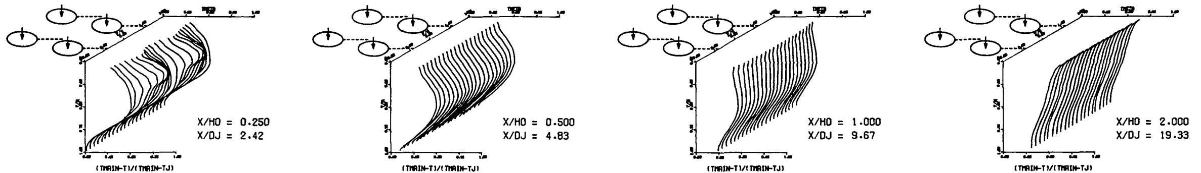
MEASURED THETA PROFILES FOR TEST NO 16, TEST SECTION I, PLATE M6
