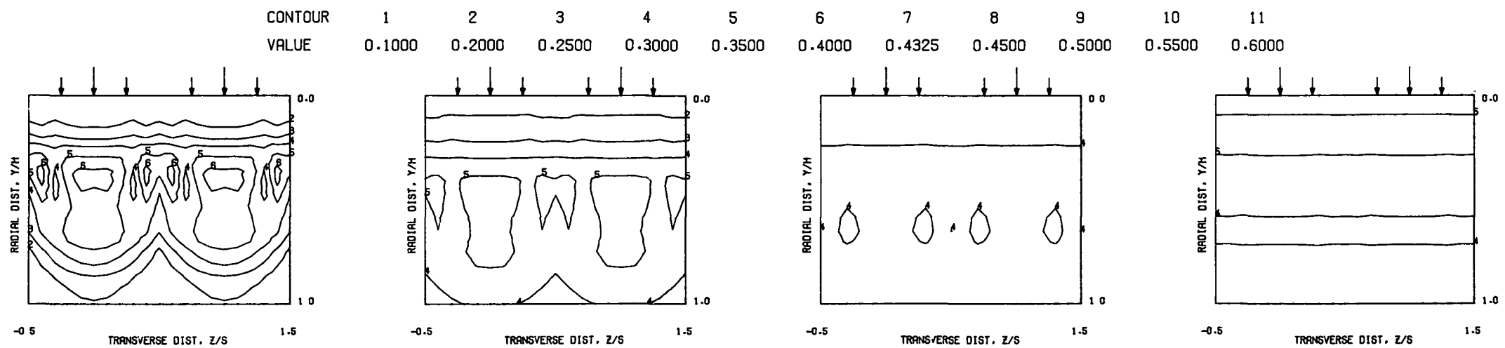
PREDICTED THETA CONTOURS FOR TEST NO 15, PLATE M5, J1=106, J2=26, S/D=2.0, H/D=4.0
