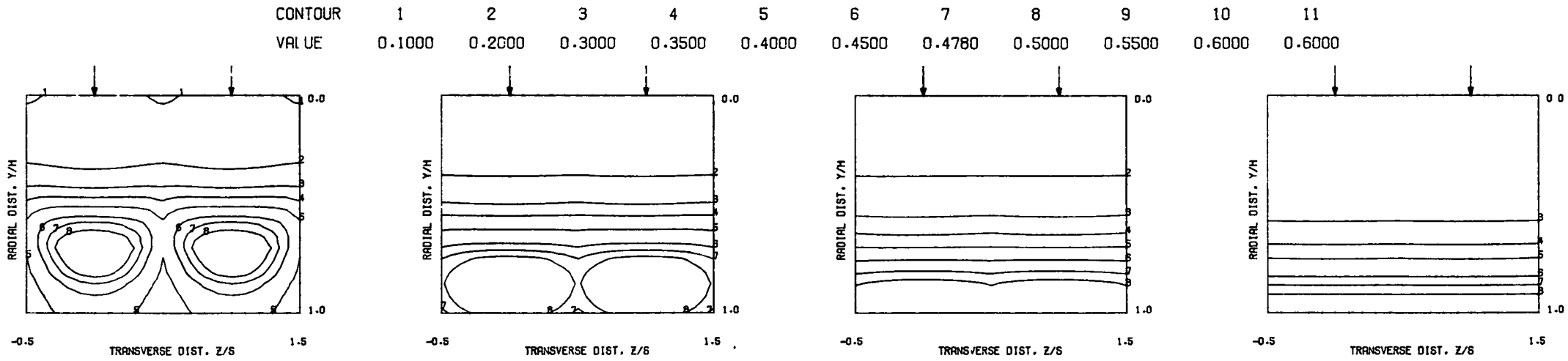
PREDICTED THETA CONTOURS FOR TEST NO. 7, PLATE M3, J=107.2, S/D=2.83, H/D=5.66
