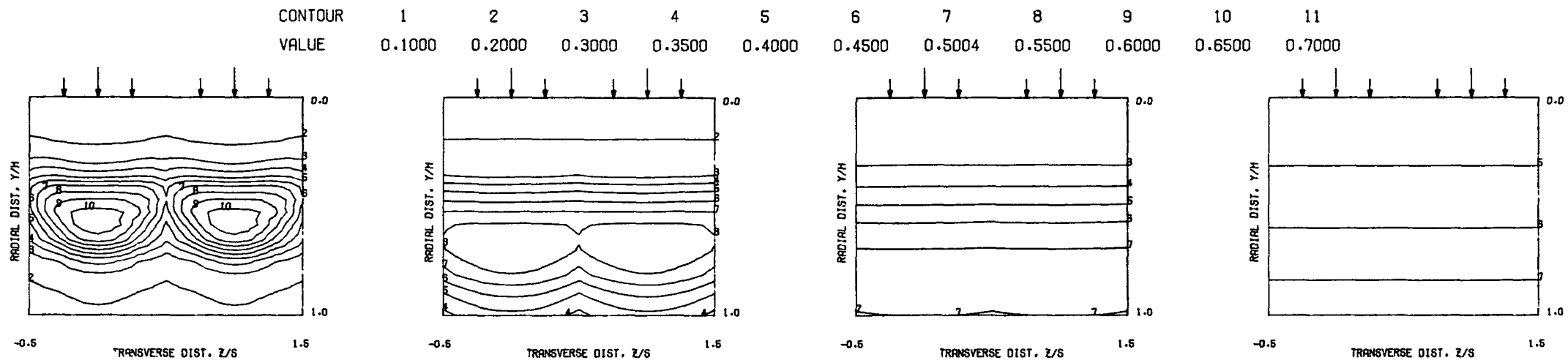
PREDICTED THETA CONTOURS FOR TEST NO. 12, PLATE M5, J=106.3, S/D=2.83, H/D=5.66
