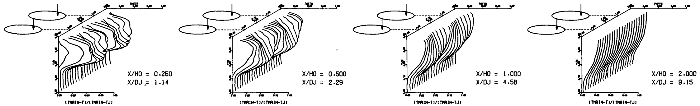
MEASURED THETA PROFILES FOR TEST NO 1, TEST SECTION I, STREAMLINED SLOTS, J = 6.60, S/D = 2.00, H/D = 4.00
