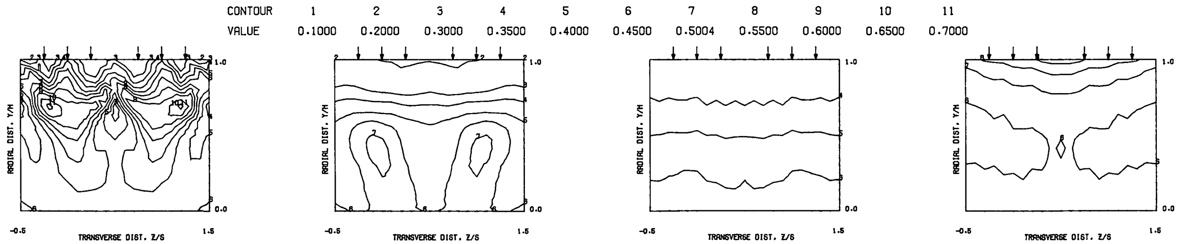
MEASURED THETA CONTOURS FOR TEST NO 12, PLATE M5, J=106.3, S/D=2.83, H/D=5.66
