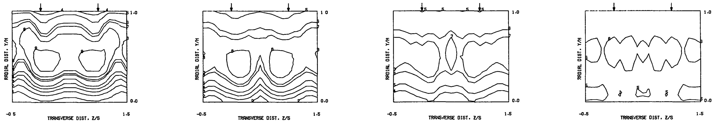
MEASURED THETA CONTOURS FOR TEST NO 6, PLATE M3, J=26.27, S/D=2.83, H/D=5.66
