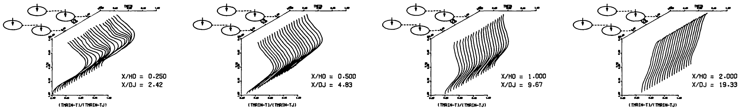
MEASURED THETA PROFILES FOR TEST NO 17, TEST SECTION I, PLATE M6
