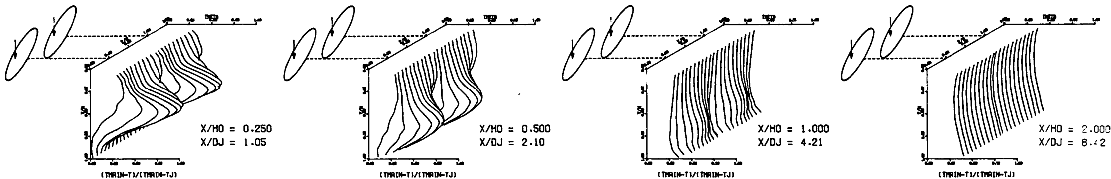
MEASURED THETA PROFILES FOR TEST NO 3, TEST SECTION I, BLUFF SLOTS , J = 26.59 , S/D = 2.00 , H/D = 4.00
