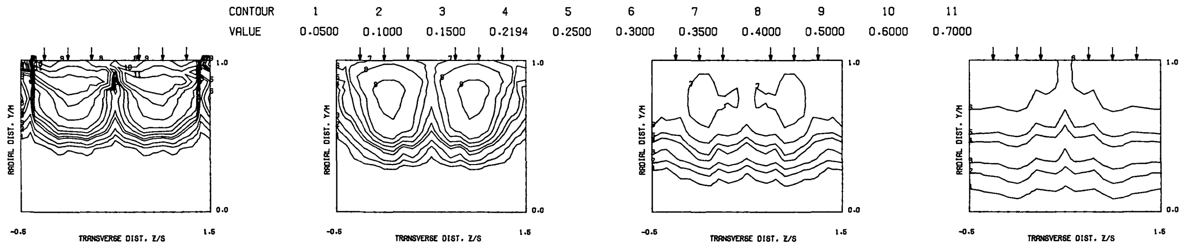
MEASURED THETA CONTOURS FOR TEST NO 10, PLATE M5, J=6.72, S/D=2.83, H/D=5.66
