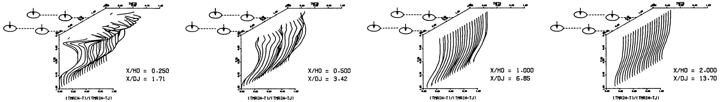
MEASURED THETA PROFILES FOR TEST NO 13, TEST SECTION I, PLATE M5(INL) , J = 26.20 , S/D = 2.83 , H/D = 5.66
