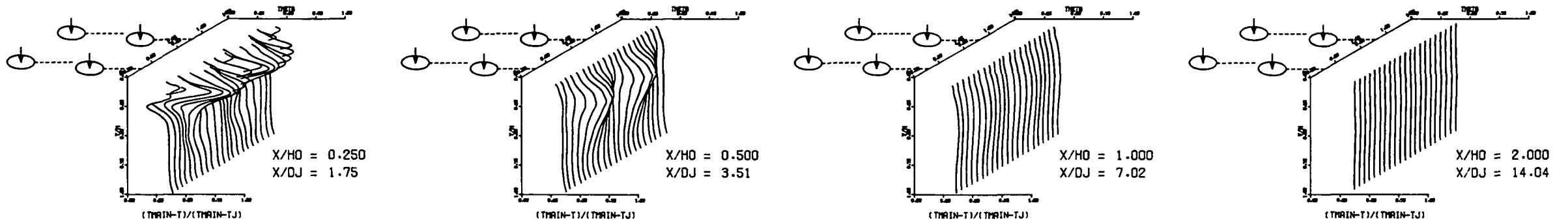
MEASURED THETA PROFILES FOR TEST NO 15, TEST SECTION I, PLATE M5(INL) , J = 106.29 , S/D = 2.83 , H/D = 5.66
