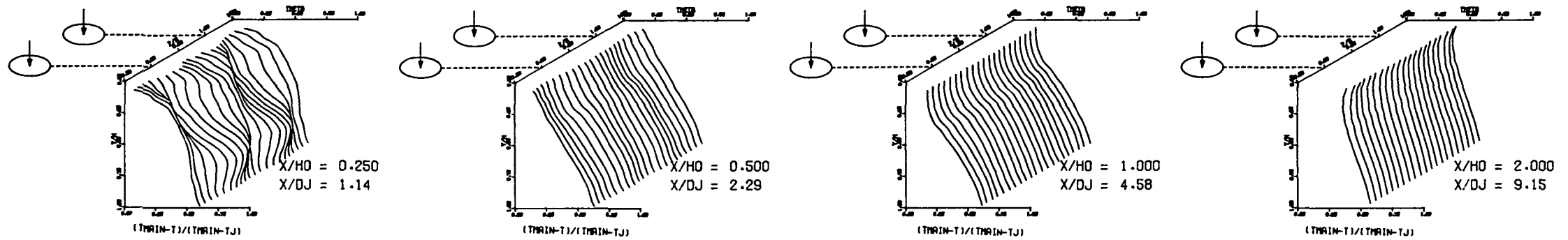
MEASURED THETA PROFILES FOR TEST NO 21, TEST SECTION I, TM=CONST, J = 103.19, S/D = 2.00, H/D = 4.00
