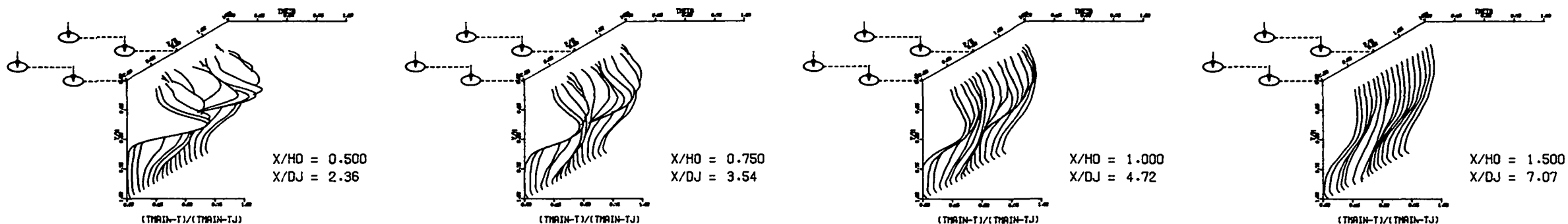
MEASURED THETA PROFILES FOR TEST NO. 8, TEST SECTION I, PLATE M4 (STG), J = 6.67, S/D = 4.00, H/D = 4.00
