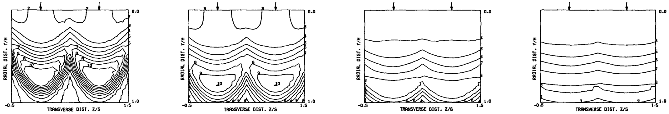
PREDICTED THETA CONTOURS FOR TEST NO. 2, S.L.SLOT, J=26.47, S/D=2.00, H/D=4.00
