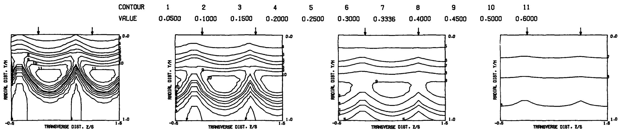
PREDICTED THETA CONTOURS FOR TEST NO 19, PLATE M-7, J=27.13, S/D=2.00, H/D=4.00
