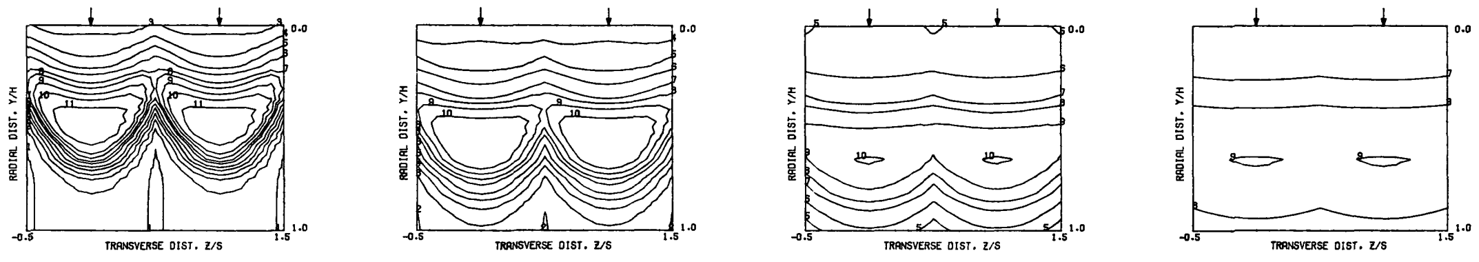
PREDICTED THETA CONTOURS FOR TEST NO 22, TM=CONST, J=26.24, S/D=2.00, H/D=4.00
