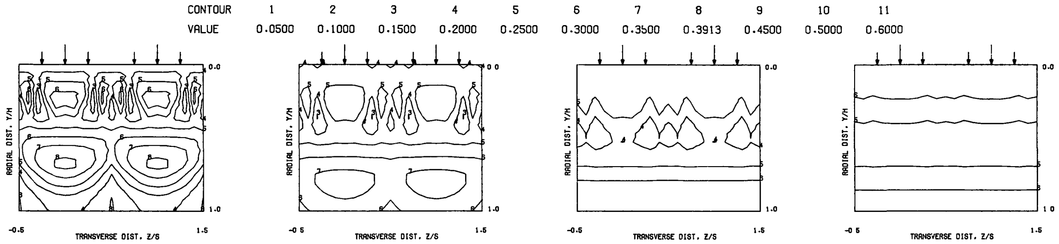
PREDICTED THETA CONTOURS FOR TEST NO 14, PLATE M5, J1=106, J2=6.4, S/D=2.0, H/D=4.0
