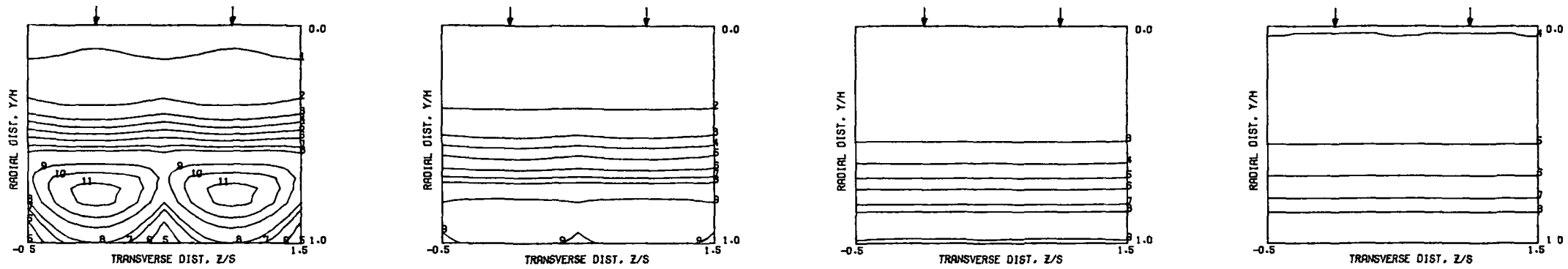
PREDICTED THETA CONTOURS FOR TEST NO 21, T_M=CONST , J=103.2 , S/D=2.00 , H/D=4.00
