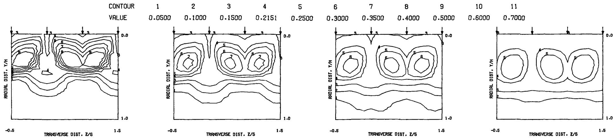
PREDICTED THETA CONTOURS FOR TEST NO. 8, PLATE M4, J=6.67 , S/D=4.00 , H/D=4.00
