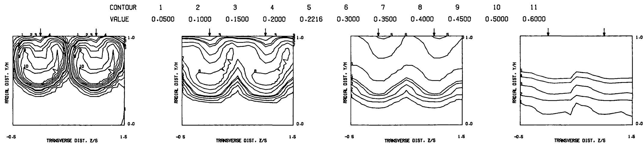
MEASURED THETA CONTOURS FOR TEST NO 1, S.L. SLOTS, J=6.60, S/D=2.00, H/D=4.00
