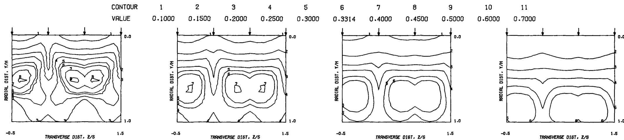
PREDICTED THETA CONTOURS FOR TEST NO. 9. PLATE M4, J=26.77 , S/D=4.00 , H/D=4.00
