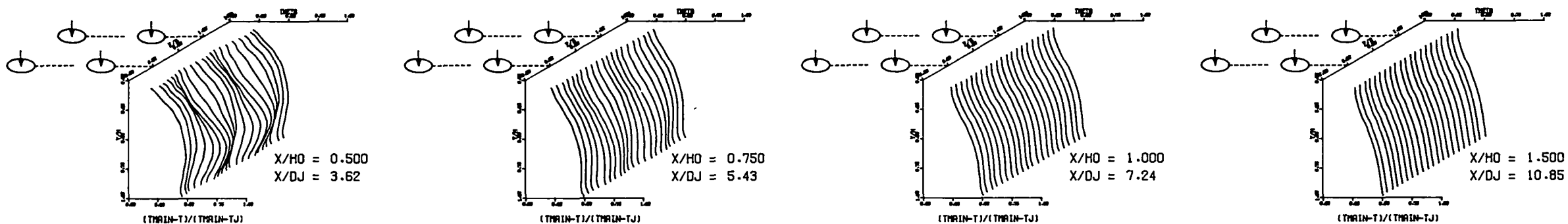
MEASURED THETA PROFILES FOR TEST NO. 7, TEST SECTION I, PLATE M3 (INL), J = 107.18, S/D = 2.83, H/D = 5.66
