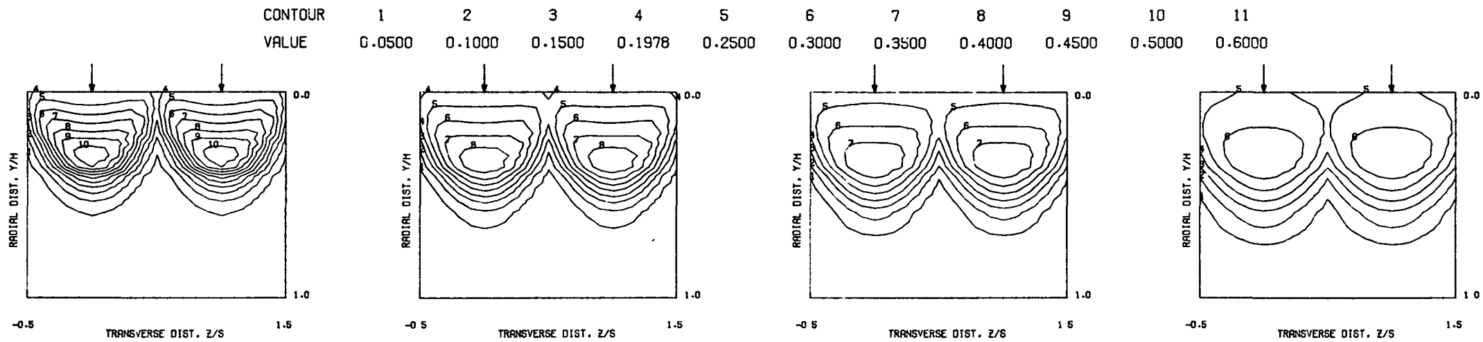
PREDICTED THETA CONTOURS FOR TEST NO. 5, PLATE M3, J=6.65 , S/D=2.83 , H/D=5.66
