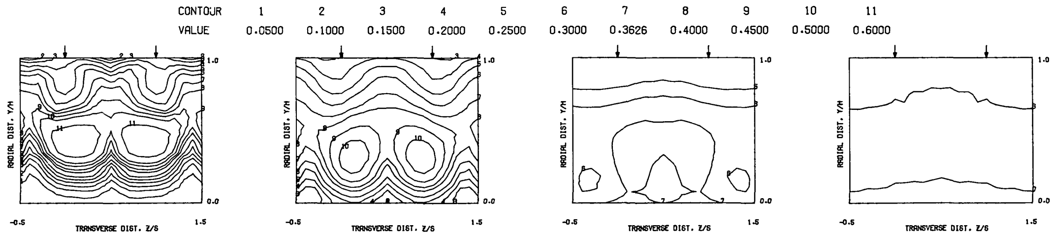
MEASURED THETA CONTOURS FOR TEST NO 22, TM=CONST, J=26.24, S/D=2.00, H/D=4.00
