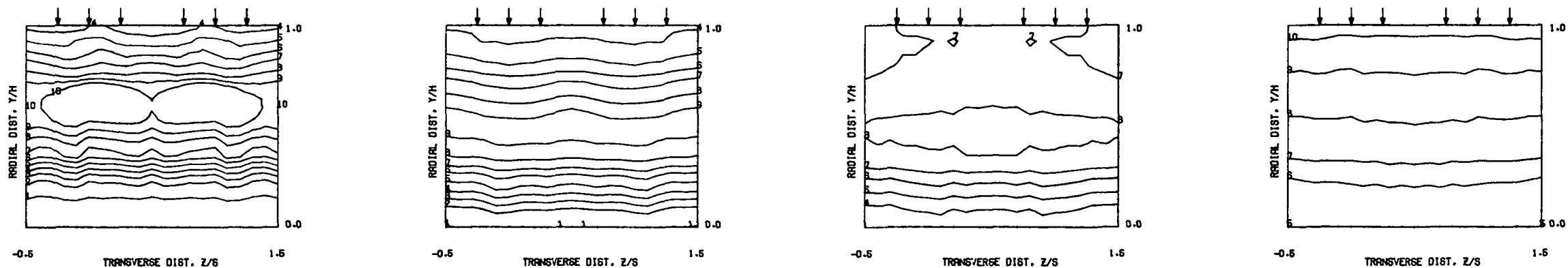
MEASURED THETA CONTOURS FOR TEST NO 17, PLATE M6, J1=106, J2=26, S/D=2.83, H/D=5.66
