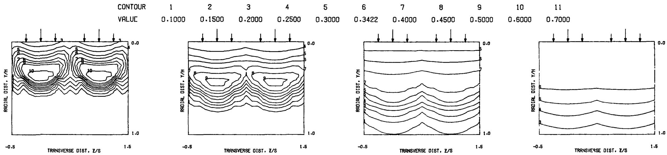
PREDICTED THETA CONTOURS FOR TEST NO. 11, PLATE M5, J=26.79, S/D=2.83, H/D=5.66
