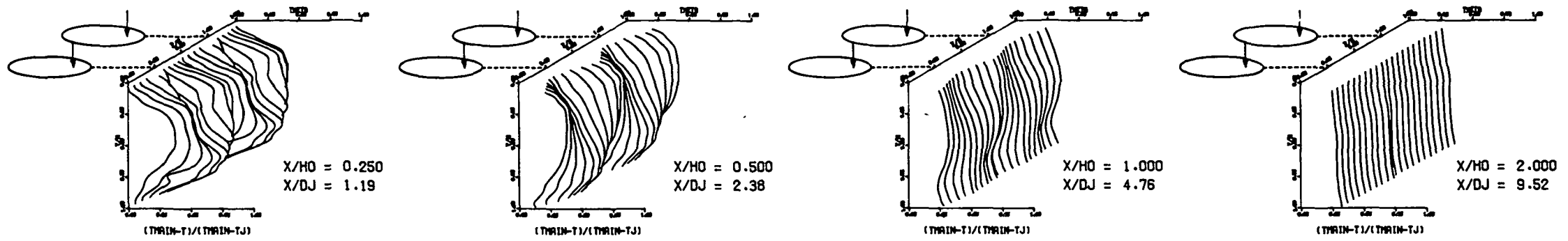
MEASURED THETA PROFILES FOR TEST NO 2, TEST SECTION I, STREAMLINED SLOTS, J = 26.47, S/D = 2.00, H/D = 4.00
