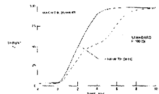
DEEC/F-15 FAST ACCEL CAPABILITY COMPARISON OF THRUST RESPONSE FOR AN IDLE-TO-MAXIMUM POWER THROTTLE SNAP
