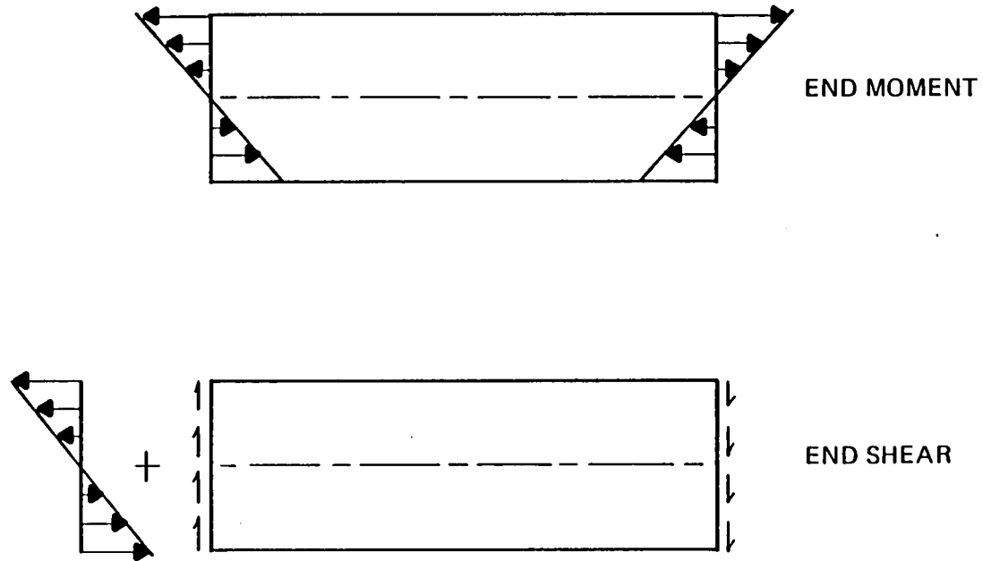
FIG. 3 BEAM LOADS
