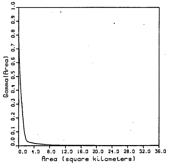
Variance Function
