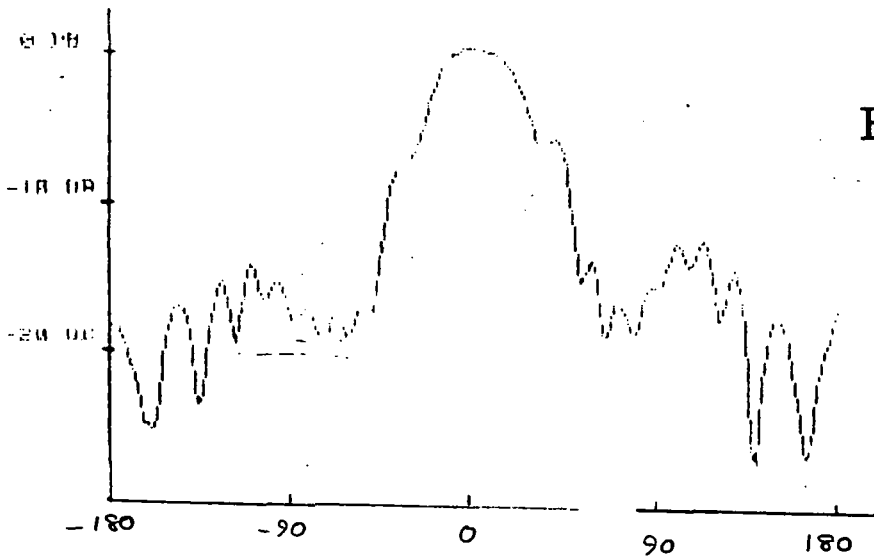
RECTANGULAR POWER PATTERN IN dB
