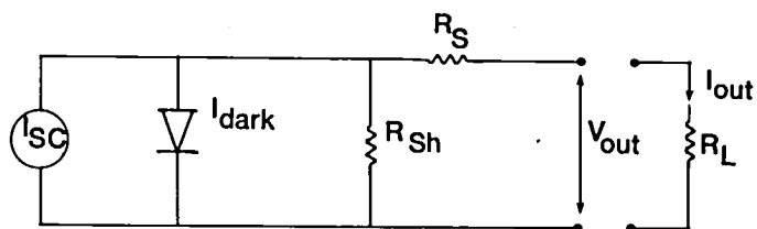
Figure 3 - Equivalent circuit
