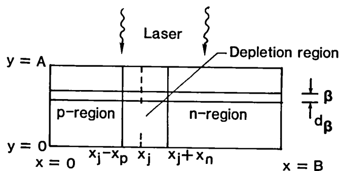
Figure 2 - Converter geometry
