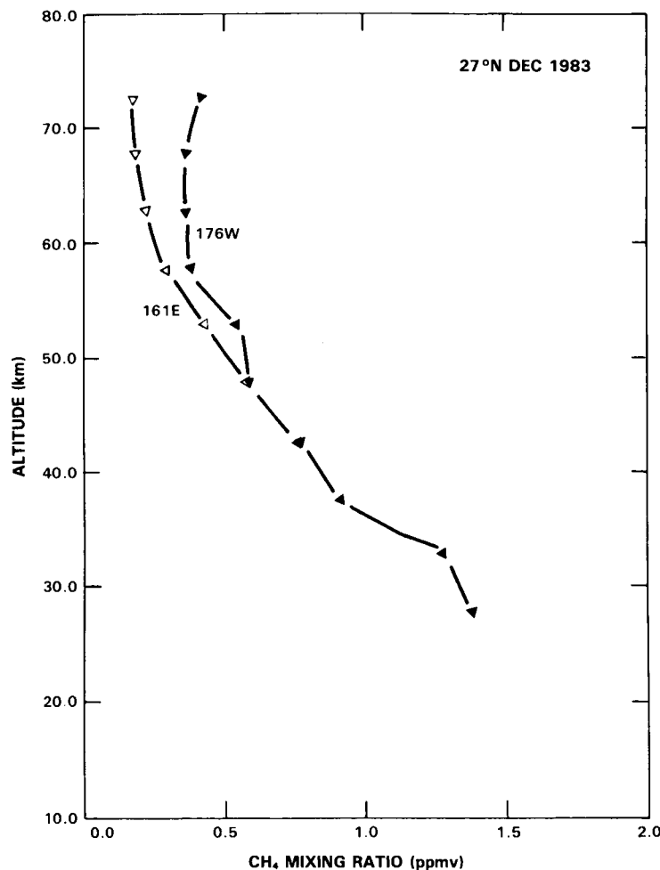
Figure 9-31. Profiles of CH 4 (ppmv) measured by the grille spectrometer on Spacelab One (Ackerman et al. , 1985). Errors on the data are estimated to be \pm 15\% . The two profiles were obtained 1.5 hours apart.
