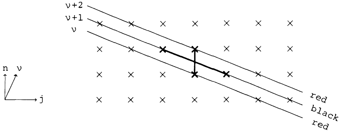
Figure 1. The SOR stencil superimposed on a space-time grid (one space dimension). Introduction of the “tilted” time index \nu makes the stencil symmetric, so that Fourier analysis can be applied. The red-black labels are explained in Section 4.
