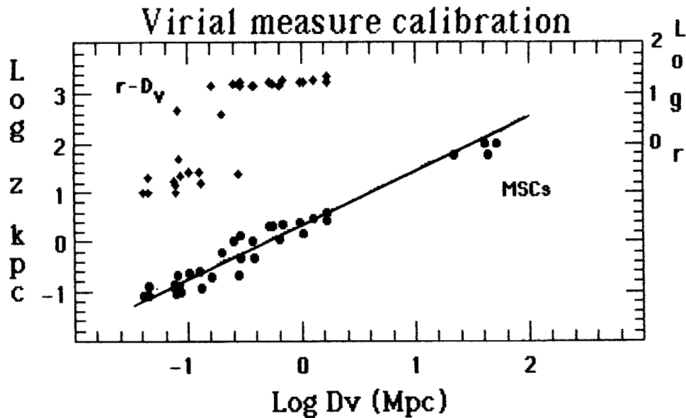
Figure 1. The calibration of the Virial Measure in terms of z-distance. Filled circles represent clouds, or averages for groups of up to 120 clouds, whose distances have been estimated by the original authors or were kinematically derived in the present work. Small plus signs indicate distance from the sun with the axis shifted 2 units. The Magellanic Stream Clouds are represented by four points at the right, but these were not used to determine the best-fit line.
