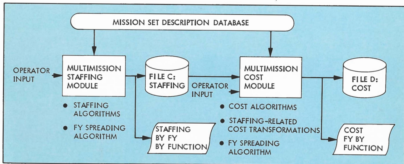
Figure II-3. Multi-Mission Configuration
