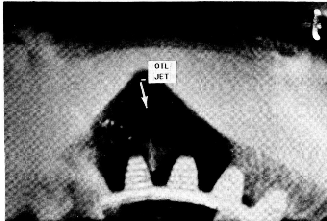
FIGURE 13. - RADIAL JET LUBRICATION 5000 rpm OIL JET PRESSURE 21 \text{ N/cm}^2 (30psi).
