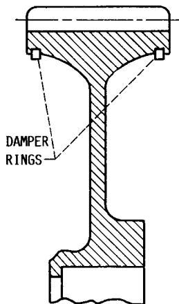
FIGURE 4. - GEAR WITH VIBRATION DAMPER RINGS.
