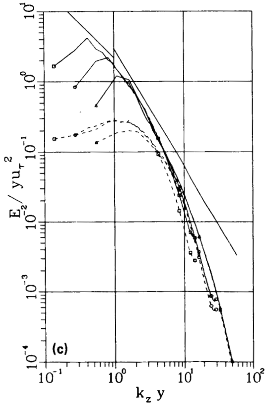
Figure 23. Spectra, normalized using y . a) x direction; — \langle u^2 \rangle ; --- \langle v^2 \rangle . b) x direction; - - - \langle w^2 \rangle ; ... \langle uv \rangle . c) z direction; — \langle u^2 \rangle ; - - - \langle v^2 \rangle . d) z direction; - - - \langle w^2 \rangle ; ... \langle uv \rangle . \square y^+ = 50 ; \circ y^+ = 100 ; \triangle y^+ = 200 .
