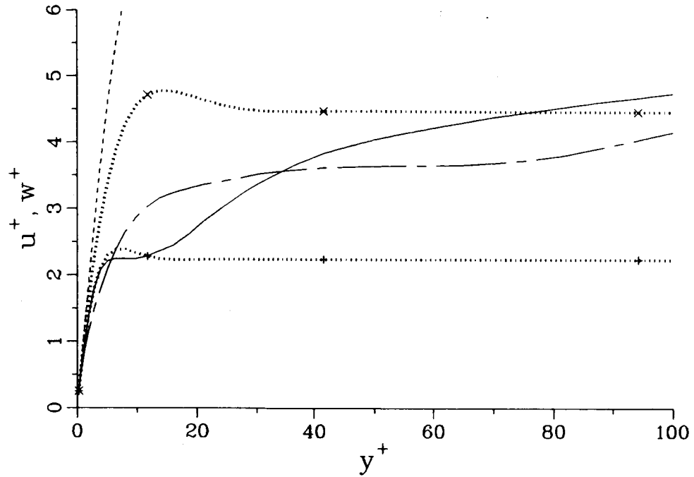
Figure 16. Profiles of inactive-motion rms. Energy difference between R_\theta = 670 and 1410: — \langle u^2 \rangle , - - - \langle w^2 \rangle . Stokes-layer model: + n^+ = 0.2 , x n^+ = 0.05 . - - - law-of-the-wall model.
