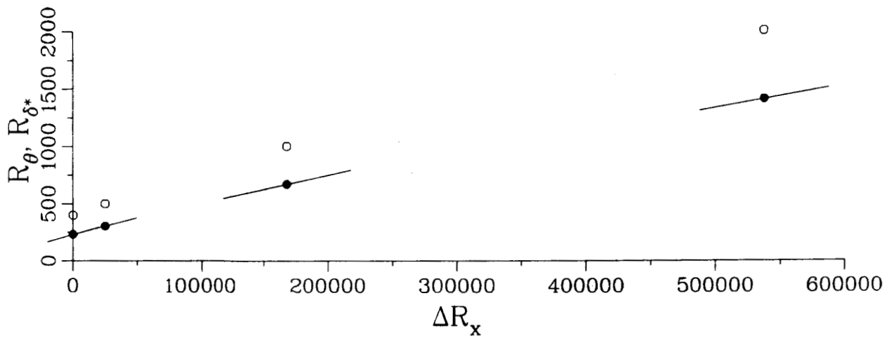
Figure 3. Streamwise thickening of the boundary layer. ○ displacement thickness \delta^* ; ● momentum thickness \theta ; —●— slope c_f/2 .
