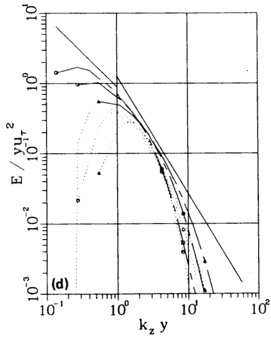
Figure 23. Spectra, normalized using y . a) x direction; — \langle u^2 \rangle ; --- \langle v^2 \rangle . b) x direction; - - - \langle w^2 \rangle ; ... \langle uv \rangle . c) z direction; — \langle u^2 \rangle ; - - - \langle v^2 \rangle . d) z direction; - - - \langle w^2 \rangle ; ... \langle uv \rangle . \square y^+ = 50 ; \circ y^+ = 100 ; \triangle y^+ = 200 .
