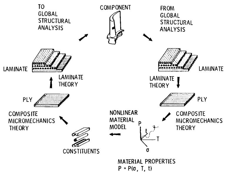
FIGURE 9. - NONLINEAR COBSTRAIN SIMULATION OF HIGH TEMPERATURE METAL MATRIX COMPOSITES.
