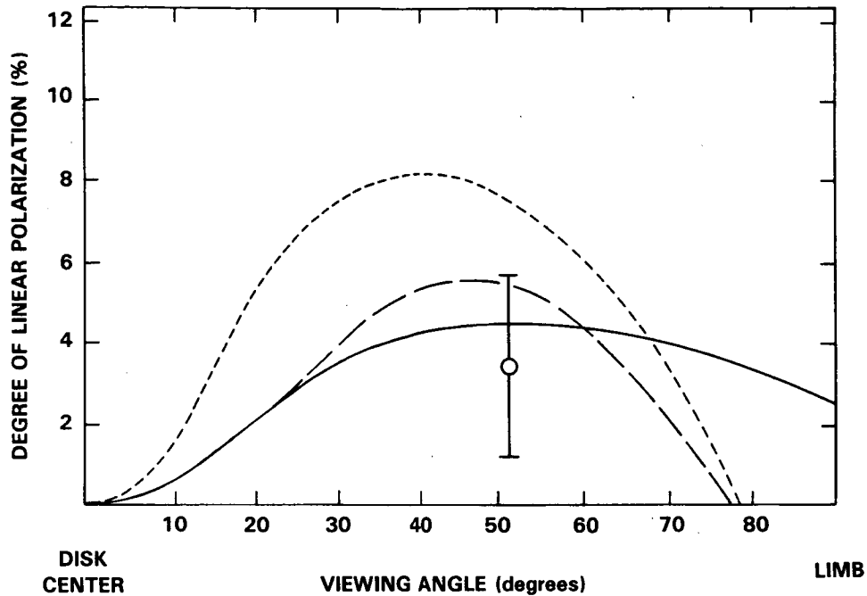
Figure 3.13 A comparison between the polarization measured for flare 2l of Tramiel et al. (1984) and the polarization calculated for three of the models of Leach and Petrosian (1983). For the solid line \alpha_0^2 = 0.4 and d\ln B/d\tau = 0.0 , the dashed line \alpha_0^2 = 0.4 and d\ln B/d\tau = 1.5 \times 10^{-9} , and for the dotted line \alpha_0^2 = 0.1 and d\ln B/d\tau = 1.5 \times 10^{-9} . A value of d\ln B/d\tau = 1.5 \times 10^{-9} corresponds to a twentyfold increase in the magnetic field strength from the top of the loop to the transition region at N_{tr} = 10^{19}\text{cm}^2 . For a flare at disk center the viewing angle would be 0^\circ ; for one on the solar limb it would be 90^\circ (from Leach et al. , 1984).
