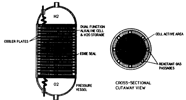
Figure 11. Dual Function Alkaline Cell Stack
