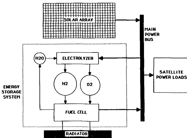
Figure 1. Satellite Energy Storage System
