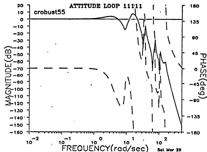
Figure 20. Tilt Angle (rad)/Gimbal Point Torque (N-m) All Loops Closed. First 2 Modes Reduced in Frequency by 20%.
