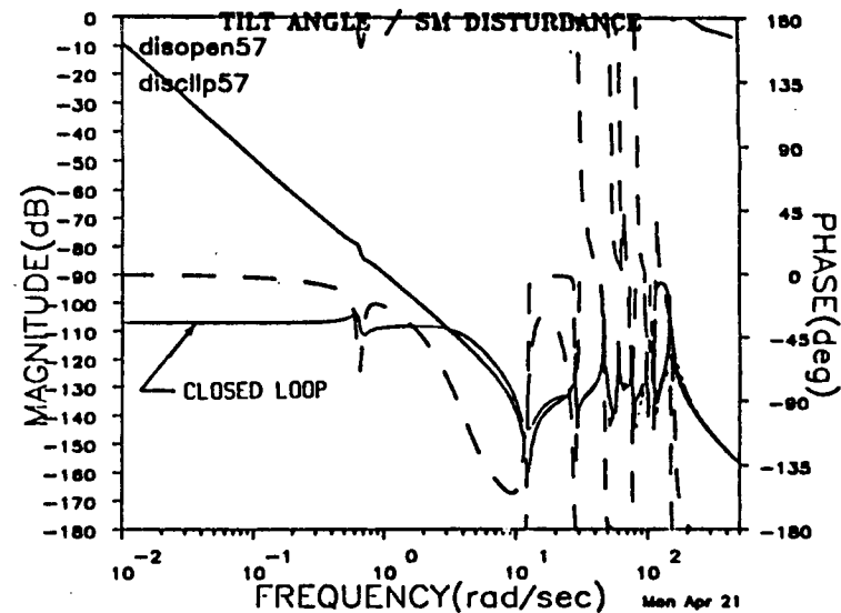
Figure 24 Tilt Angle (Rad)/SM Coolant Disturbance, Open Loop and with all Loops Closed.
