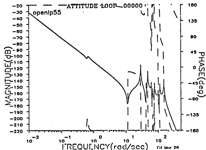
Figure 10. Tilt Angle (Rad)/Gimbal Point Torque (N-m), all Feedback Paths Open.
