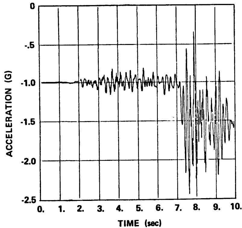
TIME HISTORY
