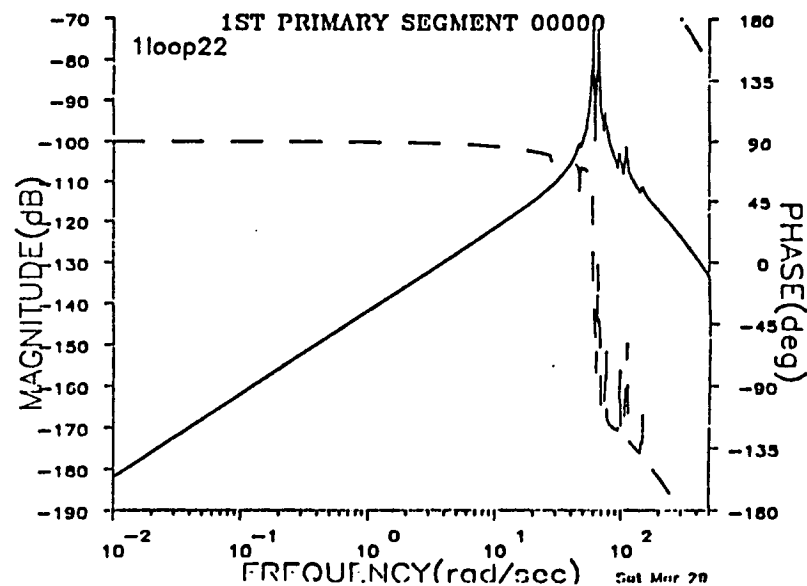
Figure 8. 1st Primary Mirror Rate (rad/sec)/1st Primary Mirror Applied Torque (N-m) all Feedback Paths Open.
