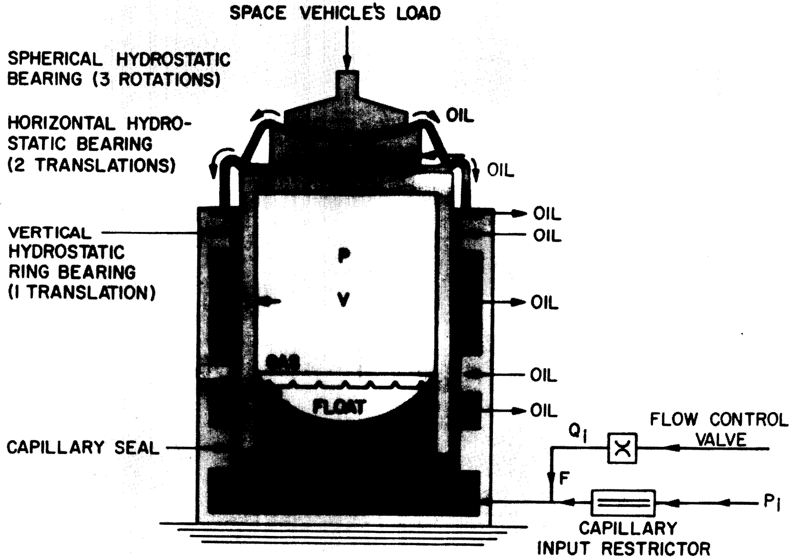
SCHEMATIC OF HYDRAULIC SUPPORT UNIT
