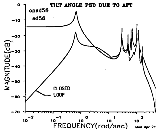
Figure 26 Tilt Angle PSD Due to AFT Body Disturbance, Open Loop and with all Loops Closed \text{dB}=10 \log_{10} (\text{Mag}) .
