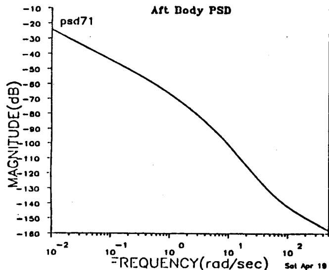
Figure 25 AFT Body Disturbance PSD \text{dB}=10 \log_{10} (\text{Mag})
