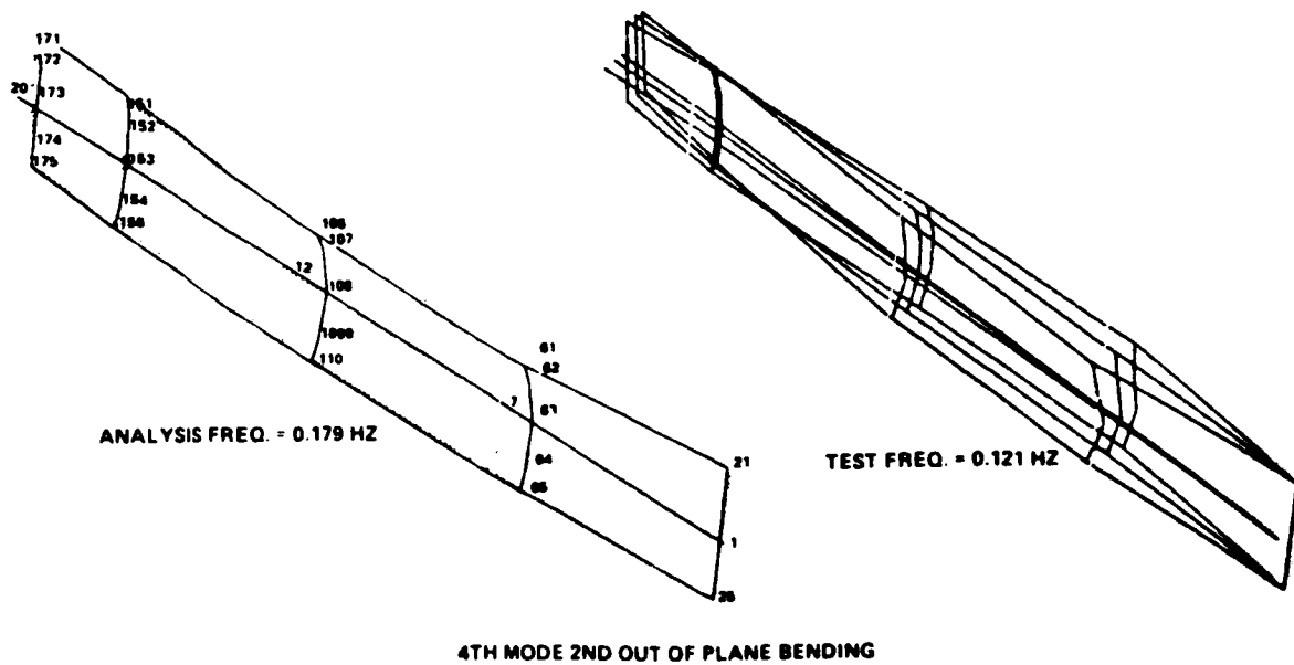
FIGURE 11. SOLAR ARRAY DYNAMICS ANALYSIS/TEST COMPARISON
