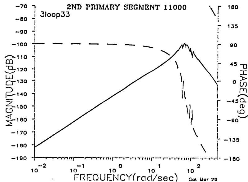
Figure 12. 2nd Primary Mirror Rate (rad/sec)/2nd Primary Mirror Applied Torque (N-m) SM, and 1st PM Loops Closed.
