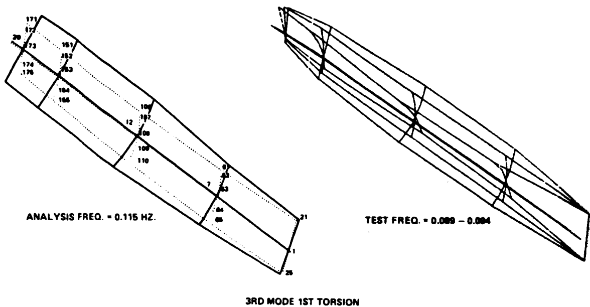
FIGURE 10. SOLAR ARRAY DYNAMICS ANALYSIS/TEST COMPARISON
