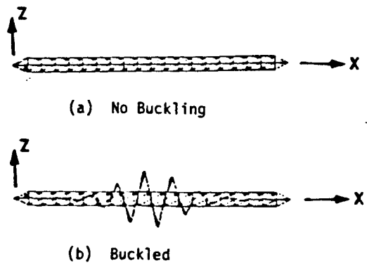
Figure 3 Buckling Mode of a 20-bay Feed Support Structure (Top View)
