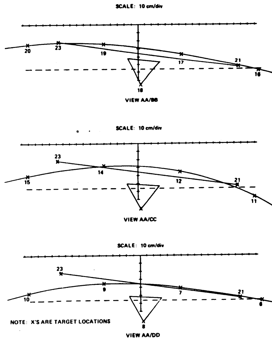
FIGURE 7. BLANKET CURVATURE FIRST SAFDE TEST
