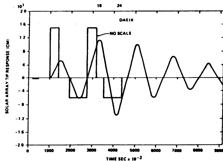
FIGURE 5. 1ST SAFDE ORBITER IMPULSE INPUT AND SOLAR ARRAY TIP RESPONSE
