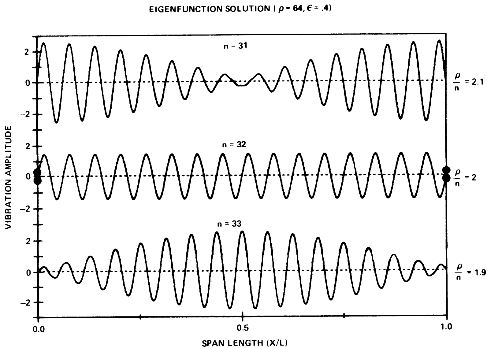
FIGURE 4 EIGENFUNCTION SOLUTIONS NEAR THE ANOMALY, \rho/n = 2
