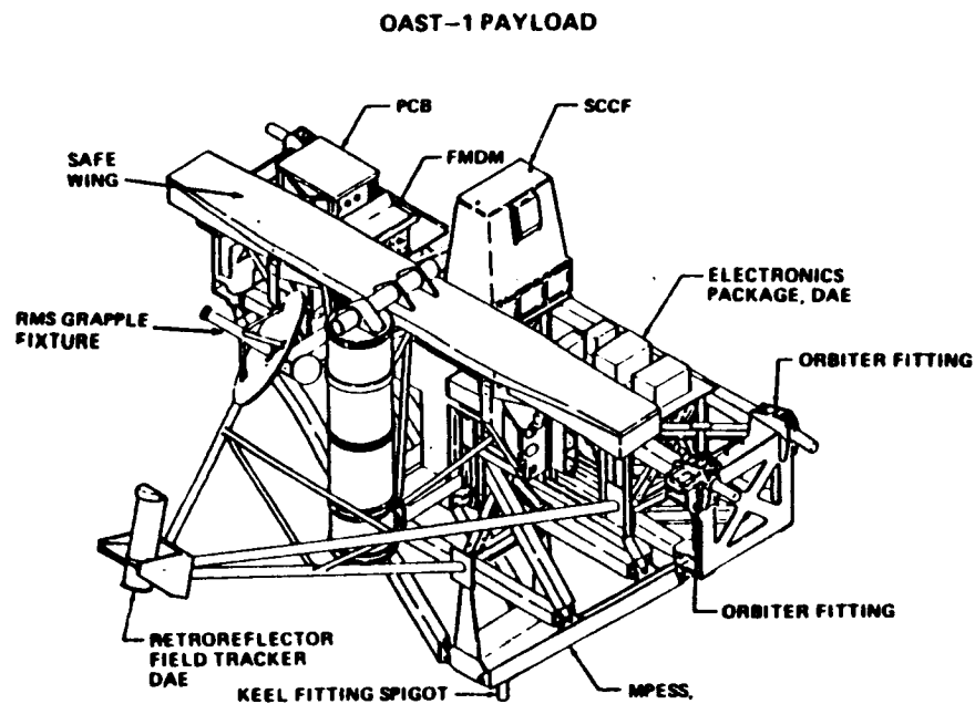
FIGURE 4 OAST-1 SAFE/DAE FLIGHT CONFIGURATION
