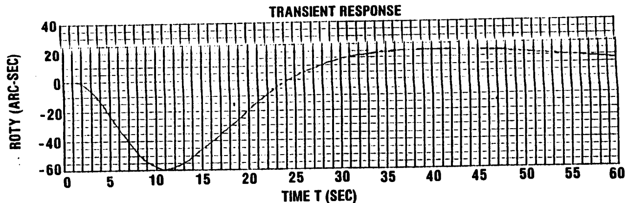
Y—ROTATION AT BASE
