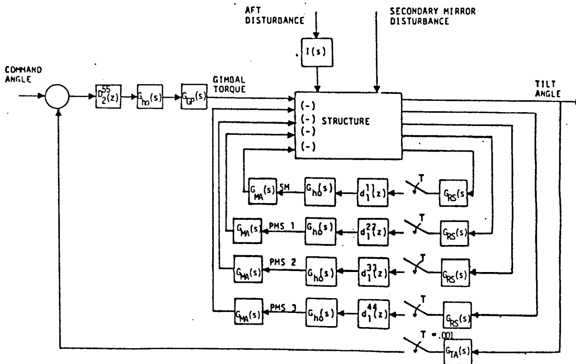
Figure 6. Block Diagram For OSBL
