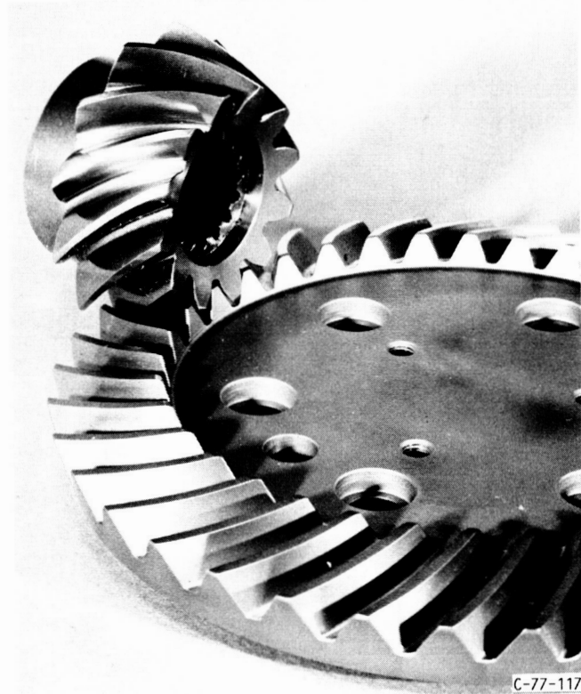
FIGURE 13. - NASA LEWIS BEVEL GEAR APPARATUS TEST GEARS.
