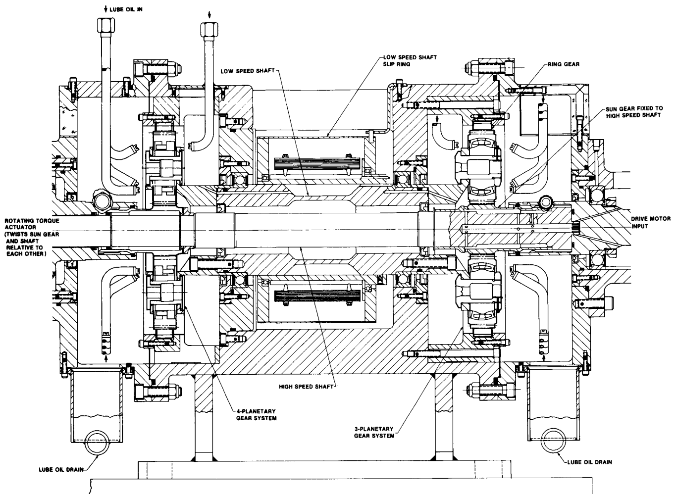
FIGURE 8. - NASA LEWIS PLANETARY GEAR TEST STAND.
