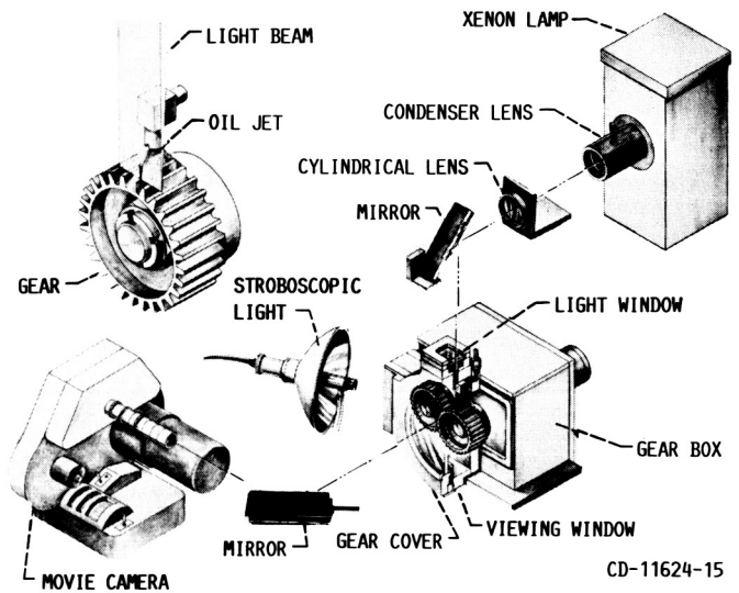
FIGURE 11. - THE NASA LEWIS GEAR FATIGUE TEST APPARATUS MODIFIED FOR OIL JET PENETRATION STUDIES.
