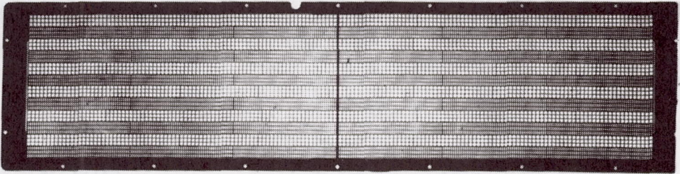
Figure 3. A cross-sectional photograph of the MED collimator showing cellular structure providing 3^\circ \times 3^\circ and 3^\circ \times 1.5^\circ dual collimation.
