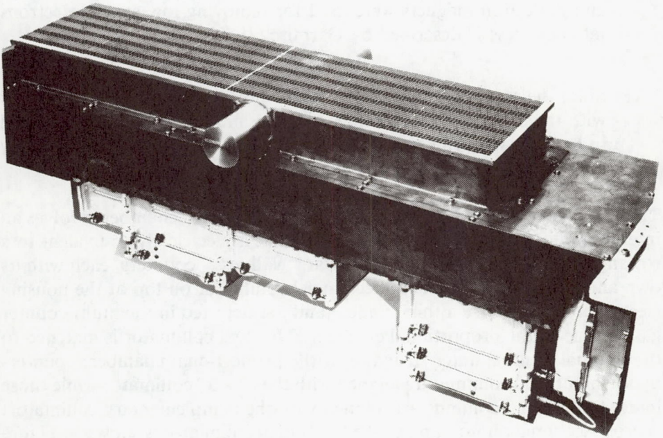
Figure 2. Photograph of a medium energy detector (MED) for the HEAO-1 (A2) experiment; overall length is about one meter. X-rays enter via mechanical collimator on top of housing. Boxes attached to bottom of detector housing are for associated electronics.
