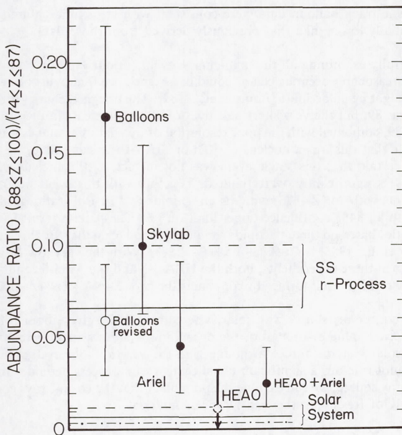
Figure 4. The abundances of “actinides”: ( 88 \leq Z \leq 100 ) relative to “Pt-Pb” ( 74 \leq Z \leq 87 ). Data are from balloons [Fowler et al., 1977], Skylab [Shirk and Price, 1978], Ariel-6 [Fowler et al., 1985], and HEAO-3 [Binns et al., 1985]. The revised balloon point is from O’Sullivan [1985]. Expected values [Blake et al., 1978] are solid lines without FIP fractionation and dashed lines with FIP fractionation, for sources with composition of the solar system at the time of its formation or for a source with the composition of freshly synthesized r -process material. The dot-dash solar system line substitutes present-day abundances for the (solid line) abundances at the formation of the solar system.
