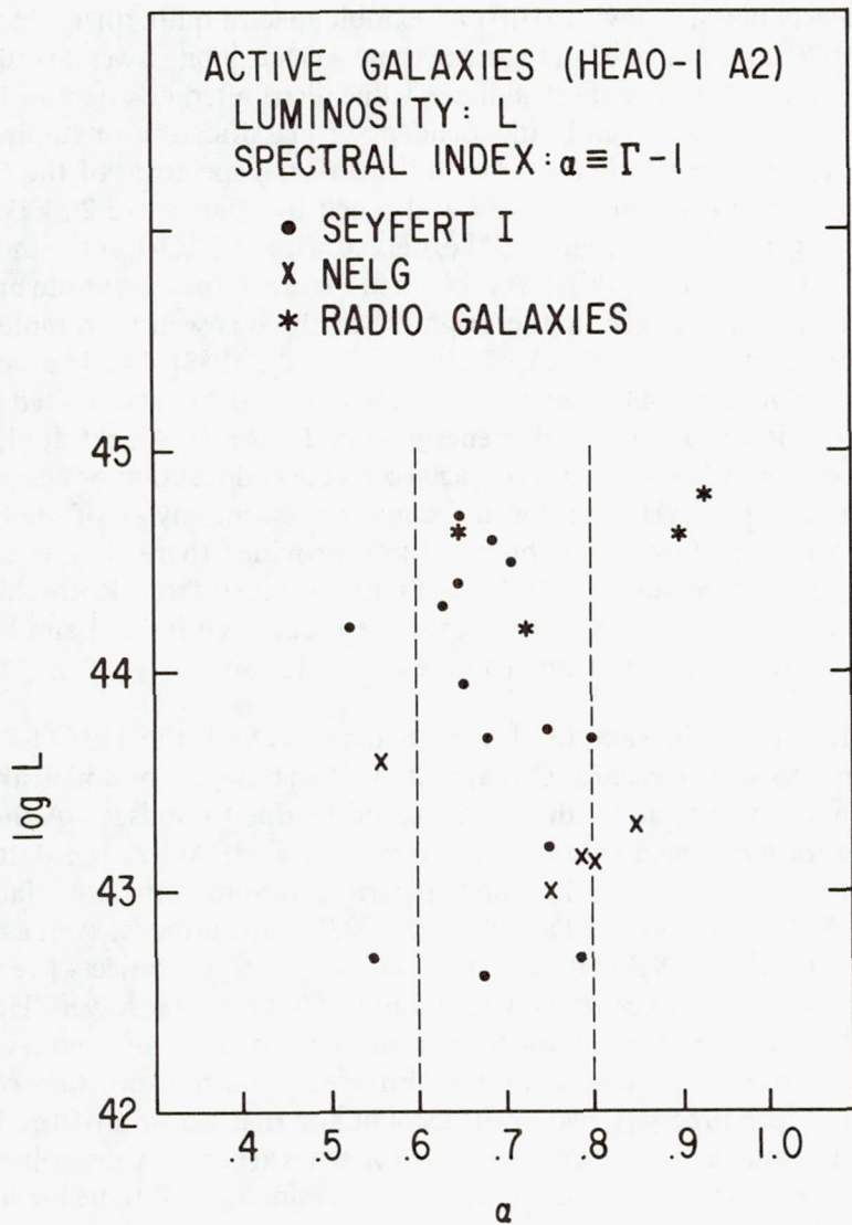
Figure 6. Active galaxies measured with the HEAO-1 (A2) experiment [Mushotzky, 1982] plotted with regard to X-ray luminosity ( L ergs s^{-1} ) below 20 keV and energy spectral index \alpha .
