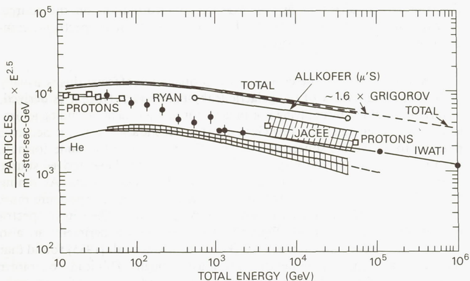
Figure 5. Observed spectra compared with various source spectra. Proton and possibly helium are consistent with source spectra with indices 2.1. Heavier nuclei, on the other hand, may require steeper source spectra. [This figure is from Engelmann et al., 1985. Original references can be found therein.]
