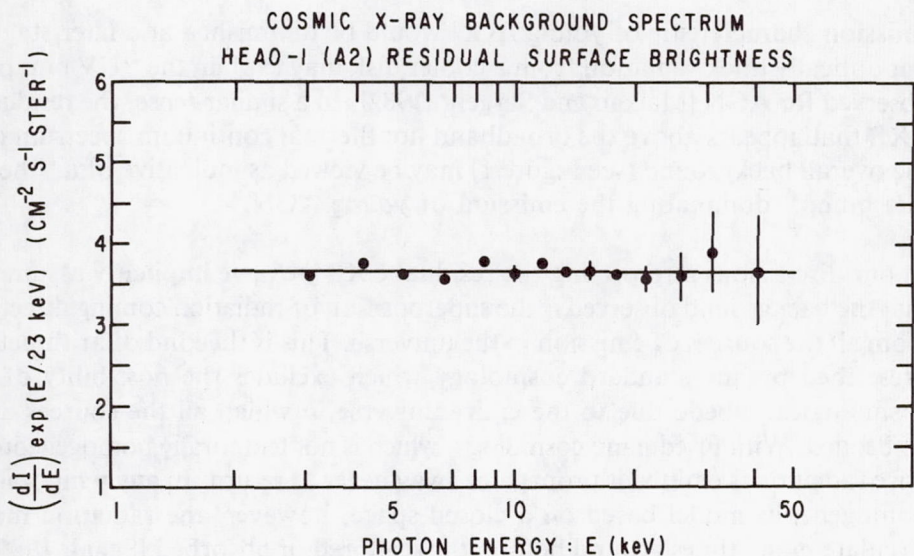
Figure 11. The residual energy spectrum for the CXB multiplied by \exp(E/23 \text{ keV}) as a function of photon energy [Leiter and Boldt, 1982]. In general, the statistical errors associated with the data points increase with energy and are indicated only for representative energies ( \sim 5 \text{ keV} , 10 \text{ keV} and > 20 \text{ keV} ).
