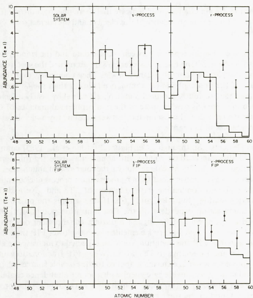
Figure 2. Comparison of our measured abundances (data points) with those expected at Earth after galactic propagation, through an exponential path length distribution with mean 5.5 \text{ g/cm}^2 from sources with solar system abundances [Anders and Ebihara, 1982], s-process abundances [Kaeppeler et al., 1982], or r-process abundances [Krombel, 1983]. The upper panels assume no FIP fractionation and the lower panels assume exponential FIP fractionation of the form 9.31 \exp(-0.288\text{FIP}) .
