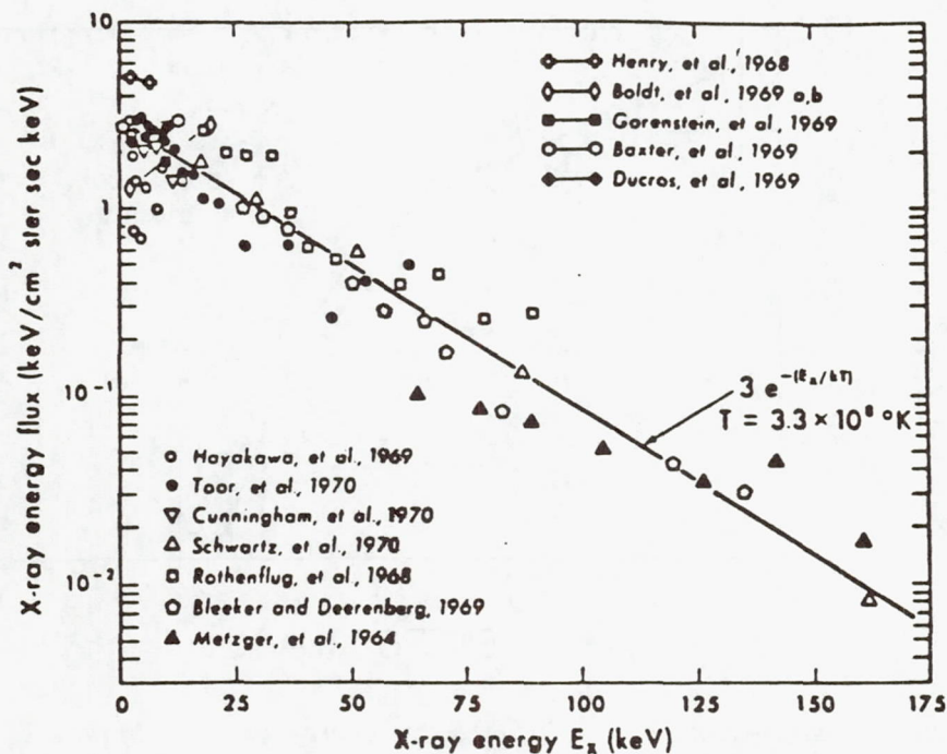
Figure 5. The difference between the observed energy flux and the calculated flux in the energy interval 2 keV E_x 200 keV is plotted as a function of X-ray energy. The line represents the thermal-bremsstrahlung emission for a hydrogen plasma at 3.3 \times 10^8 K. The line-of-sight integral \int N_e N_p dl for this emission is 1.3 \times 10^{17} \text{ cm}^{-3} . If one assumes no clumping and \int dl \approx 2c/3H_0 \approx 10^{28} \text{ cm} , one gets N_e \approx N_p \approx 3 \times 10^{-6} \text{ cm}^{-3} . Such a density is adequate to close the Universe if H_0 \approx 55 \text{ km s}^{-1} \text{ Mpc}^{-1} . Cowsik and Kobetich, 1972, Astrophys. J. , 177, 585.
