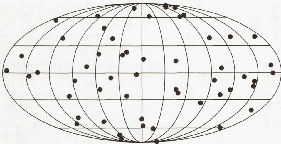
Figure 5. One source distribution pattern of gamma ray bursts [Atteia et al., 1986], seen to be consistent with isotropy. Different instruments produce their individual catalogs; this one was recently compiled with observations from the interplanetary network.
