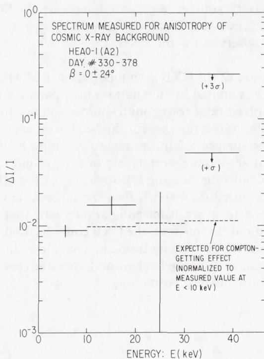
Figure 14. The fore-aft asymmetry ( \Delta I/I ) of the cosmic X-ray background, as measured with the HEAO-1 (A2) experiment, is exhibited as a function of photon energy E (keV). The reference direction is that defined by ecliptic coordinates: \beta (latitude) = 0^\circ and \lambda (longitude) = 178^\circ , corresponding to \delta (declination) = 1^\circ and \alpha (right ascension) = 178^\circ . The average surface brightness for a region 48^\circ \times 48^\circ ( \Delta\beta \times \Delta\lambda ), centered on the reference direction, is compared with that for an equivalent region in the opposite direction. Resolved sources, brighter than 2.1 \times 10^{-11} ergs \text{cm}^{-2} \text{s}^{-1} (2-10 keV), have been excluded in the sample analyzed. Data were obtained with xenon gas proportional counters (high energy detectors HED-I and HED-III) and an argon counter (MED: medium energy detector) during the 48-day interval when great-circle scans with HEAO-1 covered the regions of the sky considered here. The one-sigma errors shown correspond to photon counting statistics. Dashed lines indicate the asymmetry expected for the Compton-Getting effect (normalized to the value measured for the band 1.3-10.3 keV).
