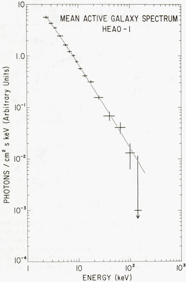
Figure 8. The mean spectrum obtained for a sample of bright AGN observed with the HEAO-1 (A2) and (A4) experiments [Rothschild et al., 1983]. The solid line is the best-fit power law model.
