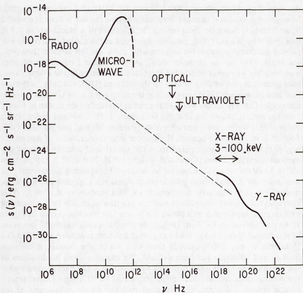
Figure 1. The isotropic sky flux s(\nu) versus frequency \nu [from Shafer, 1983]. The dashed line extends the power law spectrum at radio frequencies to higher photon energies ( E = h\nu ) assuming s(\nu) \propto \nu^{-\alpha} , with \alpha = 0.7 . References are: Clark, Brown, and Alexander [1970] for radio; Weiss [1980] for microwave; Dube, Wickes, and Wilkinson [1979] for optical; Paresce, McKee, and Bowyer [1980] for UV; Marshall et al. [1980] and Rothschild et al. [1983] for X-rays; and Fichtel and Trombka [1981] for gamma rays.
