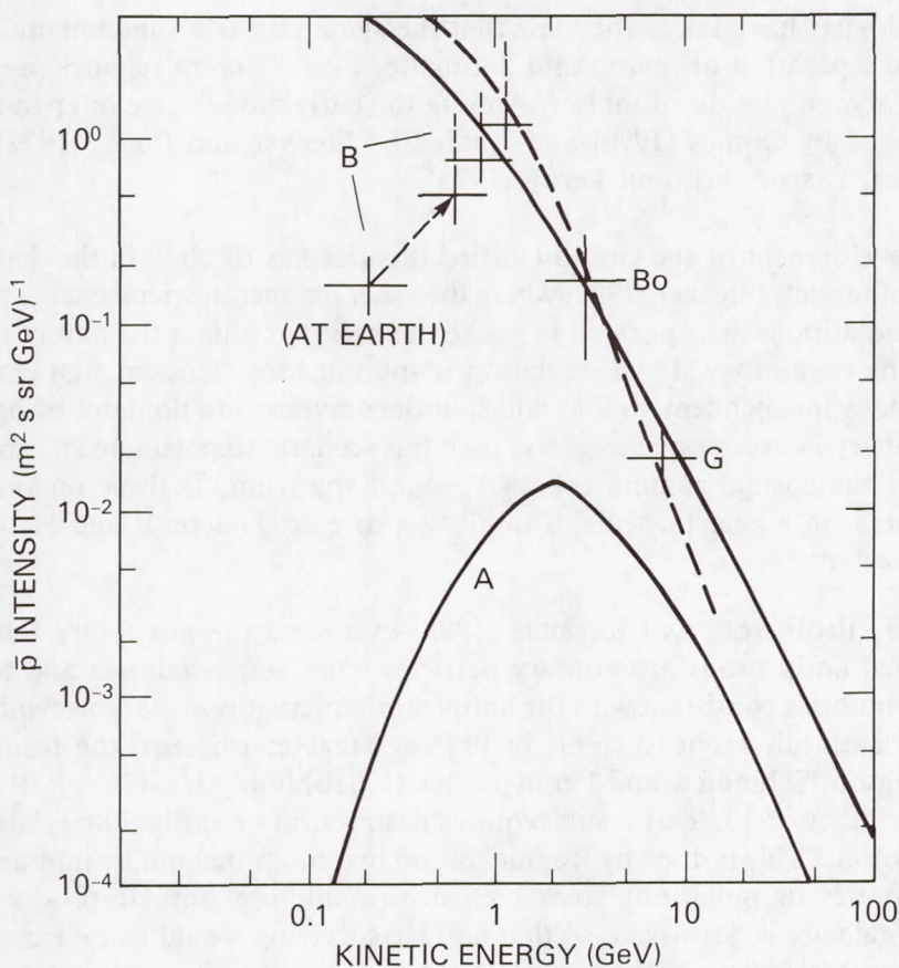
Figure 2. Following Kiraly et al. [1981] and Stecker and Wolfendale [1984] the data are shown with antiproton spectra expected from primordial black holes (dashed curve) and extragalactic antiprotons (solid curve). The differential flux represented by the [Buffington, Schindler, and Pennypacker, 1981b] point has been demodulated assuming three different mean energy losses (see text), adiabatic deceleration, and the applicability of Liouville's theorem. The vertical dashes on the three demodulated points represent plausible uncertainties in this procedure. Both spectra have been normalized at 9 GeV. For comparison, curve A shows the spectrum expected from a leaky box model with 5 \text{ g/cm}^2 .
