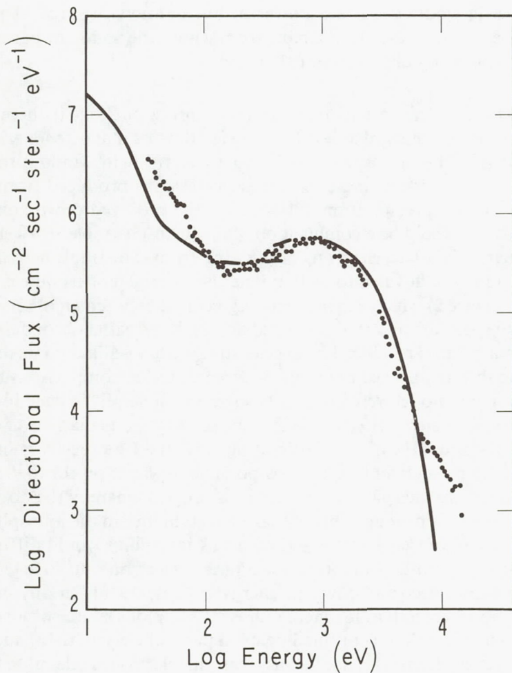
Figure 2. An example of a comparison between an observed auroral electron spectrum and one modeled by accelerating a Maxwellian distribution through a 500 volt field-aligned potential drop, computing the backscatter and secondary population created in the atmosphere by the precipitation, and reflecting that population from the potential barrier back downward. The good agreement overcame one of O'Brien's objections to the existence of parallel electric field acceleration.
