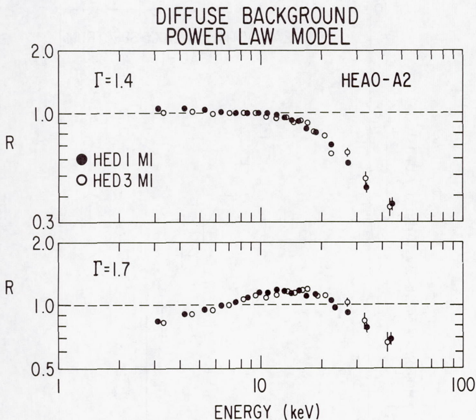
Figure 7. The ratio ( R ) as a function of energy of the counts observed for the X-ray background to that predicted by convolving, with the detector response function, power law spectra characterized by photon number spectral indices \Gamma = 1.4 and \Gamma = 1.7 . Different symbols distinguish data obtained with HED-1 and HED-3 detectors of HEAO-1 (A2). Statistical errors are shown when larger than the size of the symbols [Marshall et al., 1980].
