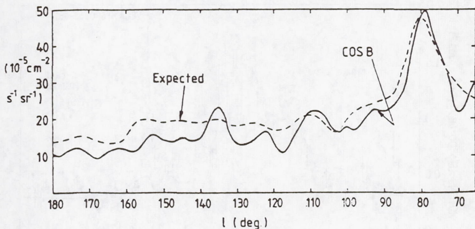
Figure 3. A comparison of the gamma ray intensity ( E_\gamma > 100 MeV) on a longitude along b = 0^\circ between that observed by COS-B [Mayer-Hasselwander et al. 1982] and that calculated by Arnaud et al. [1982] under the assumption of a constant cosmic ray density everywhere at the local galactic value. [This figure is from Arnaud et al., 1982.]
