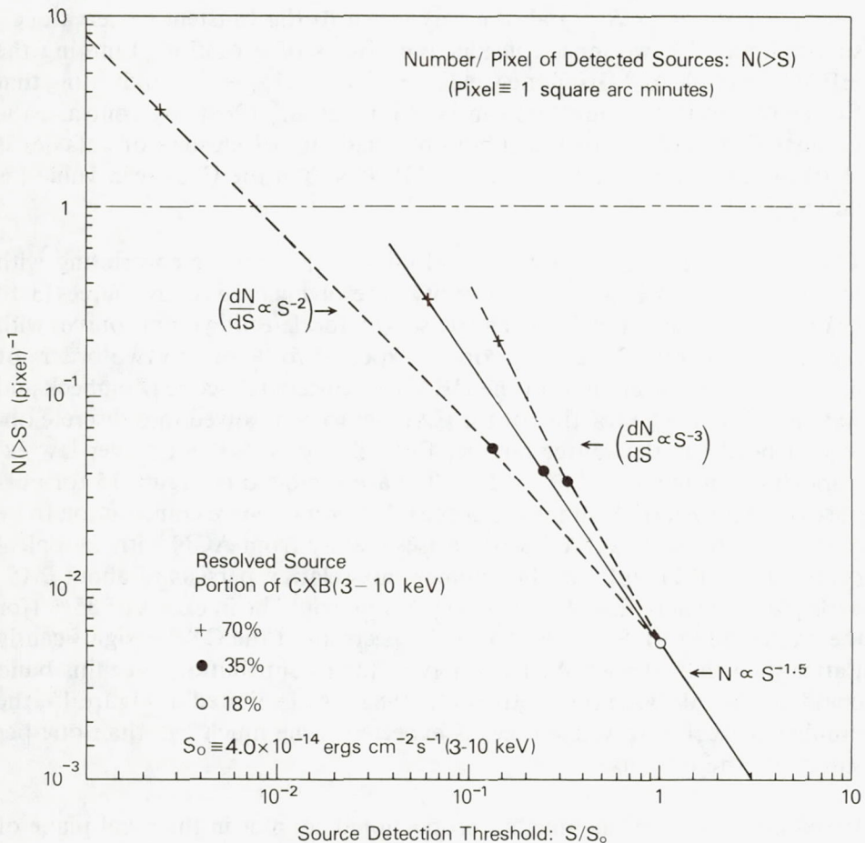
Figure 15. Extrapolation of source counts to S/S_0 < 1 , normalized to HEAO-2 measurements at S/S_0 > 1 [Gioia et al., 1984]. Points designated by various symbols indicate corresponding percentage of the CXB resolved (3-10 keV), shown separately for \gamma = 2, 2.5 and 3 (see text). For an energy spectral index \alpha = 0.7 , S_0 (3-10 keV) = 4.0 \times 10^{-14} \text{ ergs cm}^{-2} \text{ s}^{-1} corresponds to S_0 (1-3 keV) = 2.6 \times 10^{-14} \text{ ergs cm}^{-2} \text{ s}^{-1} of the HEAO-2 deep survey [Giacconi et al., 1979b]. N(>S) , average number of sources per pixel brighter than S , is plotted versus S/S_0 . Pixel size is 1 square arc-minute.
