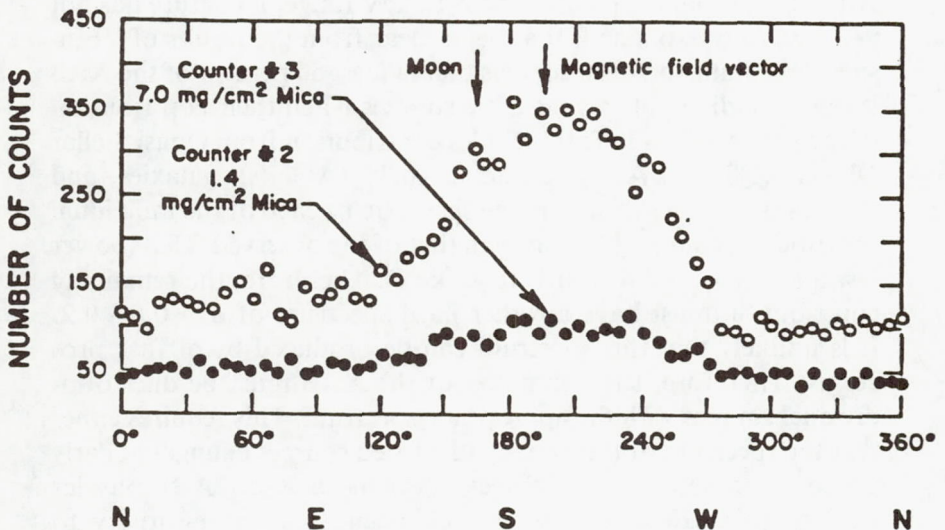
Figure 1. Azimuthal distributions of recorded counts from Geiger counters flown during June 1962. Giacconi, R. and Gursky, H., eds., X-ray Astronomy , D. Reidel Publishing Company, 1974.
