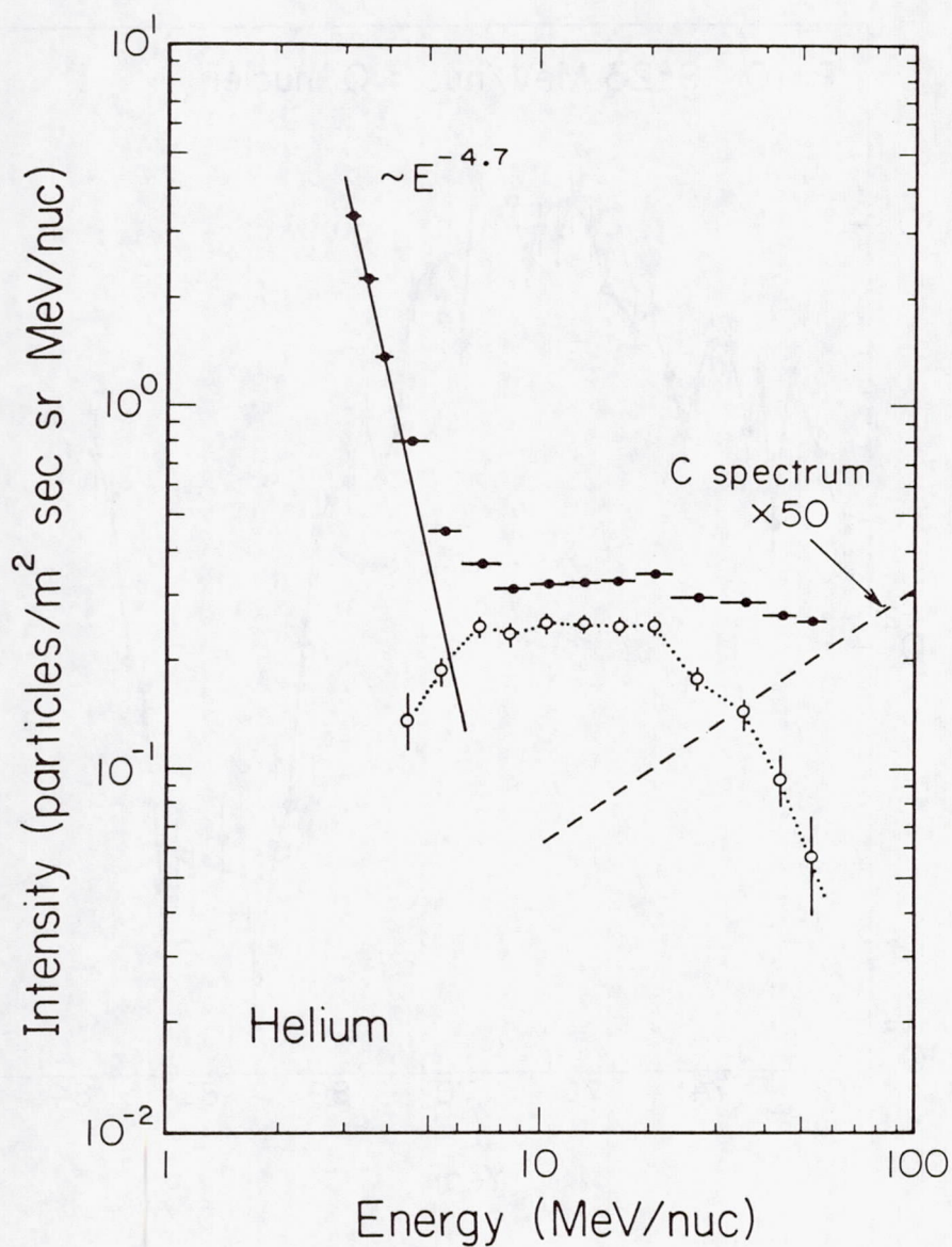
Figure 6. Helium spectrum at low energies showing separation into anomalous and galactic components between 10 and 100 MeV/nuc.
