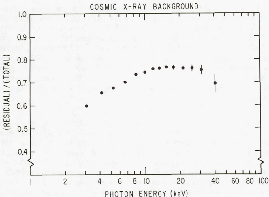
Figure 10. The ratio of the spectral density of the estimated residual CXB [Leiter and Boldt, 1982] to that of the total CXB observed with HEAO-1 (A2), plotted as a function of photon energy, in keV. Statistical errors are indicated for those data points where they exceed the size of the dots.
