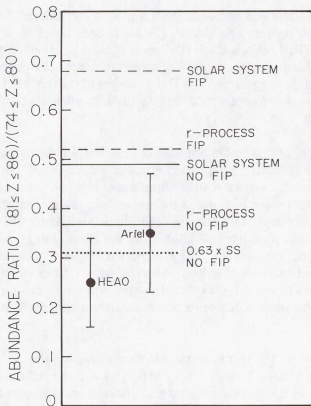
Figure 3. The ratio of "Pb" ( 81 \leq Z \leq 86 ) to "Pt" ( 74 \leq Z \leq 80 ). The data points are observations from HEAO-3 [Binns et al., 1985] and Ariel-6 [Fowler et al., 1985]. The lines are expected values after propagation through an exponential path length distribution with mean 5.5 \text{ g/cm}^2 from sources with standard solar system abundances [Anders and Ebihara, 1982] or r-process abundances derived from those solar system abundances [Fixsen, 1985; Binns et al., 1985]. Solid lines assume no FIP fractionation, which for these elements is equivalent to a step function FIP fractionation with step above 9 eV; dashed lines assume exponential FIP fractionation. Reduction of the solar system Pb abundances as suggested by Grevesse and Meyer [1985] would lower the expected solar system values by a factor 0.63, as indicated by the dotted line, and would cause an even greater reduction in the r-process expectations.
